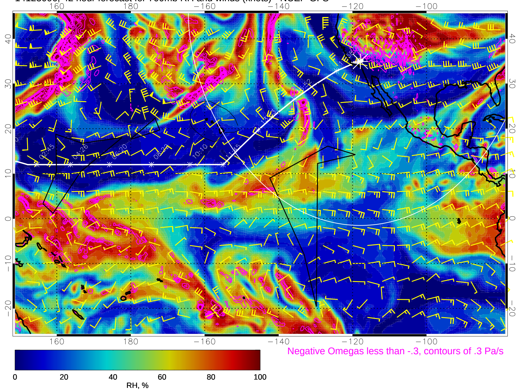
14123006, 42 hour forecast for 700mb RH and winds (knots) - NCEP GFS
