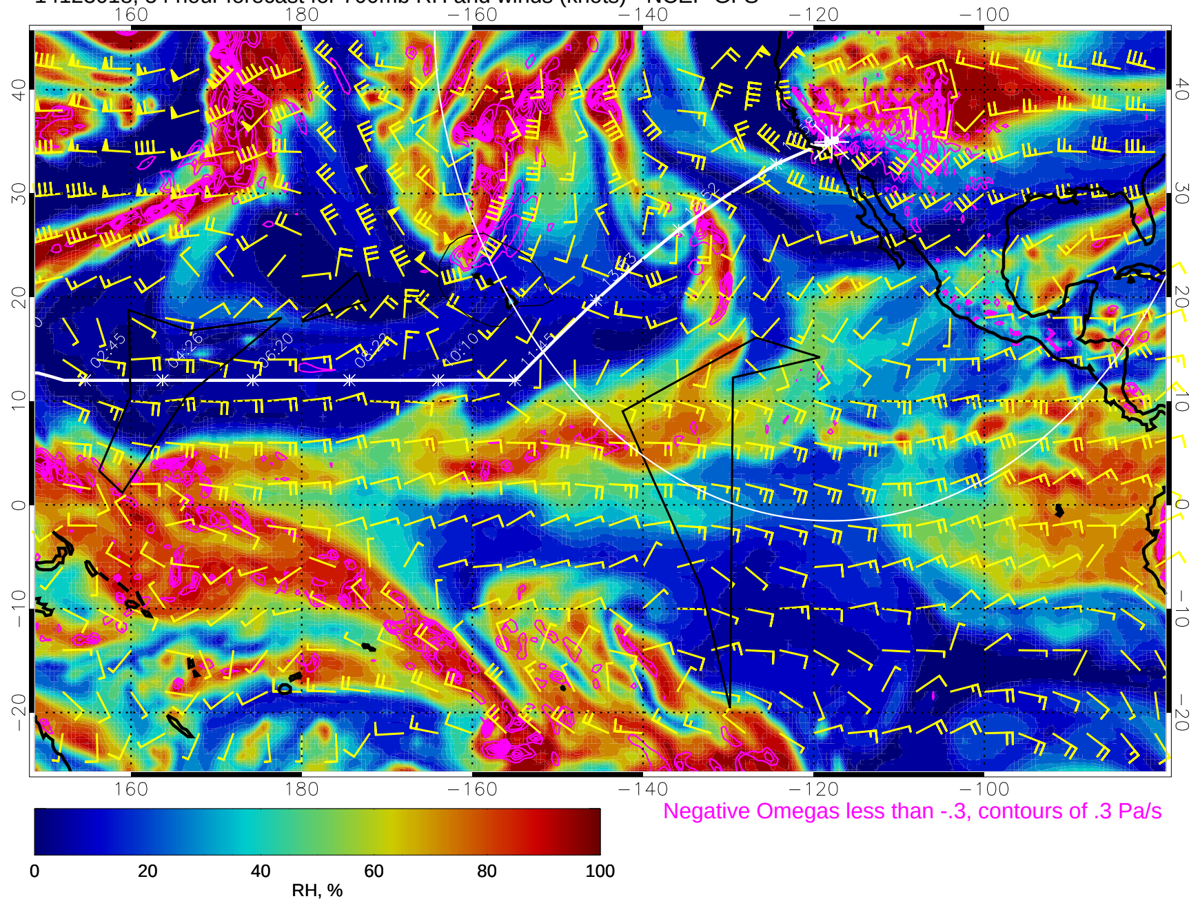
14123018, 54 hour forecast for 700mb RH and winds (knots) - NCEP GFS
