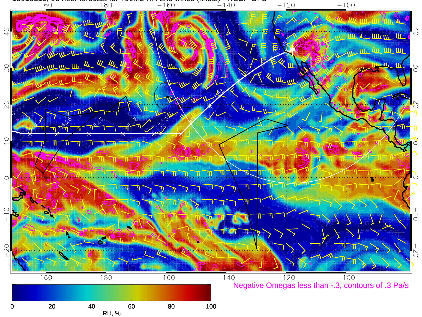
15010112, 96 hour forecast for 700mb RH and winds (knots) - NCEP GFS
