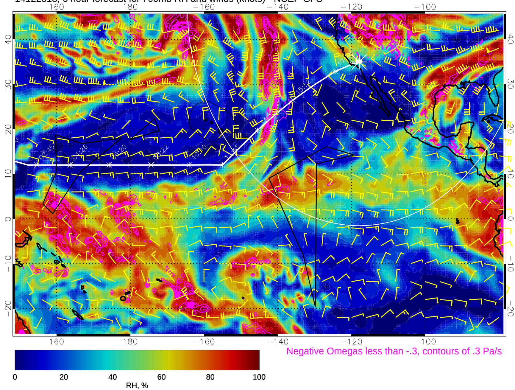
14122818, 6 hour forecast for 700mb RH and winds (knots) - NCEP GFS
