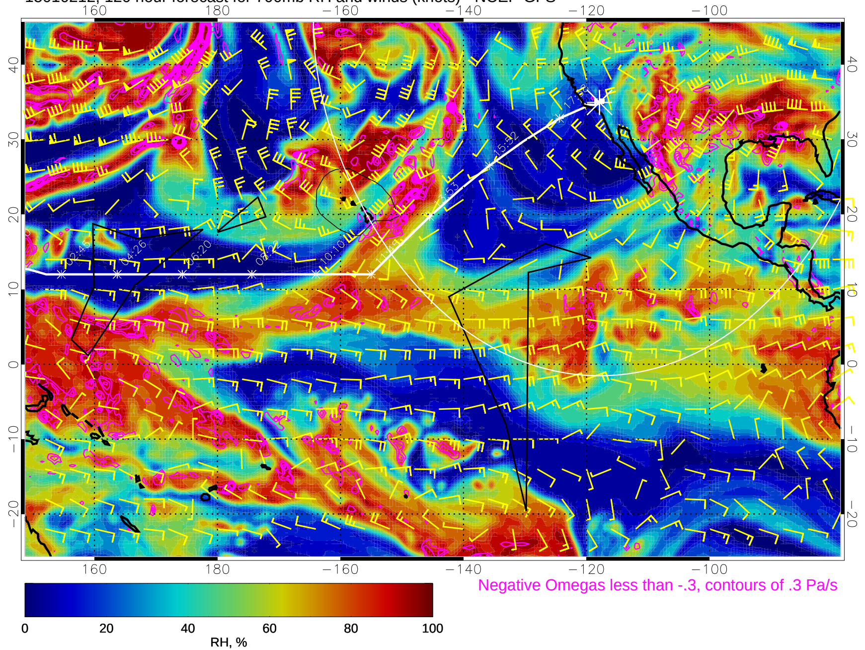
15010212, 120 hour forecast for 700mb RH and winds (knots) - NCEP GFS
