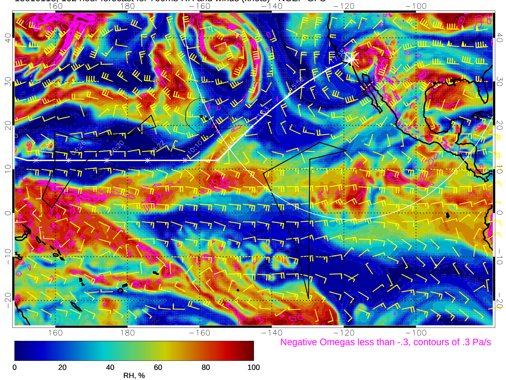
15010118, 102 hour forecast for 700mb RH and winds (knots) - NCEP GFS
