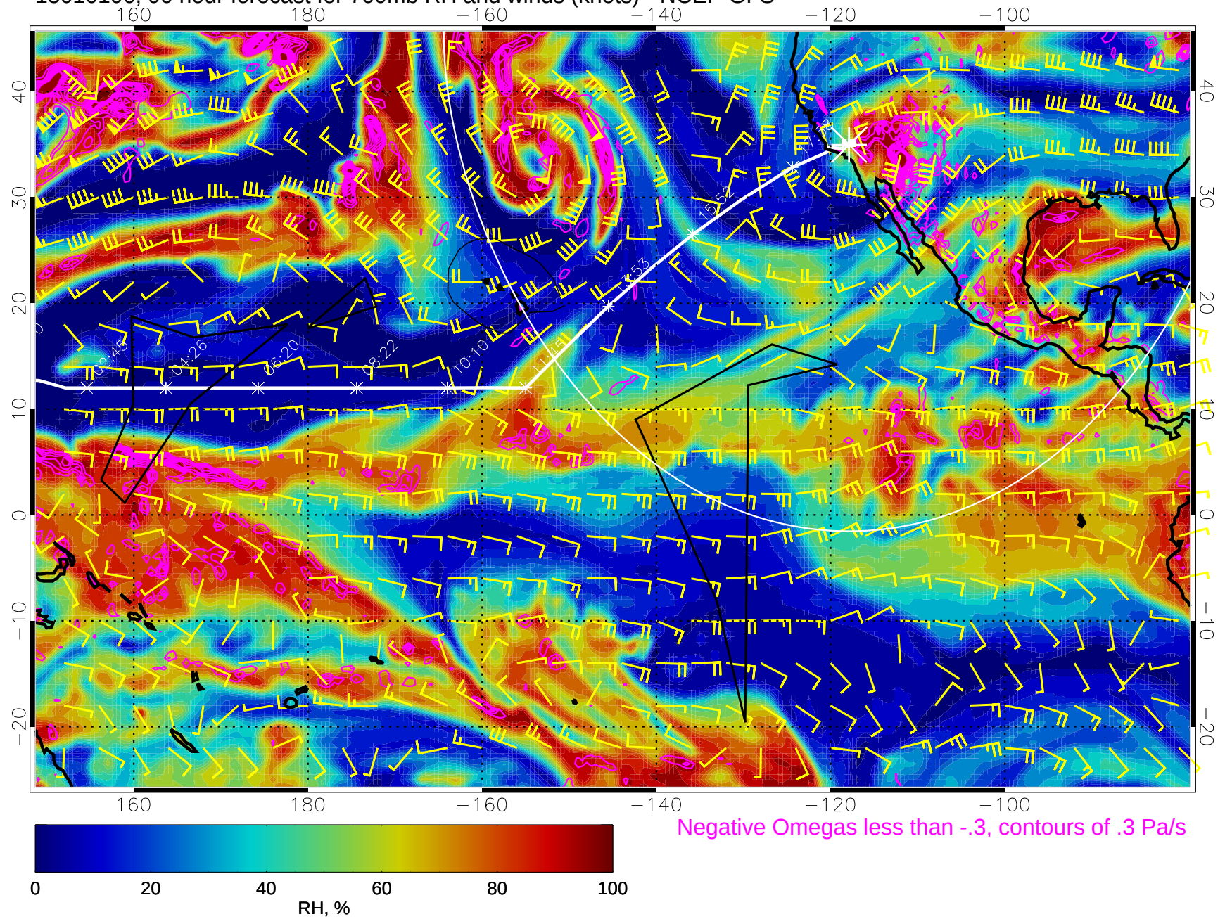
15010106, 90 hour forecast for 700mb RH and winds (knots) - NCEP GFS
