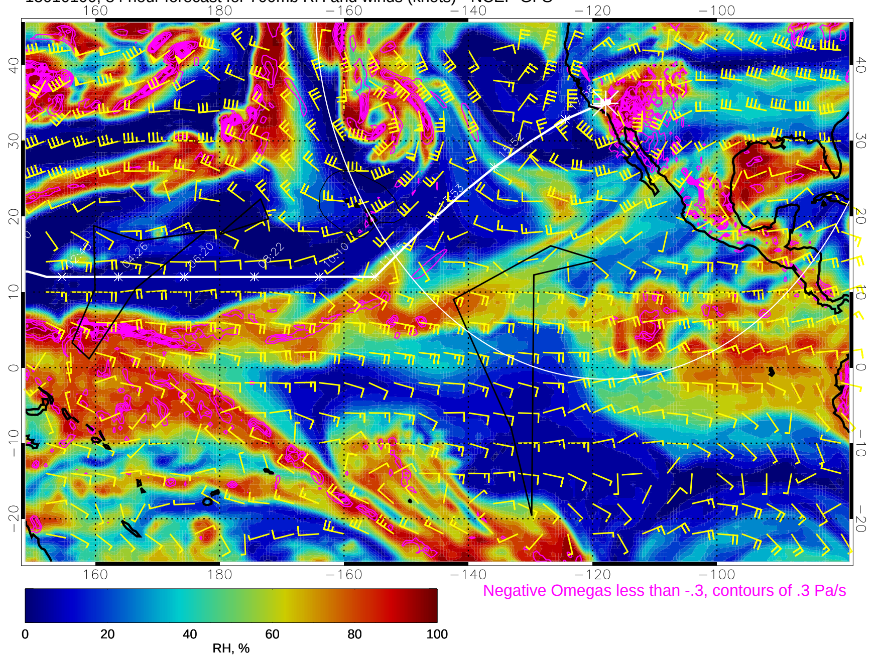
15010100, 84 hour forecast for 700mb RH and winds (knots) - NCEP GFS
