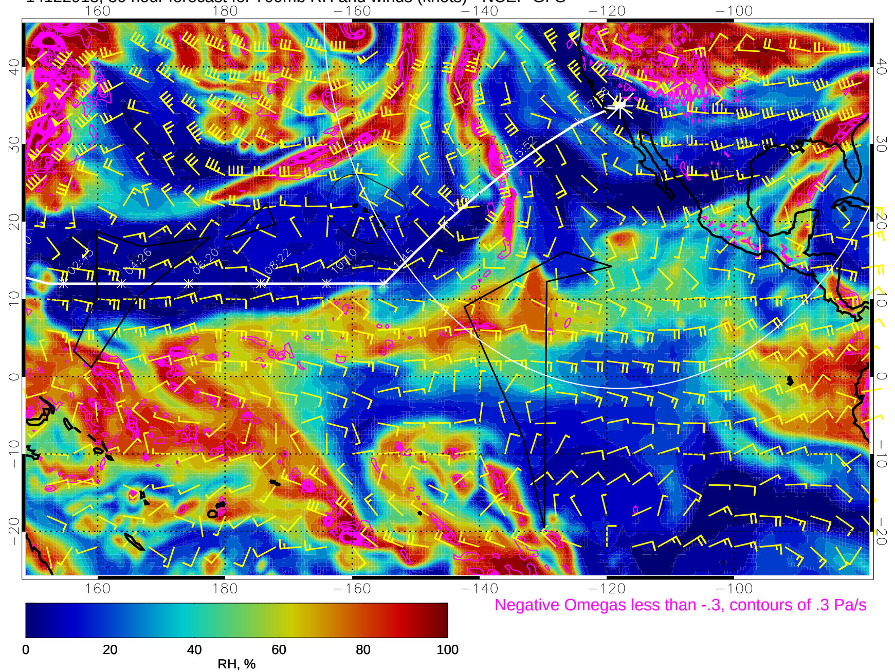
14122918, 30 hour forecast for 700mb RH and winds (knots) - NCEP GFS
