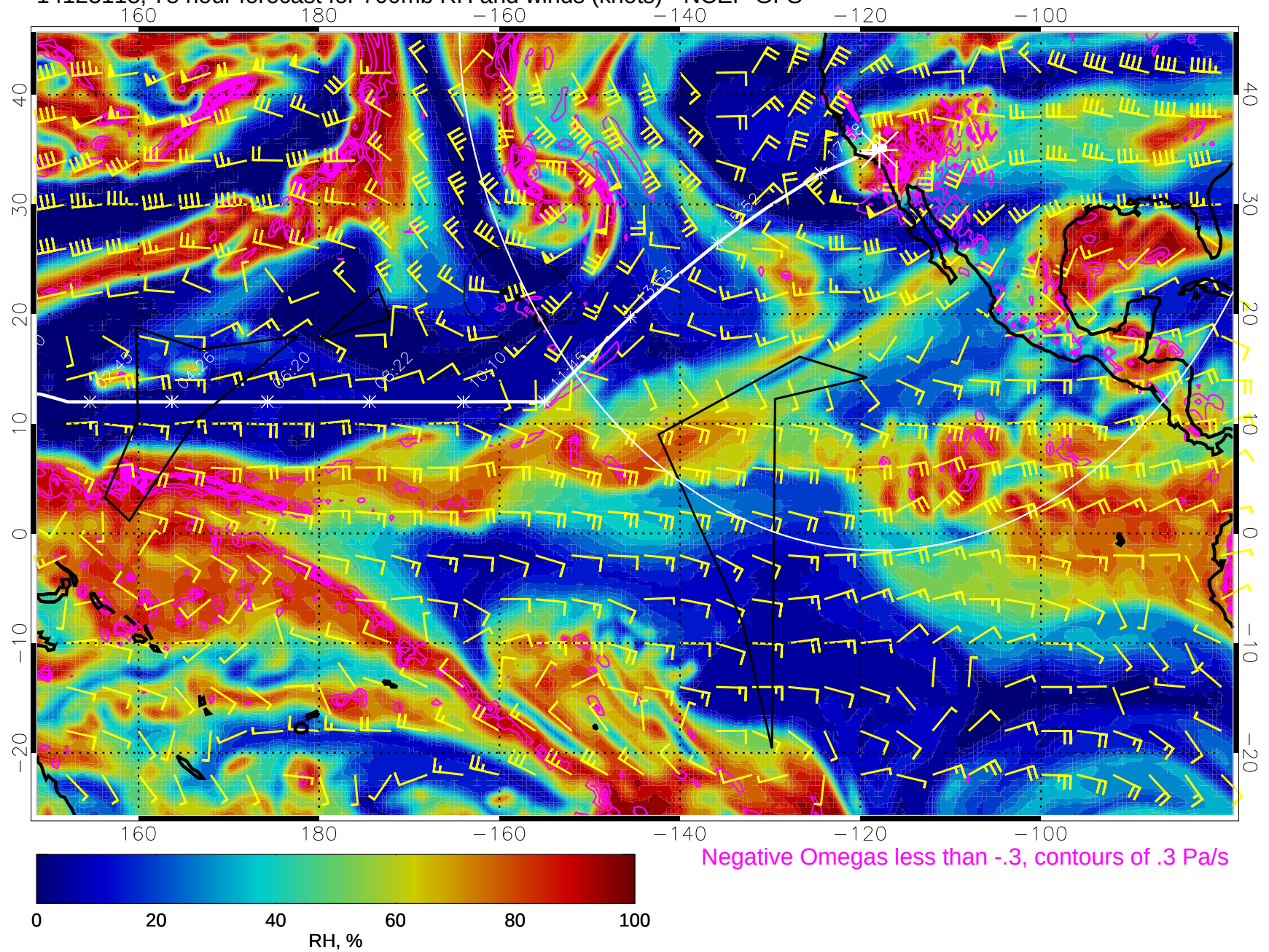
14123118, 78 hour forecast for 700mb RH and winds (knots) - NCEP GFS
