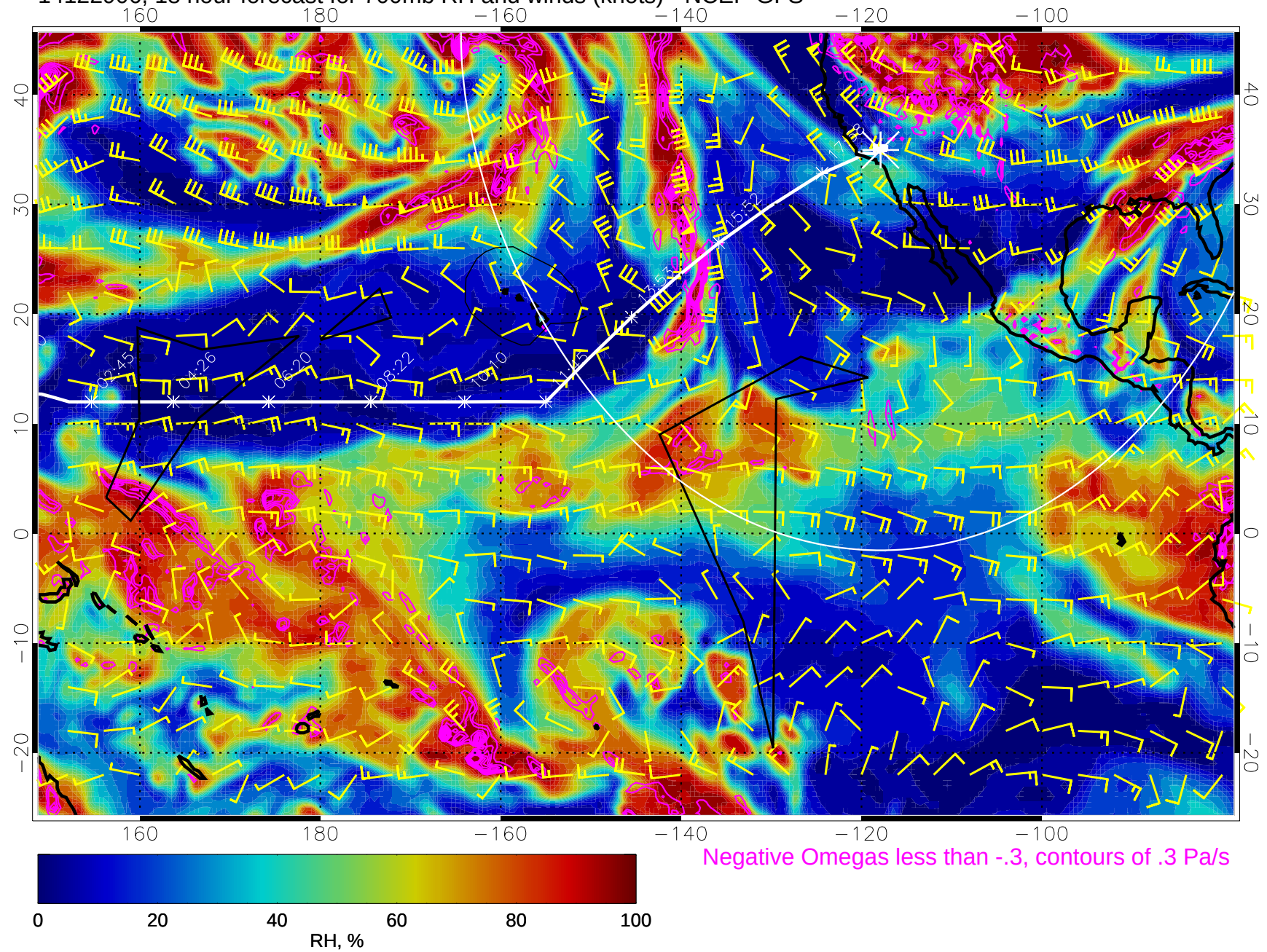
14122906, 18 hour forecast for 700mb RH and winds (knots) - NCEP GFS
