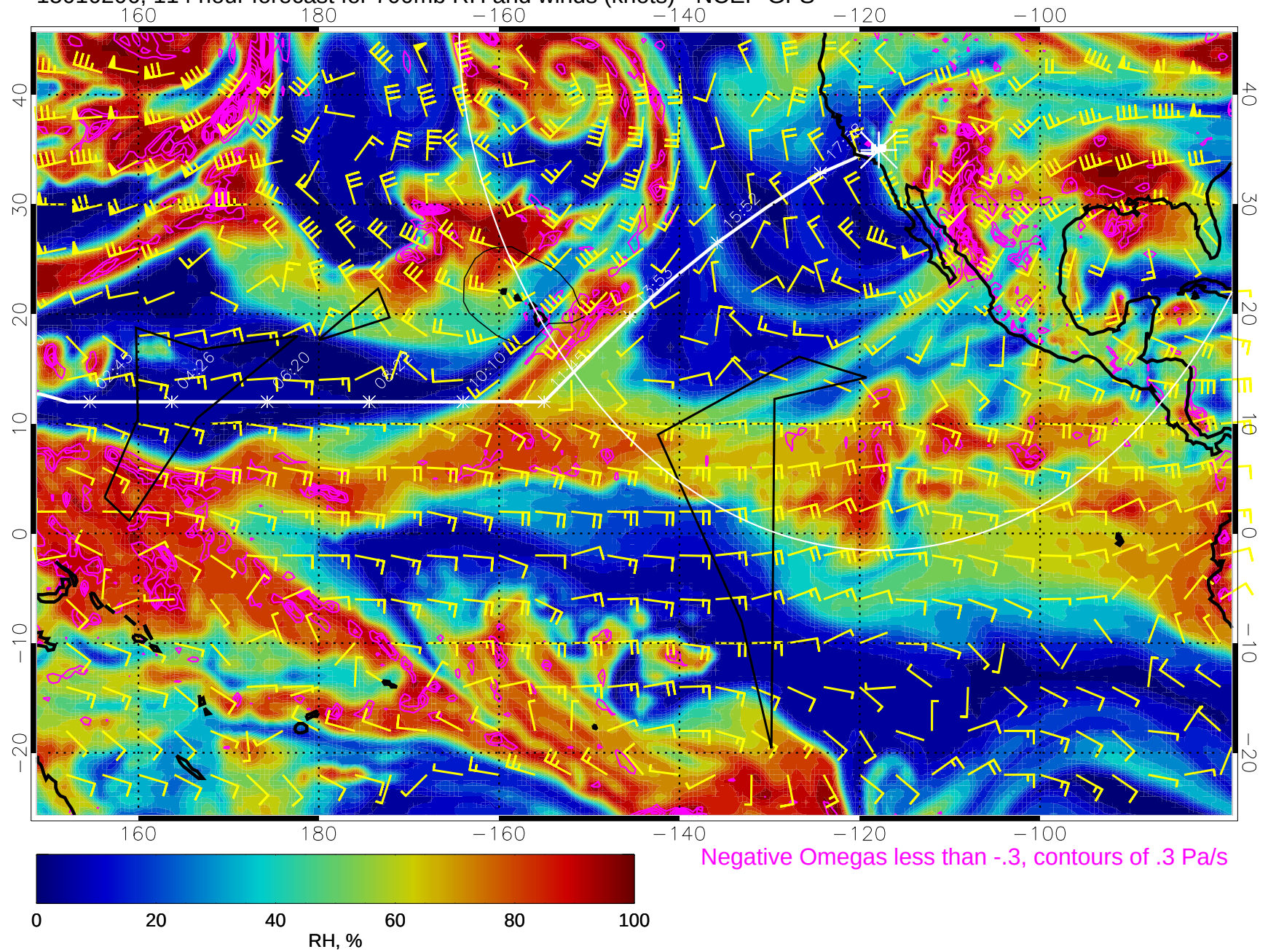
15010206, 114 hour forecast for 700mb RH and winds (knots) - NCEP GFS
