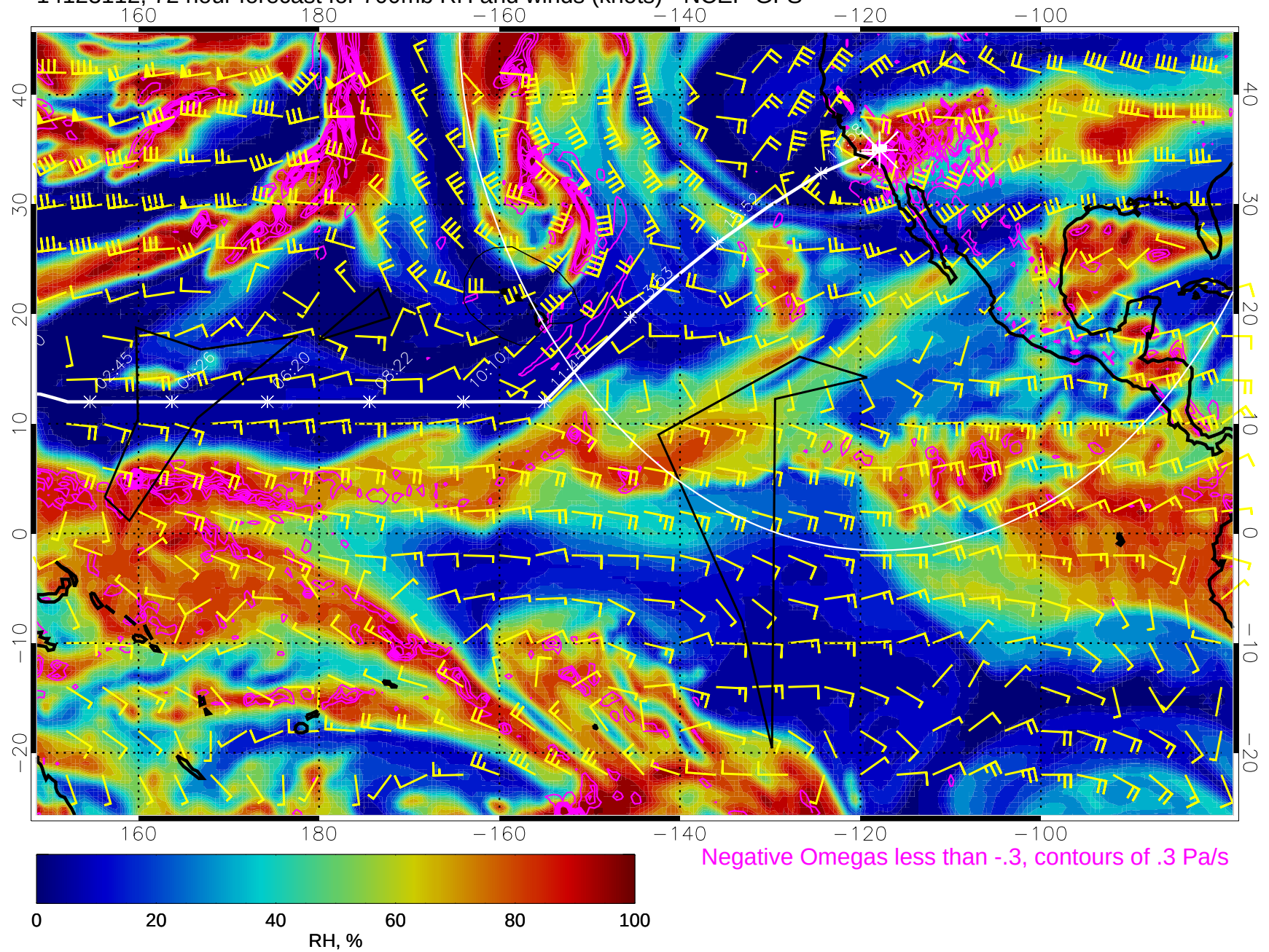
14123112, 72 hour forecast for 700mb RH and winds (knots) - NCEP GFS
