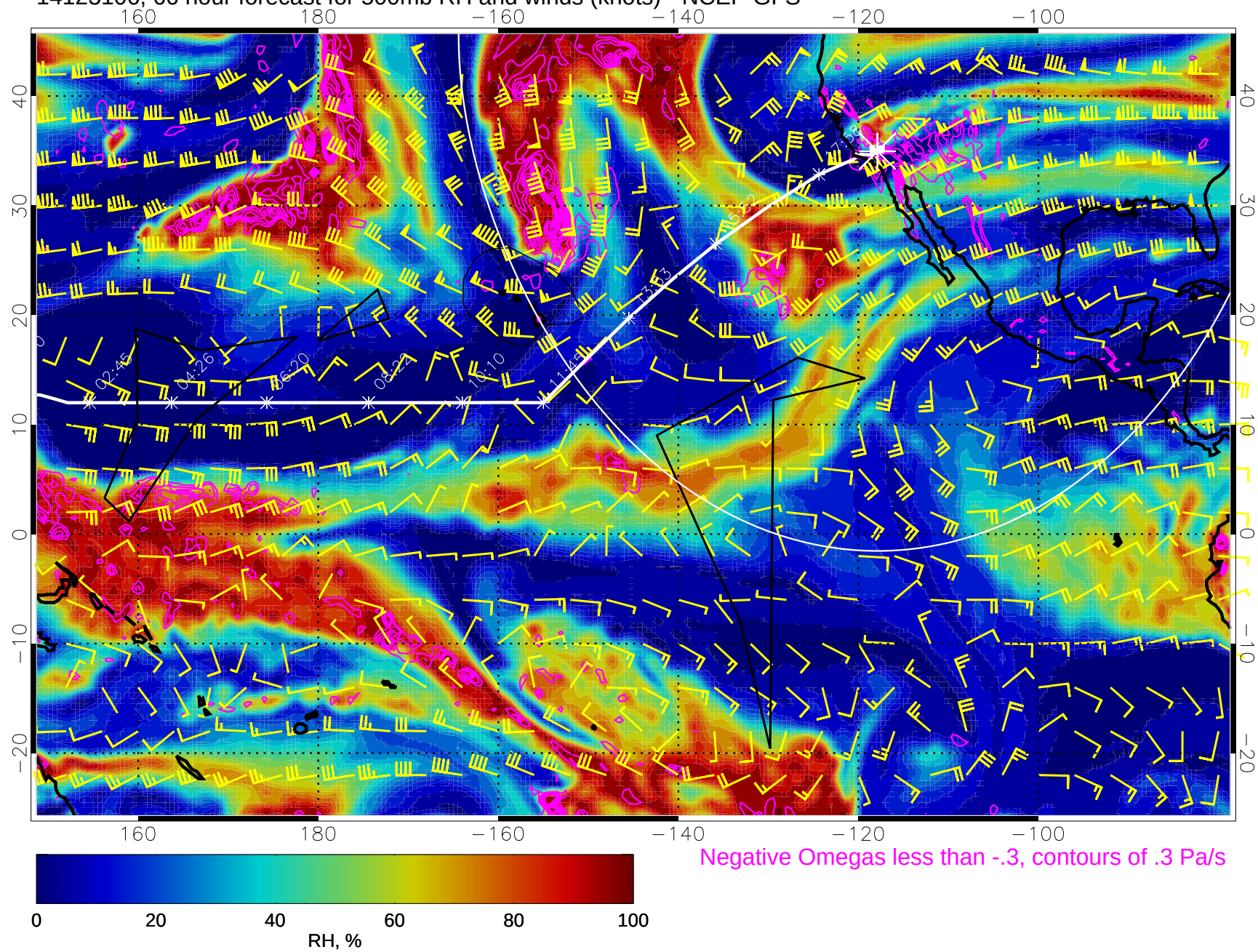
14123106, 66 hour forecast for 500mb RH and winds (knots) - NCEP GFS
