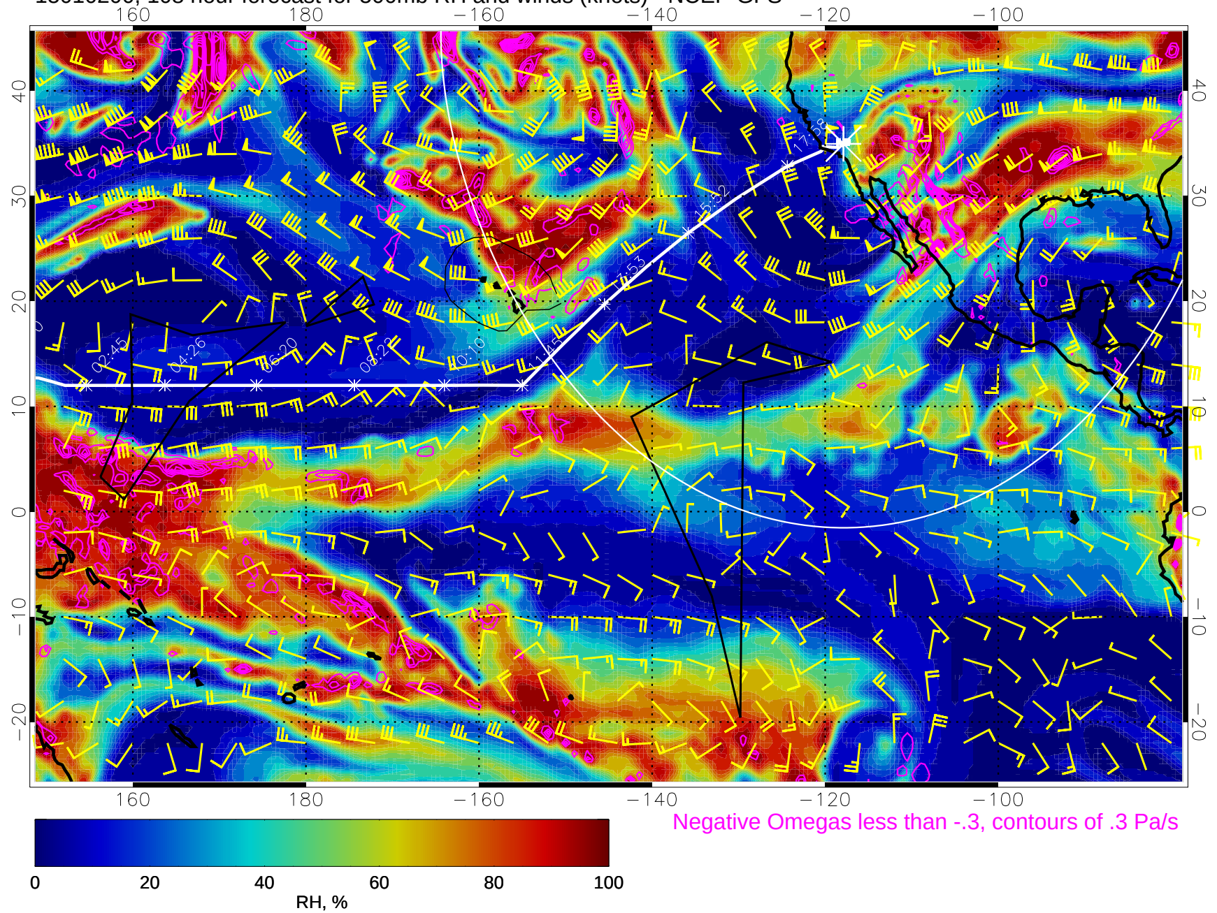
15010200, 108 hour forecast for 500mb RH and winds (knots) - NCEP GFS
