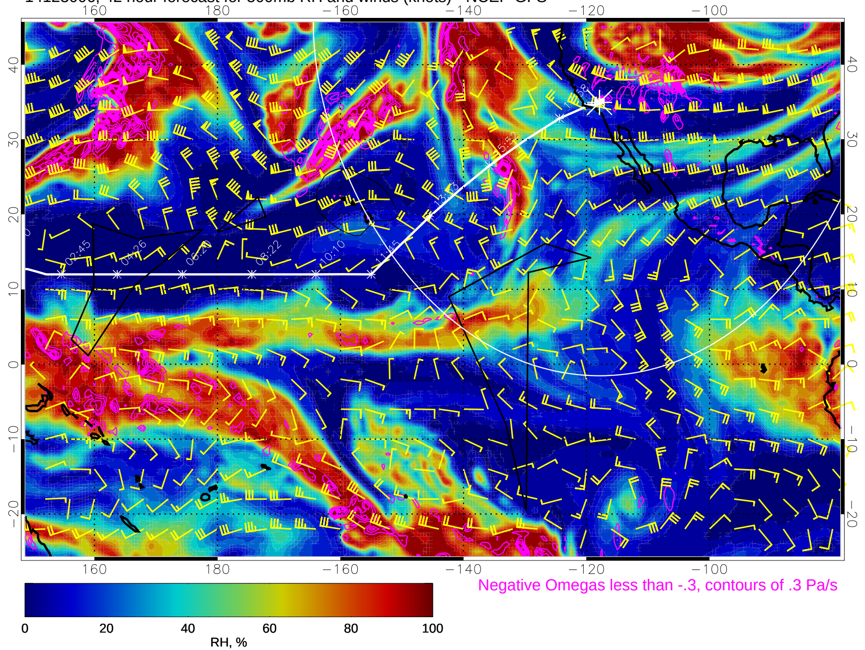
14123006, 42 hour forecast for 500mb RH and winds (knots) - NCEP GFS
