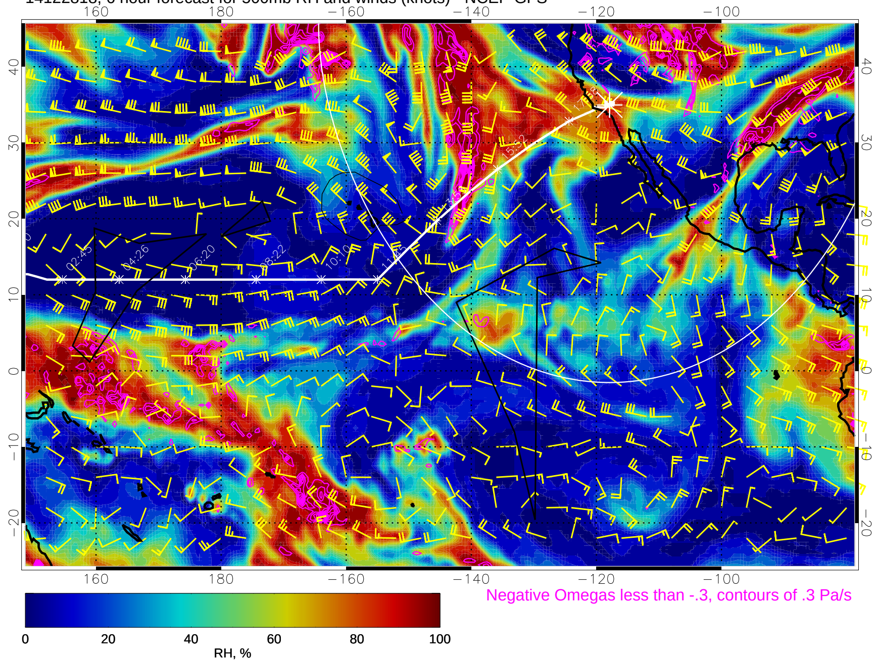
14122818, 6 hour forecast for 500mb RH and winds (knots) - NCEP GFS
