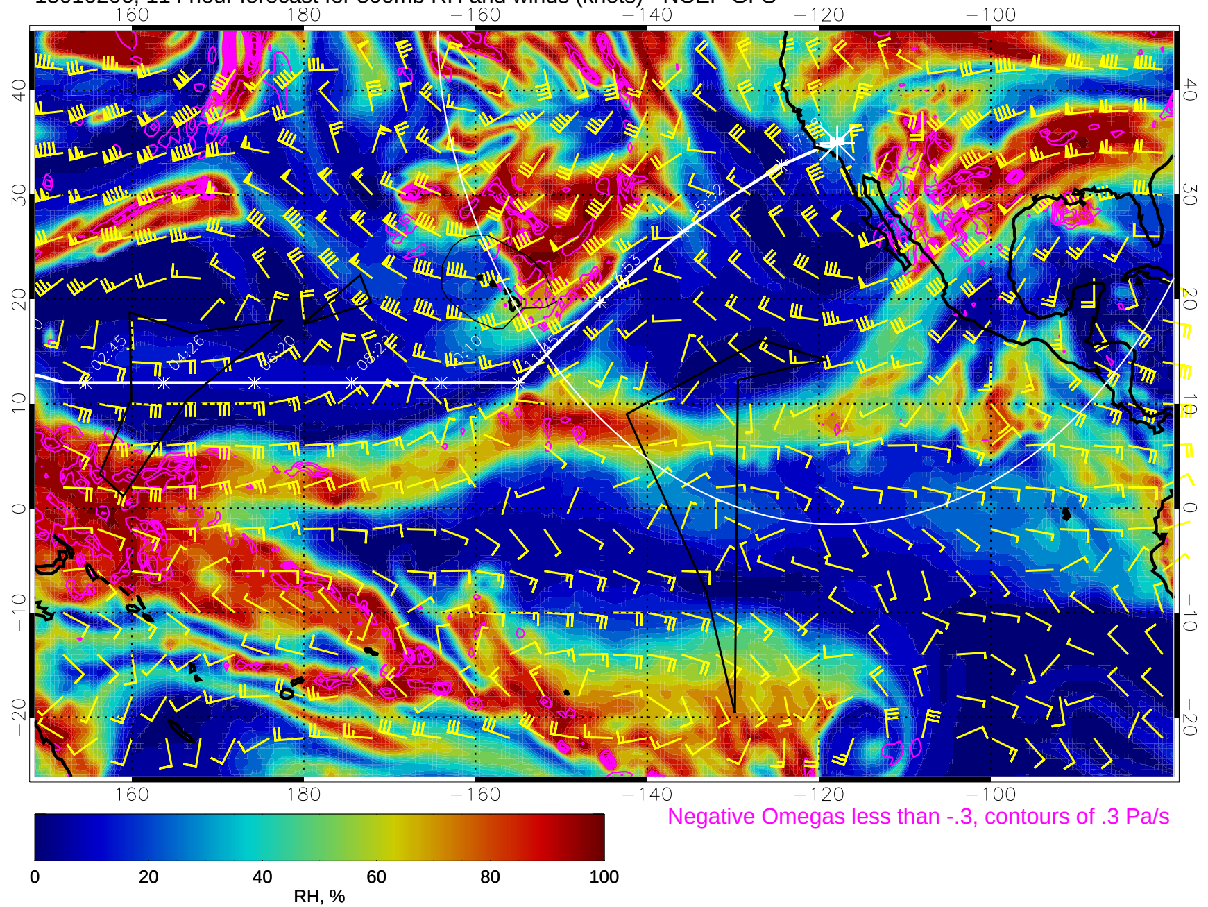
15010206, 114 hour forecast for 500mb RH and winds (knots) - NCEP GFS
