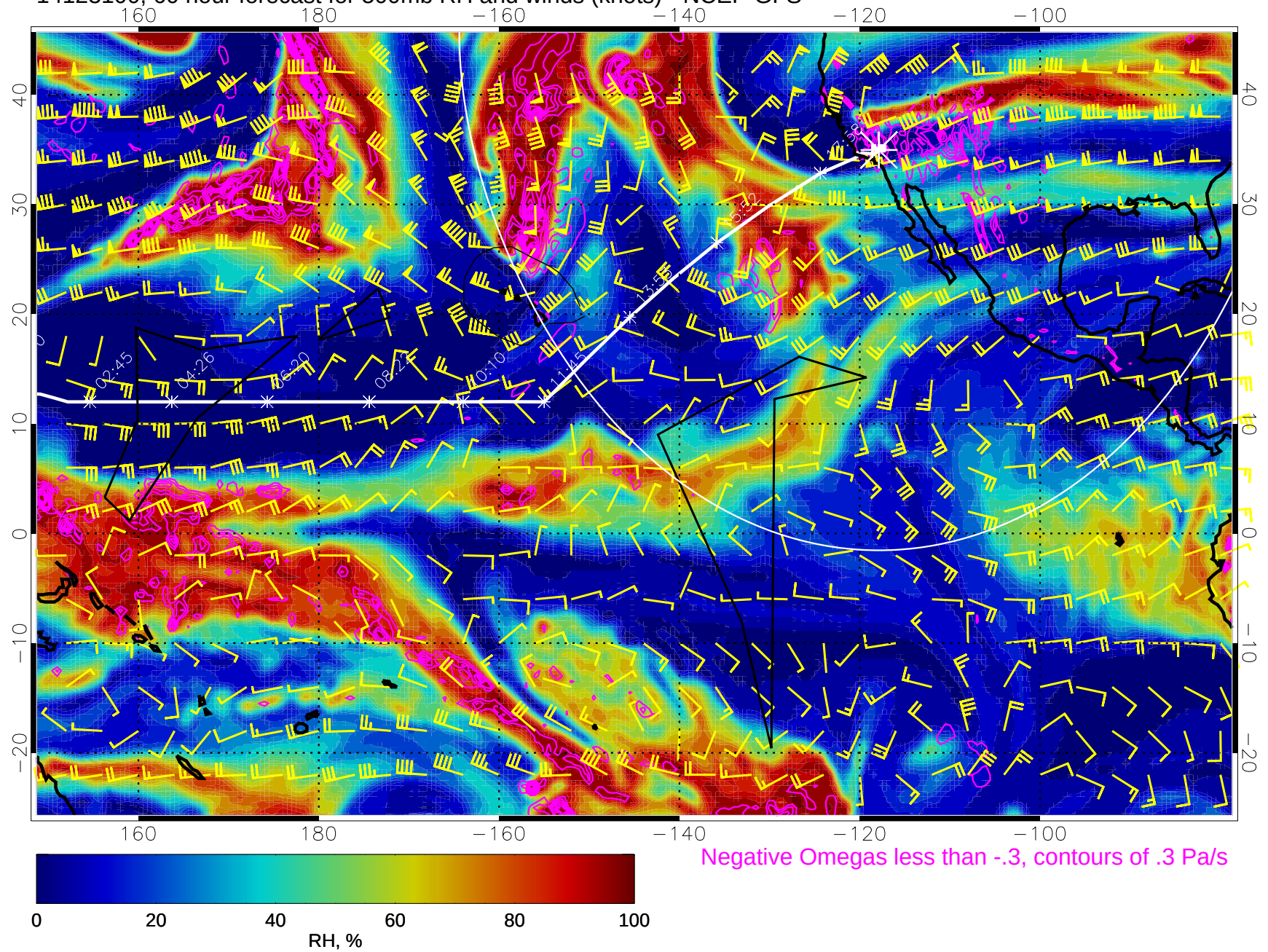
14123100, 60 hour forecast for 500mb RH and winds (knots) - NCEP GFS
