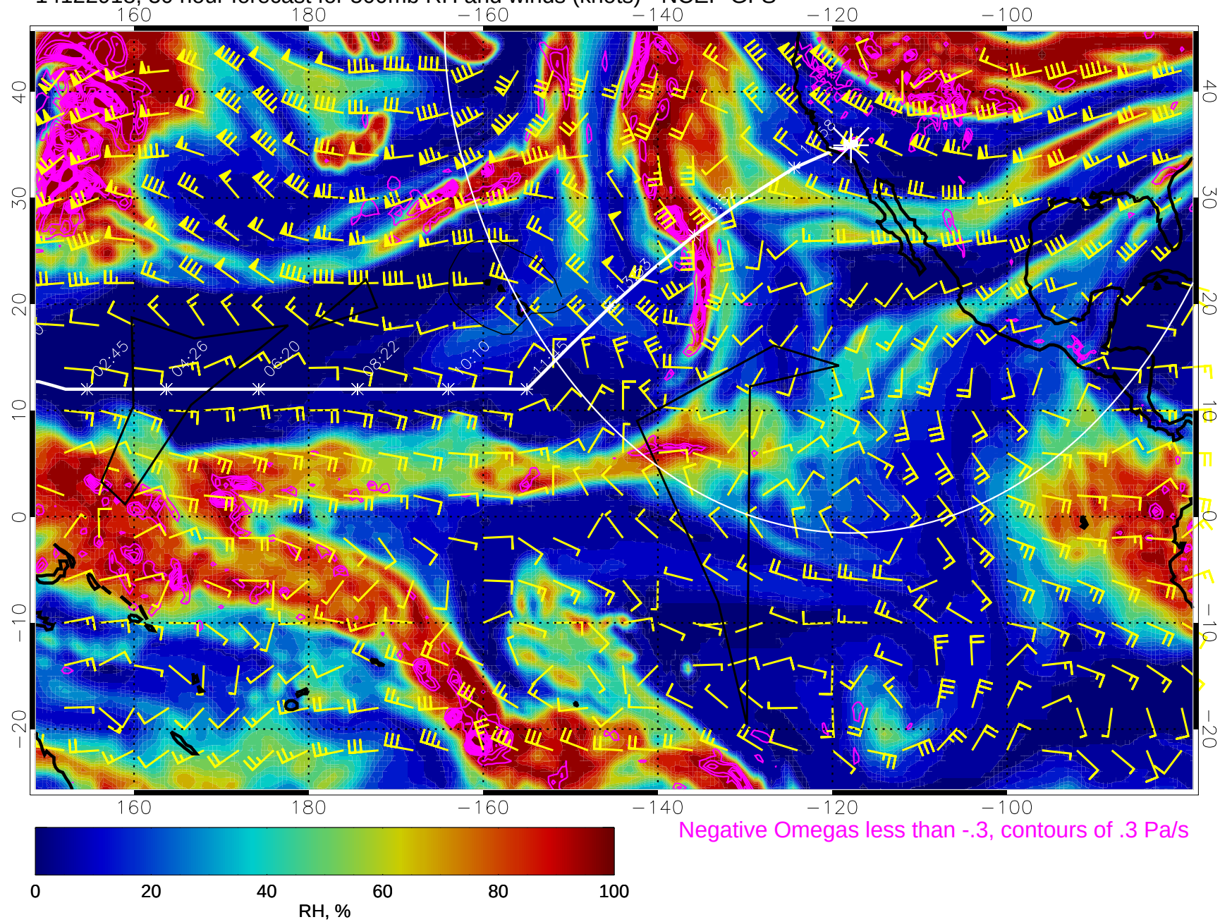
14122918, 30 hour forecast for 500mb RH and winds (knots) - NCEP GFS
