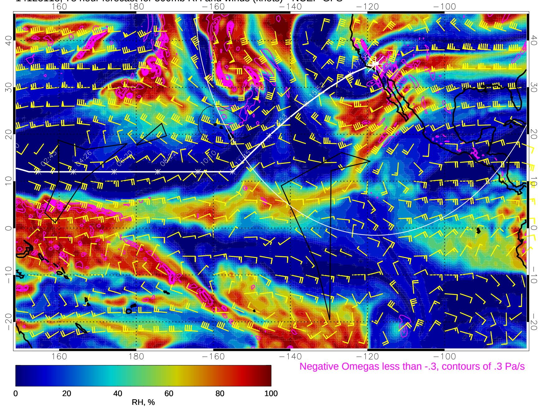
14123118, 78 hour forecast for 500mb RH and winds (knots) - NCEP GFS
