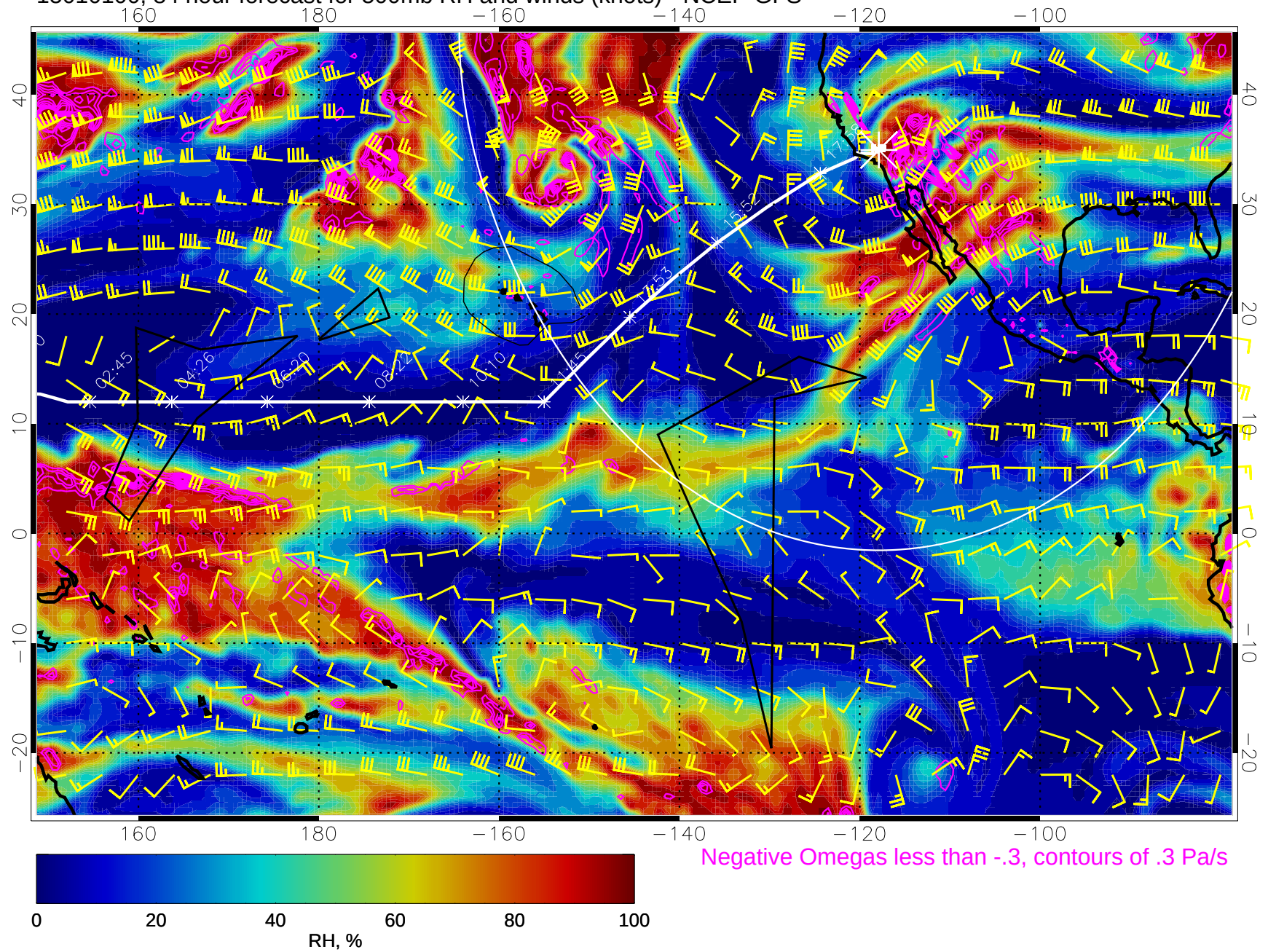
15010100, 84 hour forecast for 500mb RH and winds (knots) - NCEP GFS
