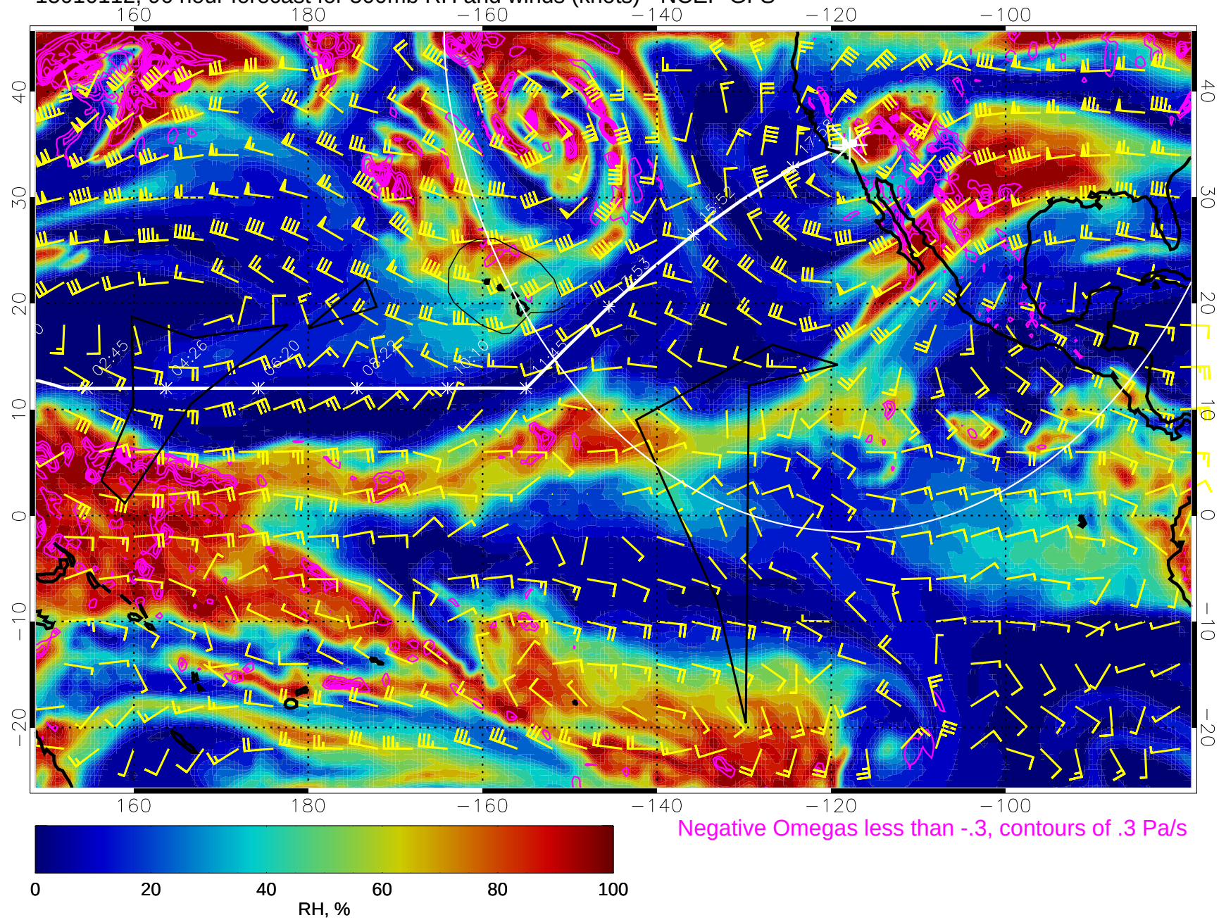
15010112, 96 hour forecast for 500mb RH and winds (knots) - NCEP GFS
