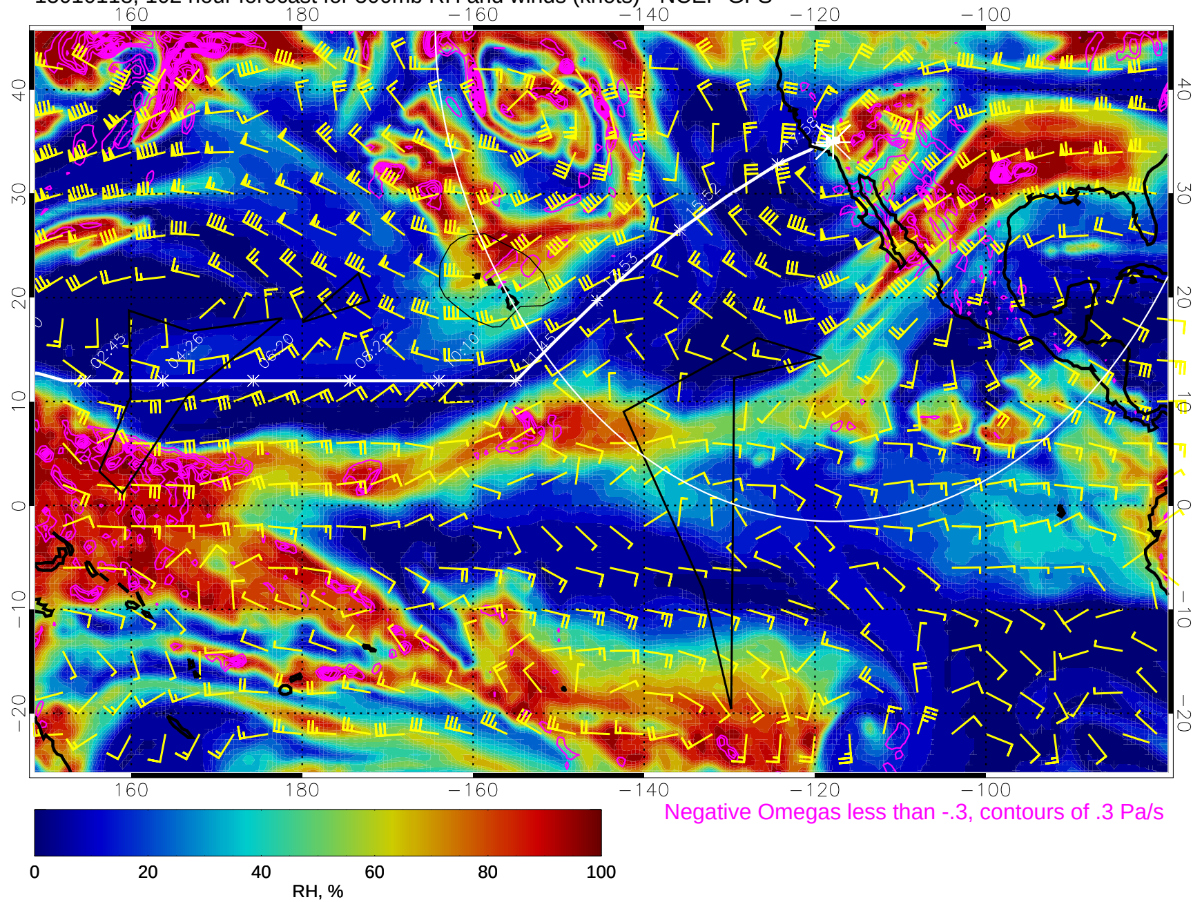
15010118, 102 hour forecast for 500mb RH and winds (knots) - NCEP GFS
