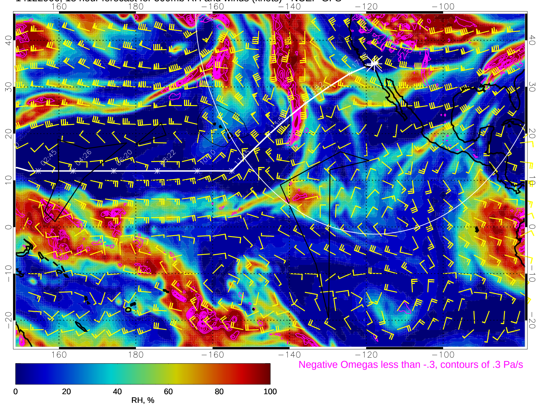
14122906, 18 hour forecast for 500mb RH and winds (knots) - NCEP GFS
