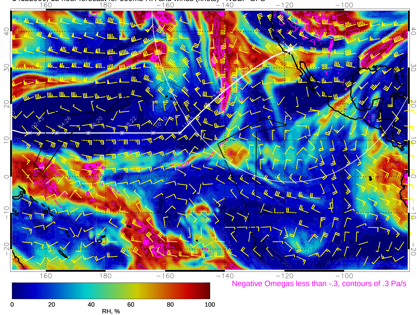
14122900, 12 hour forecast for 500mb RH and winds (knots) - NCEP GFS
