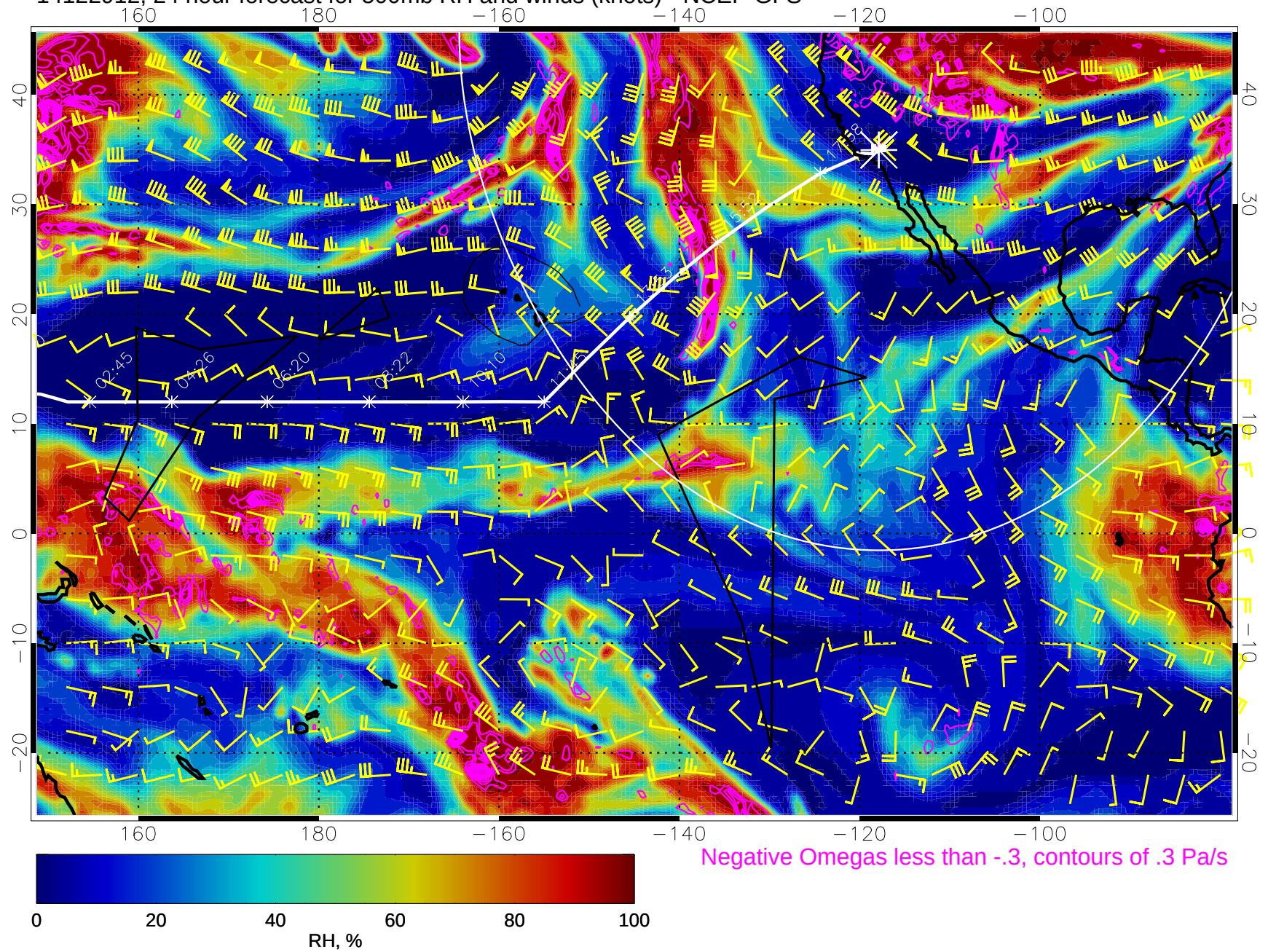
14122912, 24 hour forecast for 500mb RH and winds (knots) - NCEP GFS
