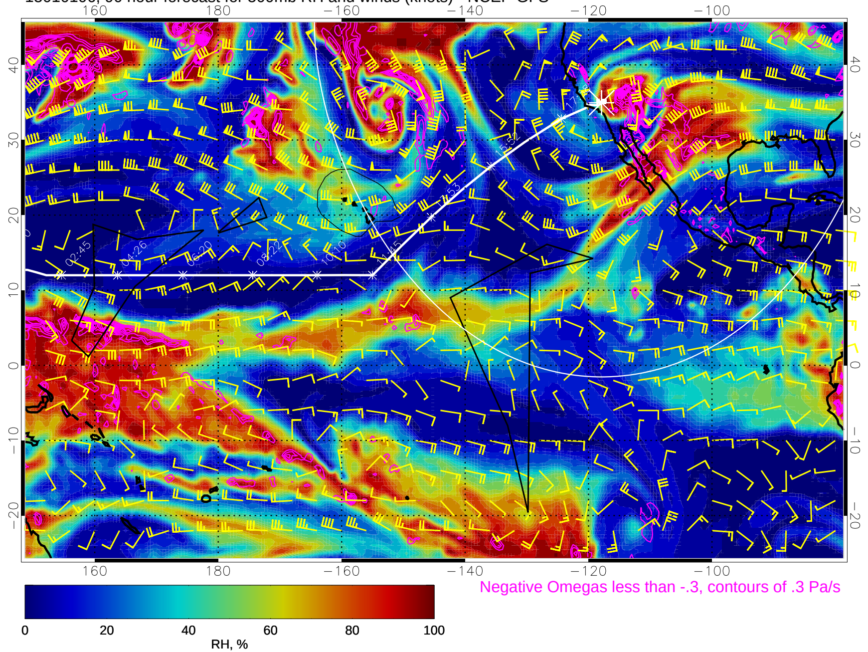
15010106, 90 hour forecast for 500mb RH and winds (knots) - NCEP GFS
