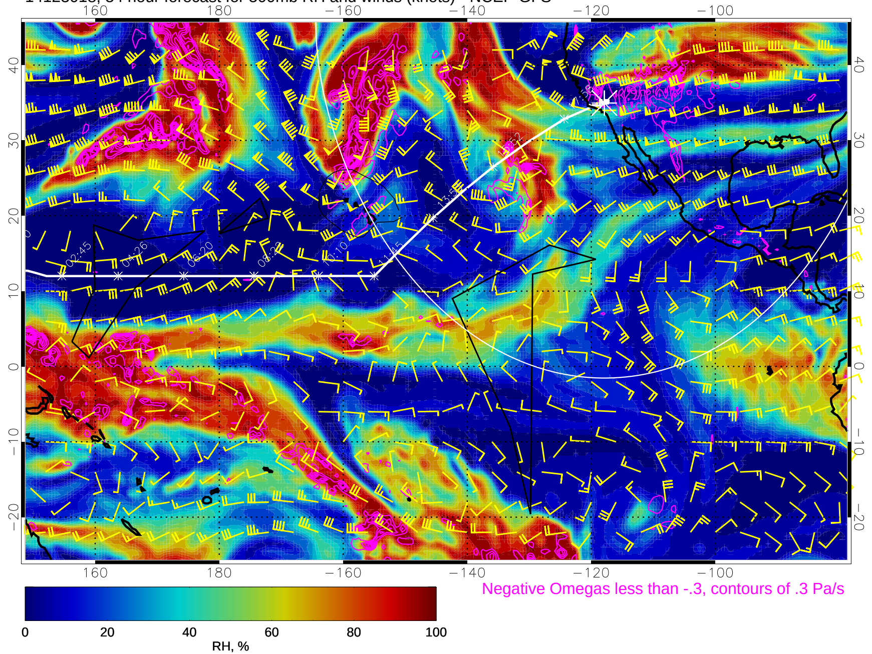
14123018, 54 hour forecast for 500mb RH and winds (knots) - NCEP GFS
