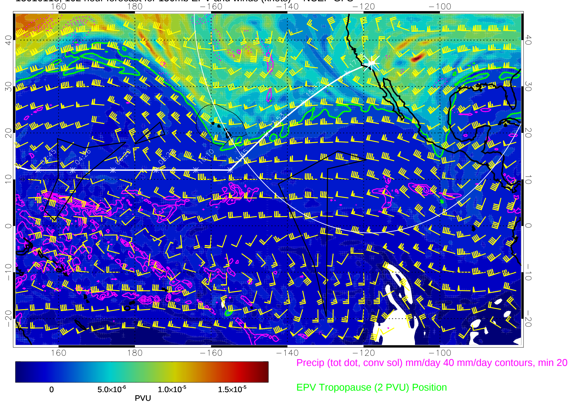
15010118, 102 hour forecast for 150mb EPV and winds (knots) -- NCEP GFS
