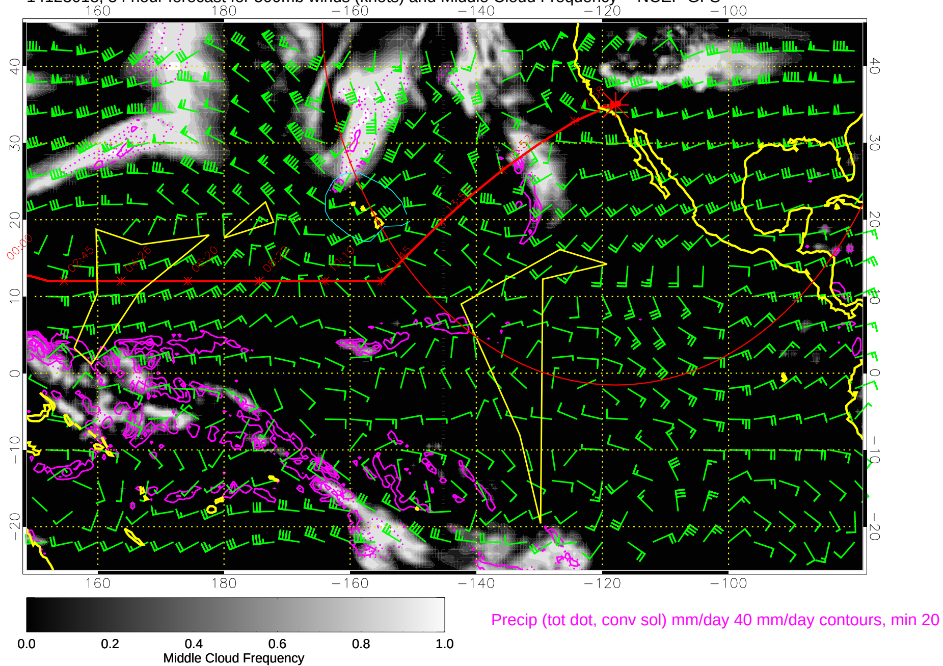
14123018, 54 hour forecast for 500mb winds (knots) and Middle Cloud Frequency -- NCEP GFS
