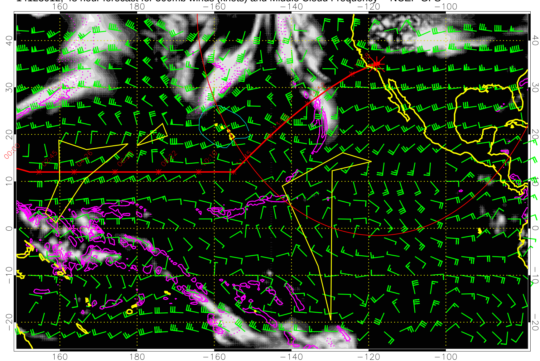
14123012, 48 hour forecast for 500mb winds (knots) and Middle Cloud Frequency -- NCEP GFS
