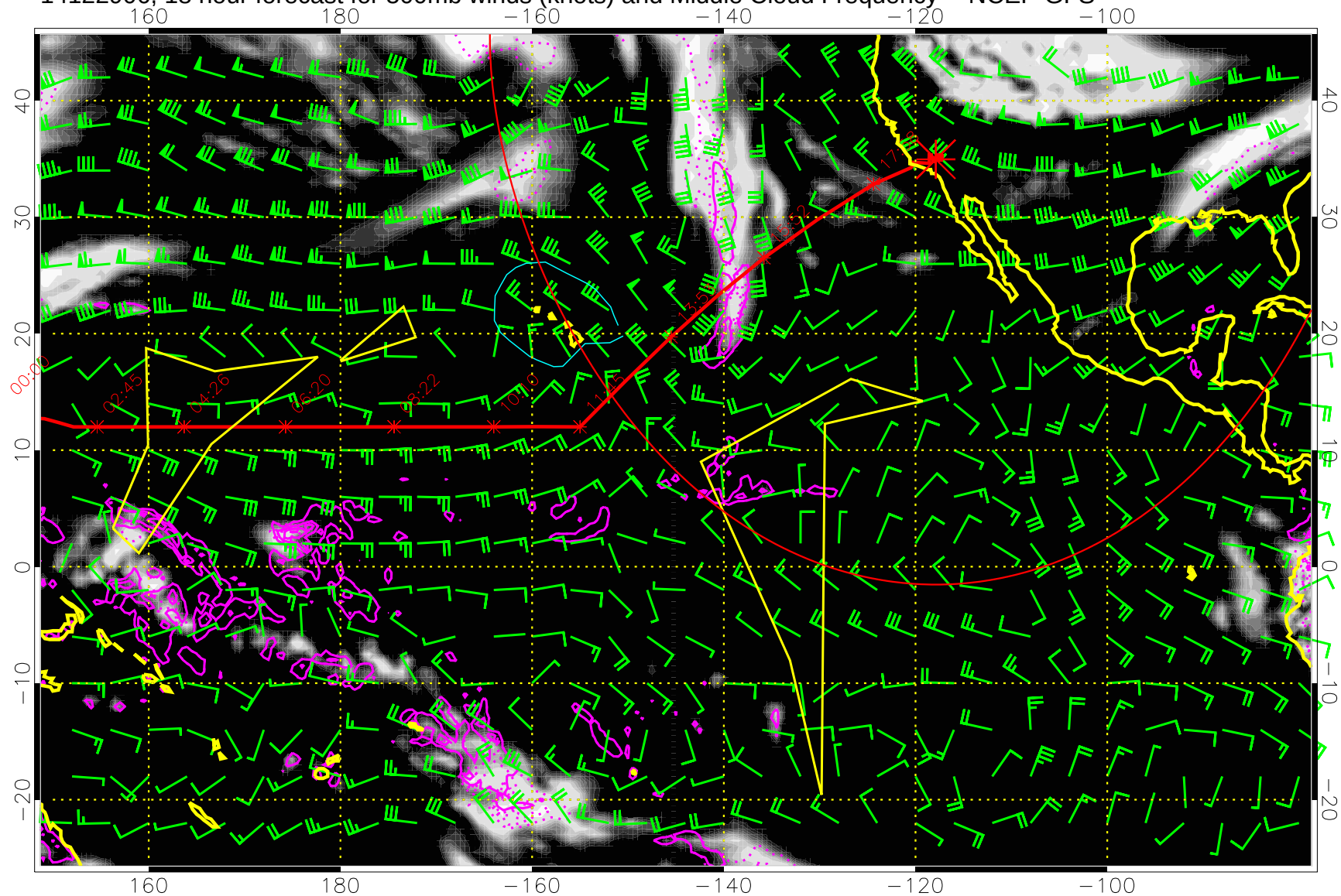
14122906, 18 hour forecast for 500mb winds (knots) and Middle Cloud Frequency -- NCEP GFS
