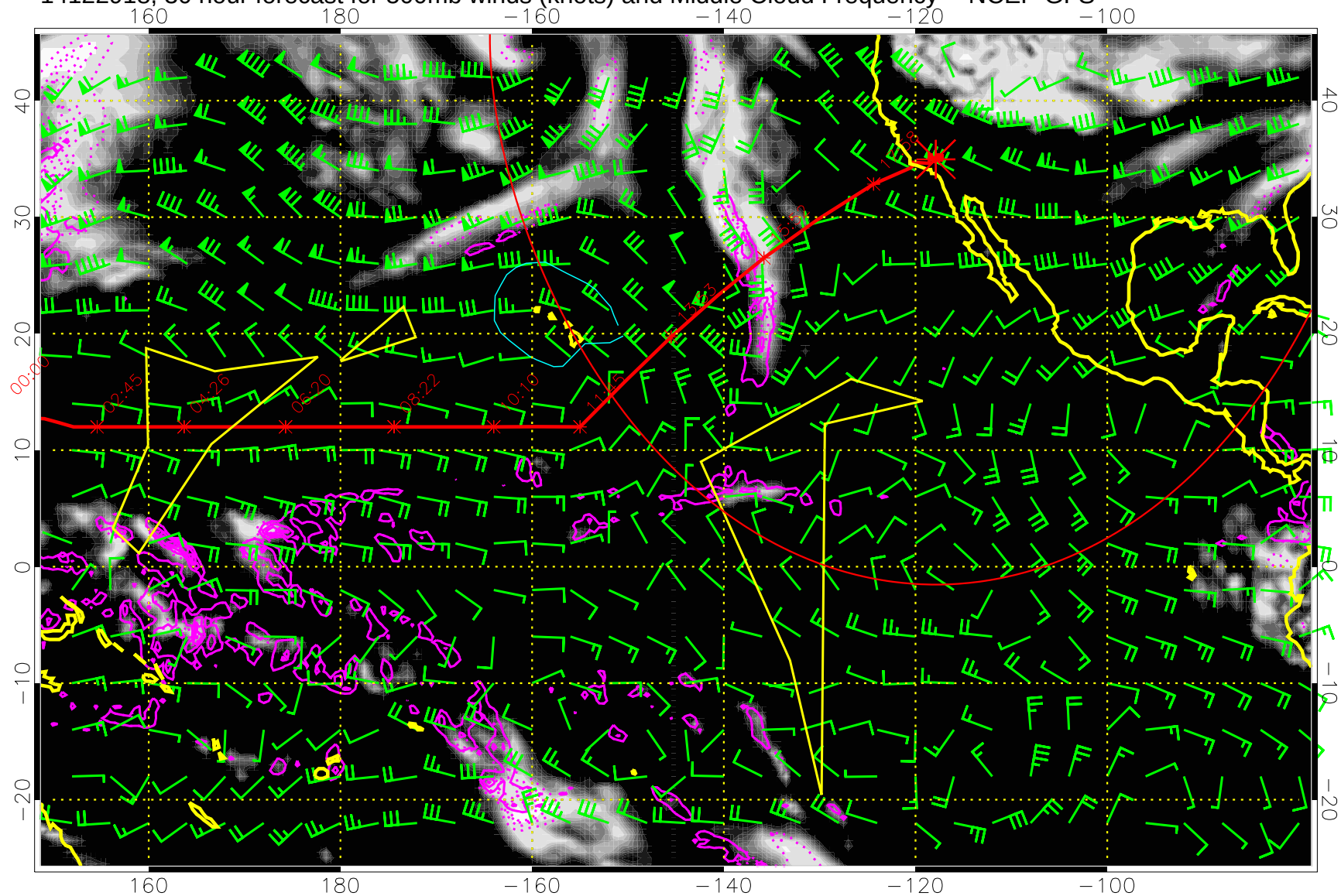
14122918, 30 hour forecast for 500mb winds (knots) and Middle Cloud Frequency -- NCEP GFS
