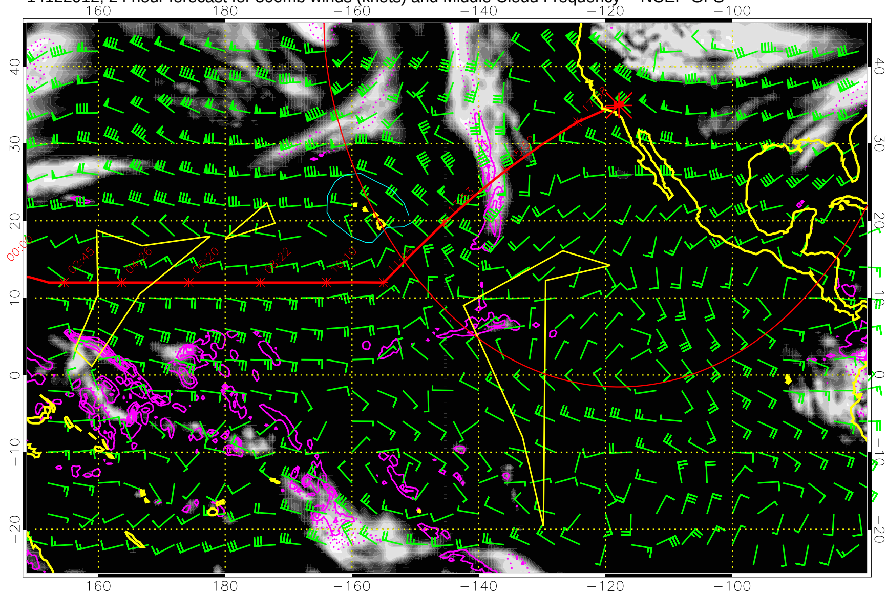
14122912, 24 hour forecast for 500mb winds (knots) and Middle Cloud Frequency -- NCEP GFS
