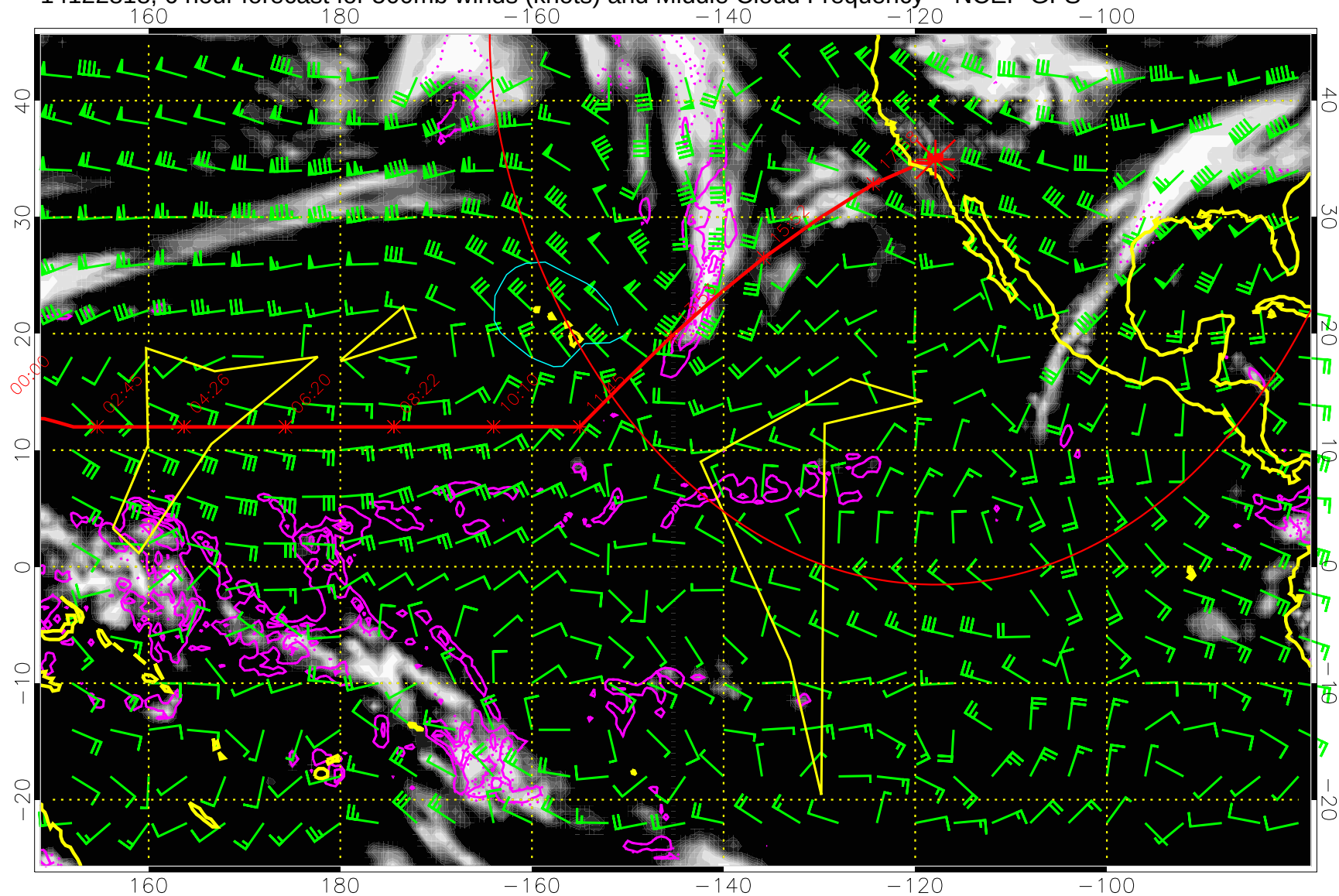
14122818, 6 hour forecast for 500mb winds (knots) and Middle Cloud Frequency -- NCEP GFS
