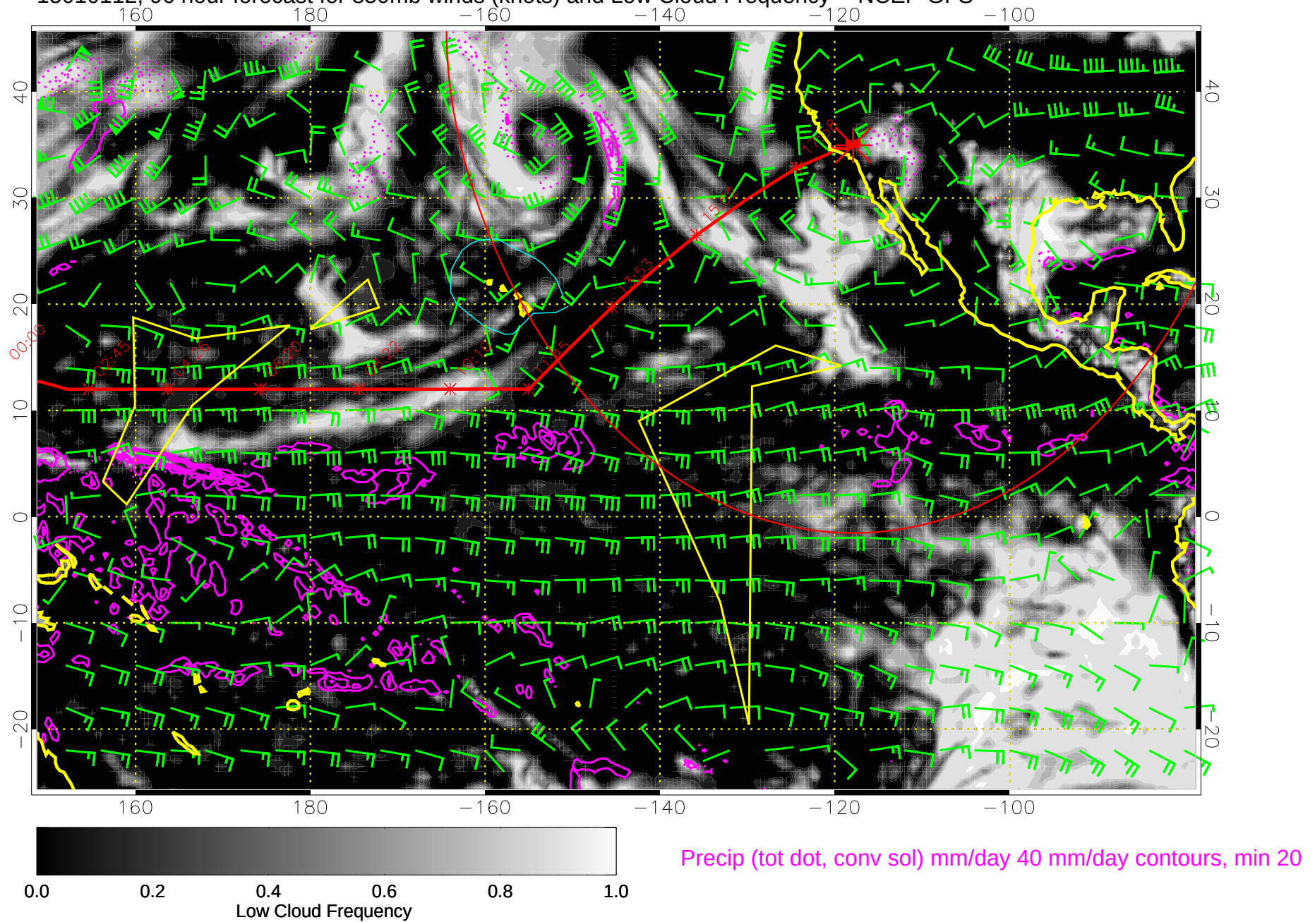
15010112, 96 hour forecast for 850mb winds (knots) and Low Cloud Frequency -- NCEP GFS
