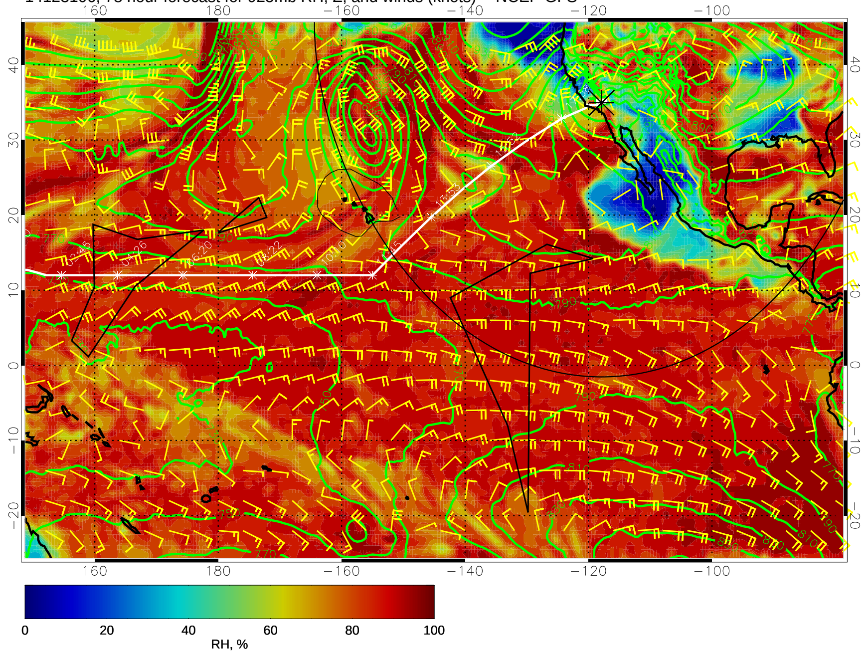
14123106, 78 hour forecast for 925mb RH, Z, and winds (knots) -- NCEP GFS
