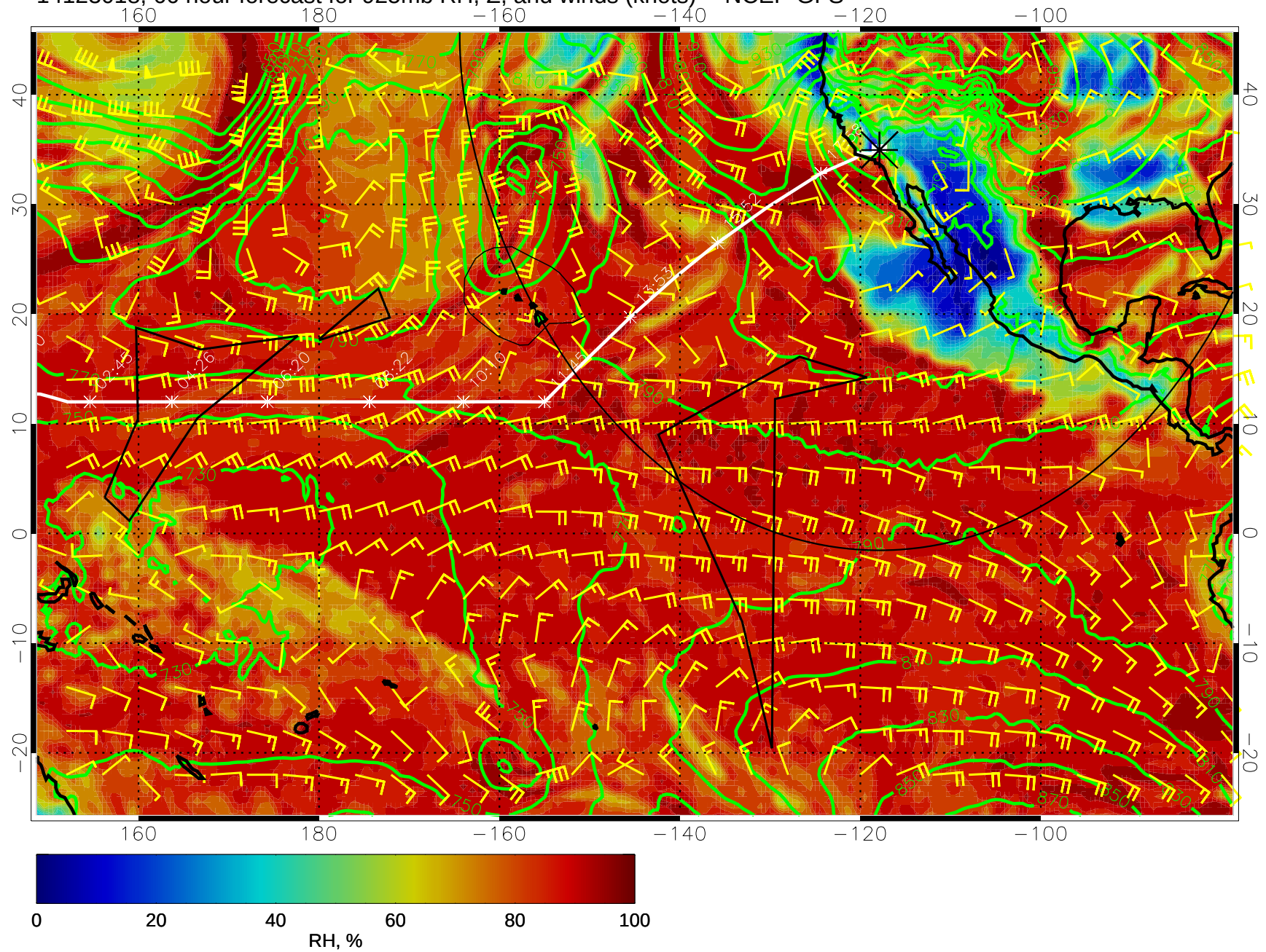
14123018, 66 hour forecast for 925mb RH, Z, and winds (knots) -- NCEP GFS
