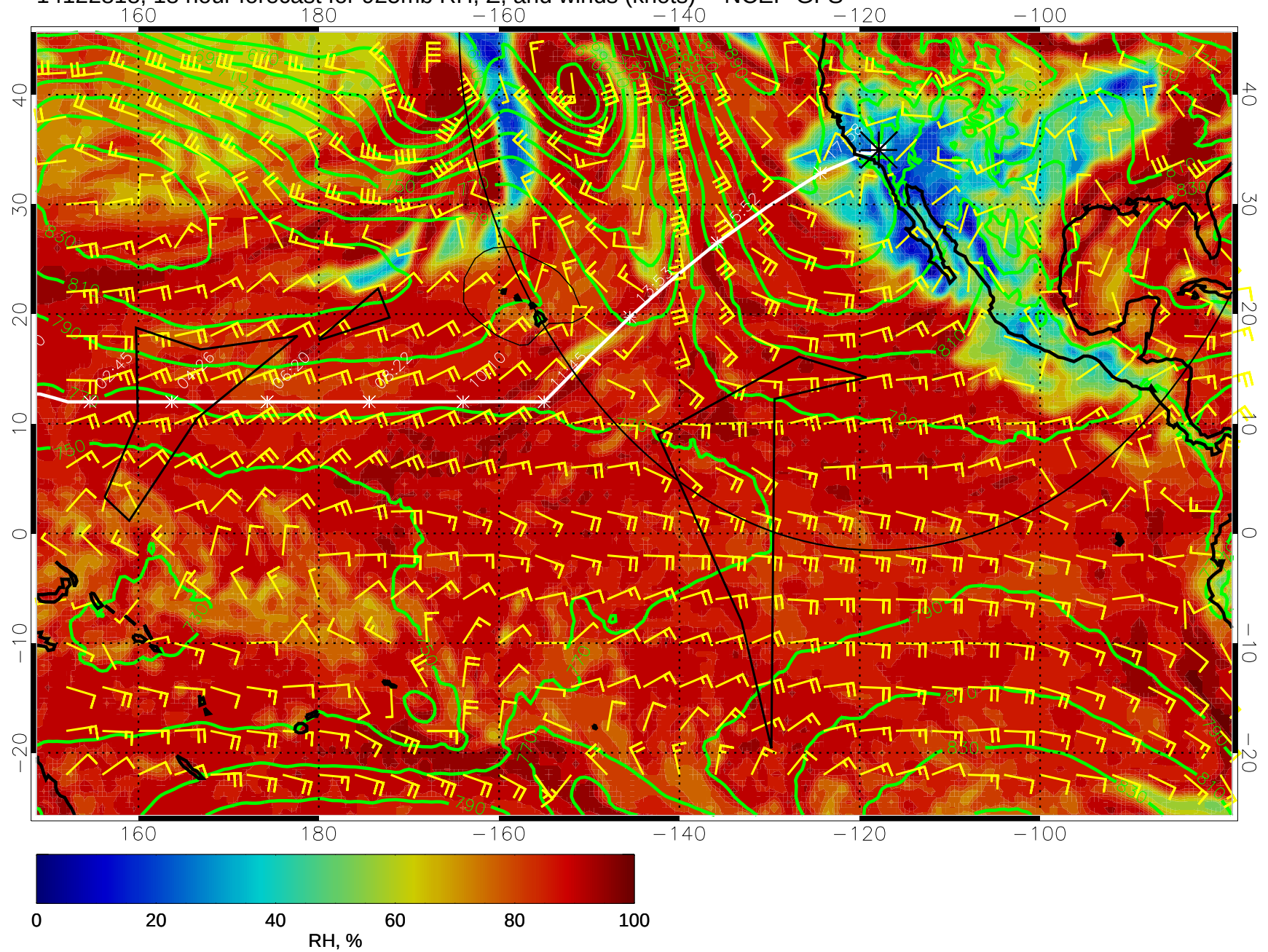
14122818, 18 hour forecast for 925mb RH, Z, and winds (knots) -- NCEP GFS
