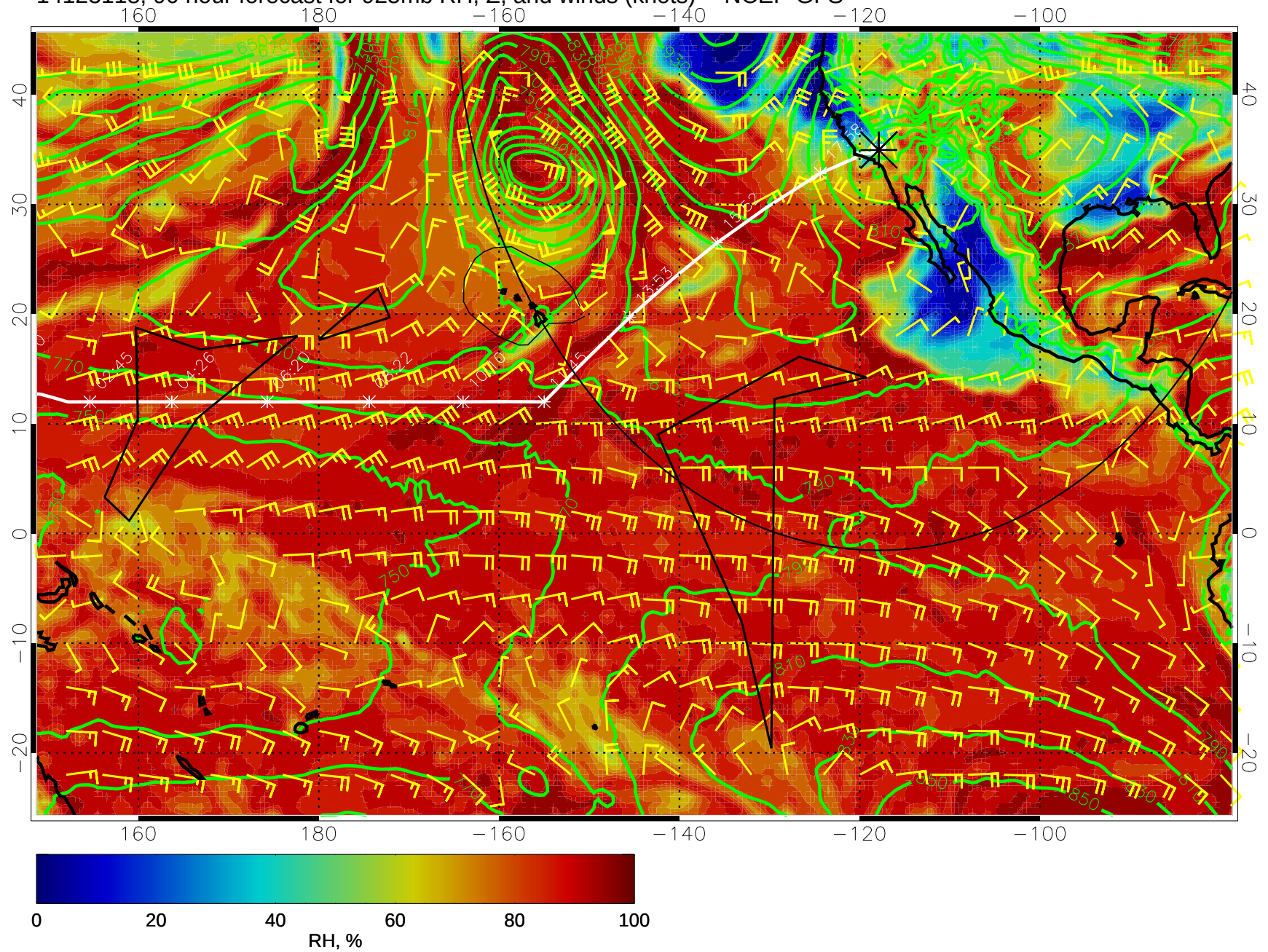
14123118, 90 hour forecast for 925mb RH, Z, and winds (knots) -- NCEP GFS
