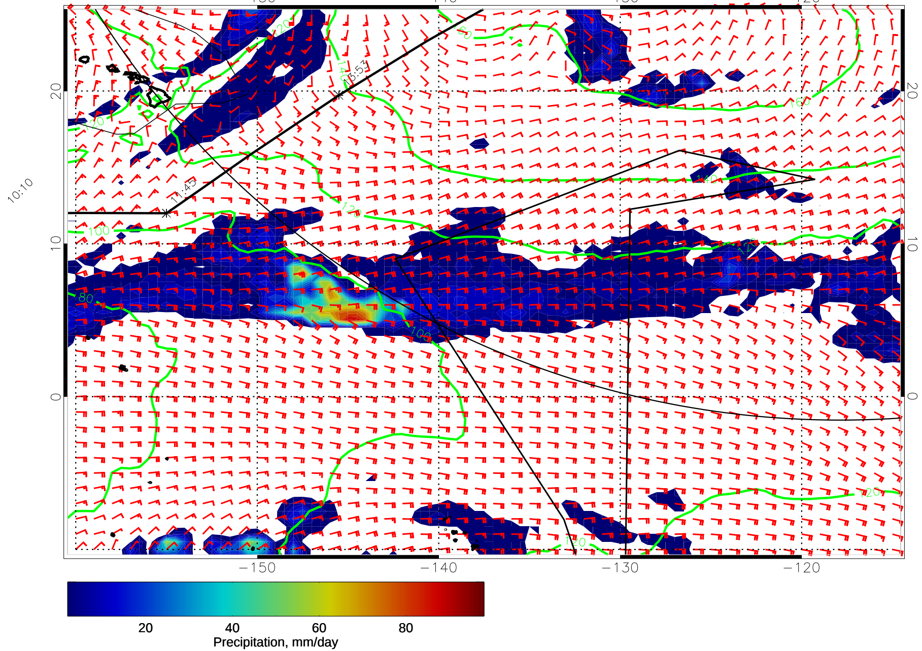
14123118, 90 hour forecast for precip, 1000mb Z, and winds (knots) -- NCEP GFS
