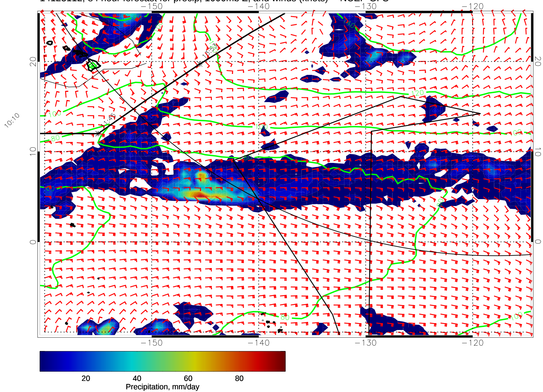
14123112, 84 hour forecast for precip, 1000mb Z, and winds (knots) -- NCEP GFS
