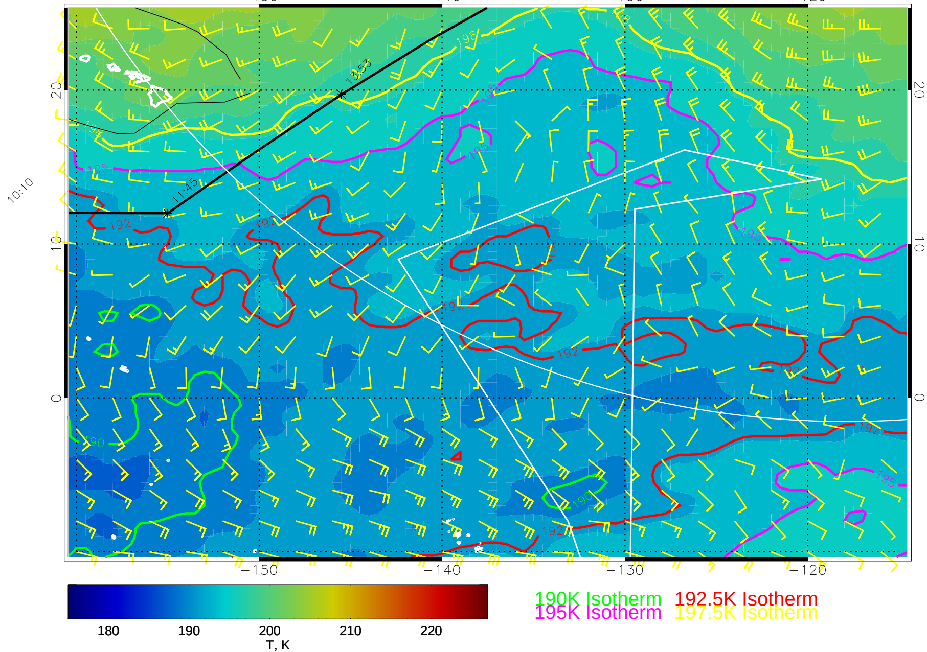
15010106, 102 hour forecast for 70mb T and winds (knots) -- NCEP GFS
