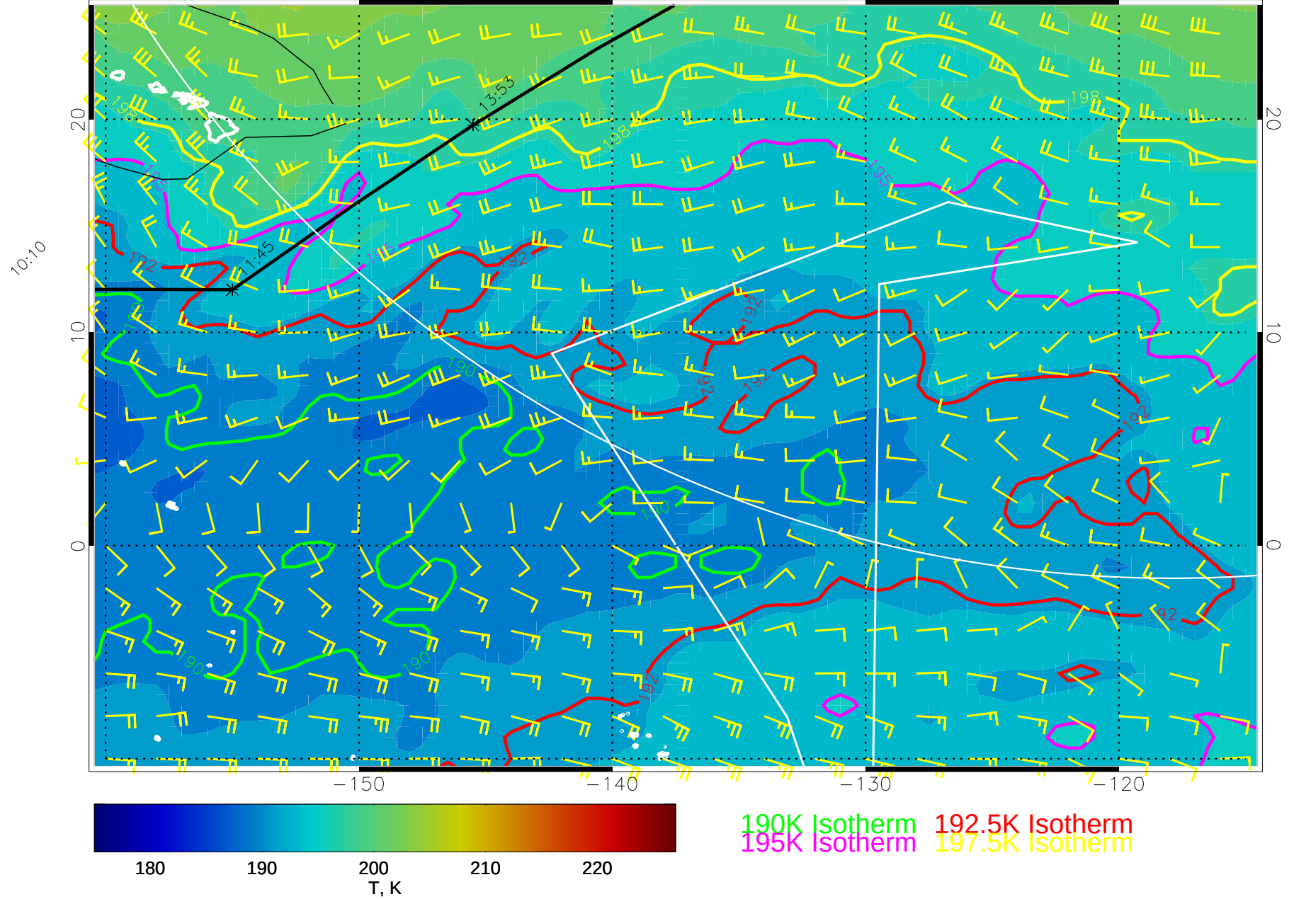
15010200, 120 hour forecast for 70mb T and winds (knots) -- NCEP GFS
