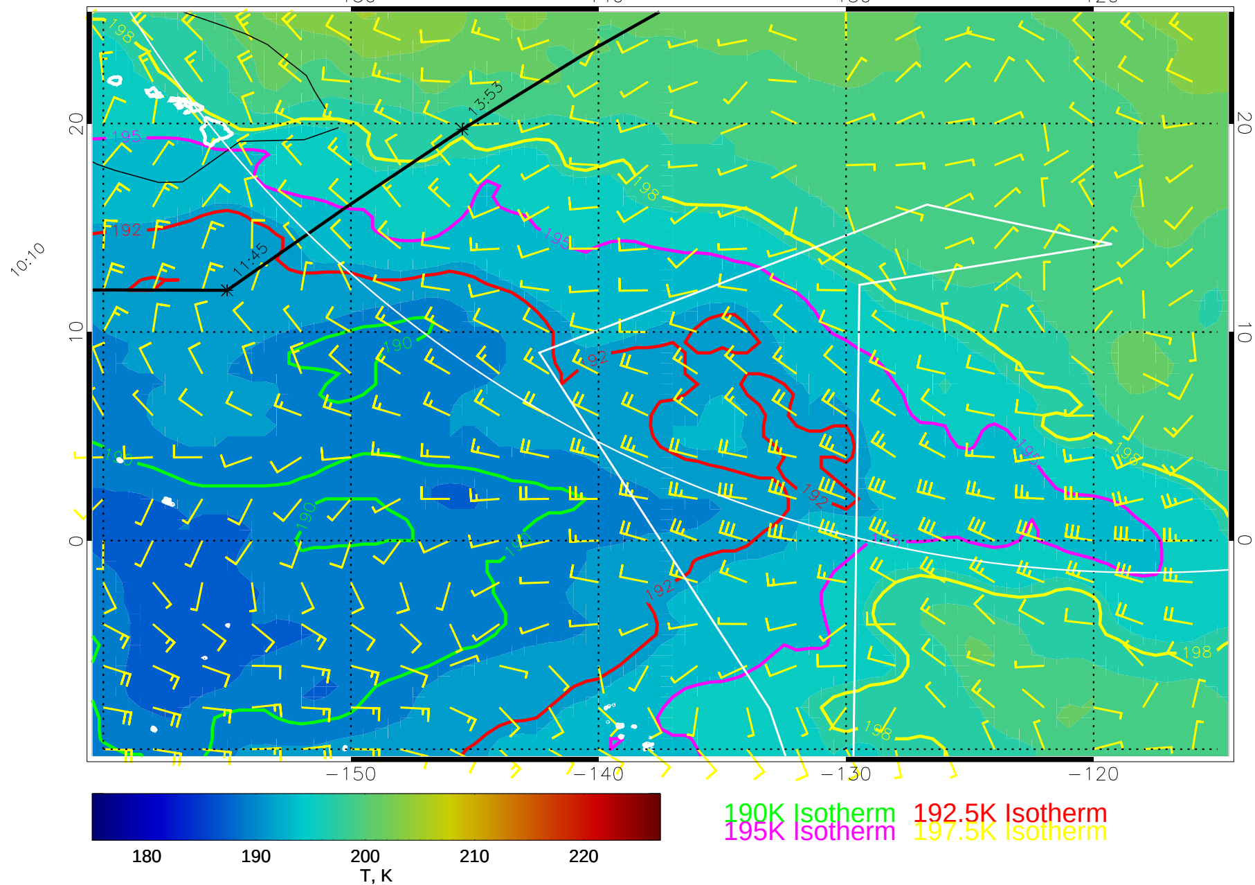
14122806, 6 hour forecast for 70mb T and winds (knots) -- NCEP GFS
