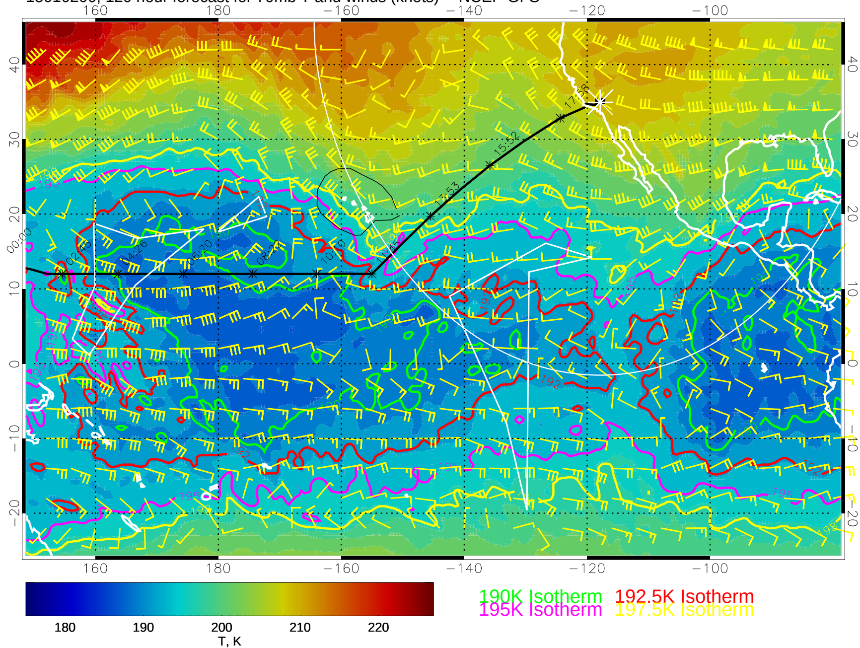
15010200, 120 hour forecast for 70mb T and winds (knots) -- NCEP GFS
