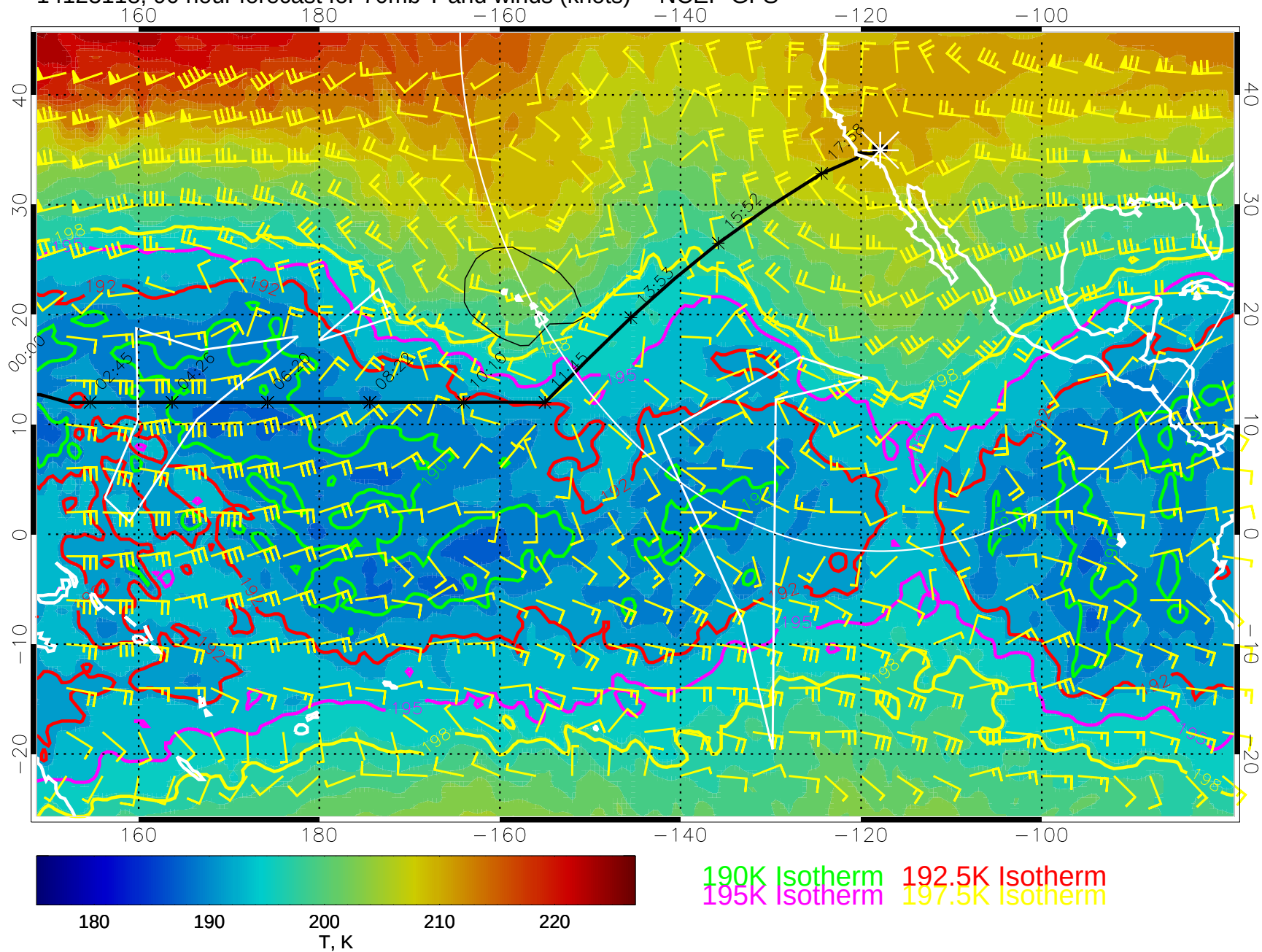
14123118, 90 hour forecast for 70mb T and winds (knots) -- NCEP GFS
