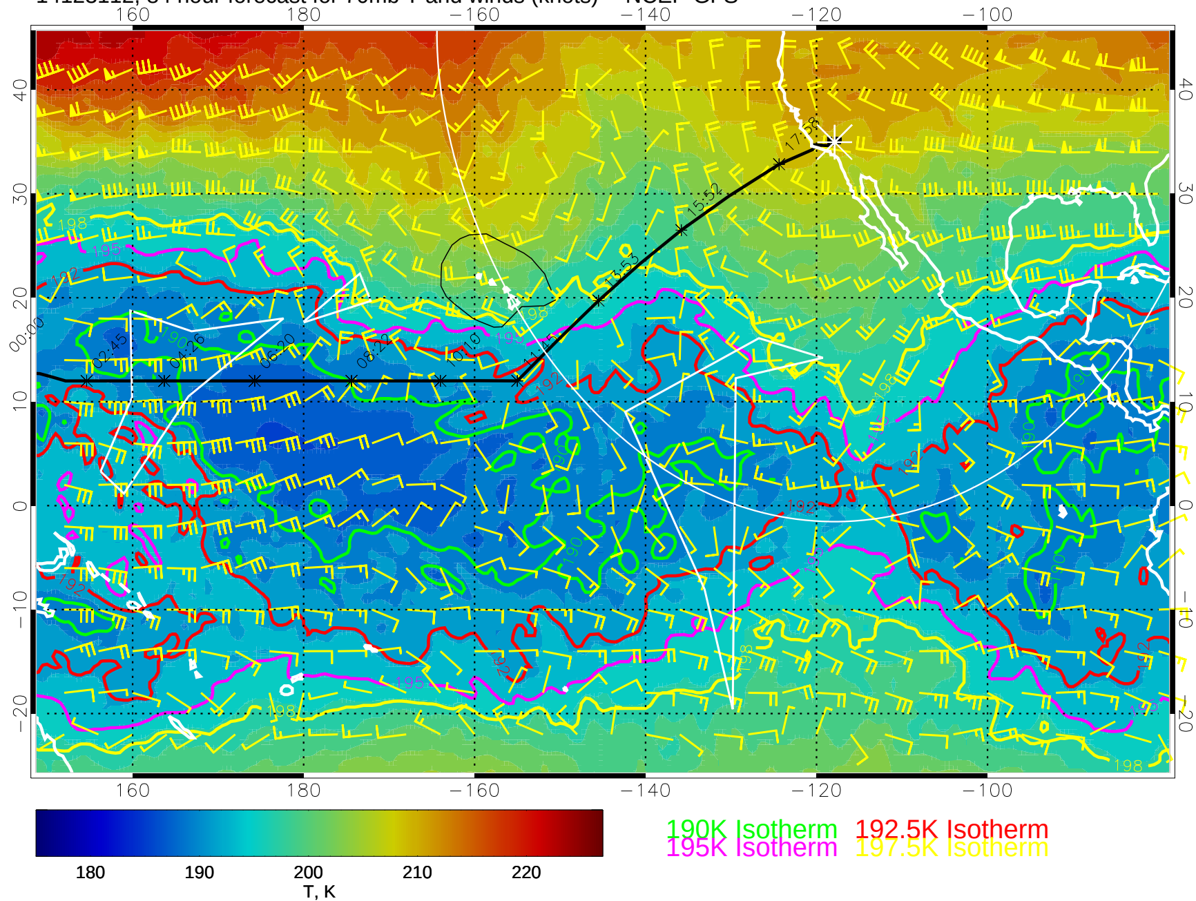
14123112, 84 hour forecast for 70mb T and winds (knots) -- NCEP GFS
