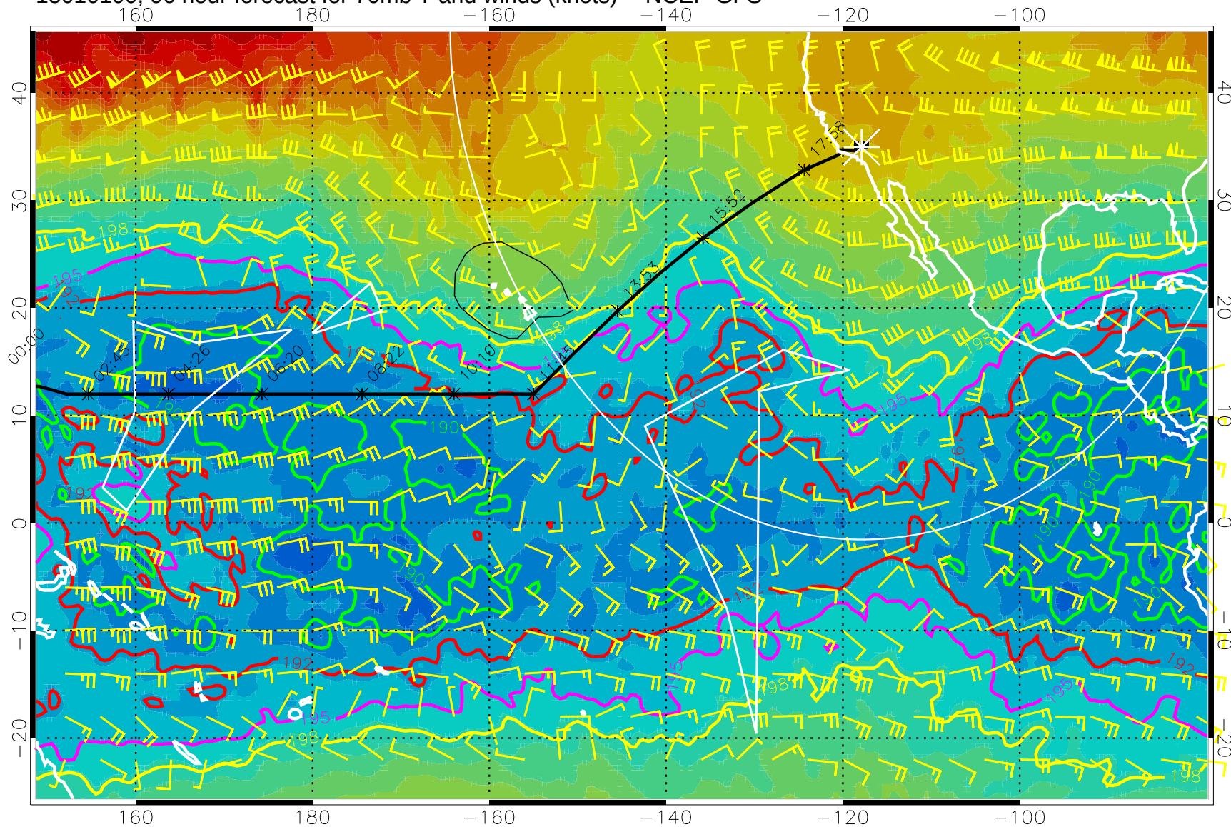
15010100, 96 hour forecast for 70mb T and winds (knots) -- NCEP GFS
