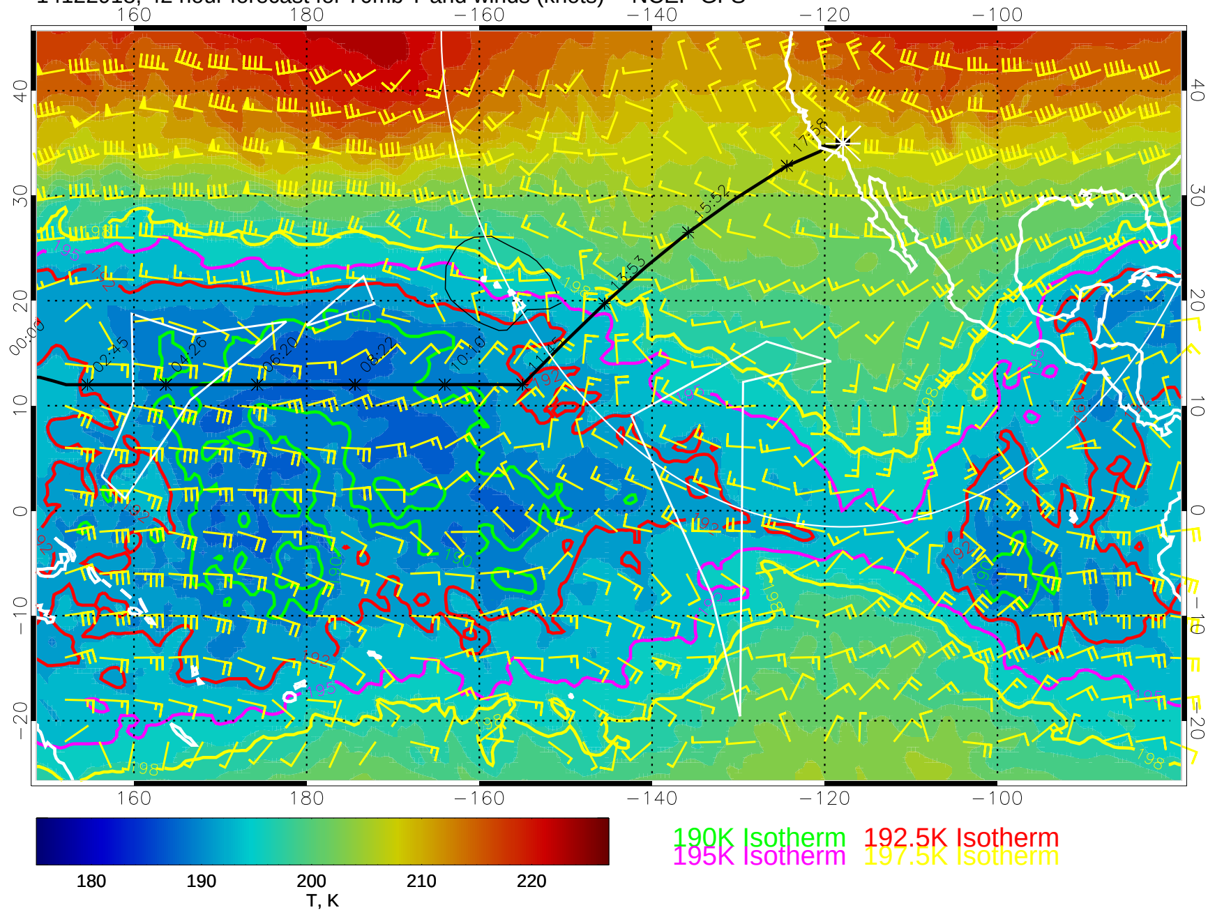
14122918, 42 hour forecast for 70mb T and winds (knots) -- NCEP GFS
