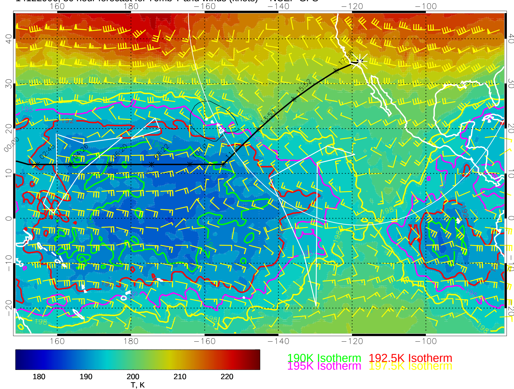
14122906, 30 hour forecast for 70mb T and winds (knots) -- NCEP GFS
