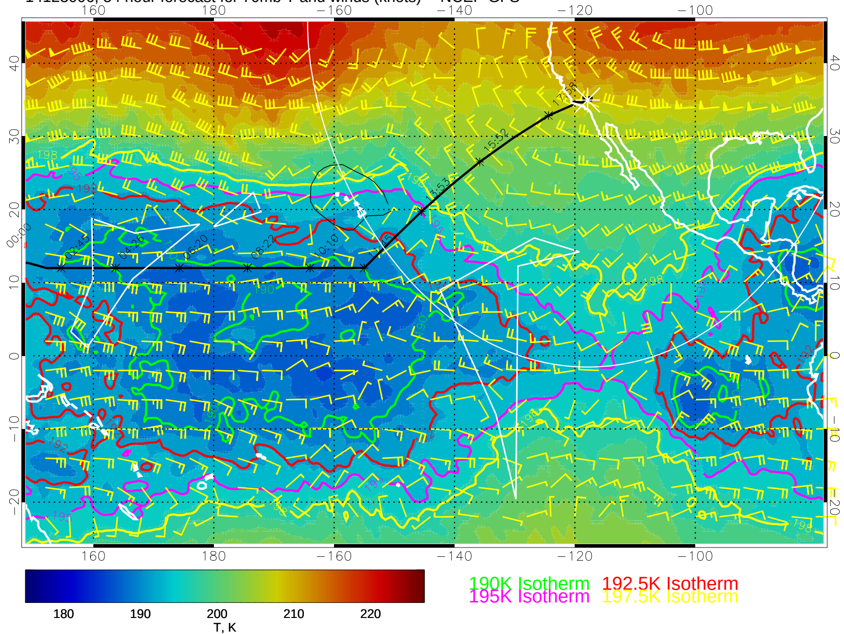
14123006, 54 hour forecast for 70mb T and winds (knots) -- NCEP GFS
