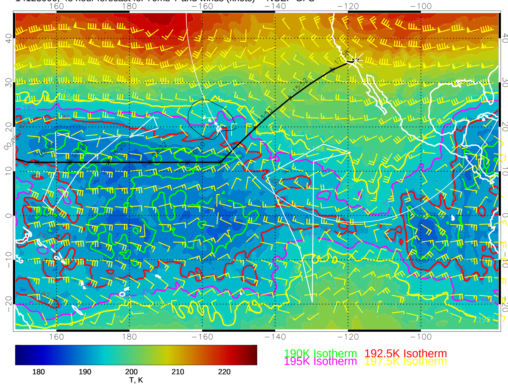
14123000, 48 hour forecast for 70mb T and winds (knots) -- NCEP GFS
