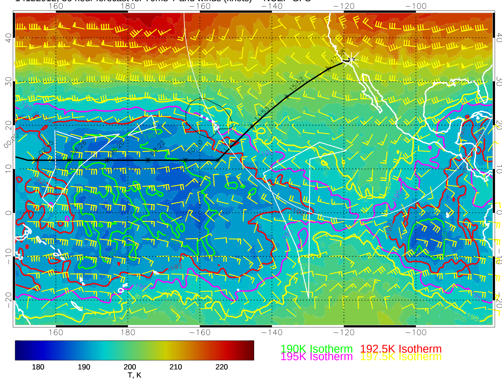
14122912, 36 hour forecast for 70mb T and winds (knots) -- NCEP GFS
