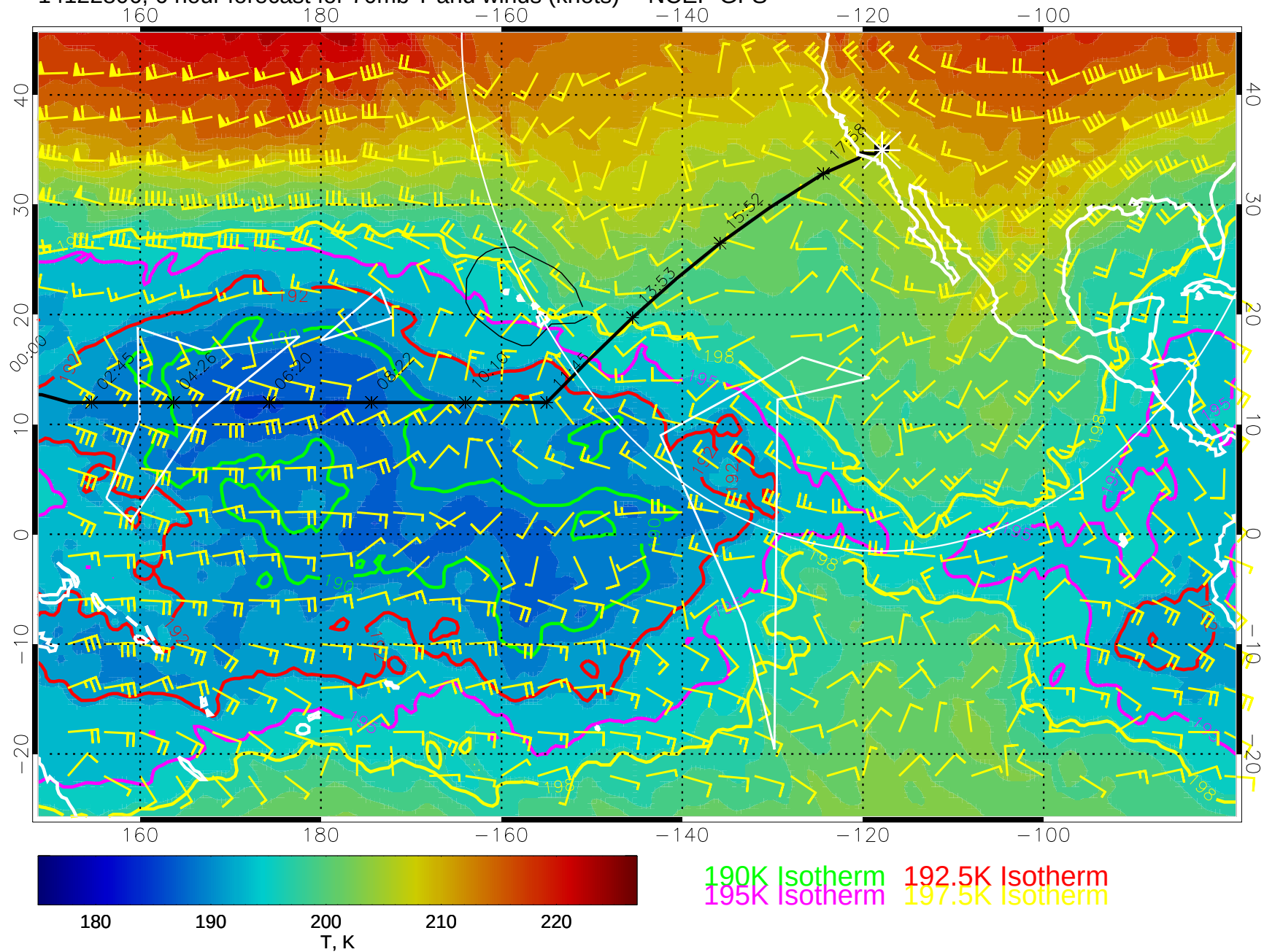
14122806, 6 hour forecast for 70mb T and winds (knots) -- NCEP GFS
