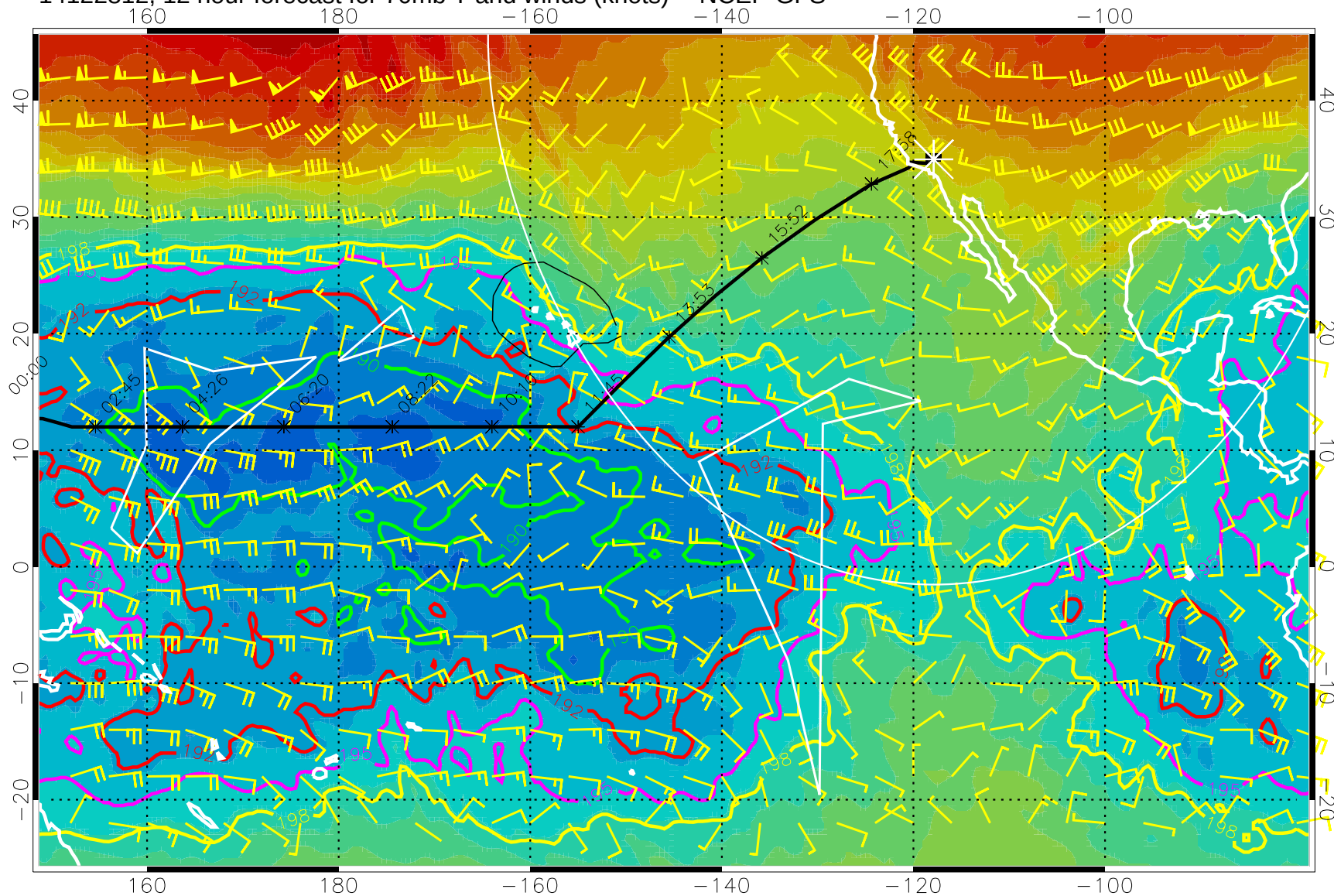
14122812, 12 hour forecast for 70mb T and winds (knots) -- NCEP GFS
