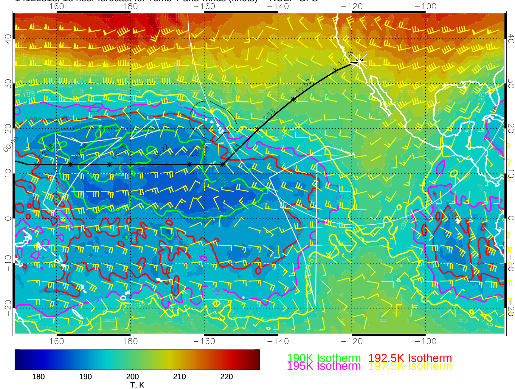
14122818, 18 hour forecast for 70mb T and winds (knots) -- NCEP GFS
