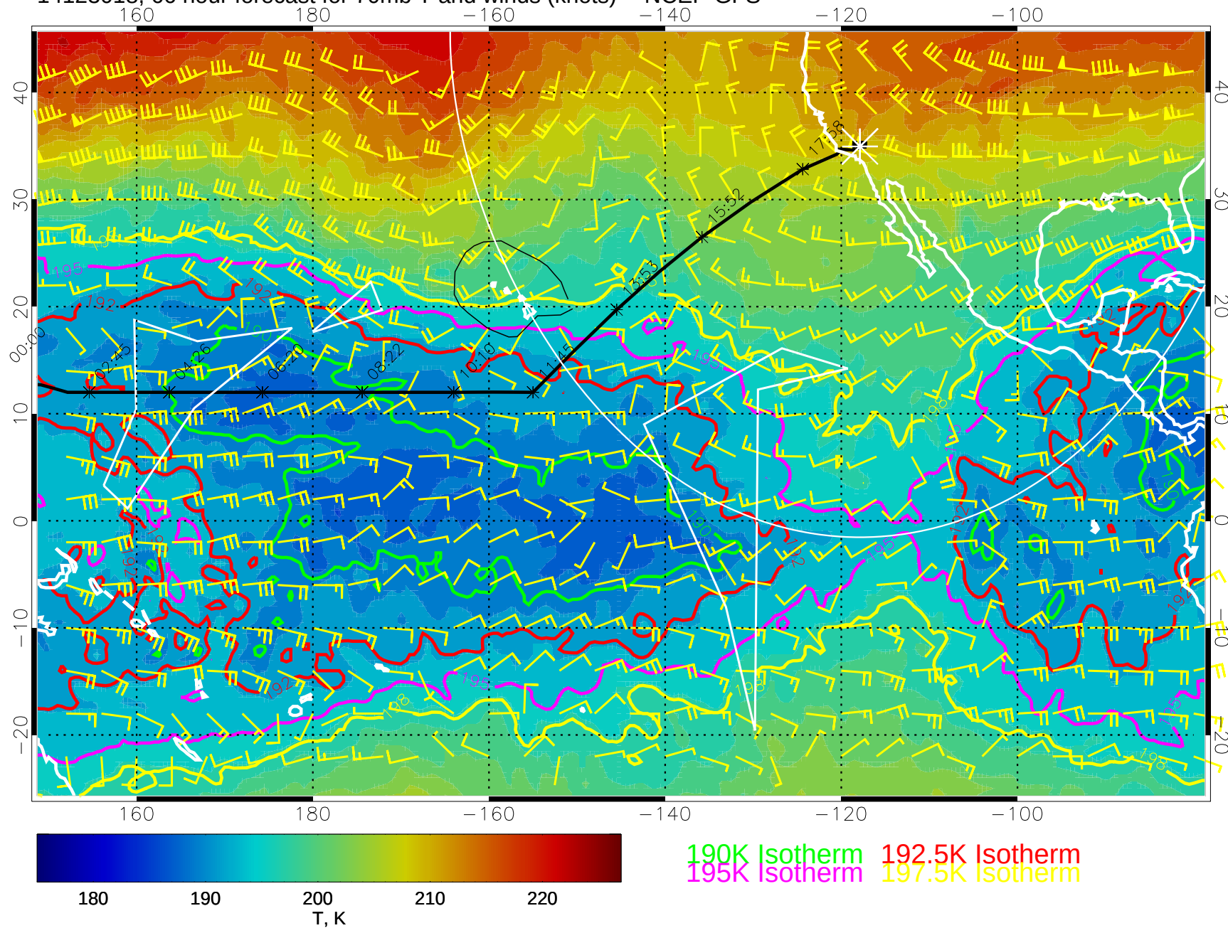
14123018, 66 hour forecast for 70mb T and winds (knots) -- NCEP GFS
