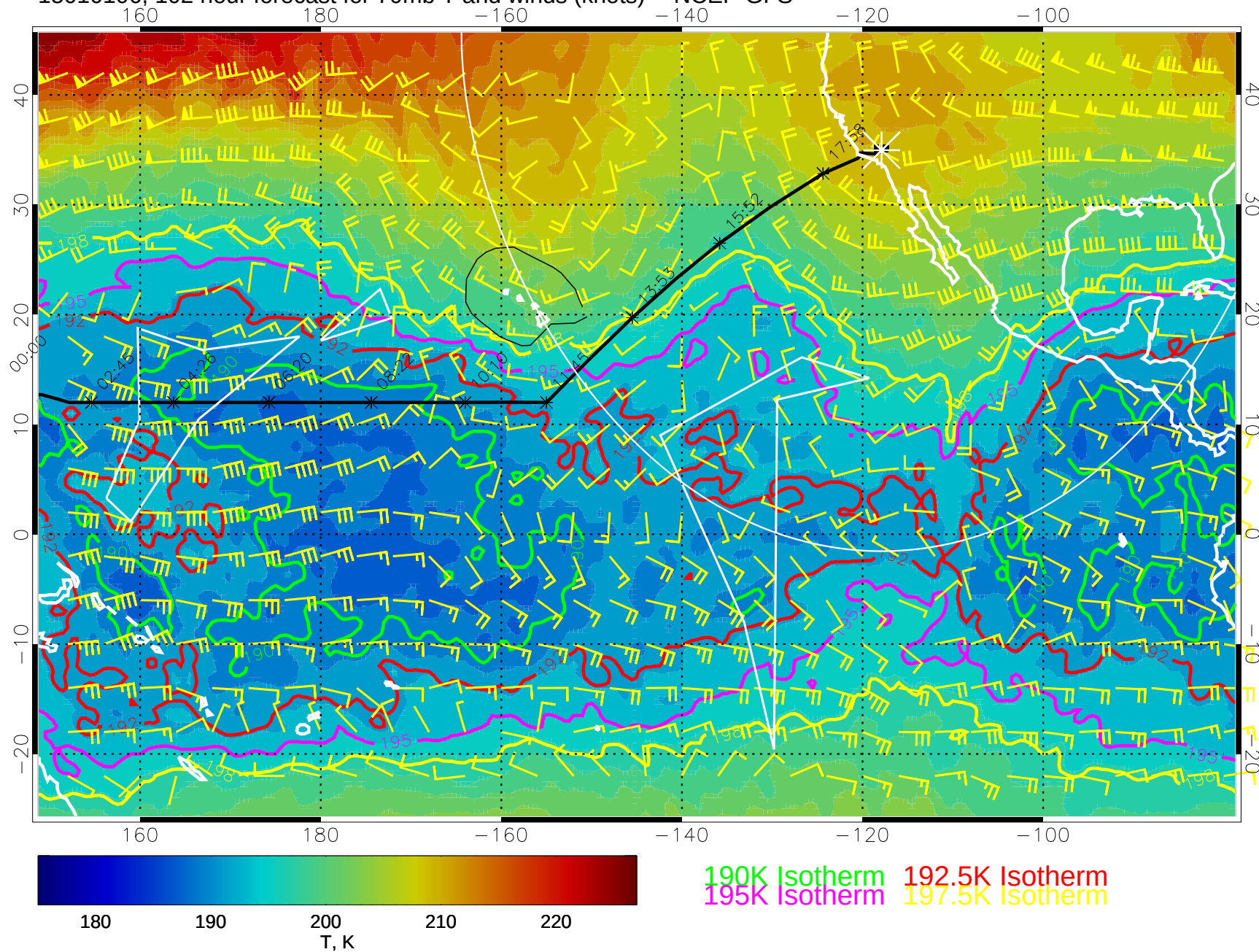
15010106, 102 hour forecast for 70mb T and winds (knots) -- NCEP GFS
