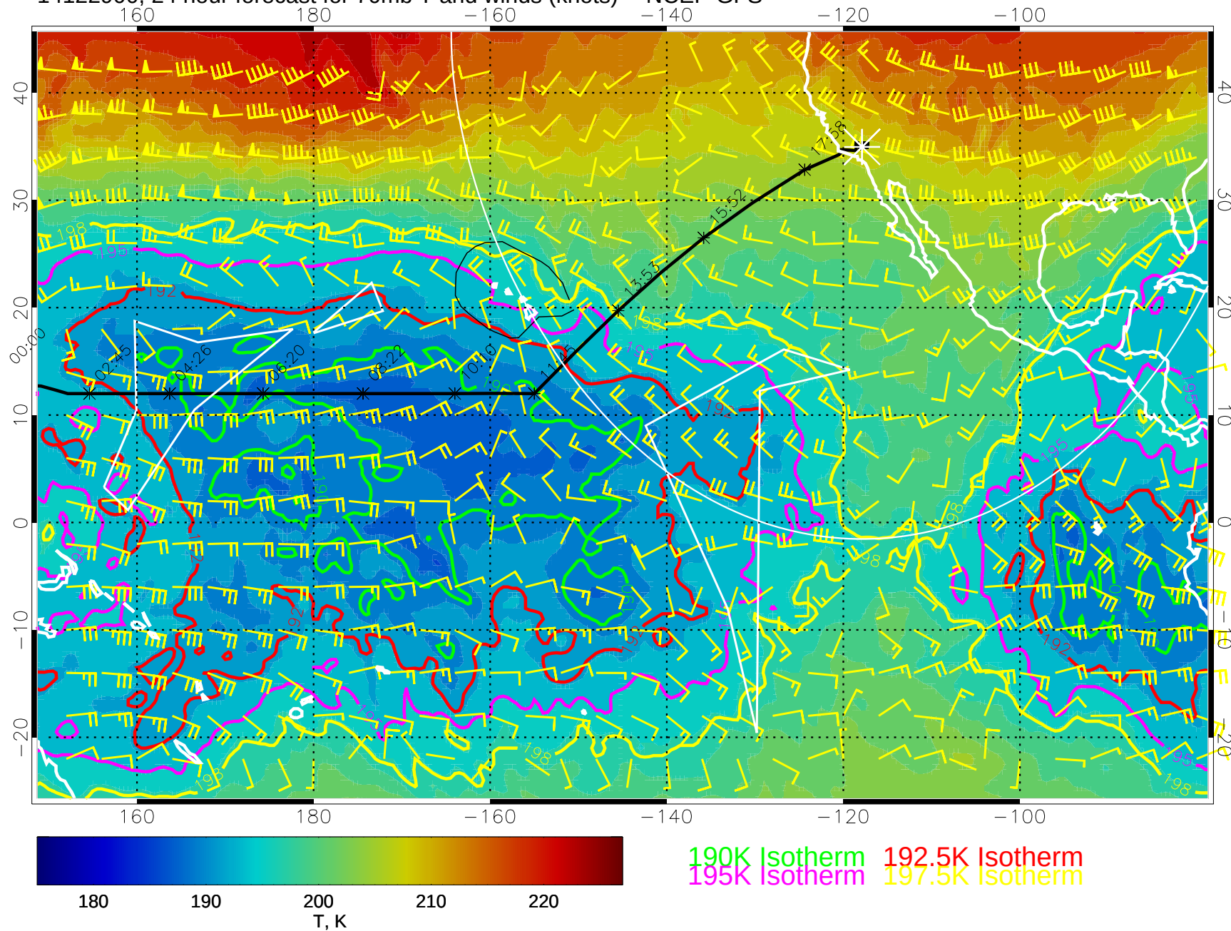
14122900, 24 hour forecast for 70mb T and winds (knots) -- NCEP GFS
