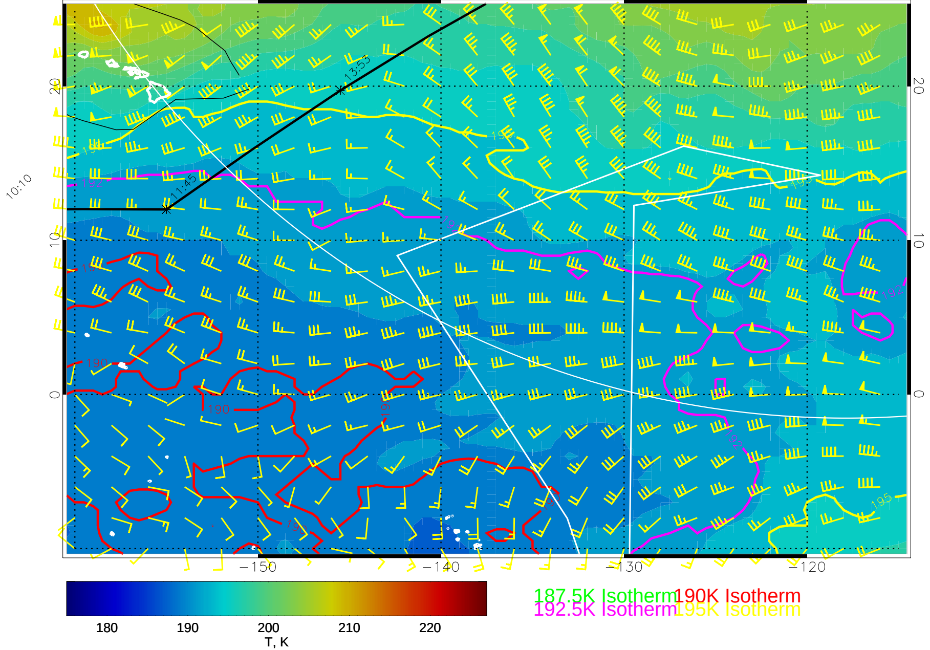
14123106, 78 hour forecast for 100mb T and winds (knots) -- NCEP GFS
