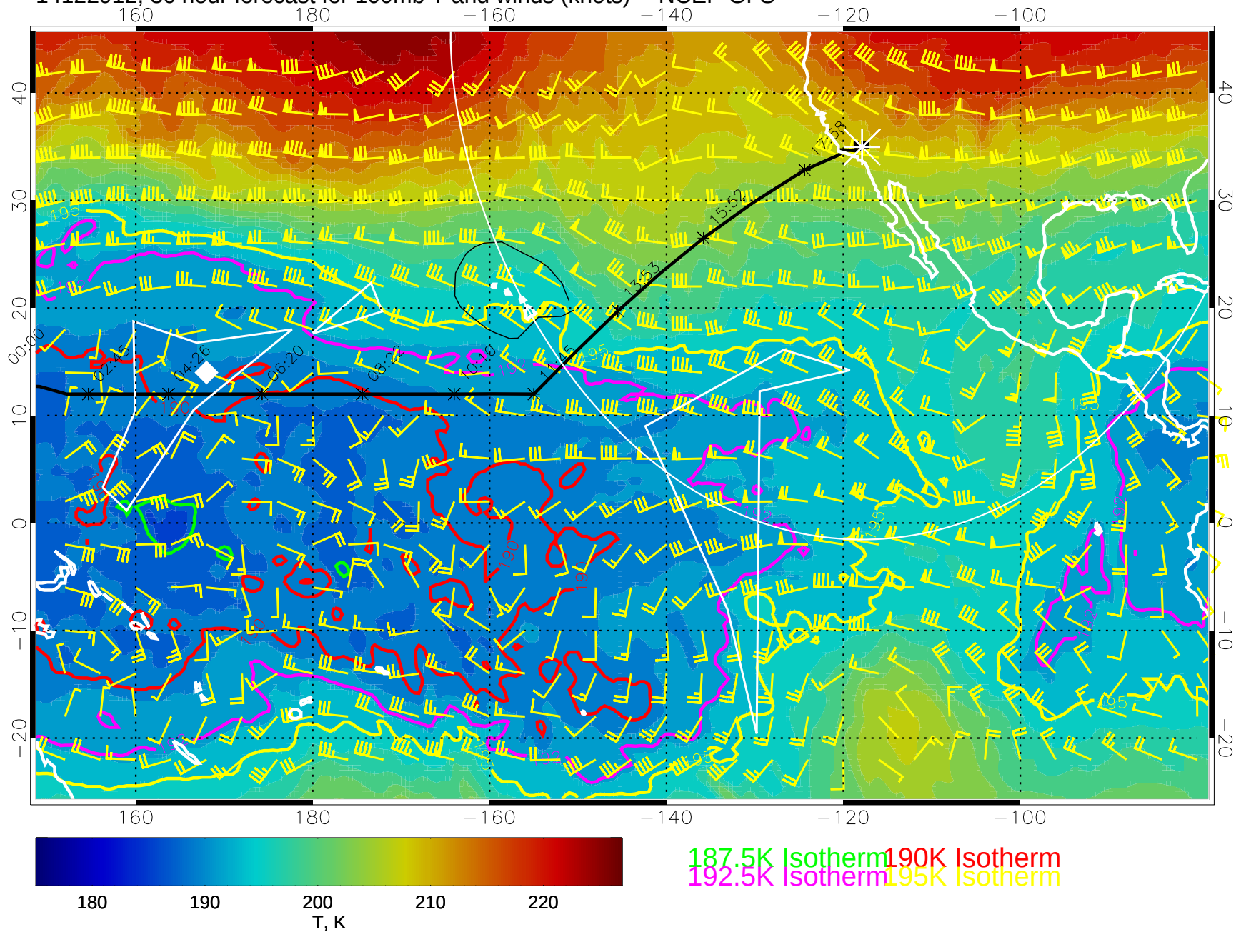
14122912, 36 hour forecast for 100mb T and winds (knots) -- NCEP GFS
