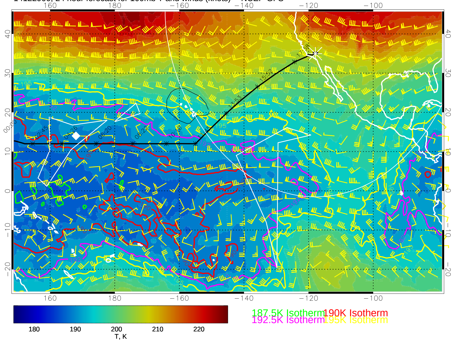
14122900, 24 hour forecast for 100mb T and winds (knots) -- NCEP GFS
