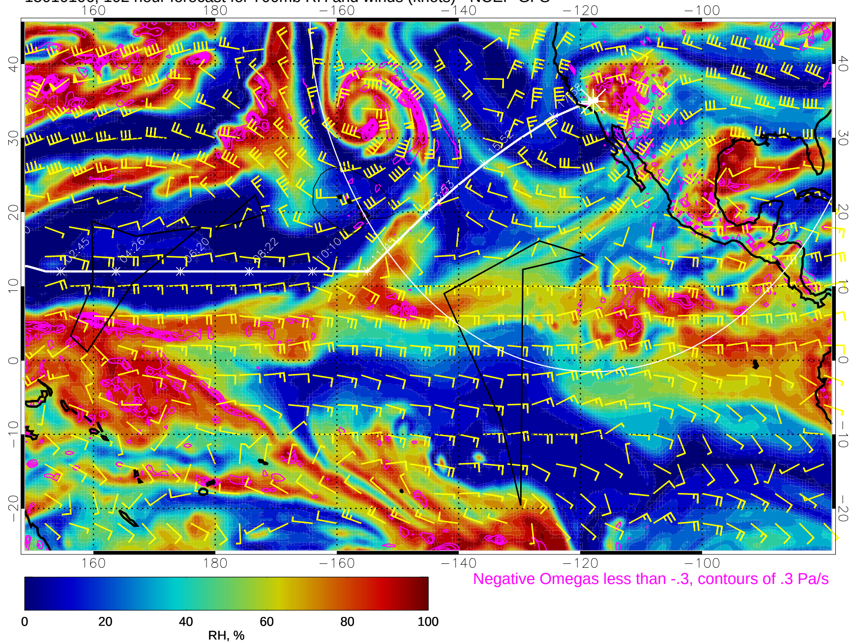
15010106, 102 hour forecast for 700mb RH and winds (knots) - NCEP GFS
