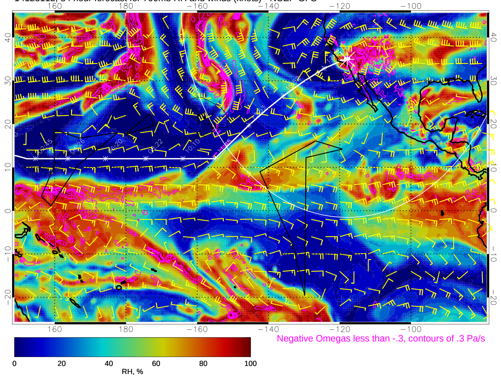
14123112, 84 hour forecast for 700mb RH and winds (knots) - NCEP GFS
