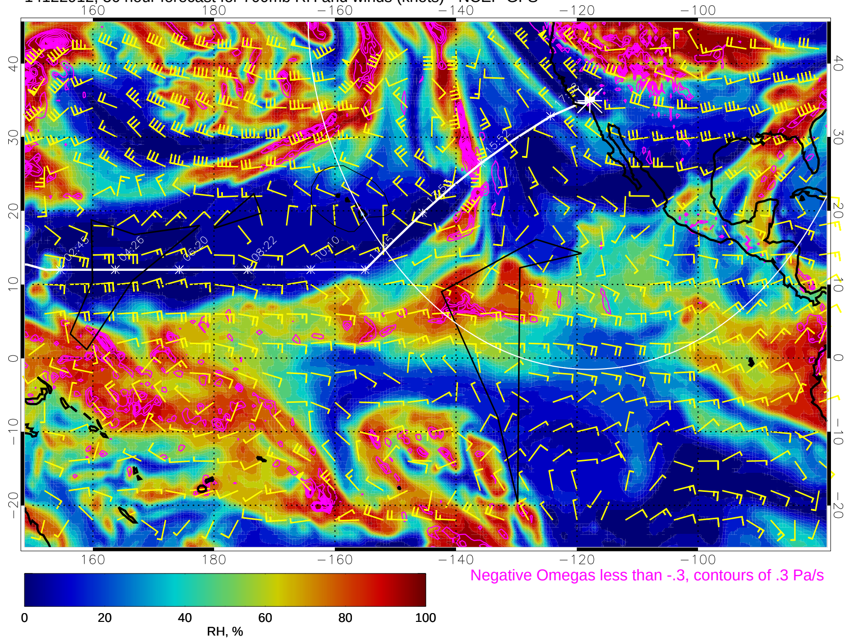
14122912, 36 hour forecast for 700mb RH and winds (knots) - NCEP GFS
