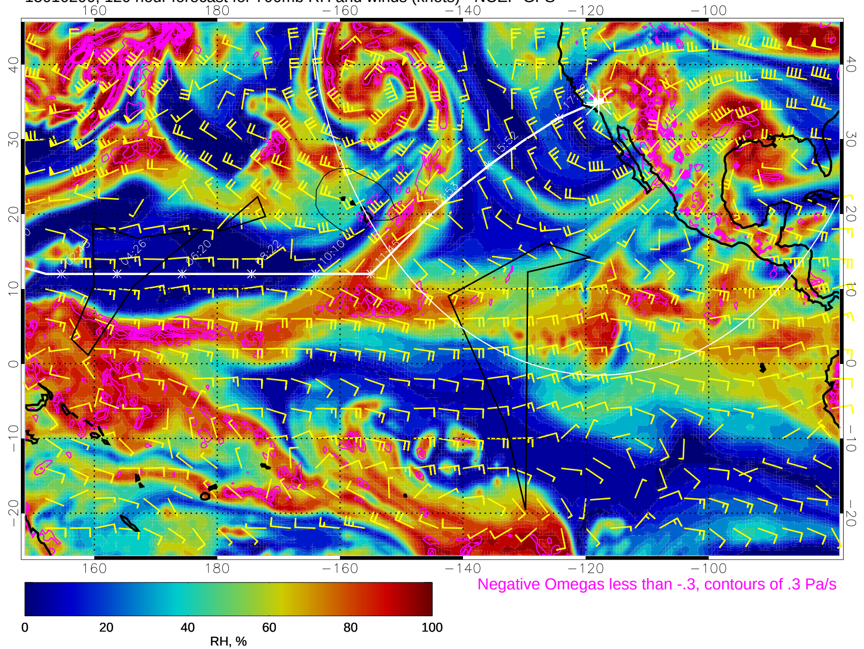
15010200, 120 hour forecast for 700mb RH and winds (knots) - NCEP GFS
