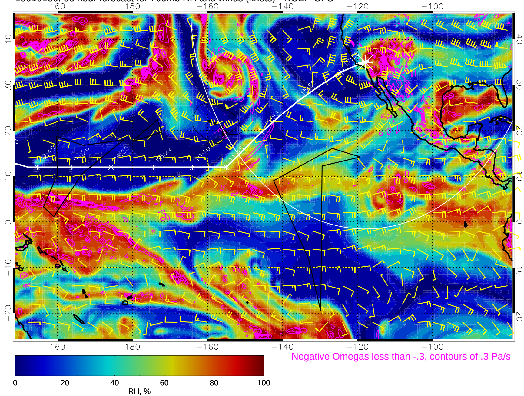
15010100, 96 hour forecast for 700mb RH and winds (knots) - NCEP GFS
