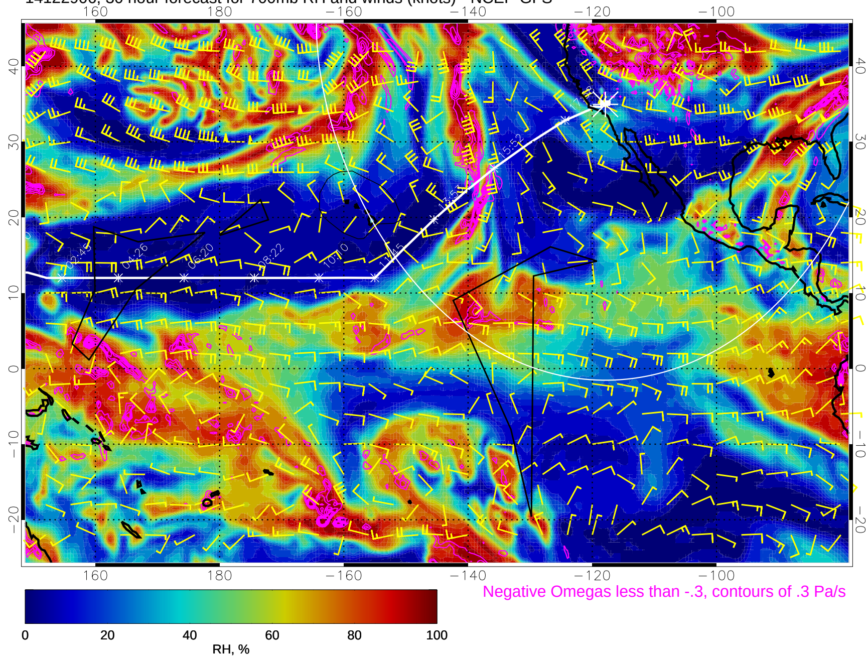
14122906, 30 hour forecast for 700mb RH and winds (knots) - NCEP GFS
