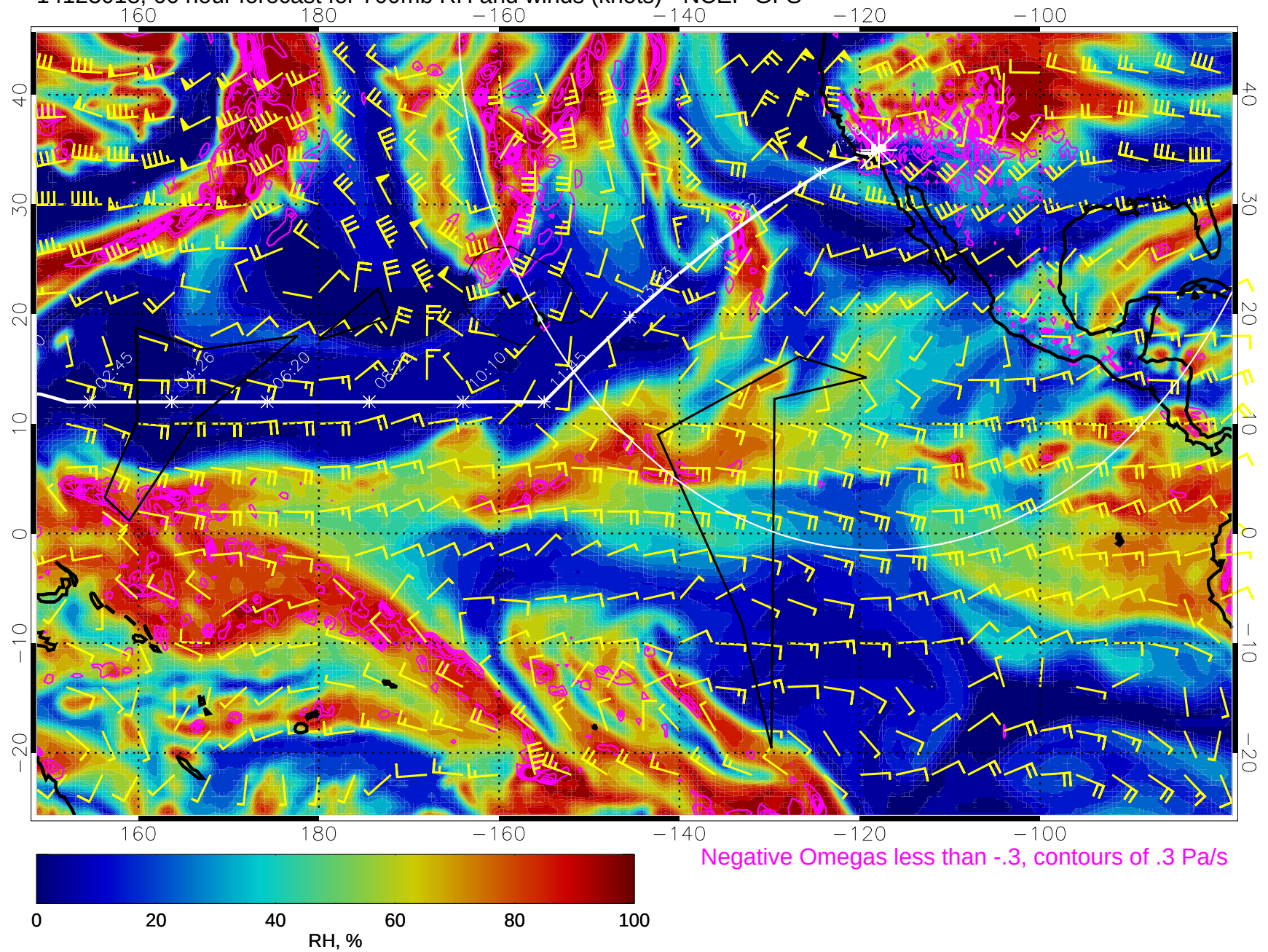
14123018, 66 hour forecast for 700mb RH and winds (knots) - NCEP GFS
