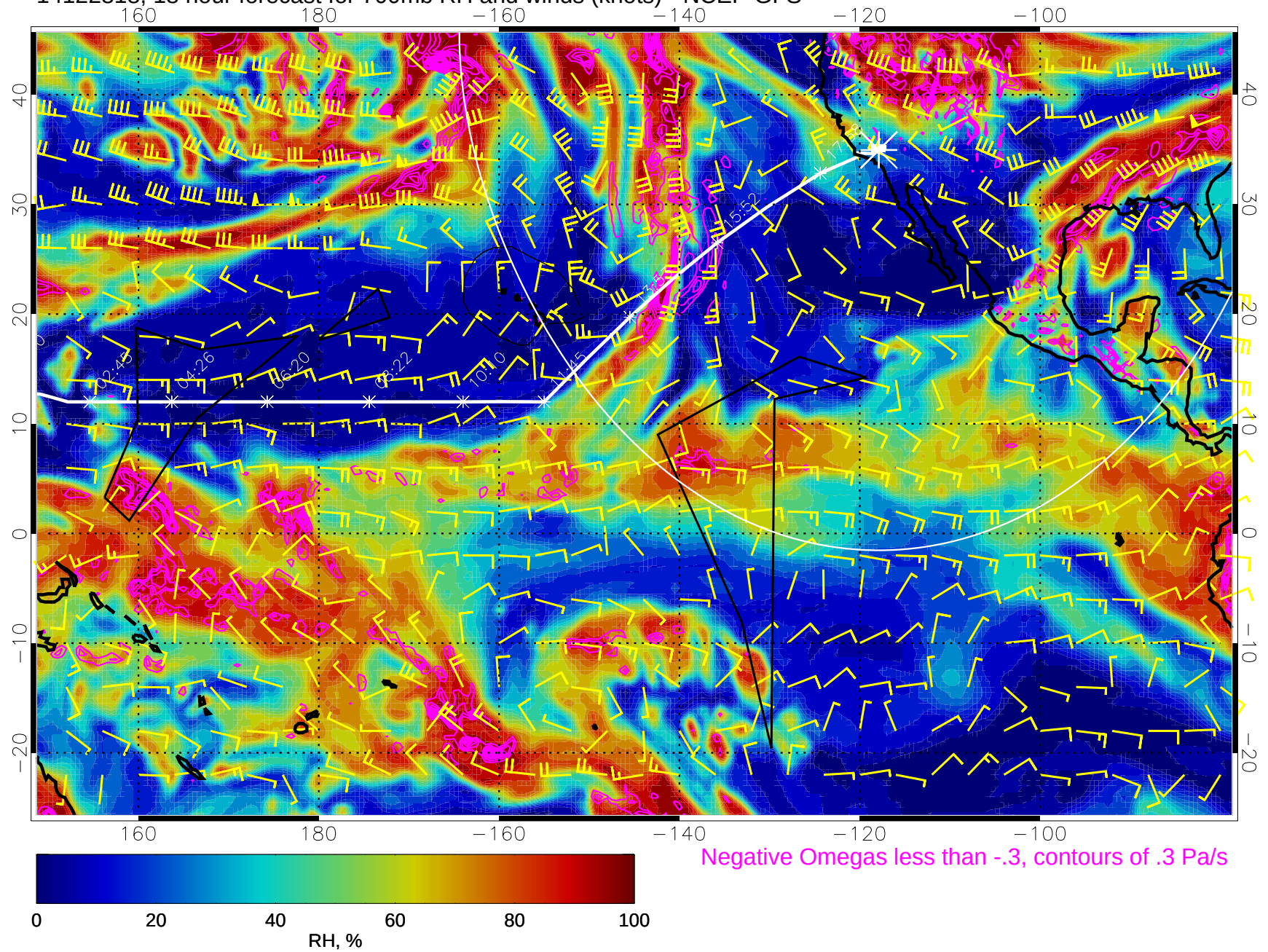
14122818, 18 hour forecast for 700mb RH and winds (knots) - NCEP GFS
