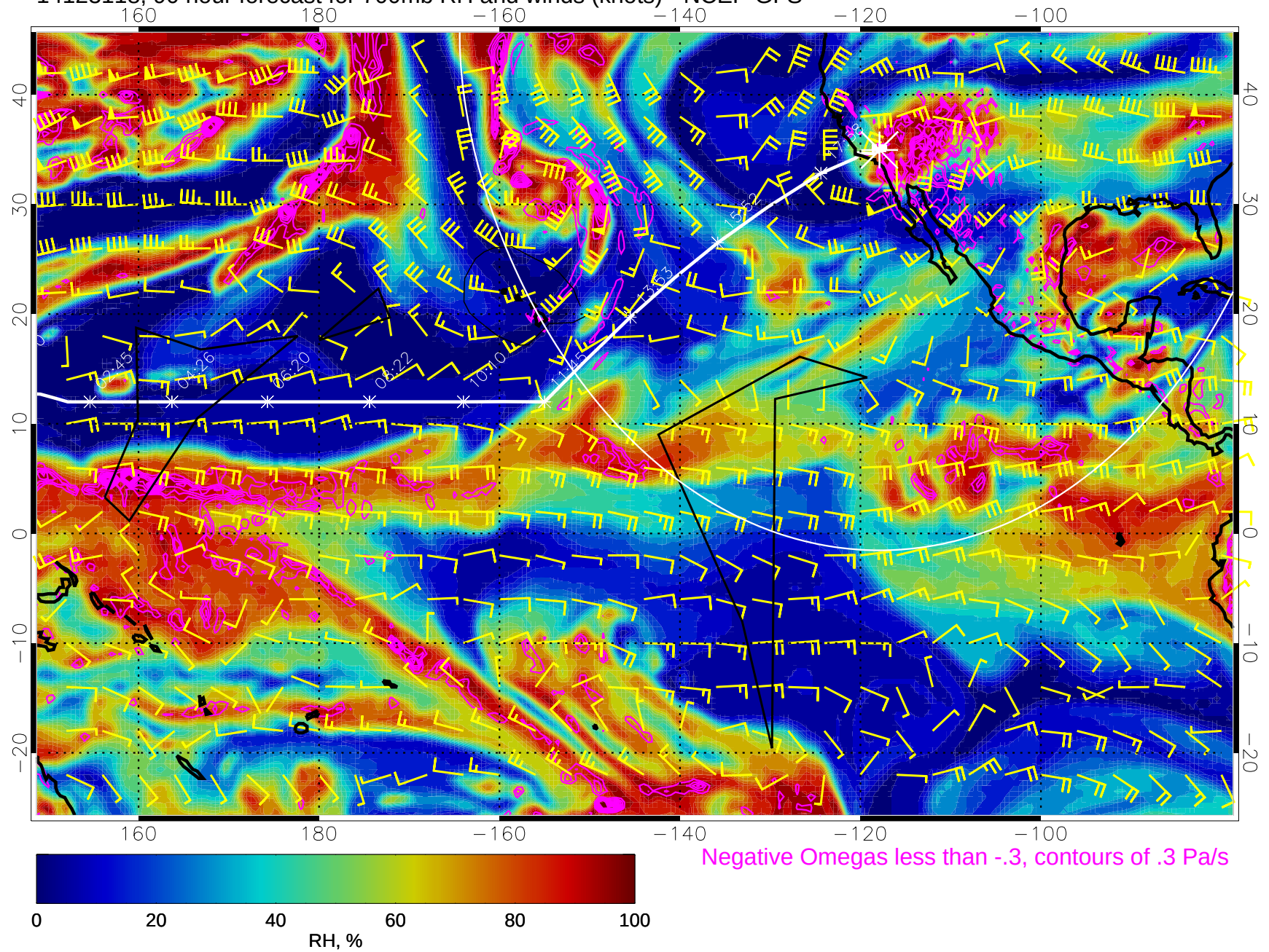
14123118, 90 hour forecast for 700mb RH and winds (knots) - NCEP GFS
