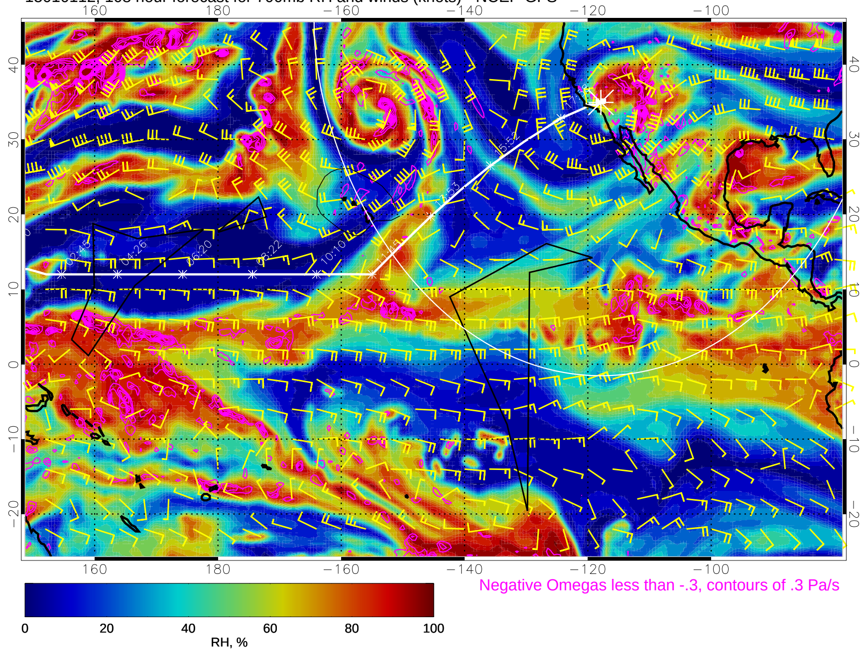
15010112, 108 hour forecast for 700mb RH and winds (knots) - NCEP GFS
