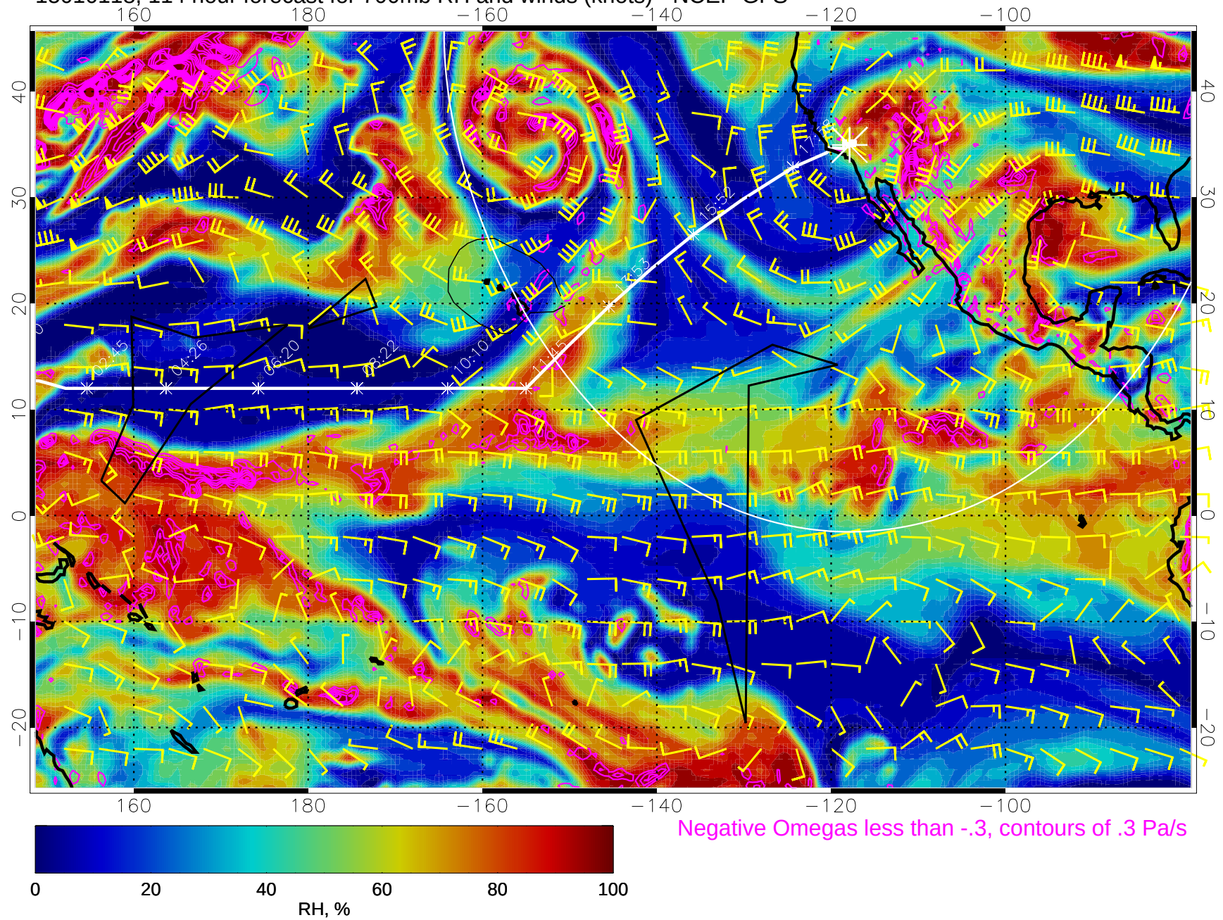
15010118, 114 hour forecast for 700mb RH and winds (knots) - NCEP GFS
