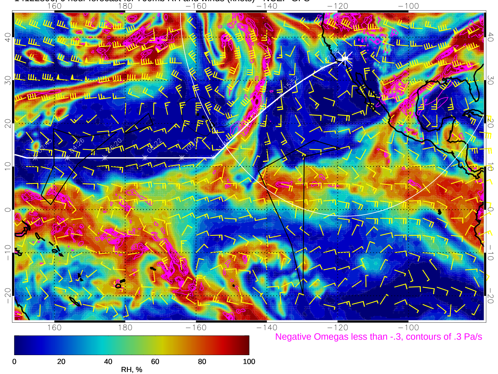
14122806, 6 hour forecast for 700mb RH and winds (knots) - NCEP GFS
