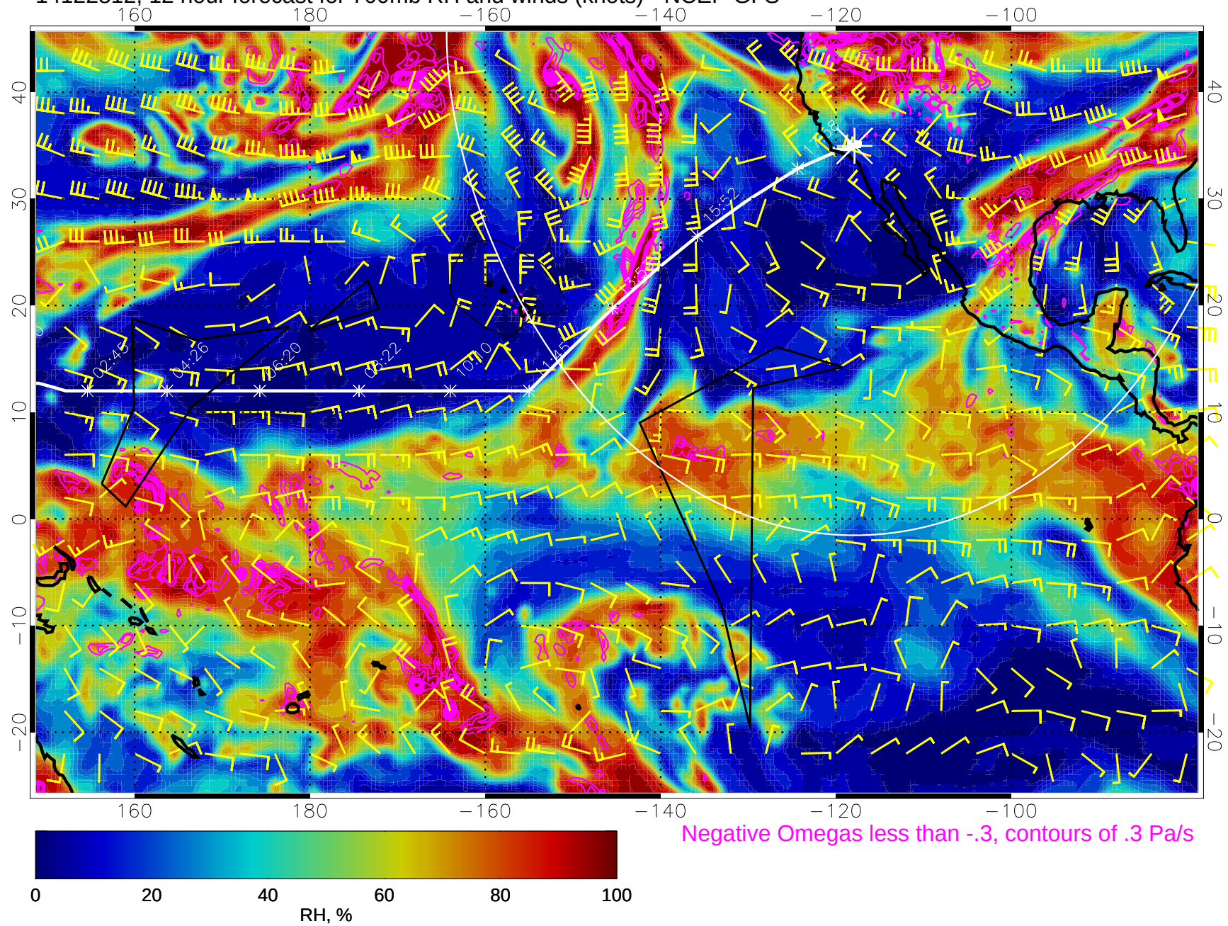
14122812, 12 hour forecast for 700mb RH and winds (knots) - NCEP GFS
