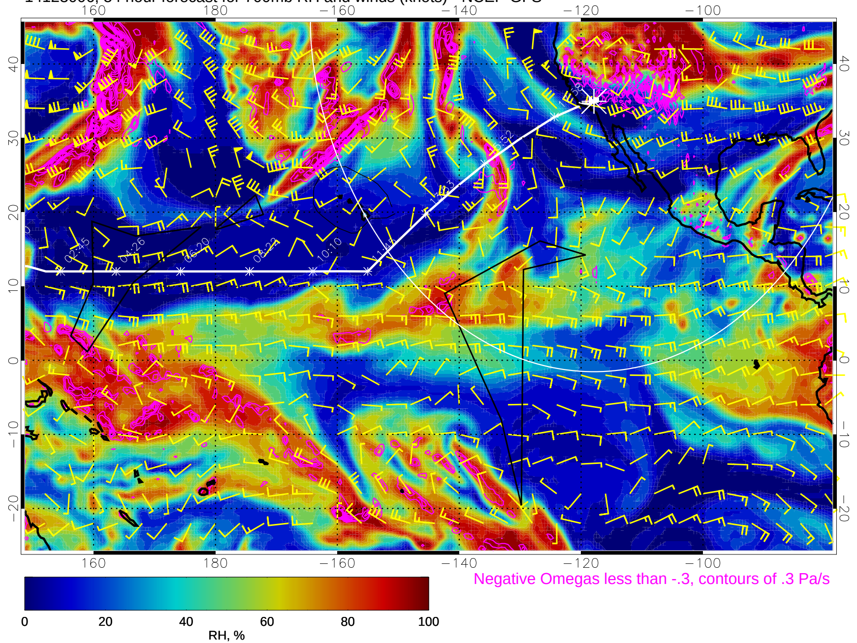
14123006, 54 hour forecast for 700mb RH and winds (knots) - NCEP GFS
