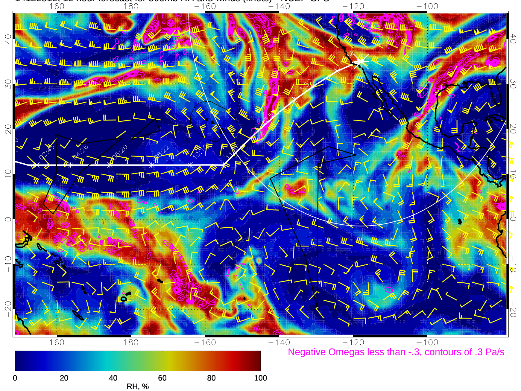
14122812, 12 hour forecast for 500mb RH and winds (knots) - NCEP GFS
