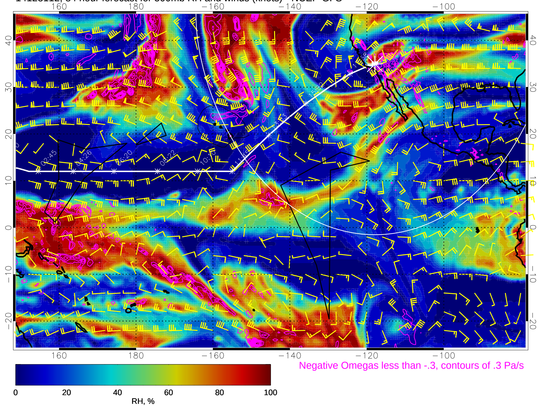
14123112, 84 hour forecast for 500mb RH and winds (knots) - NCEP GFS
