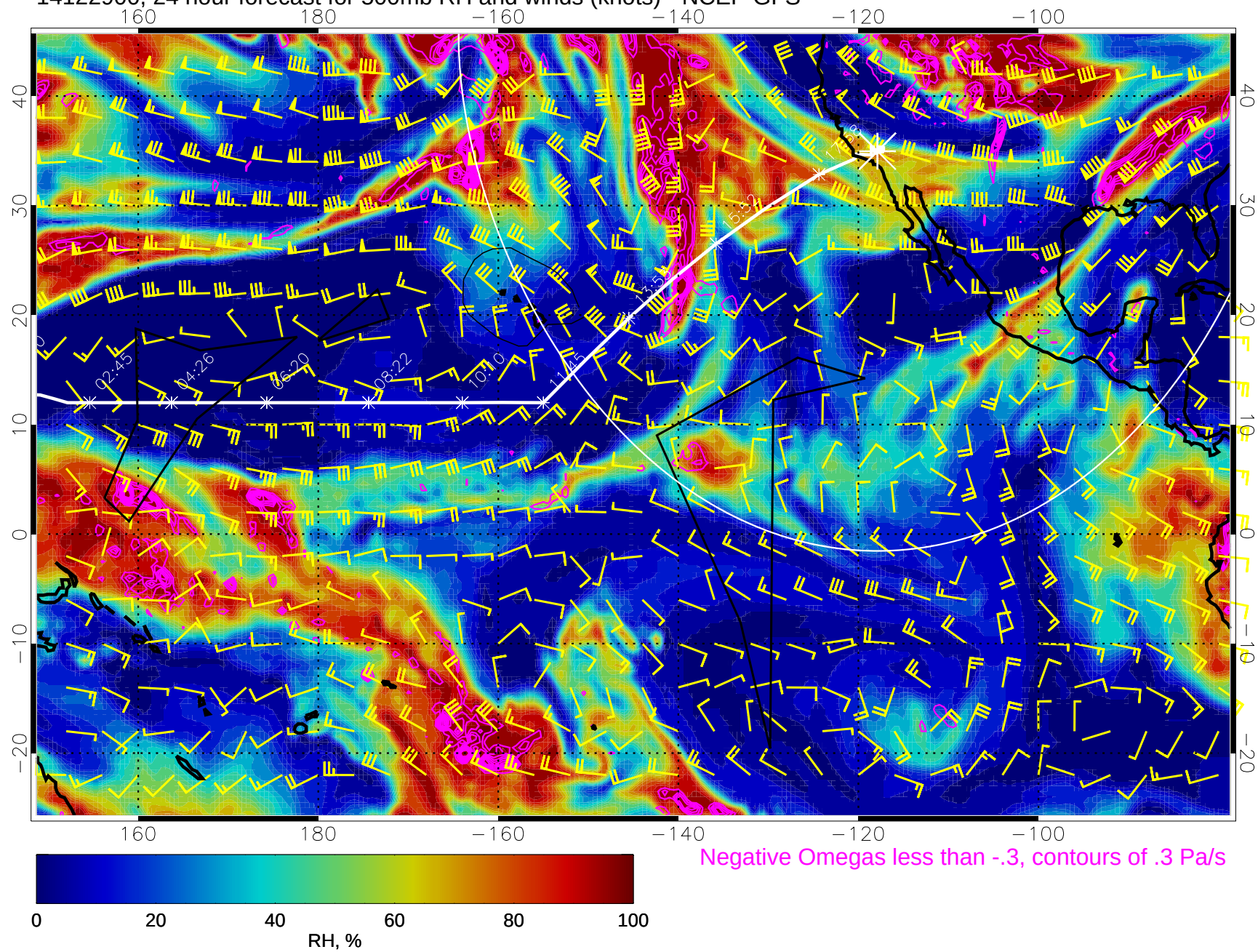
14122900, 24 hour forecast for 500mb RH and winds (knots) - NCEP GFS
