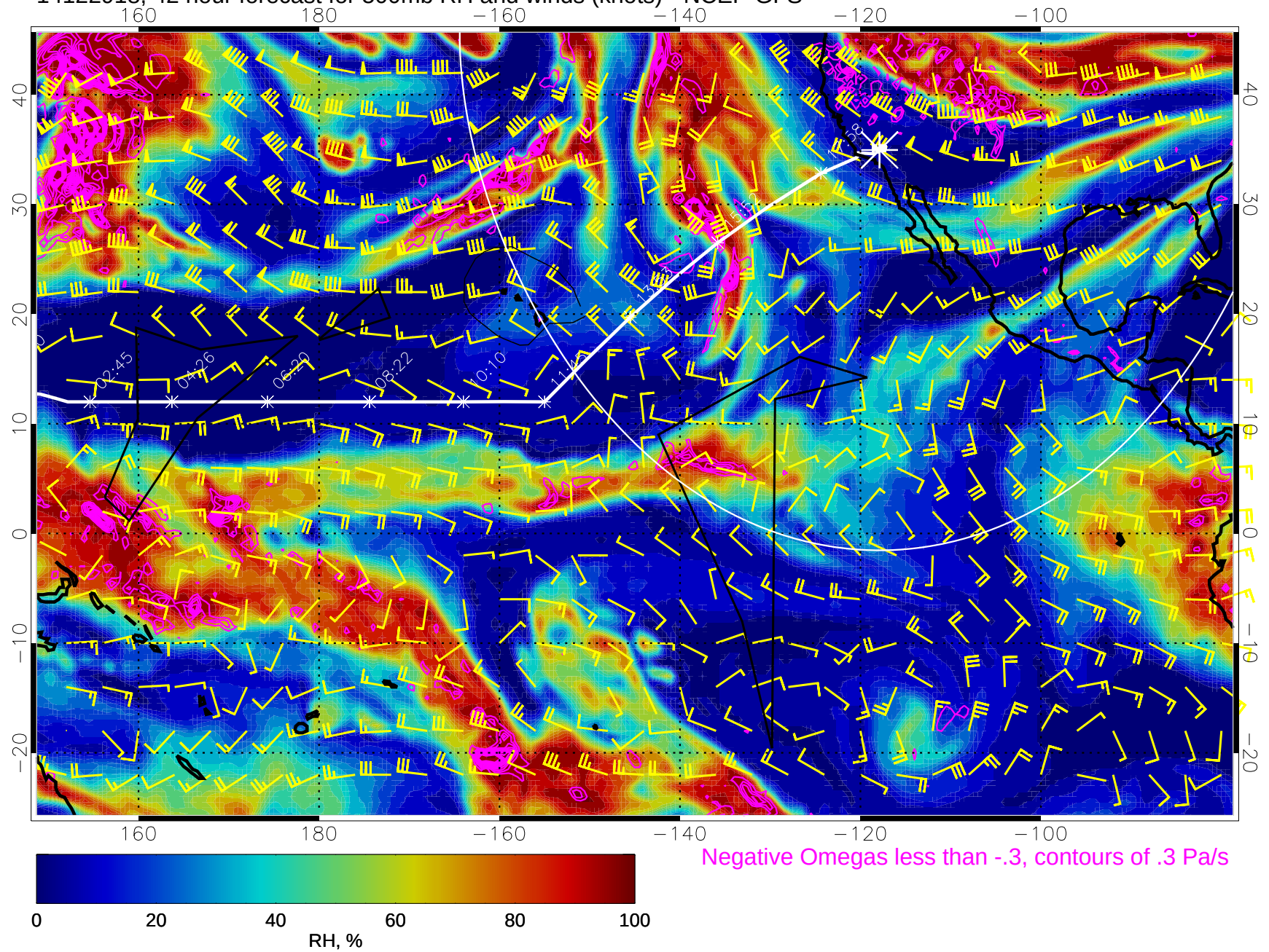
14122918, 42 hour forecast for 500mb RH and winds (knots) - NCEP GFS
