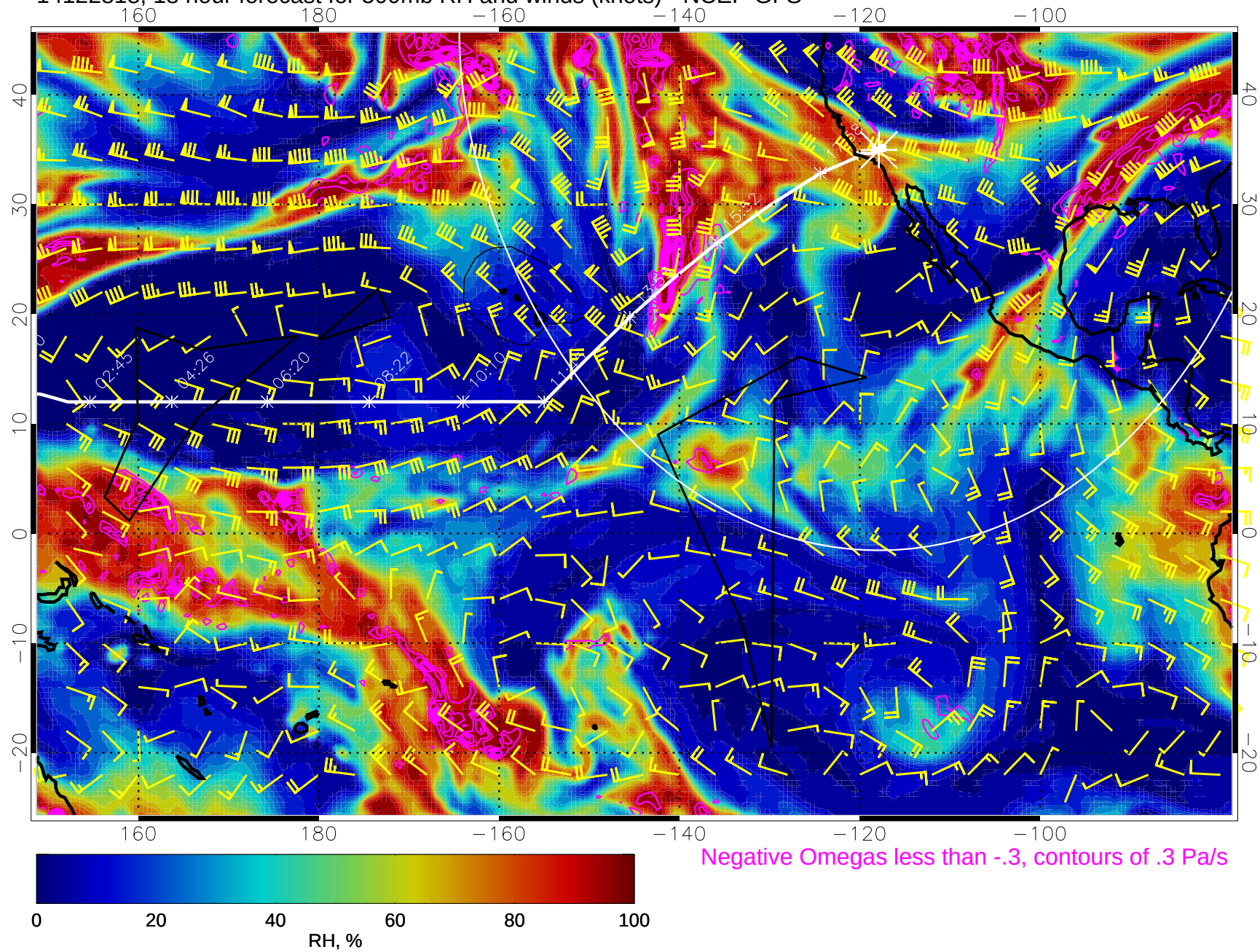
14122818, 18 hour forecast for 500mb RH and winds (knots) - NCEP GFS
