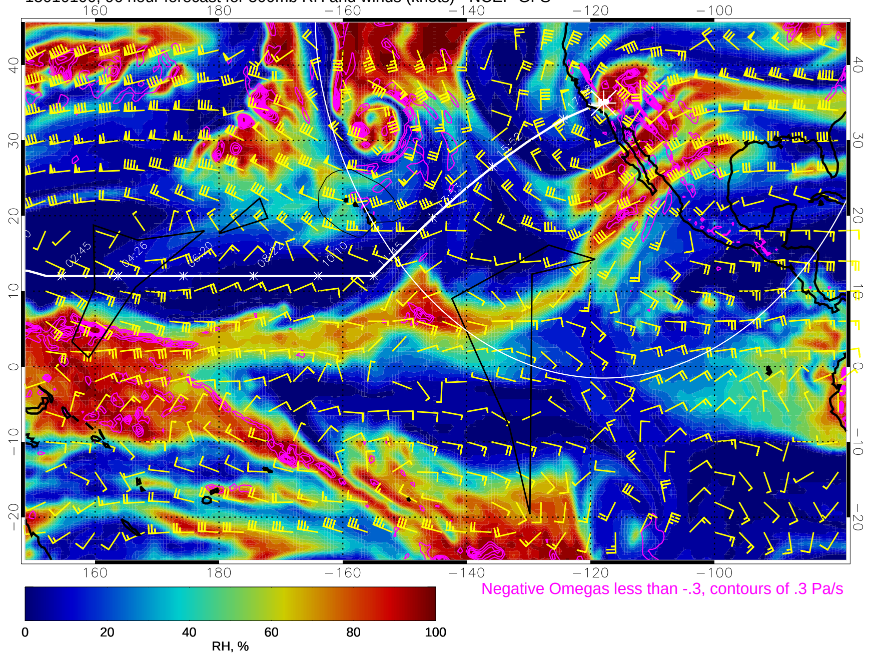
15010100, 96 hour forecast for 500mb RH and winds (knots) - NCEP GFS
