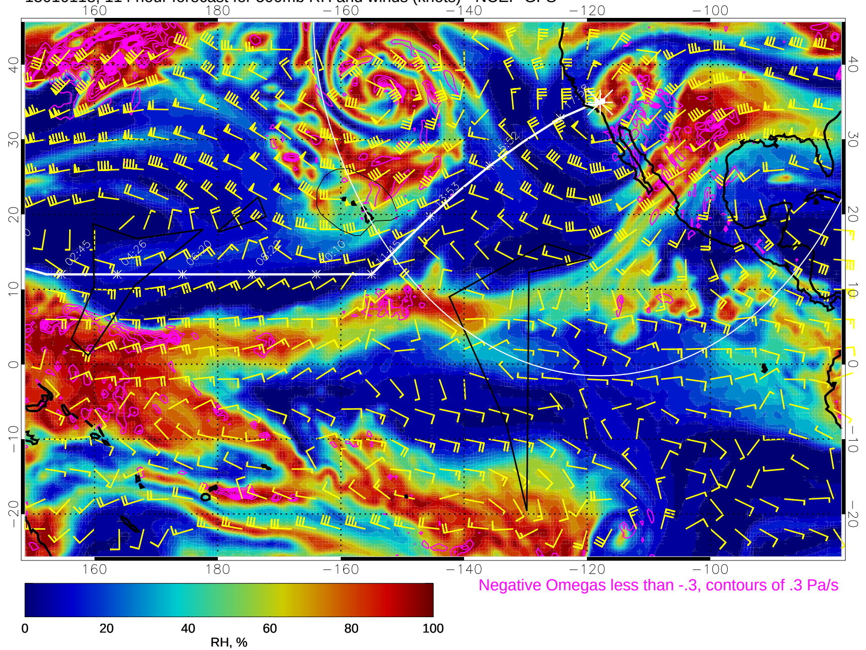
15010118, 114 hour forecast for 500mb RH and winds (knots) - NCEP GFS
