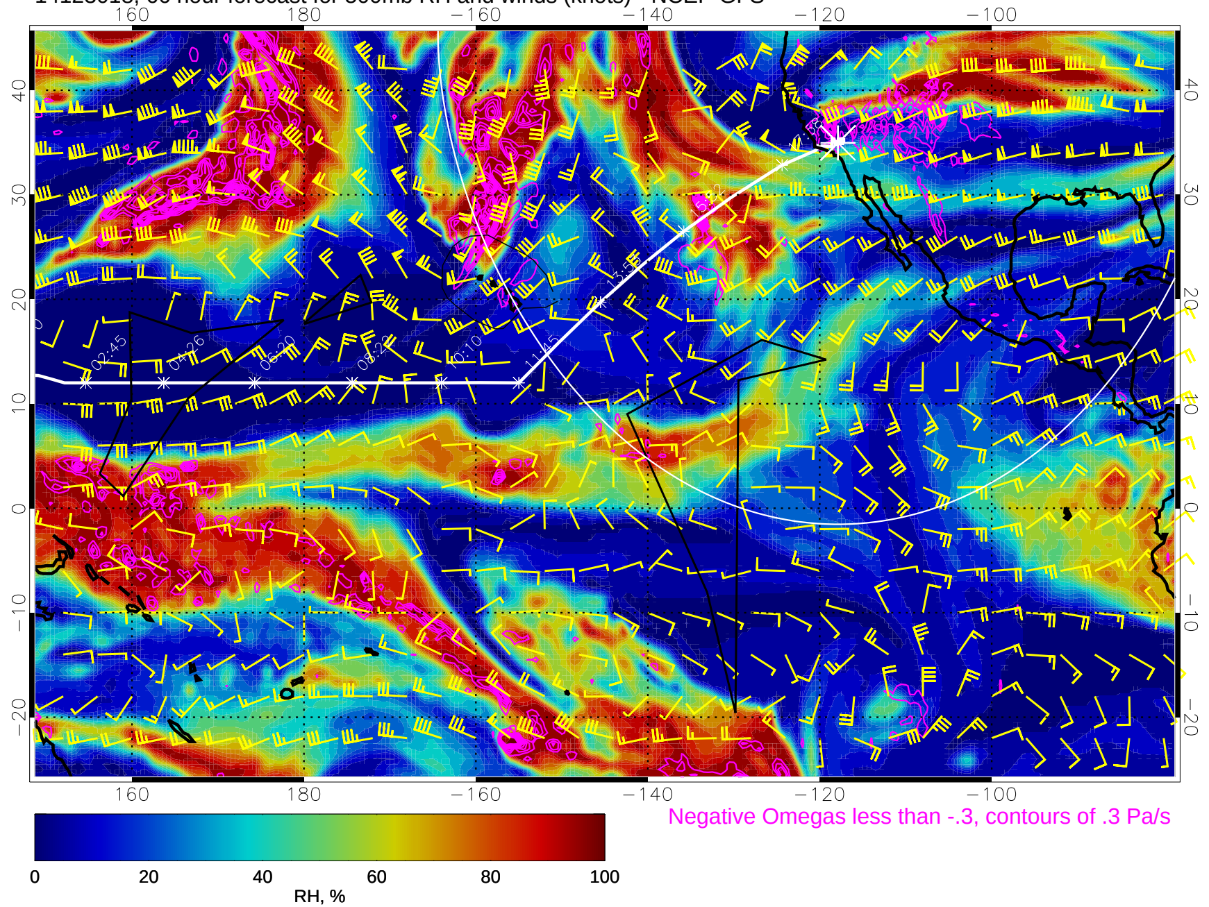
14123018, 66 hour forecast for 500mb RH and winds (knots) - NCEP GFS
