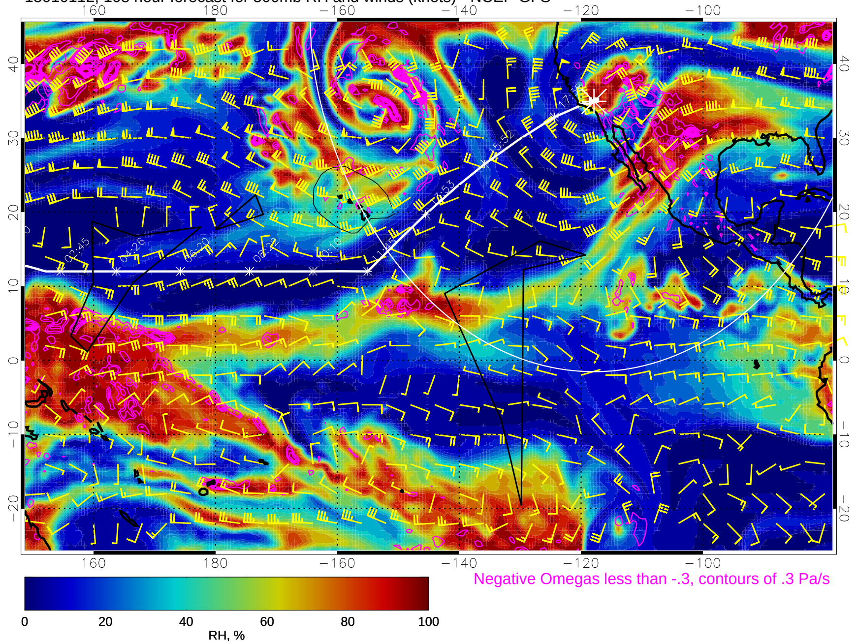
15010112, 108 hour forecast for 500mb RH and winds (knots) - NCEP GFS
