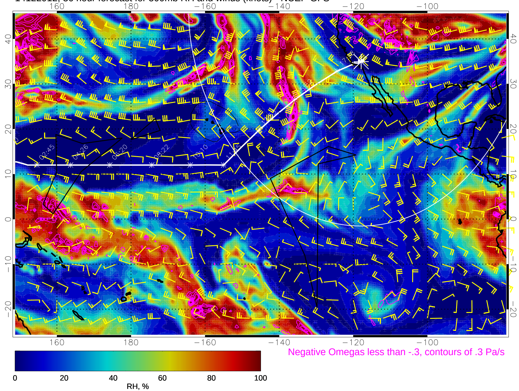
14122912, 36 hour forecast for 500mb RH and winds (knots) - NCEP GFS
