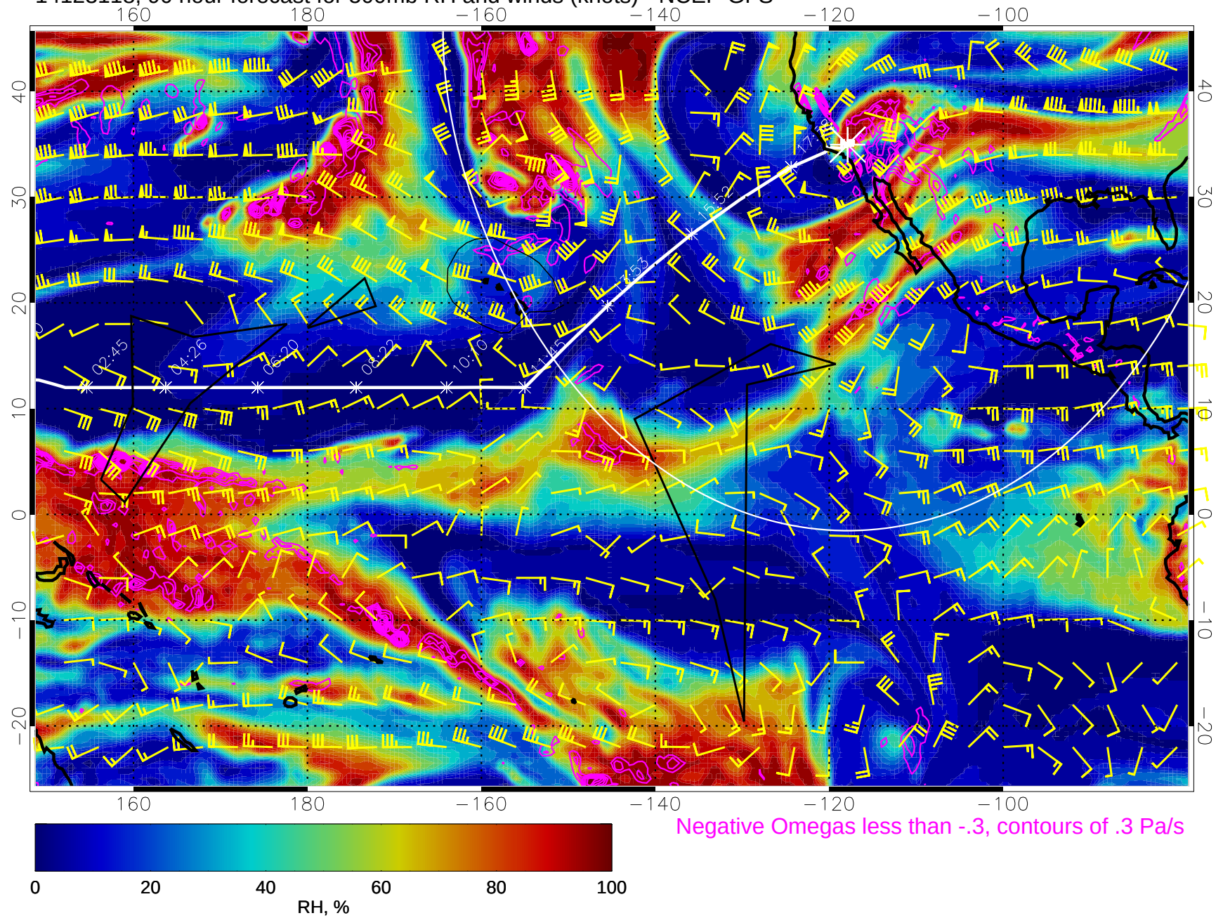
14123118, 90 hour forecast for 500mb RH and winds (knots) - NCEP GFS
