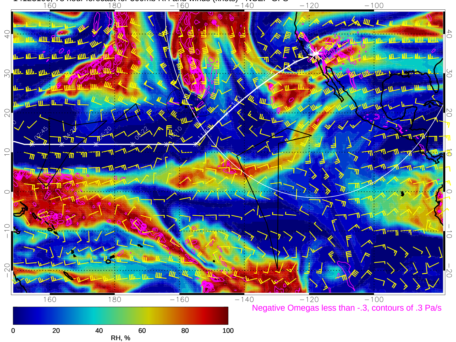
14123106, 78 hour forecast for 500mb RH and winds (knots) - NCEP GFS
