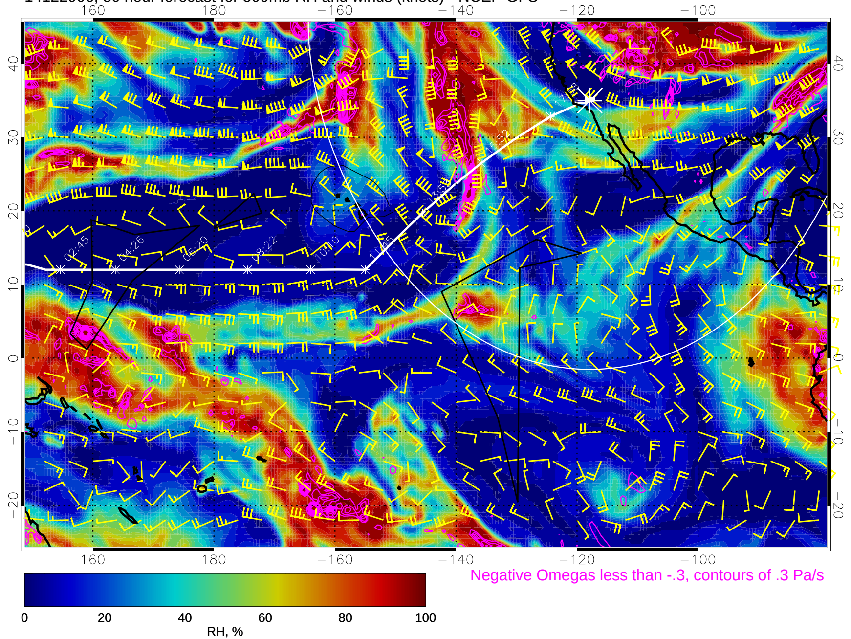
14122906, 30 hour forecast for 500mb RH and winds (knots) - NCEP GFS
