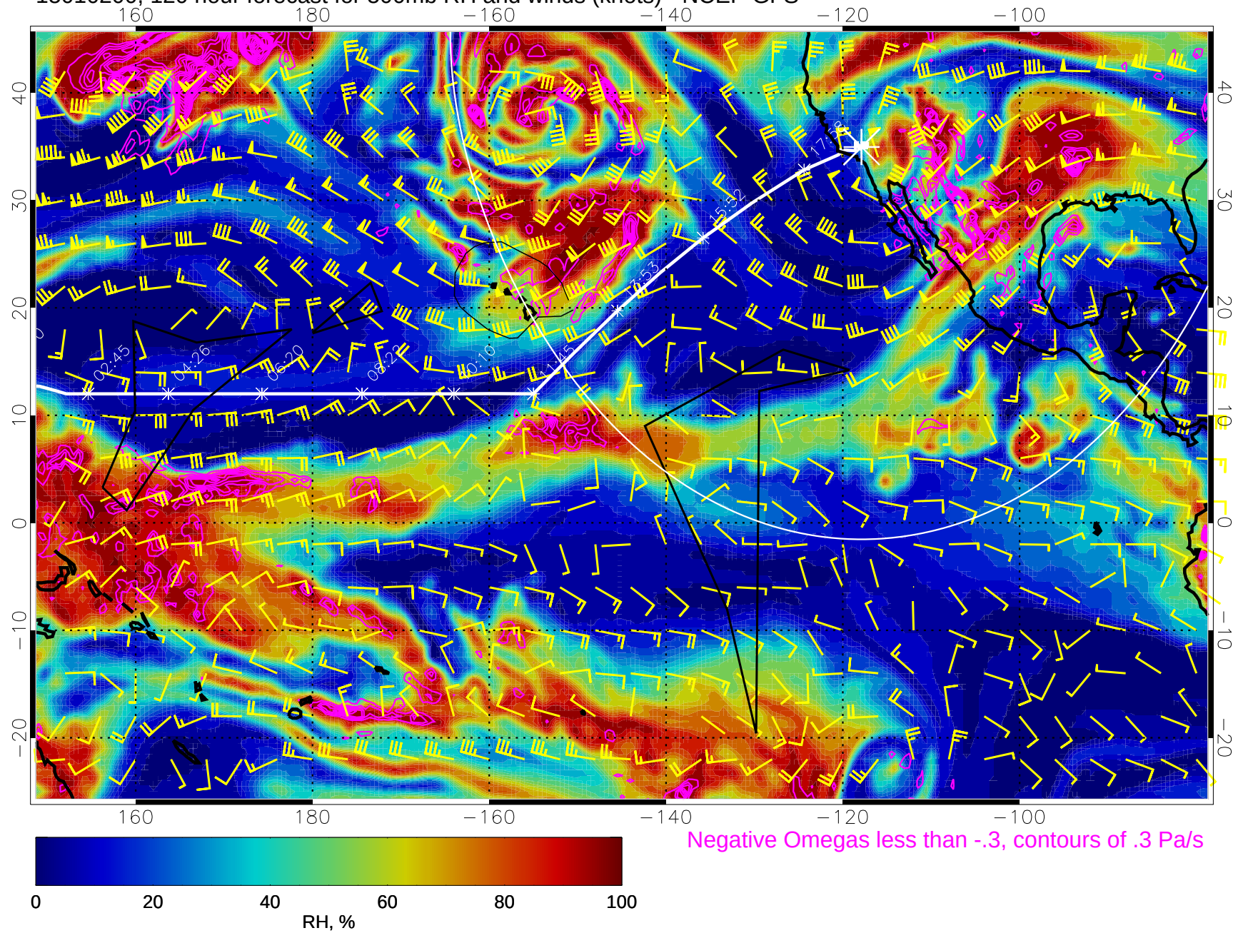
15010200, 120 hour forecast for 500mb RH and winds (knots) - NCEP GFS
