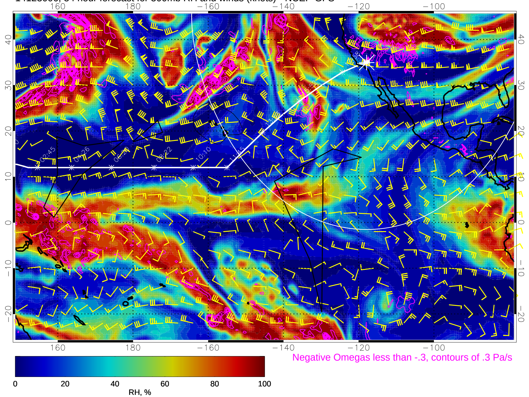
14123006, 54 hour forecast for 500mb RH and winds (knots) - NCEP GFS
