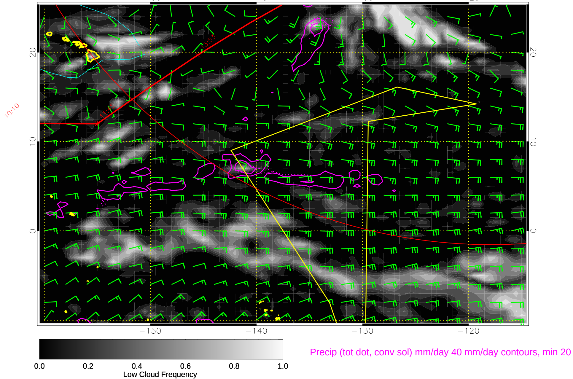
14123000, 48 hour forecast for 850mb winds (knots) and Low Cloud Frequency -- NCEP GFS
