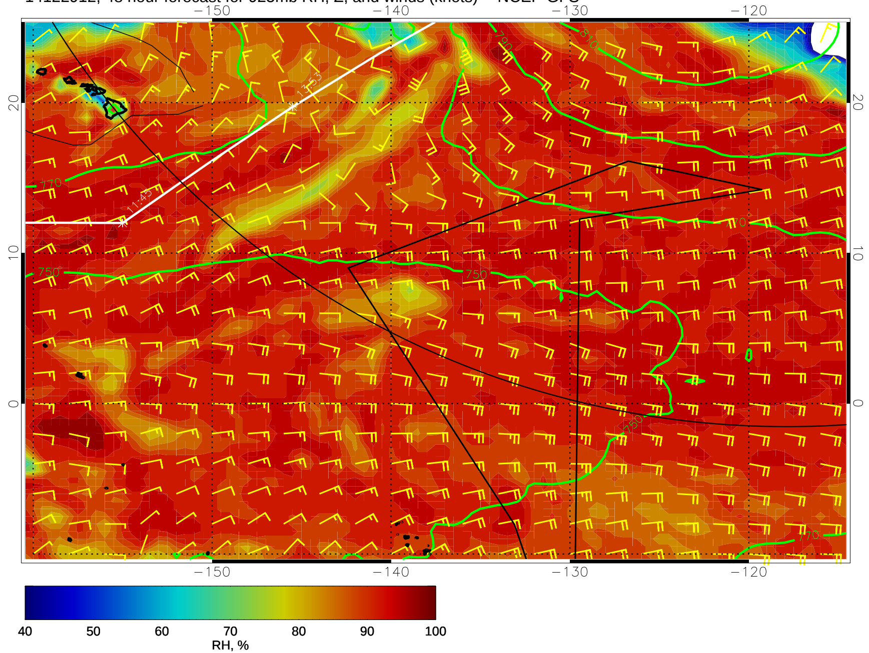
14122912, 48 hour forecast for 925mb RH, Z, and winds (knots) -- NCEP GFS
