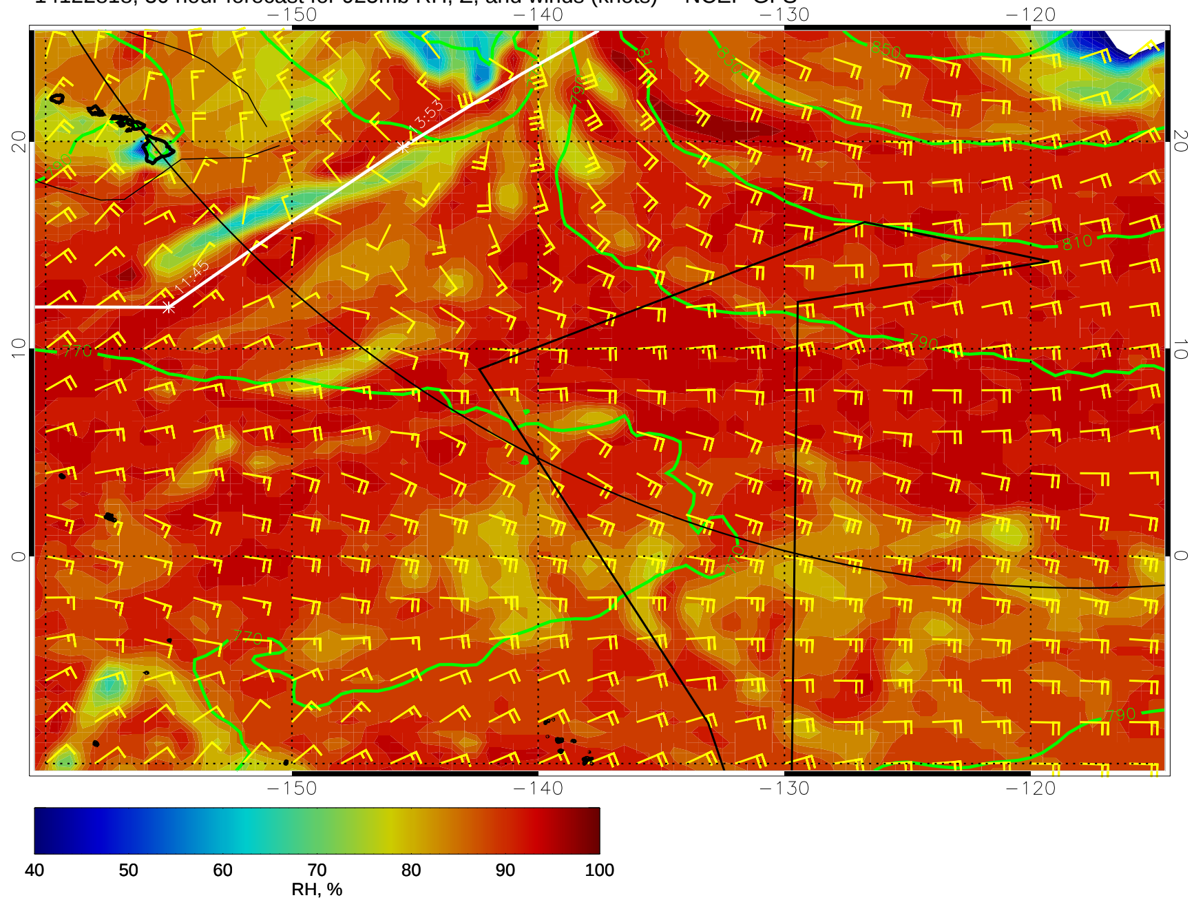
14122818, 30 hour forecast for 925mb RH, Z, and winds (knots) -- NCEP GFS
