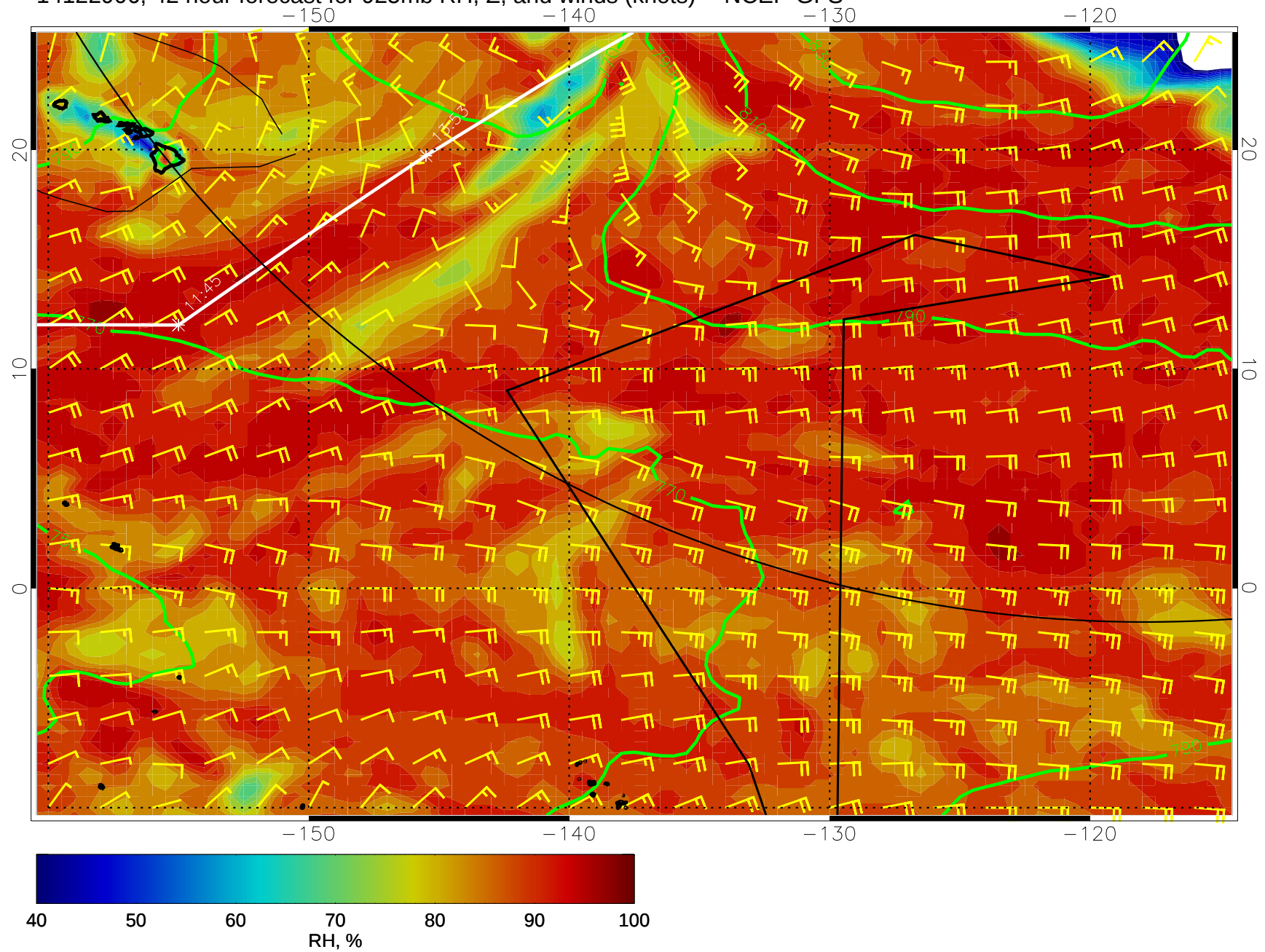
14122906, 42 hour forecast for 925mb RH, Z, and winds (knots) -- NCEP GFS
