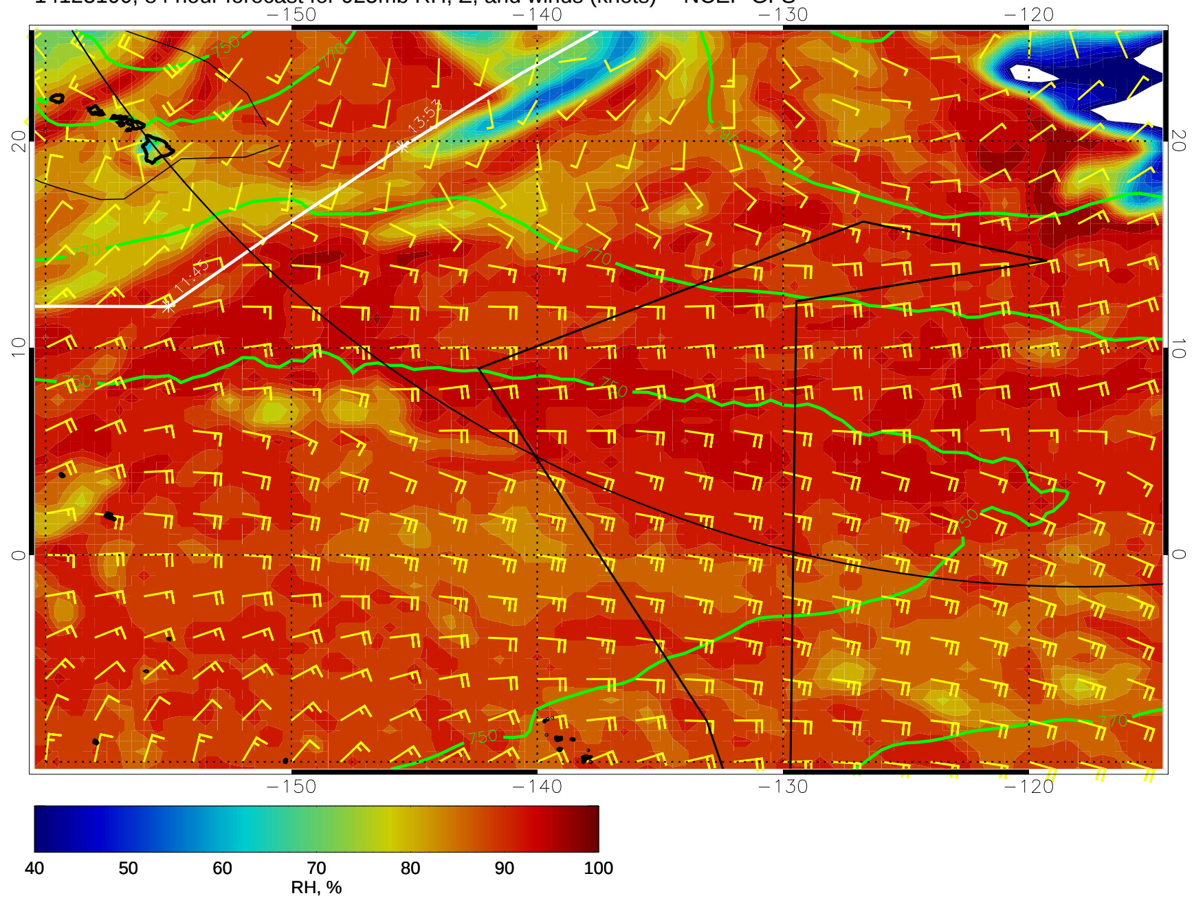
14123100, 84 hour forecast for 925mb RH, Z, and winds (knots) -- NCEP GFS
