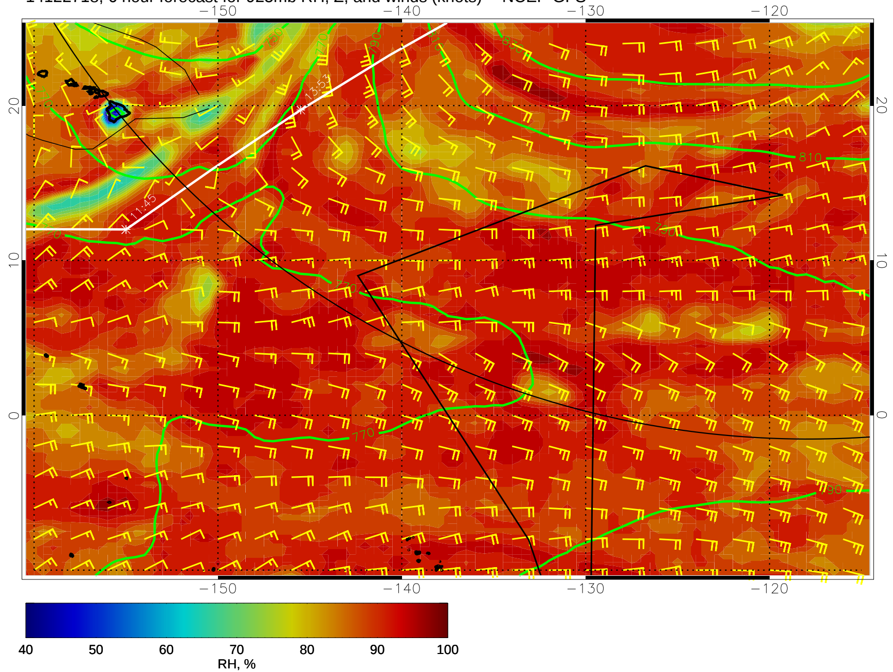
14122718, 6 hour forecast for 925mb RH, Z, and winds (knots) -- NCEP GFS
