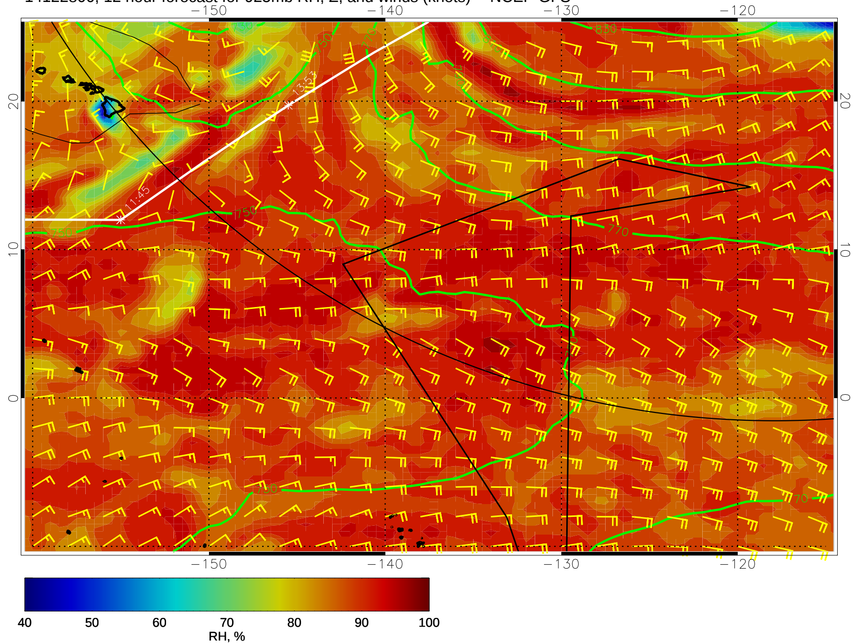
14122800, 12 hour forecast for 925mb RH, Z, and winds (knots) -- NCEP GFS
