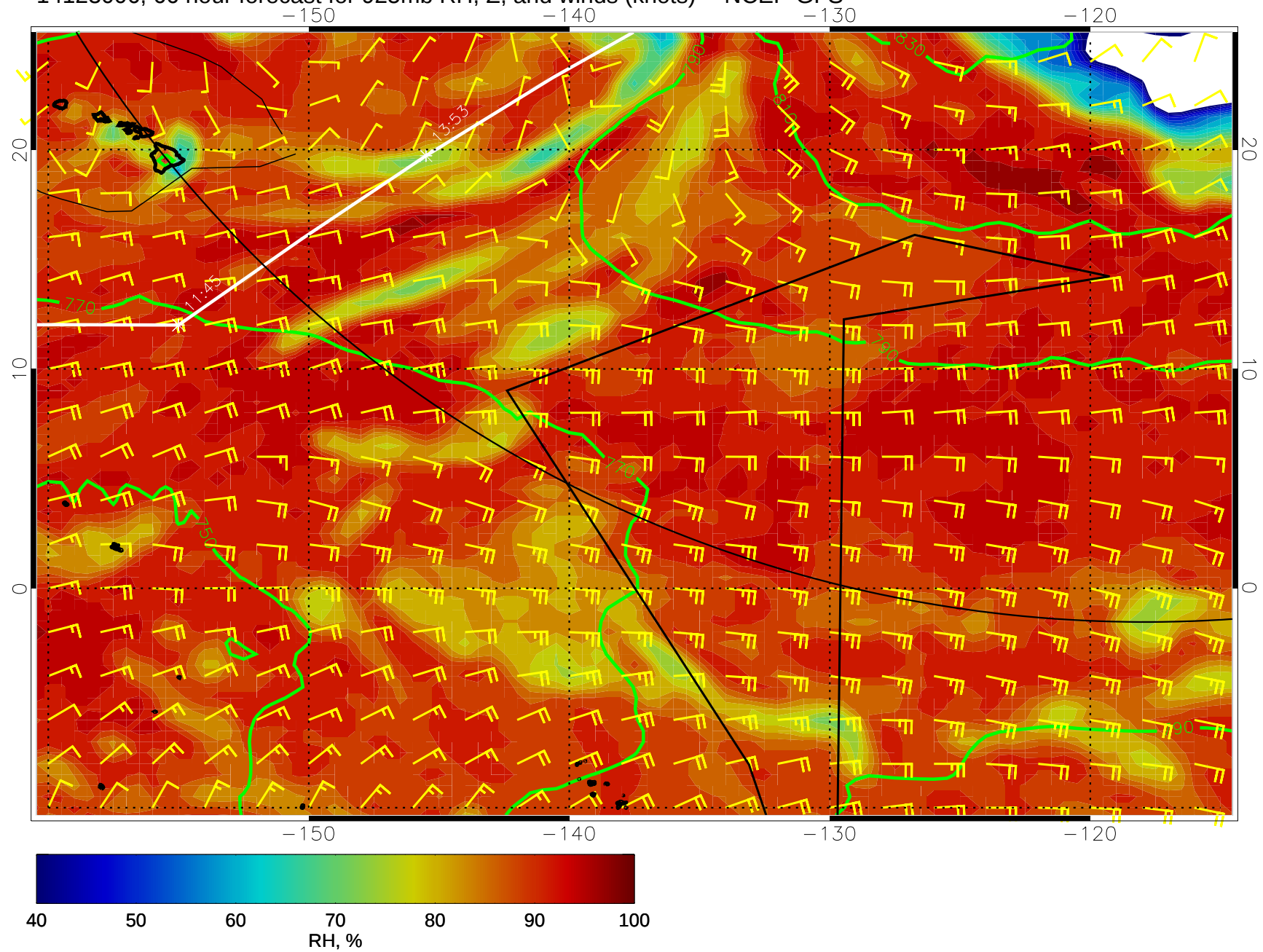
14123006, 66 hour forecast for 925mb RH, Z, and winds (knots) -- NCEP GFS
