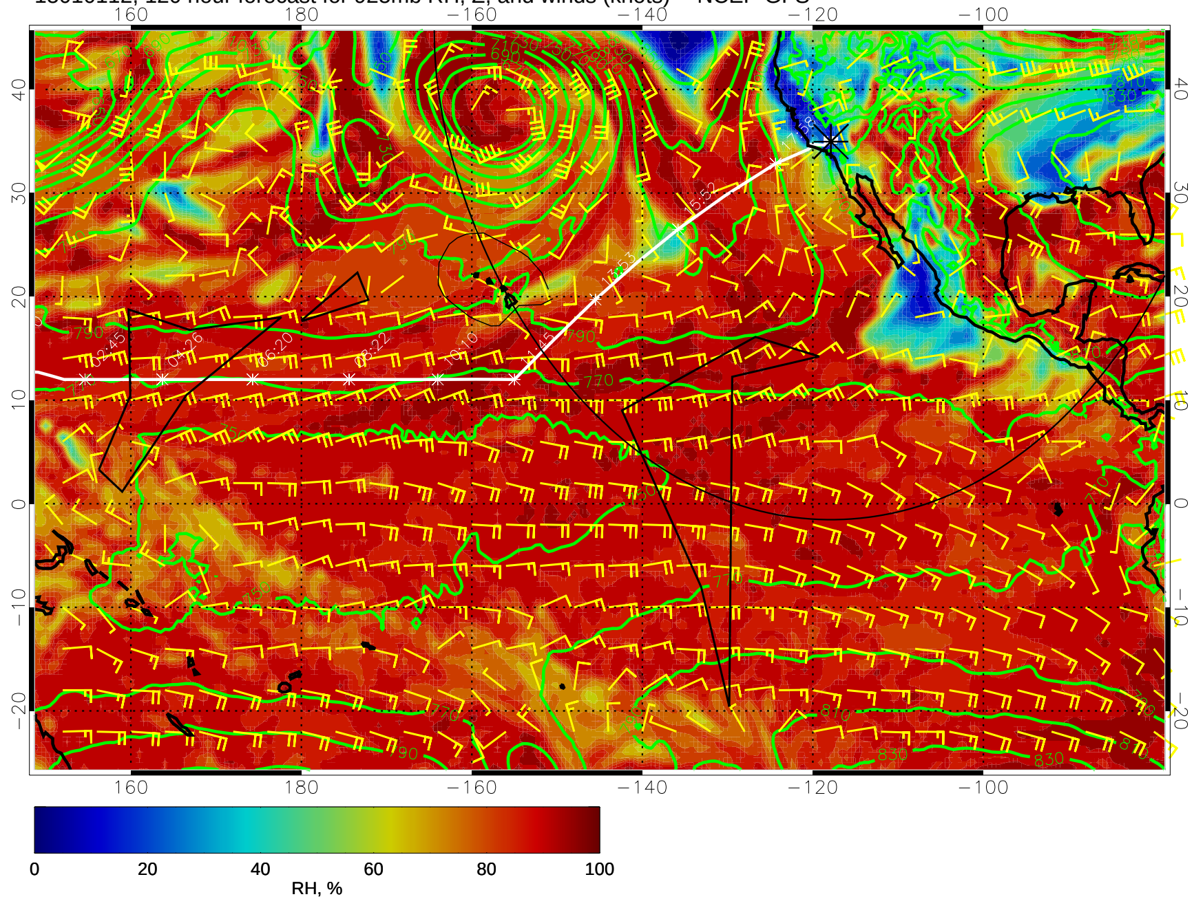
15010112, 120 hour forecast for 925mb RH, Z, and winds (knots) -- NCEP GFS
