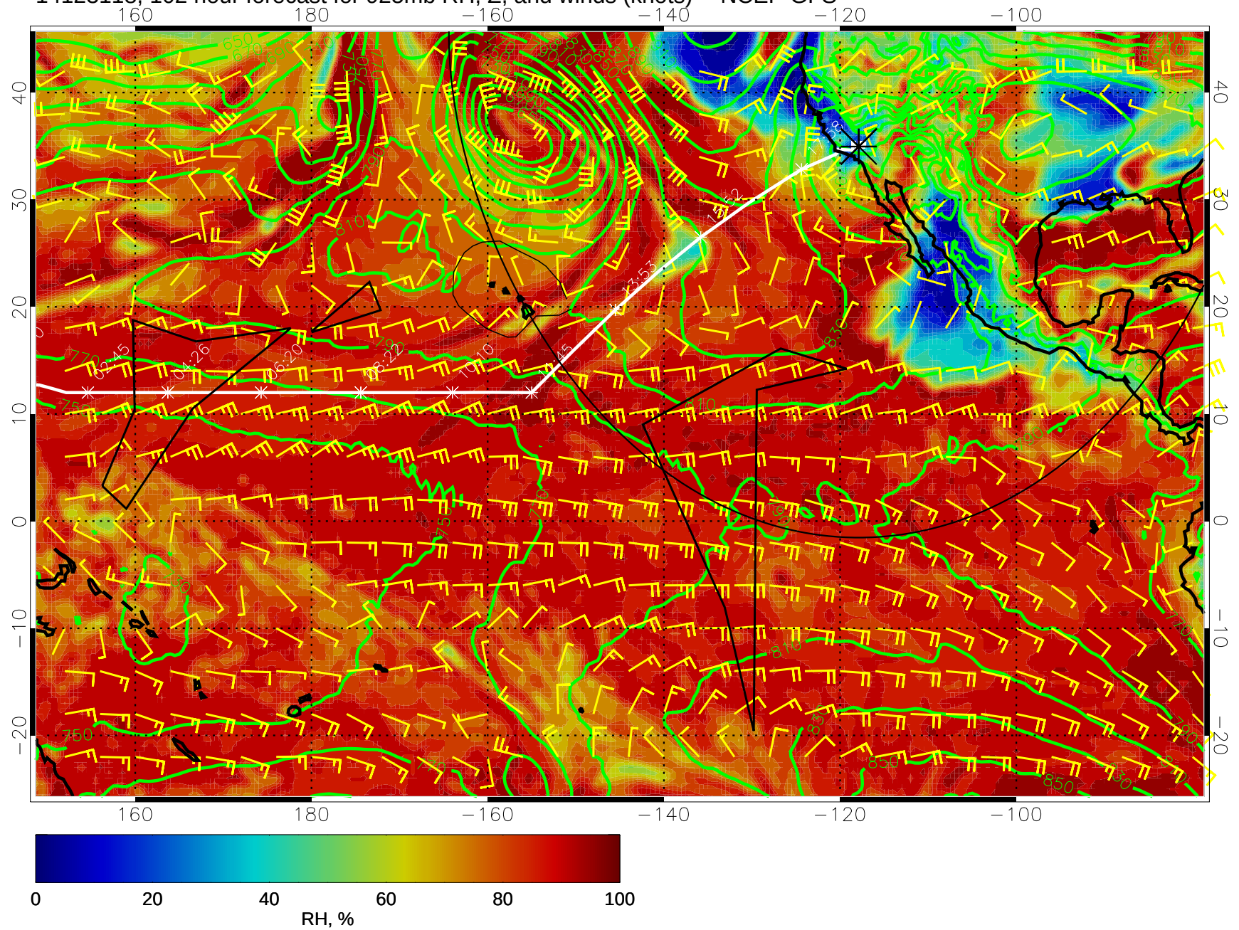
14123118, 102 hour forecast for 925mb RH, Z, and winds (knots) -- NCEP GFS
