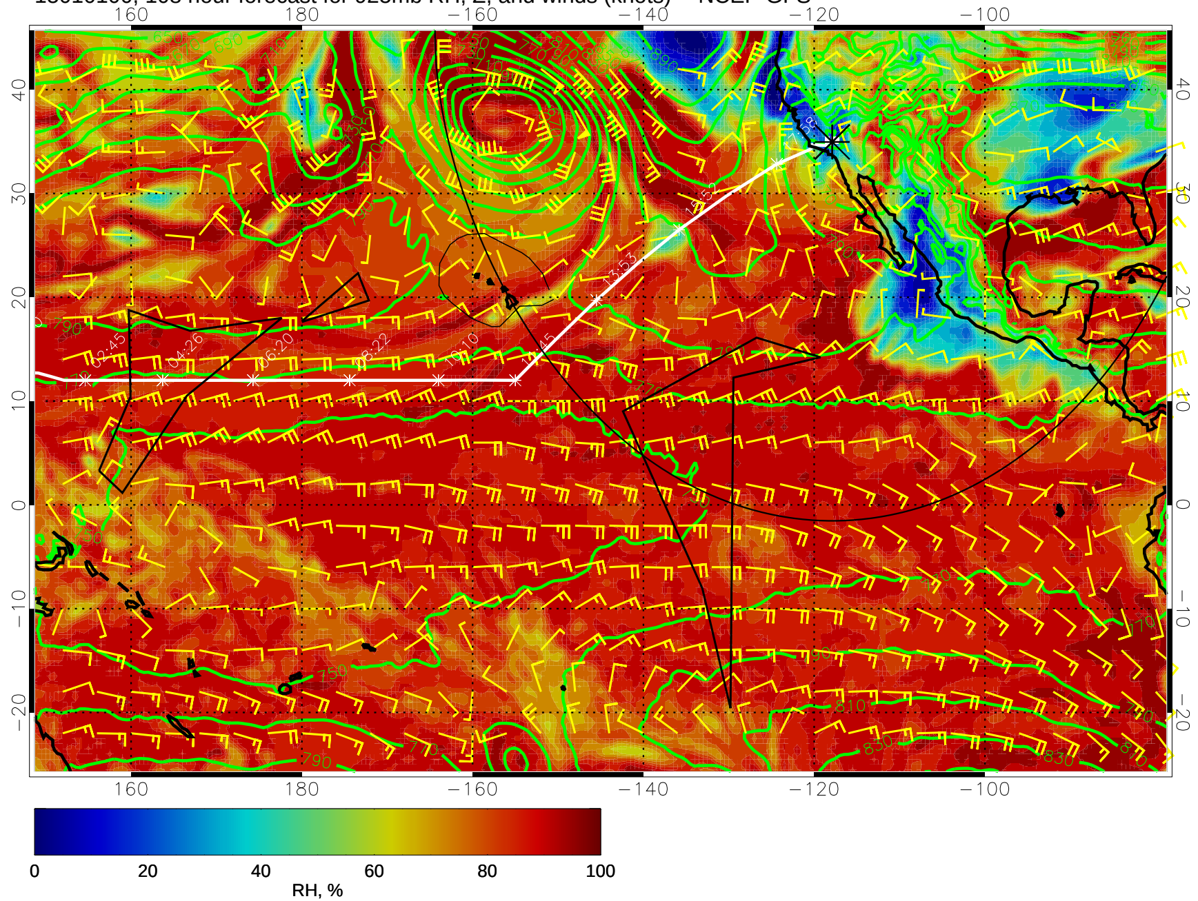
15010100, 108 hour forecast for 925mb RH, Z, and winds (knots) -- NCEP GFS
