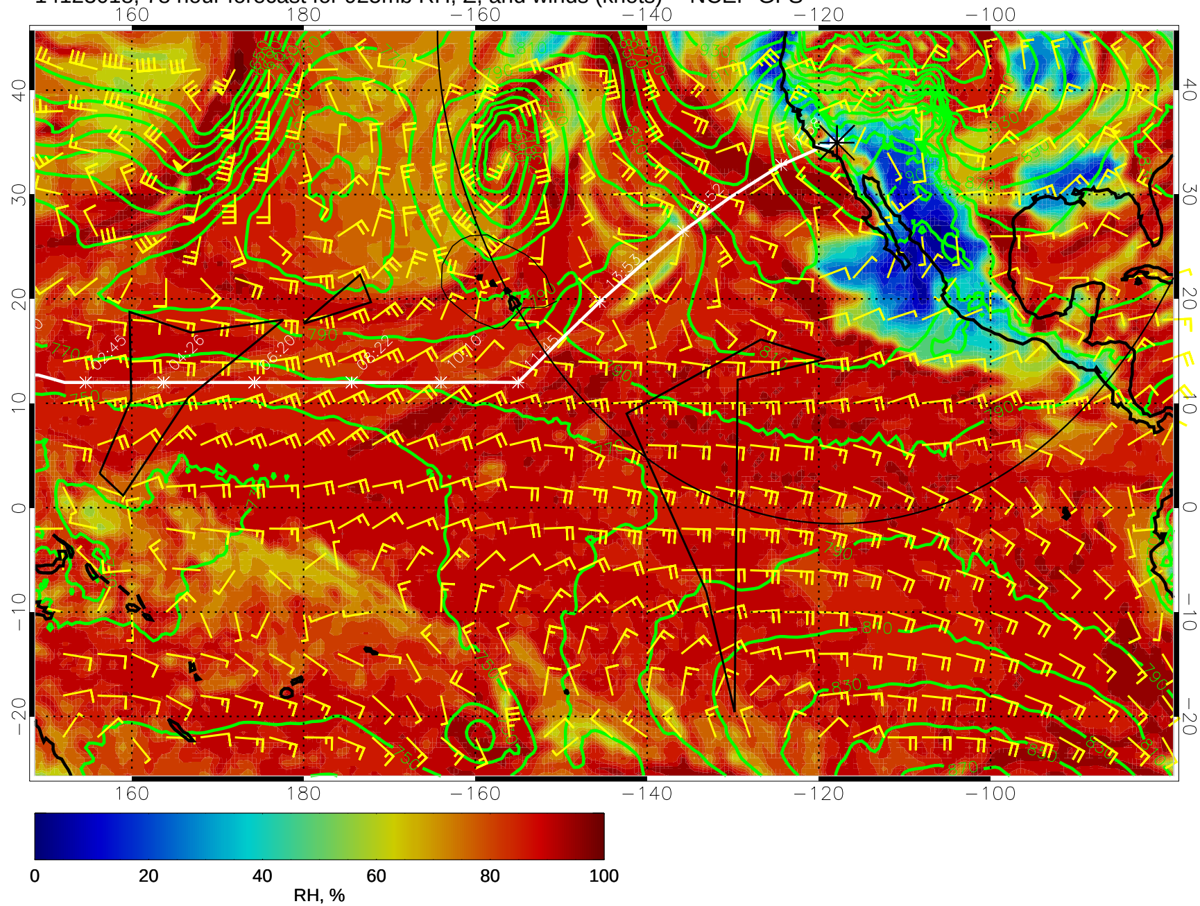
14123018, 78 hour forecast for 925mb RH, Z, and winds (knots) -- NCEP GFS
