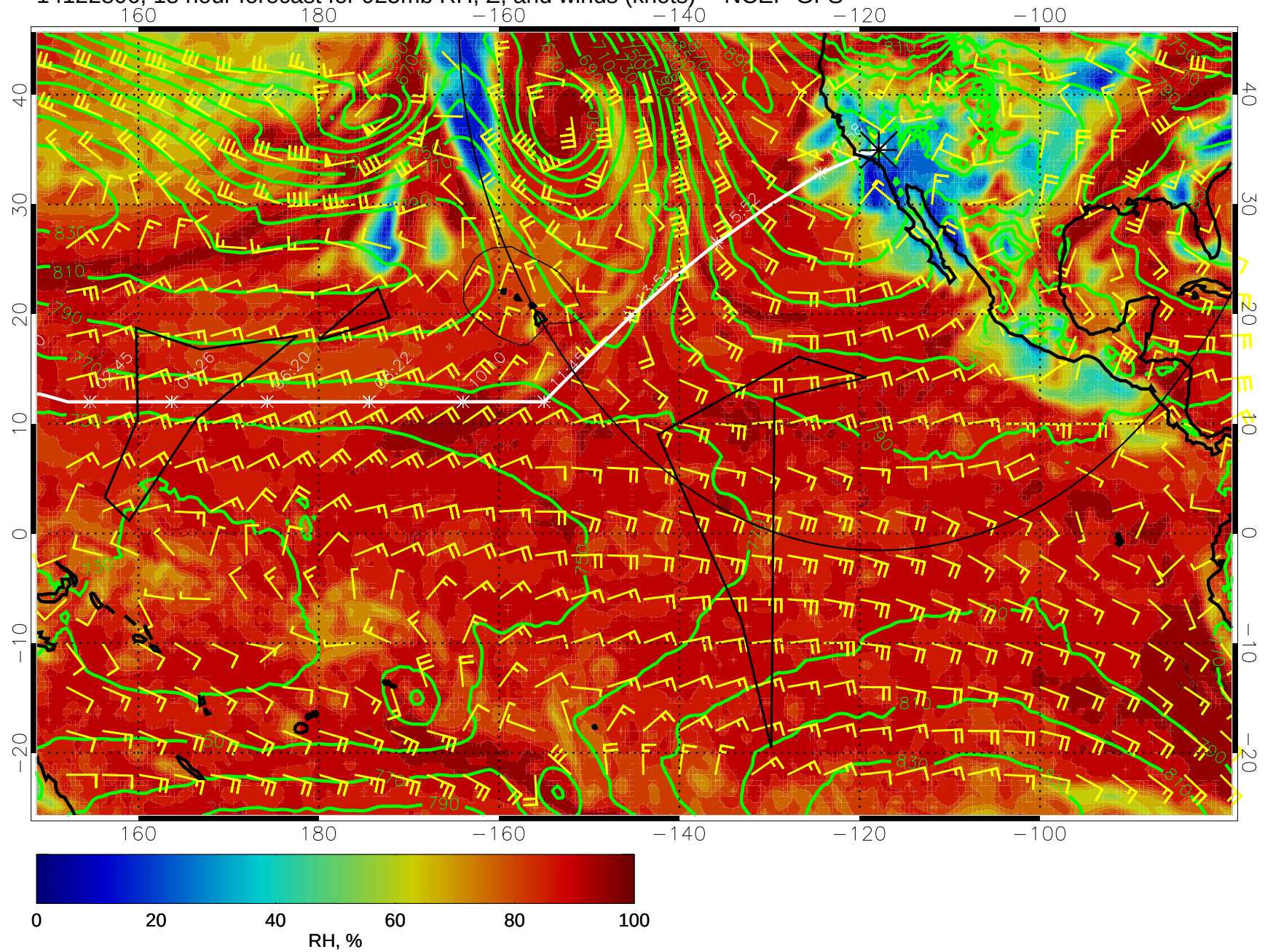
14122806, 18 hour forecast for 925mb RH, Z, and winds (knots) -- NCEP GFS
