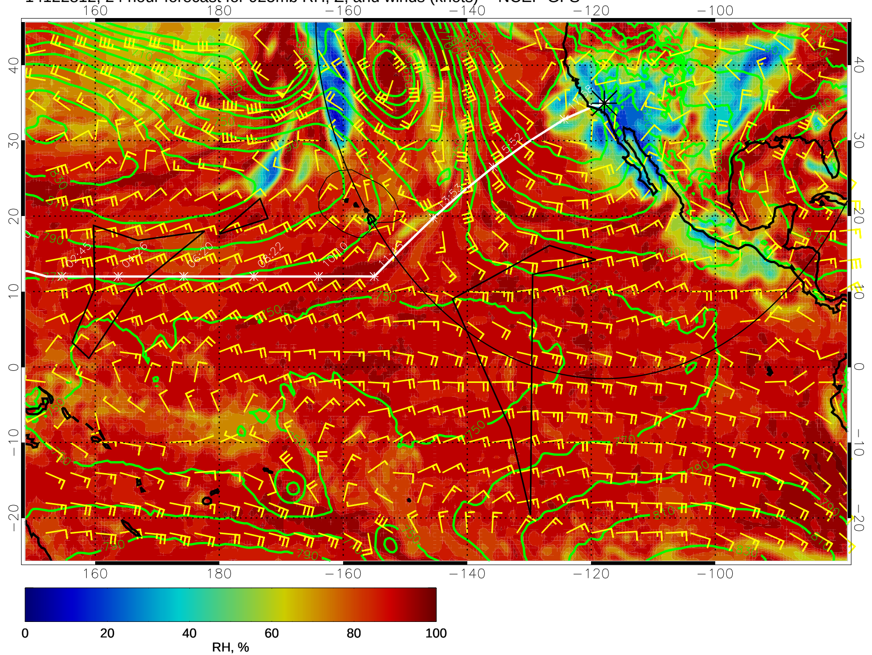
14122812, 24 hour forecast for 925mb RH, Z, and winds (knots) -- NCEP GFS
