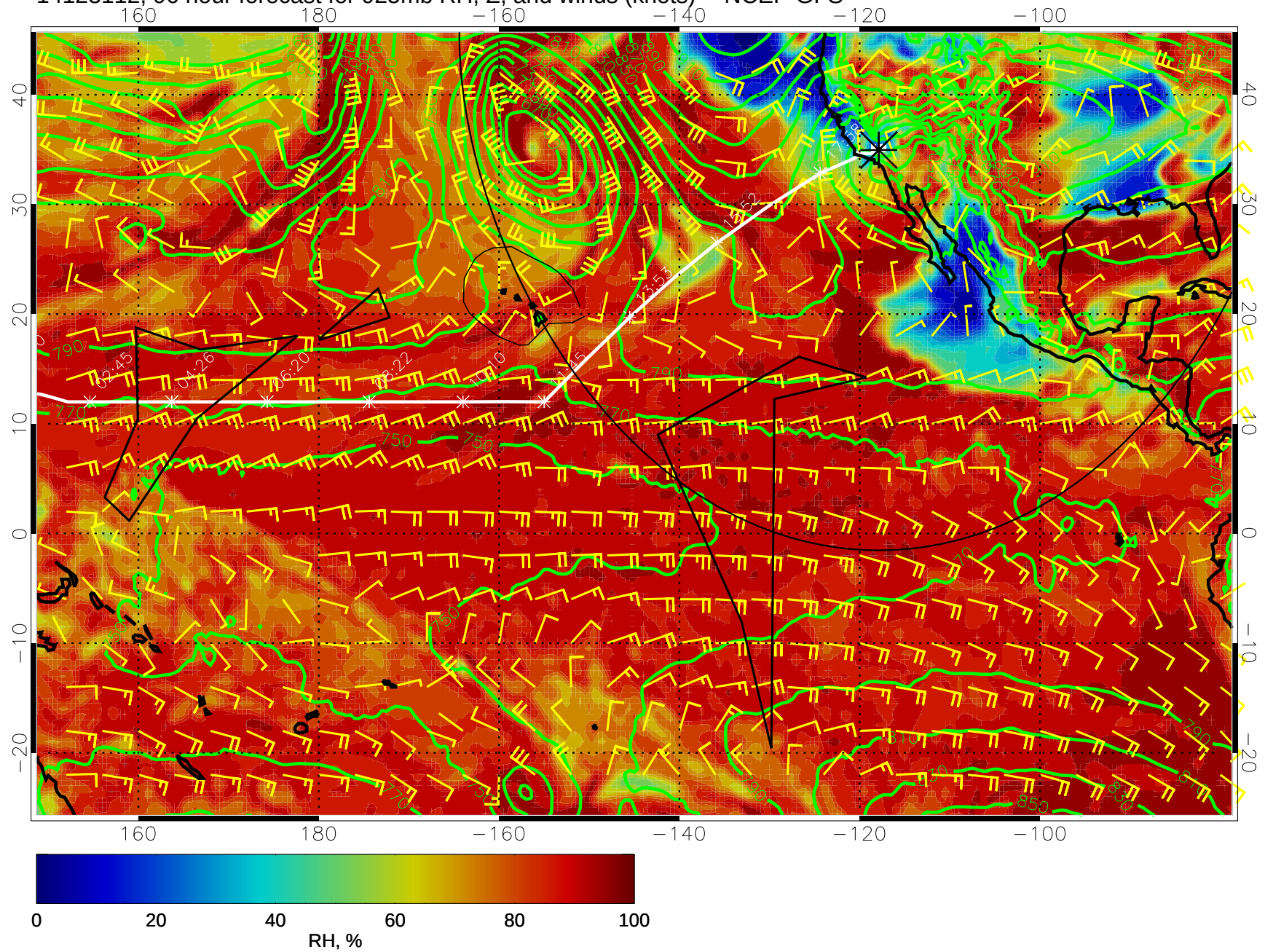
14123112, 96 hour forecast for 925mb RH, Z, and winds (knots) -- NCEP GFS
