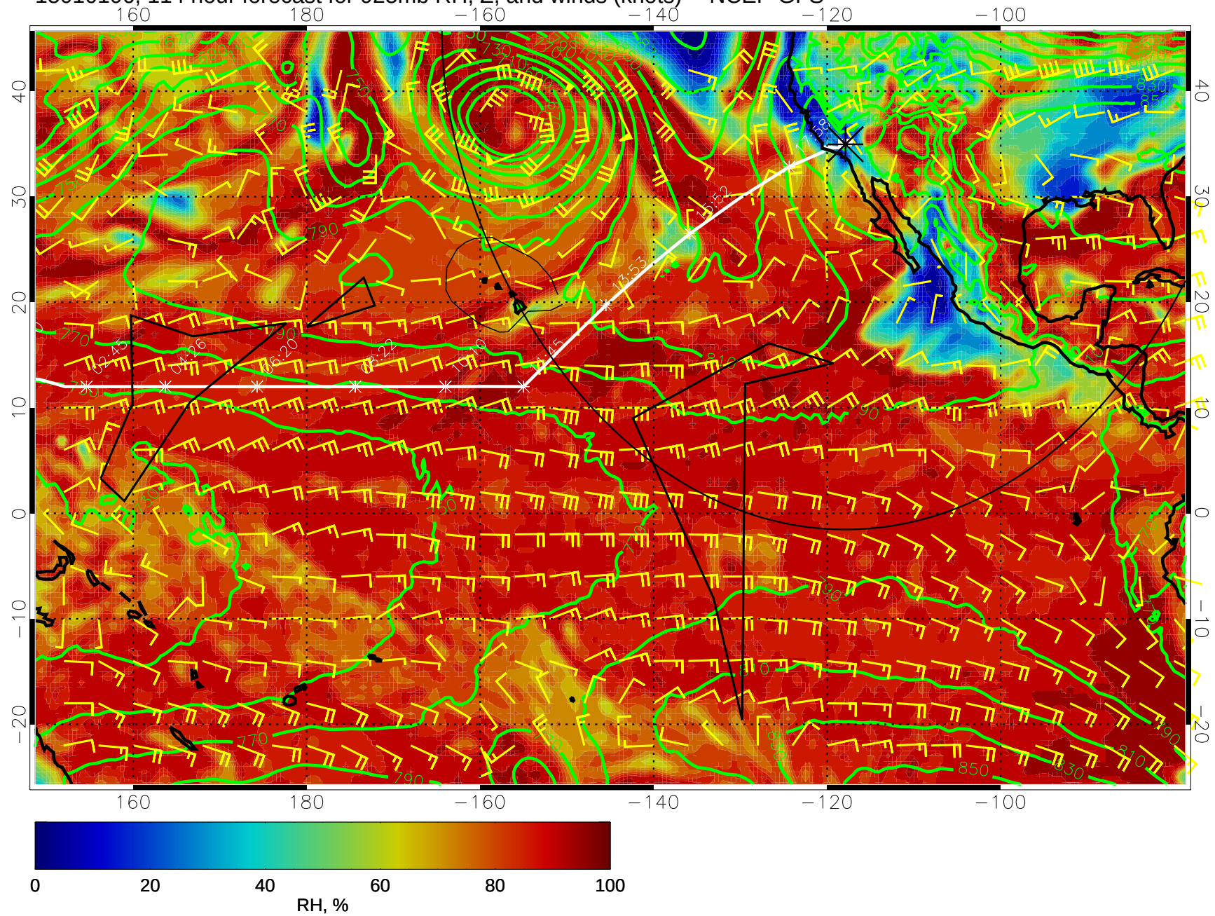
15010106, 114 hour forecast for 925mb RH, Z, and winds (knots) -- NCEP GFS
