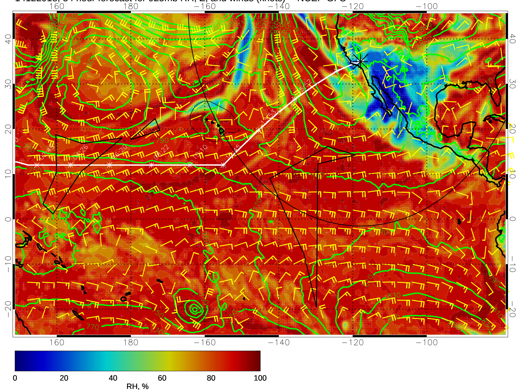
14122918, 54 hour forecast for 925mb RH, Z, and winds (knots) -- NCEP GFS
