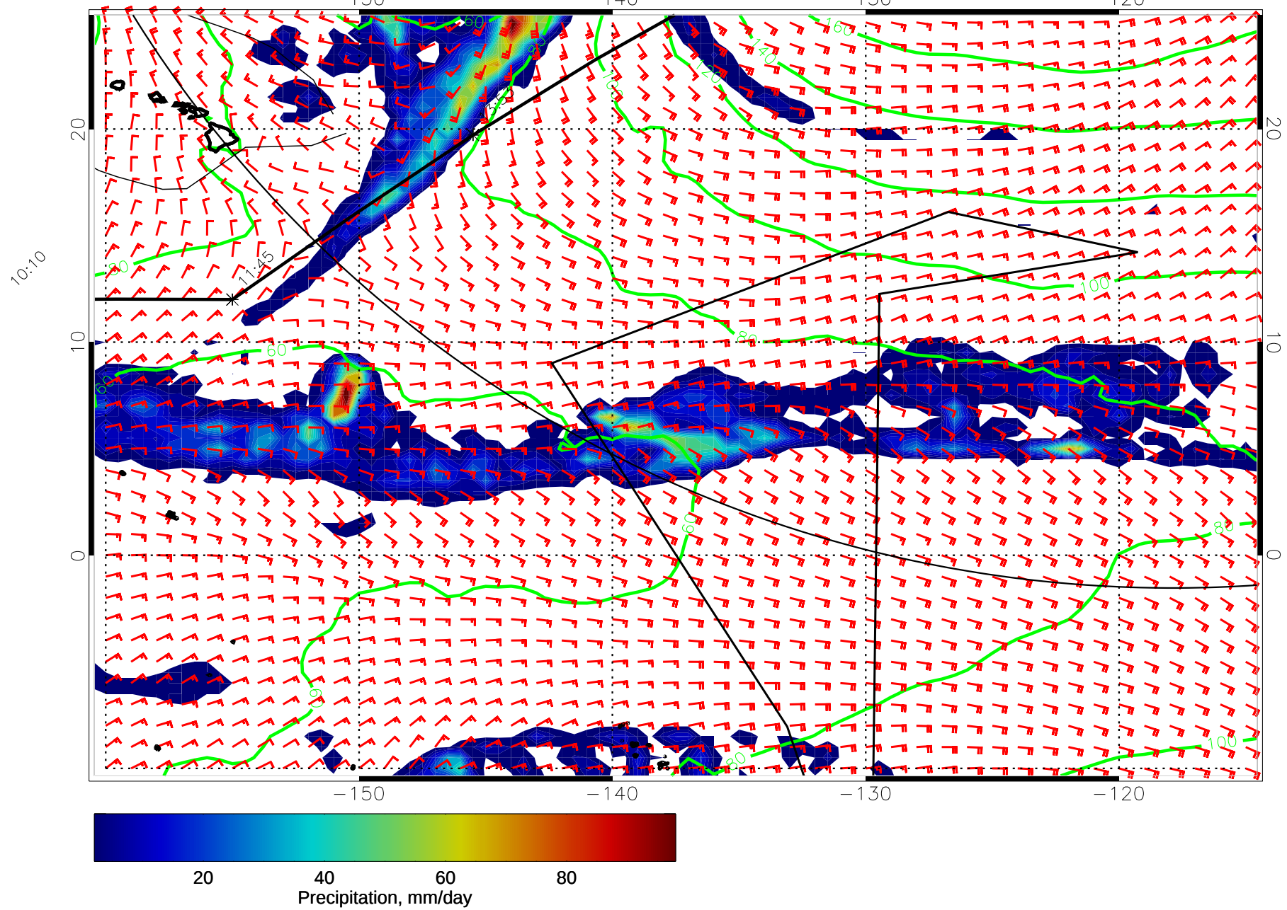
14122800, 12 hour forecast for precip, 1000mb Z, and winds (knots) -- NCEP GFS
