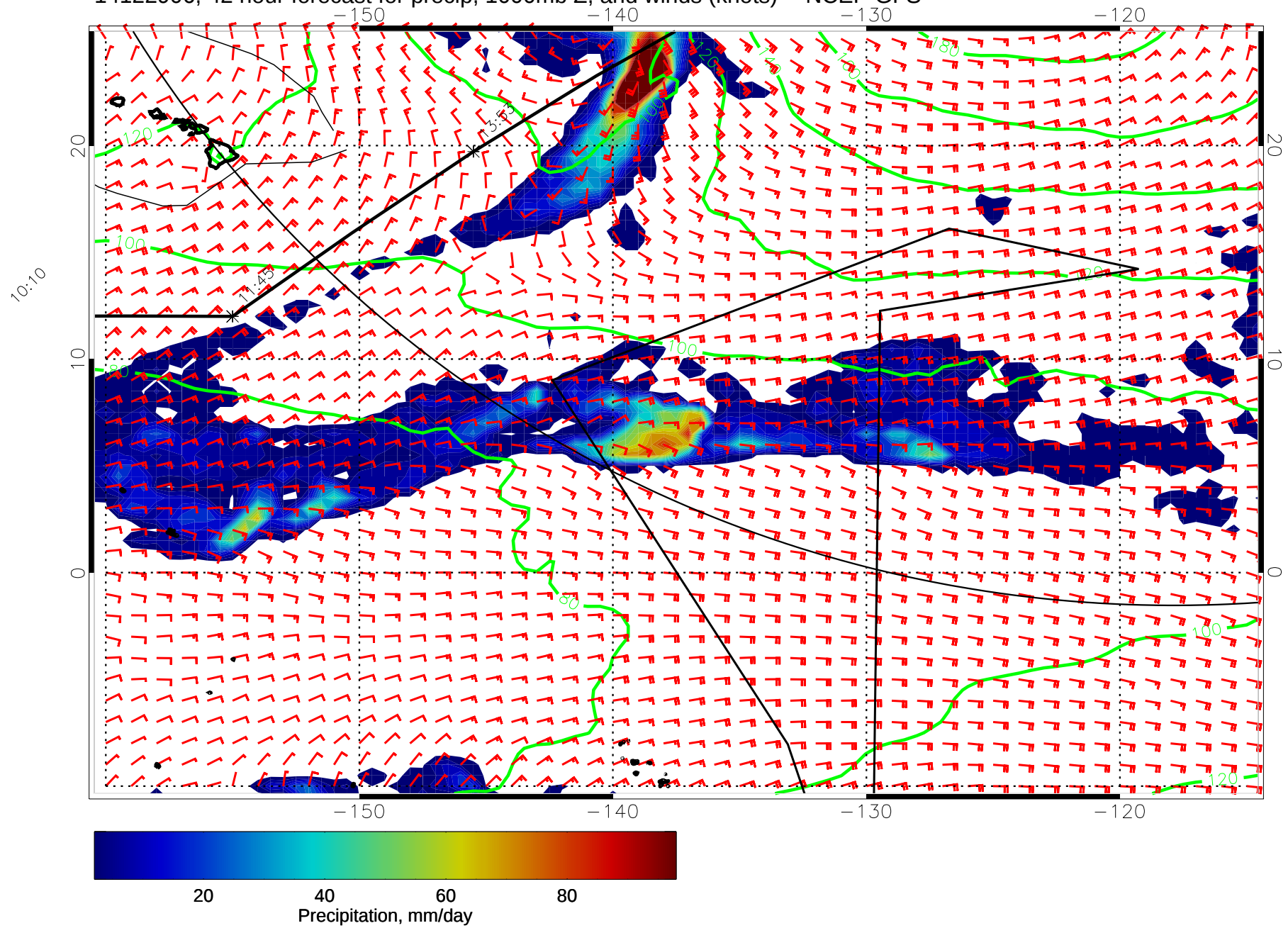
14122906, 42 hour forecast for precip, 1000mb Z, and winds (knots) -- NCEP GFS
