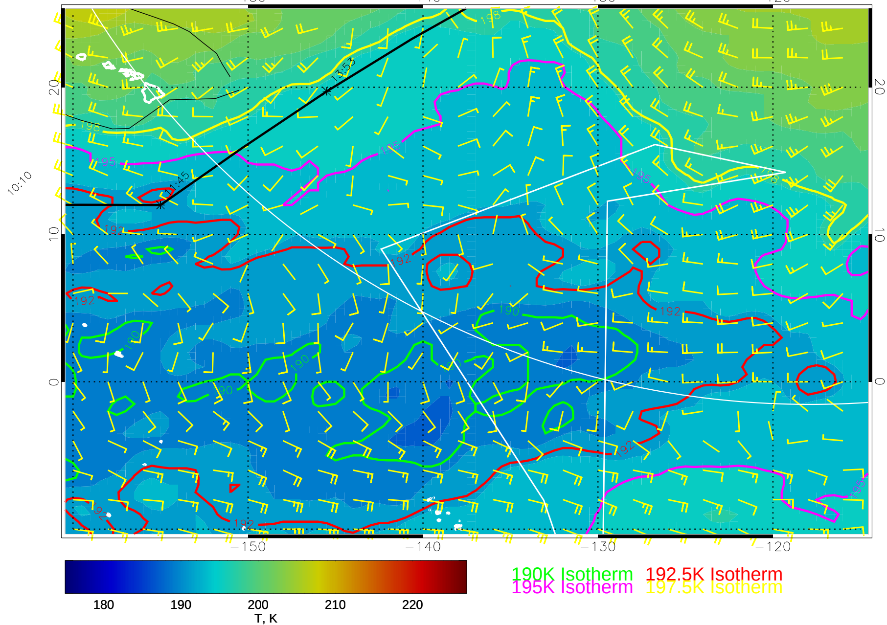
14123118, 102 hour forecast for 70mb T and winds (knots) -- NCEP GFS
