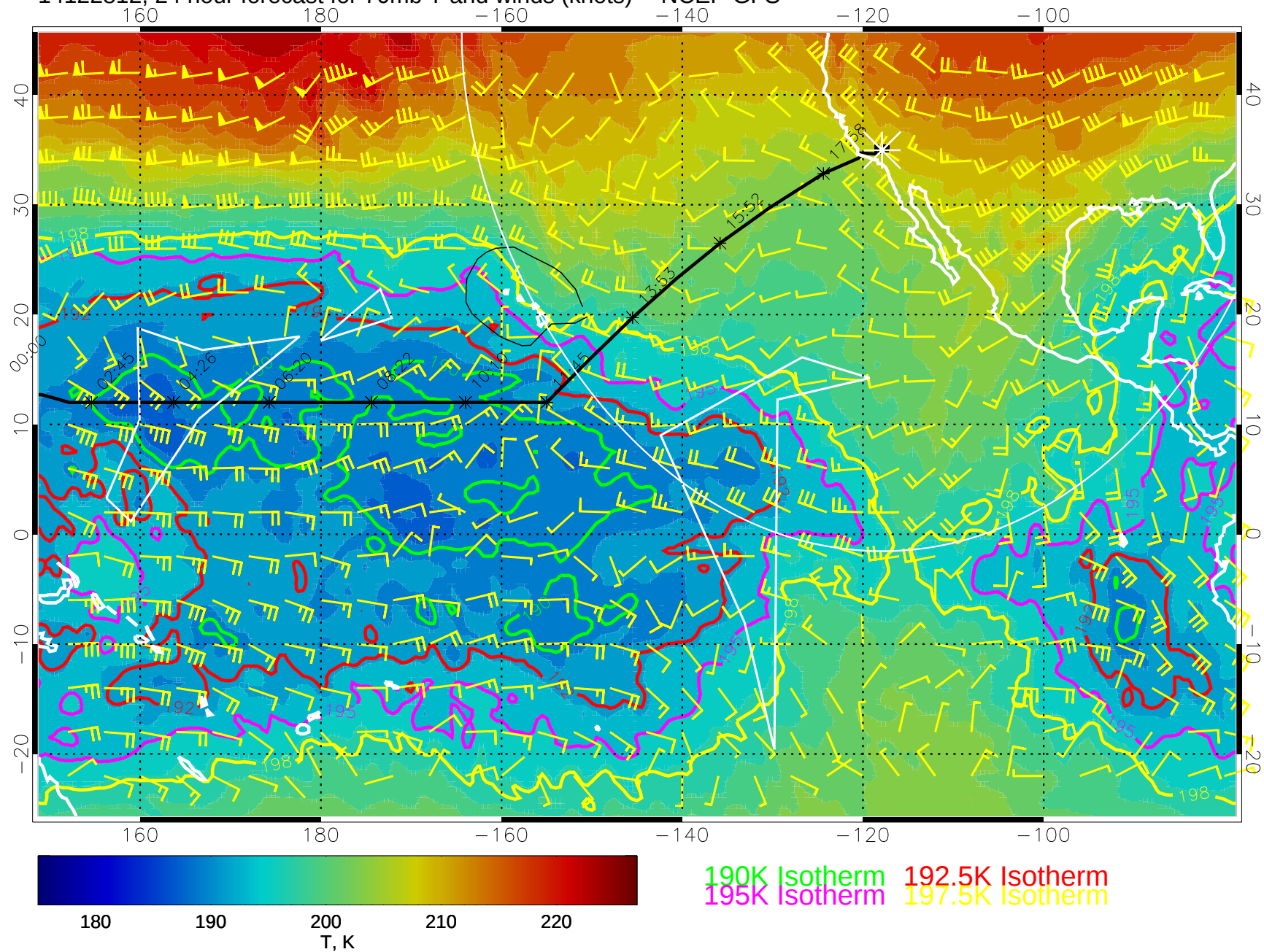
14122812, 24 hour forecast for 70mb T and winds (knots) -- NCEP GFS
