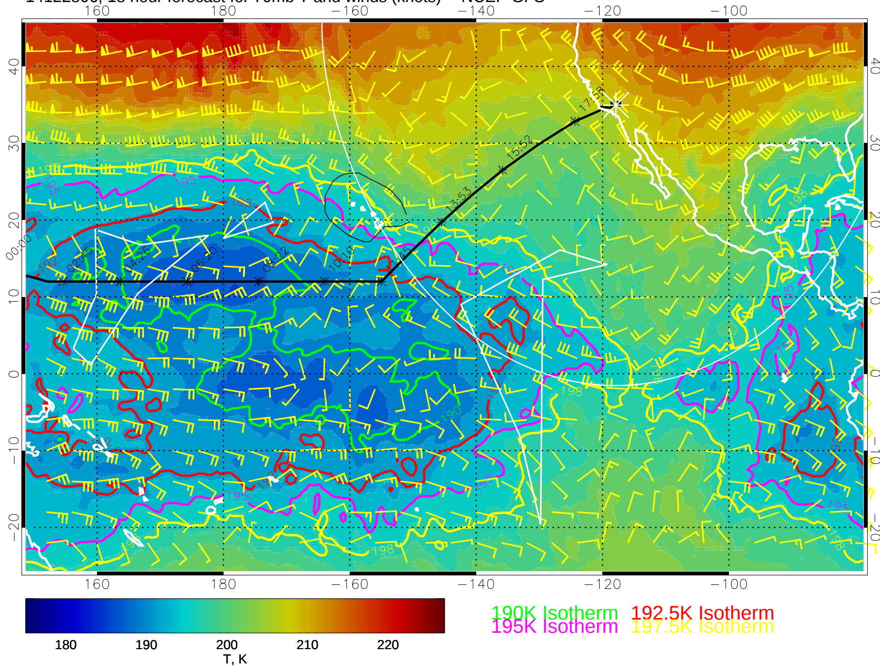
14122806, 18 hour forecast for 70mb T and winds (knots) -- NCEP GFS
