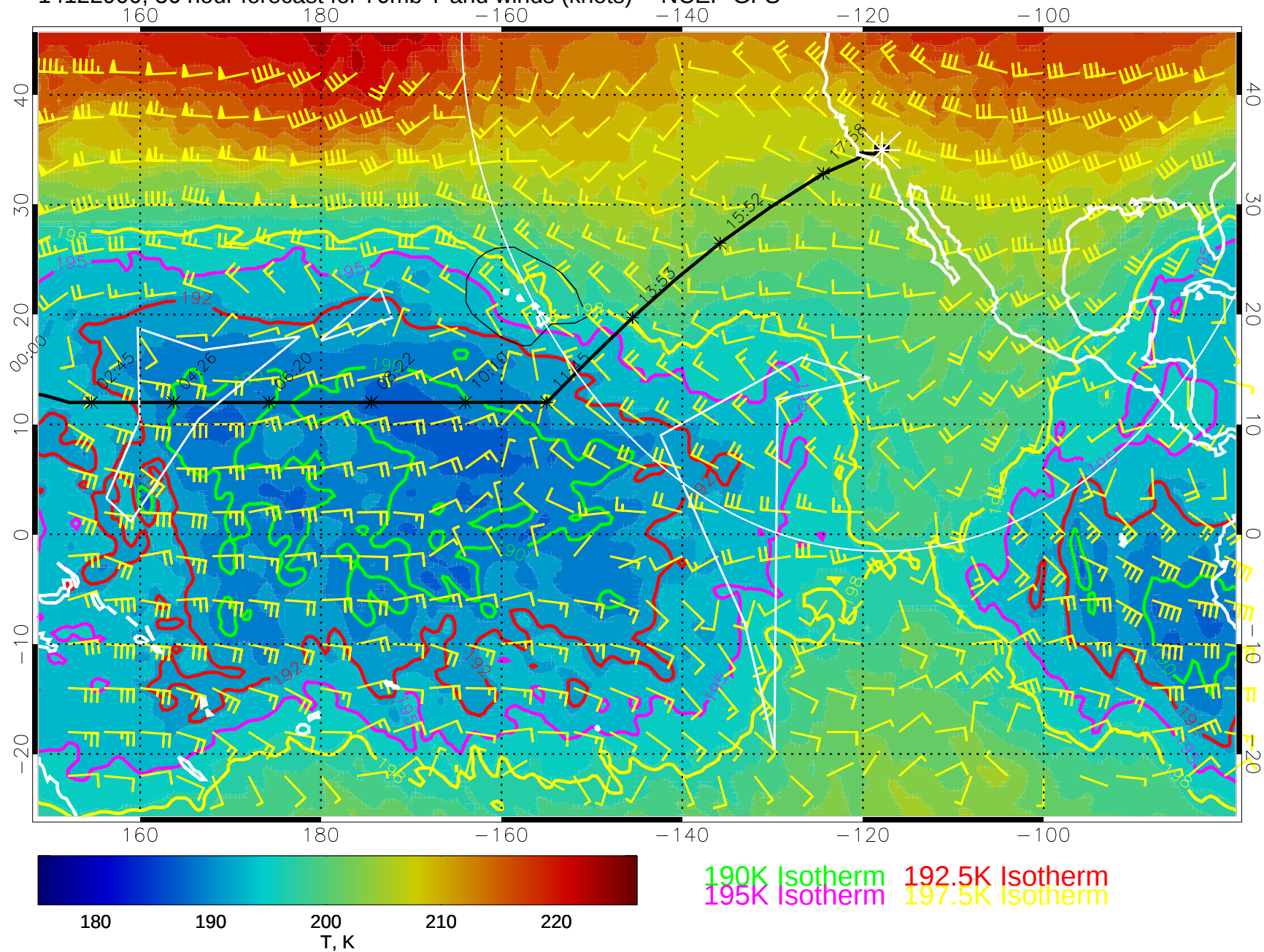
14122900, 36 hour forecast for 70mb T and winds (knots) -- NCEP GFS
