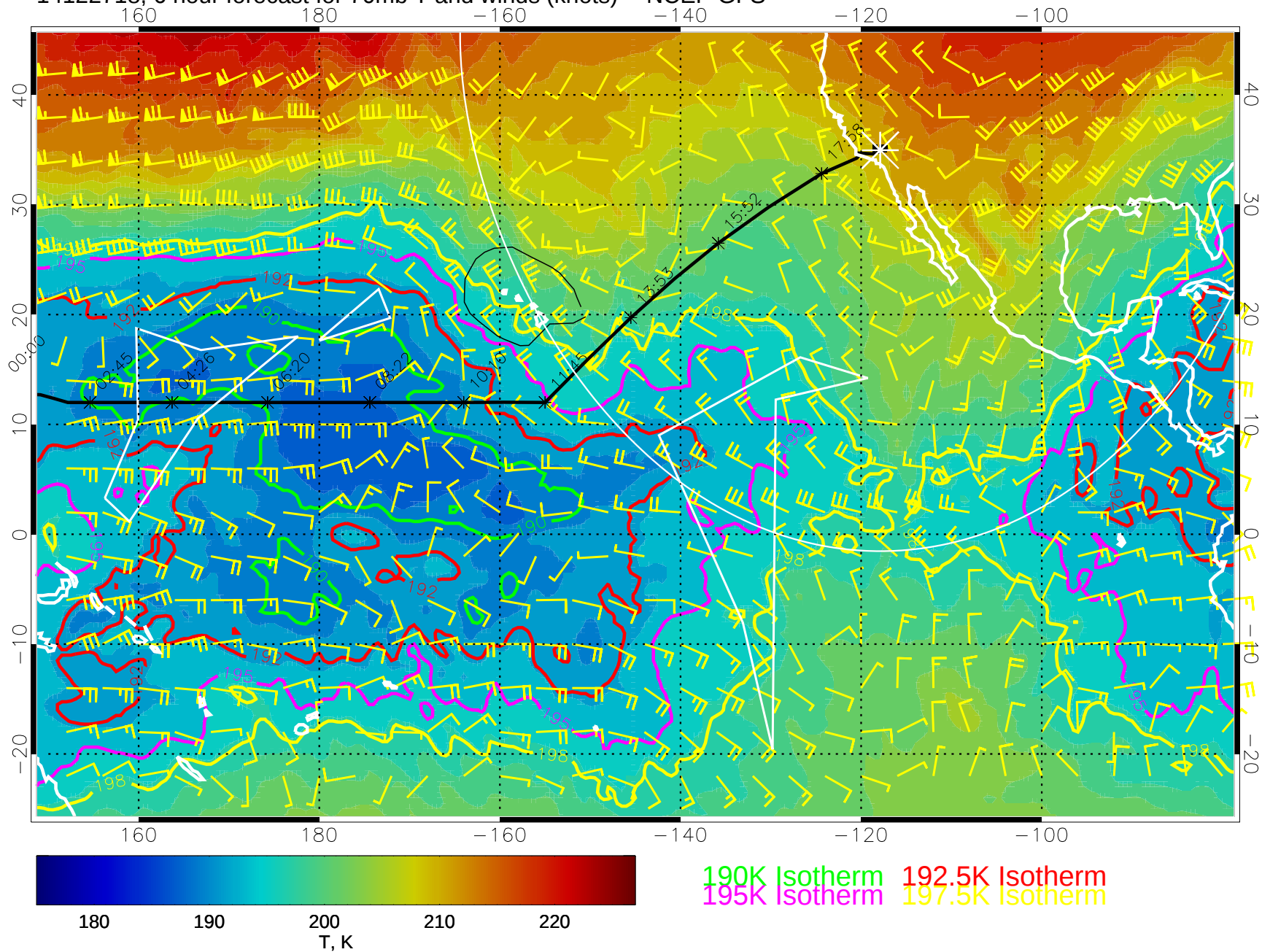
14122718, 6 hour forecast for 70mb T and winds (knots) -- NCEP GFS
