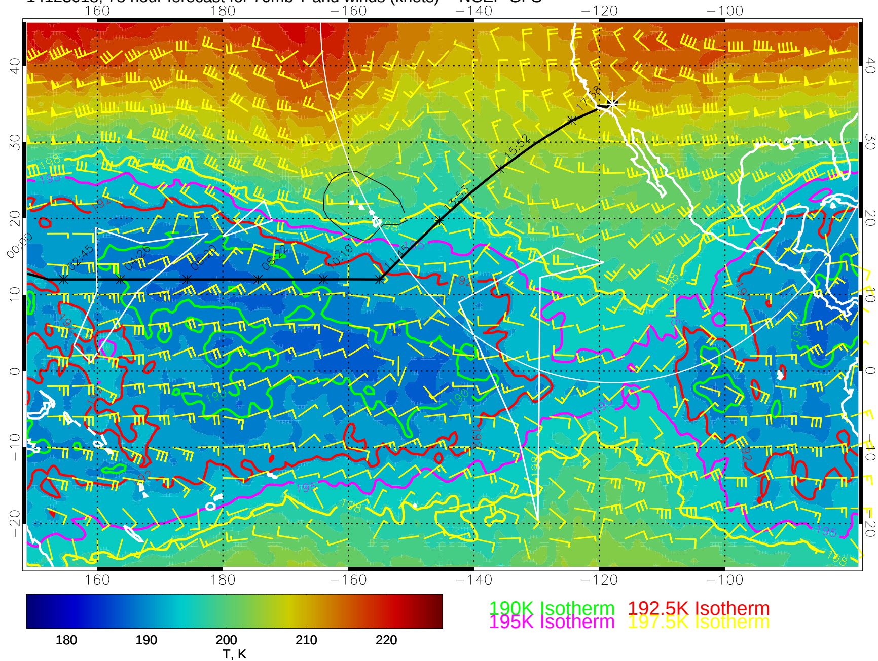
14123018, 78 hour forecast for 70mb T and winds (knots) -- NCEP GFS
