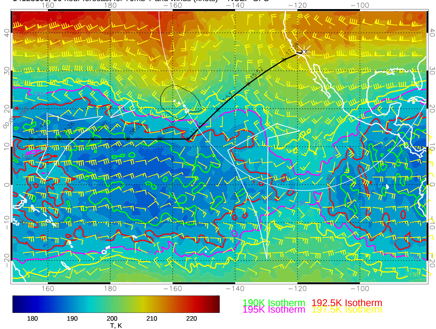
14123106, 90 hour forecast for 70mb T and winds (knots) -- NCEP GFS
