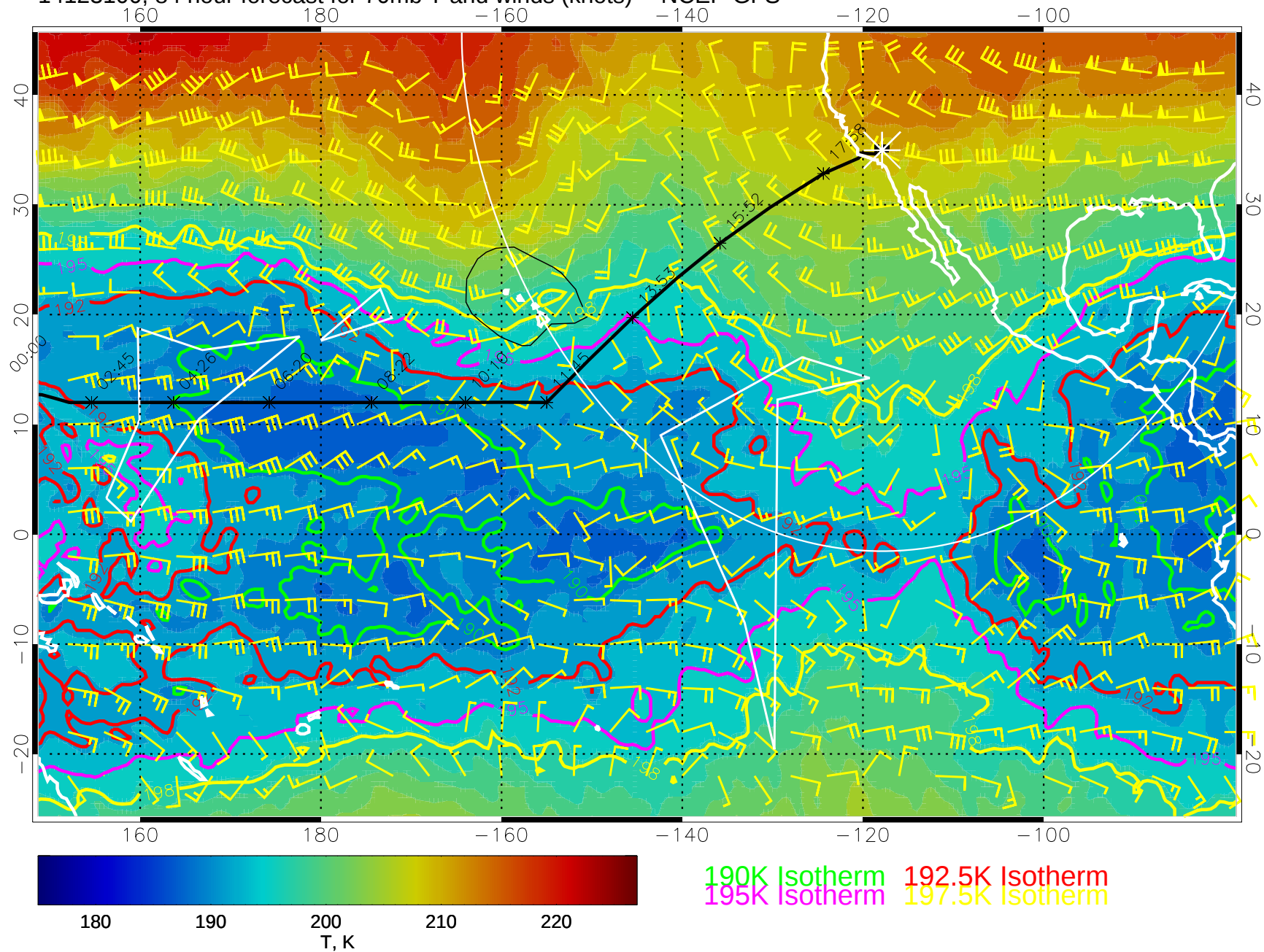
14123100, 84 hour forecast for 70mb T and winds (knots) -- NCEP GFS
