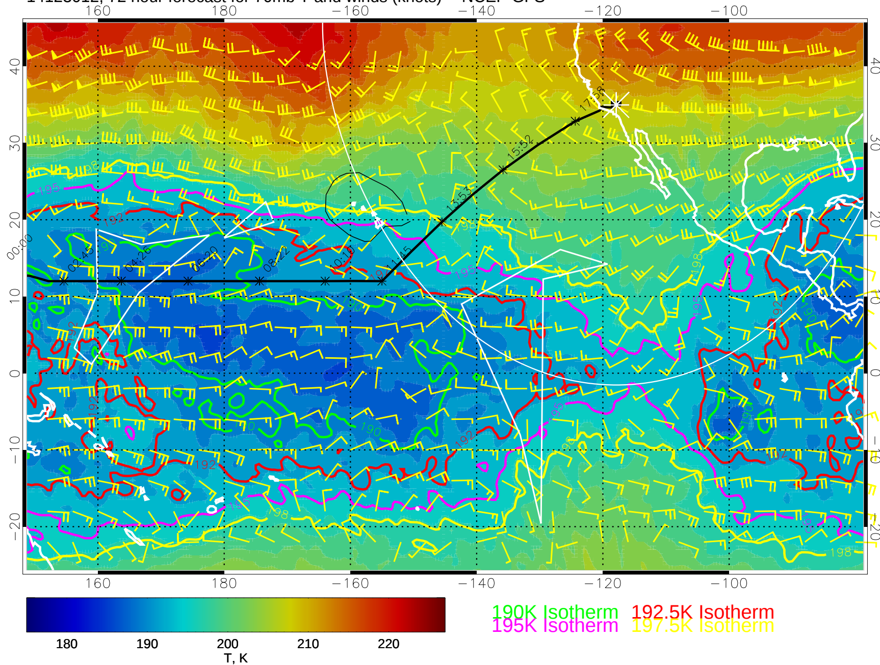
14123012, 72 hour forecast for 70mb T and winds (knots) -- NCEP GFS
