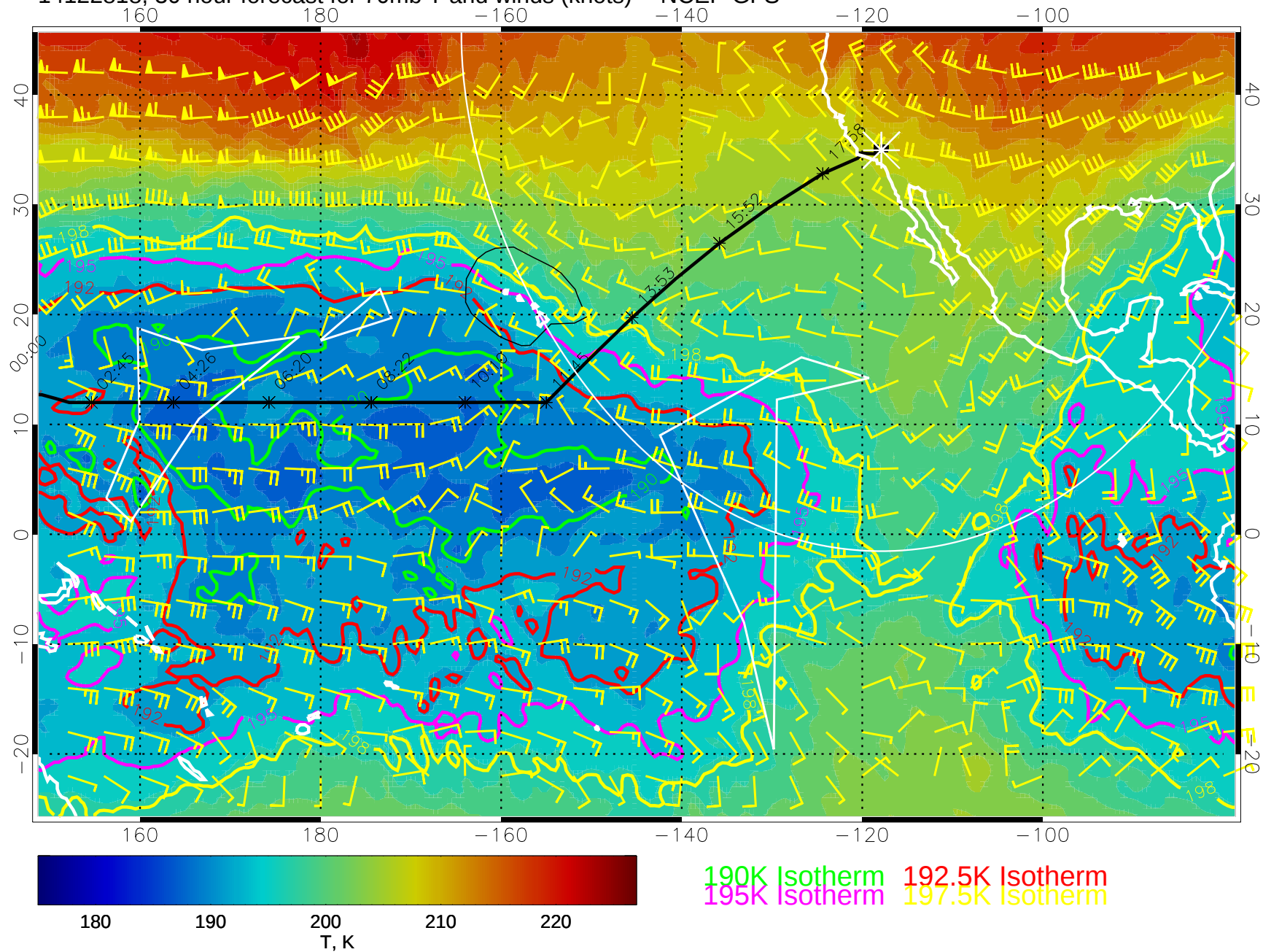
14122818, 30 hour forecast for 70mb T and winds (knots) -- NCEP GFS
