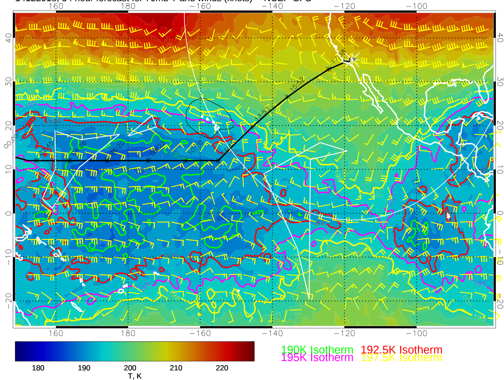
14122918, 54 hour forecast for 70mb T and winds (knots) -- NCEP GFS
