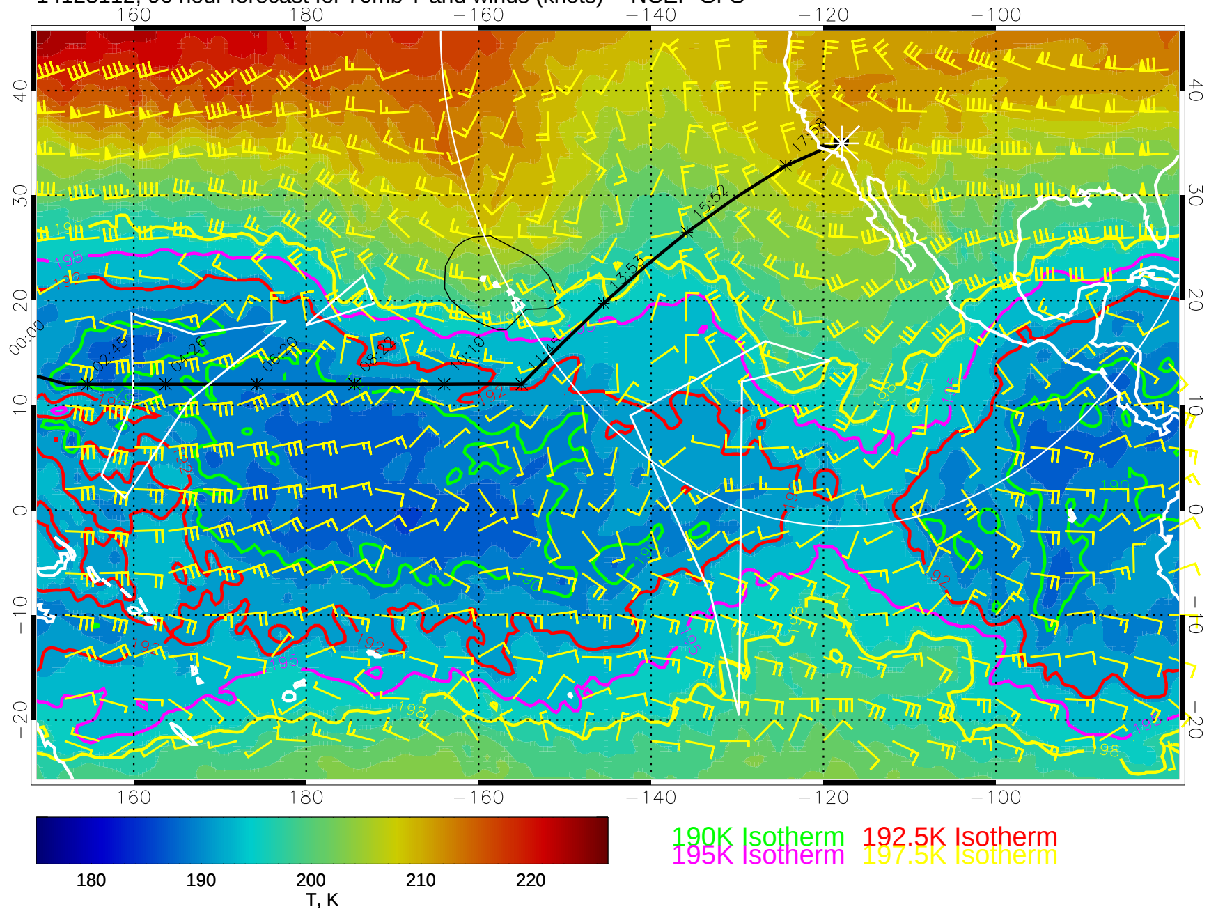
14123112, 96 hour forecast for 70mb T and winds (knots) -- NCEP GFS
