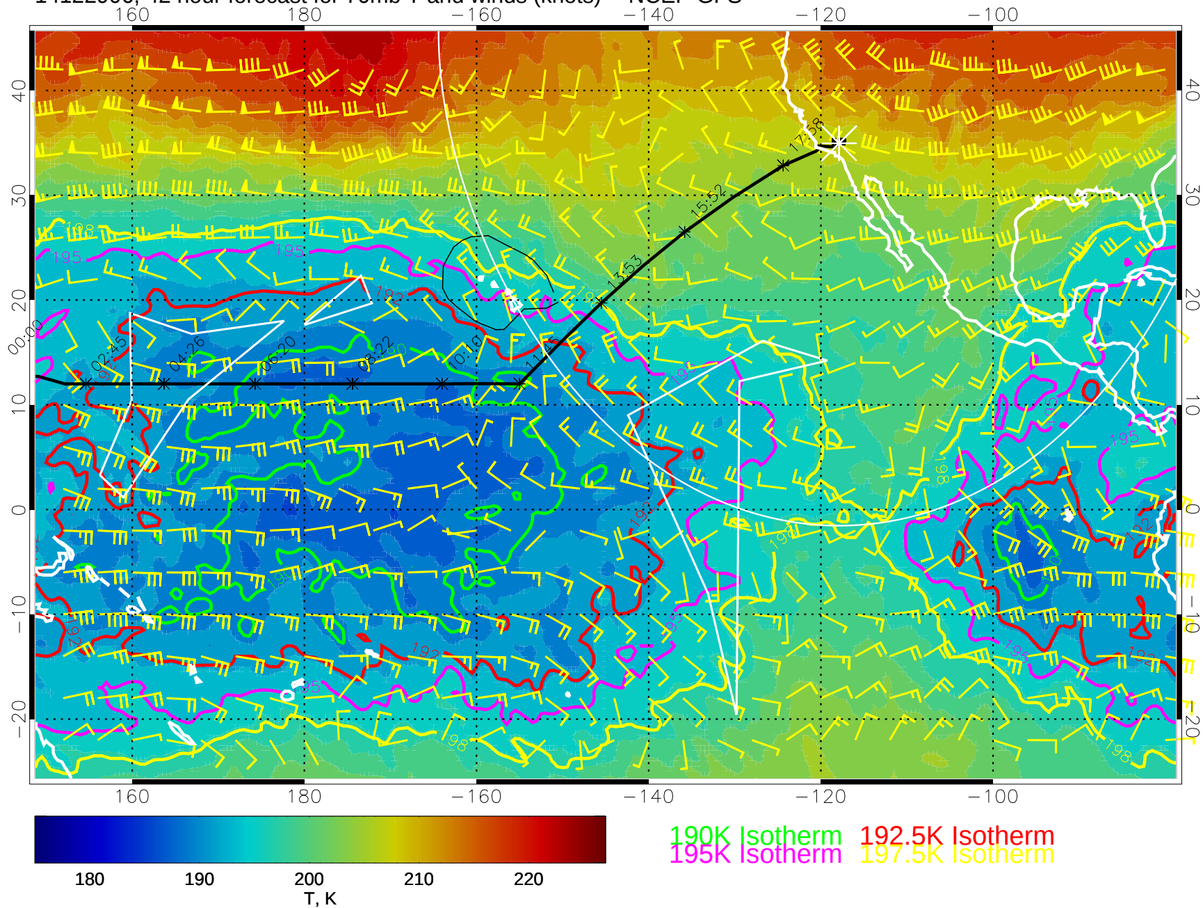
14122906, 42 hour forecast for 70mb T and winds (knots) -- NCEP GFS
