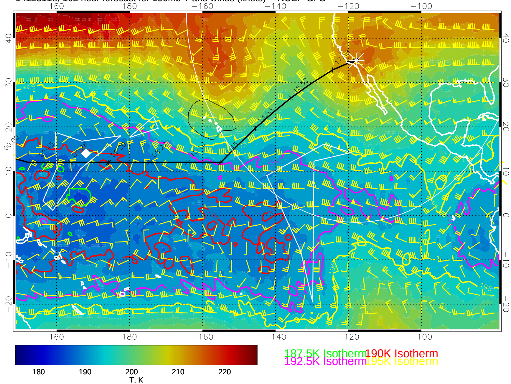
14123118, 102 hour forecast for 100mb T and winds (knots) -- NCEP GFS
