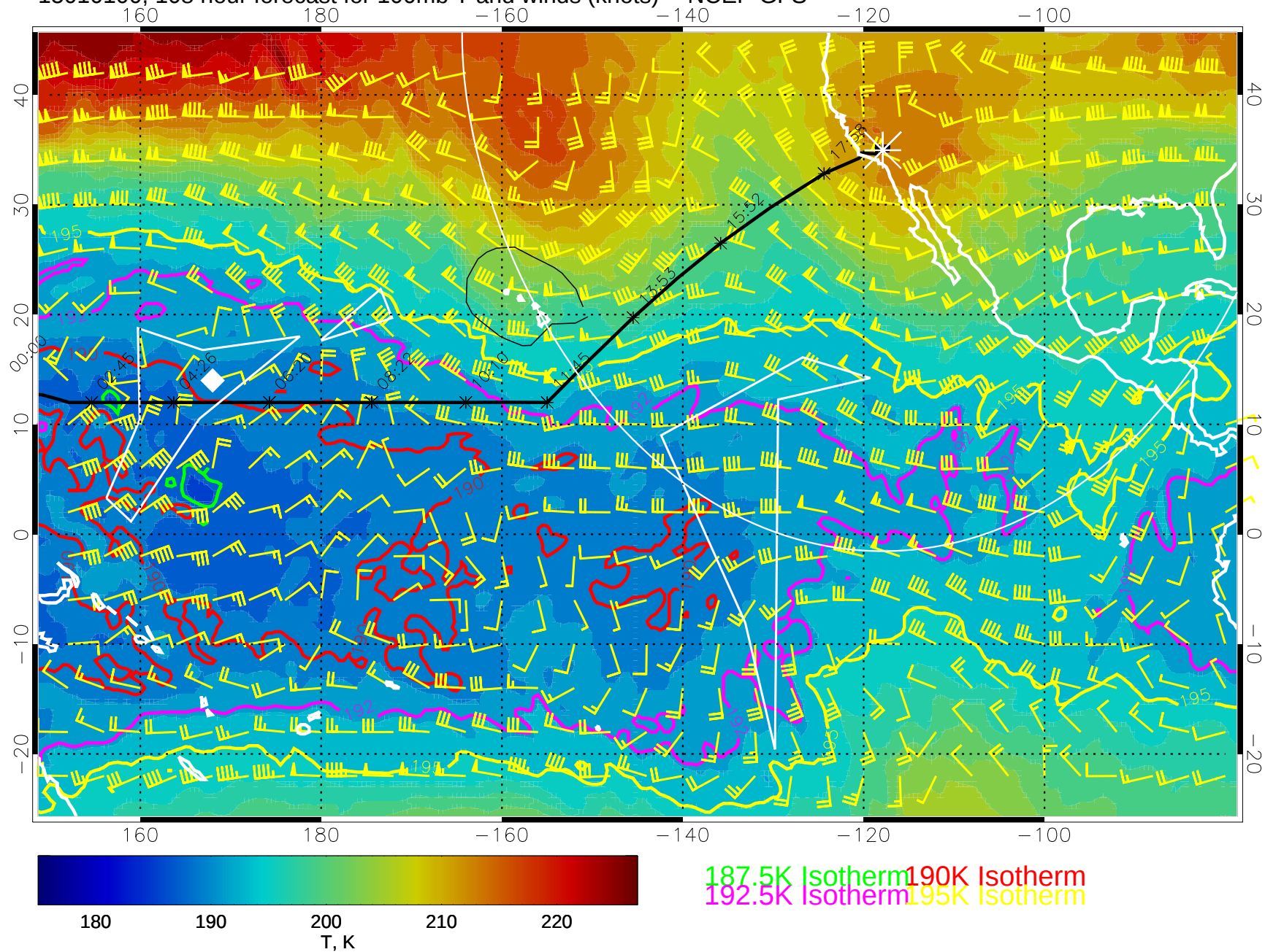
15010100, 108 hour forecast for 100mb T and winds (knots) -- NCEP GFS
