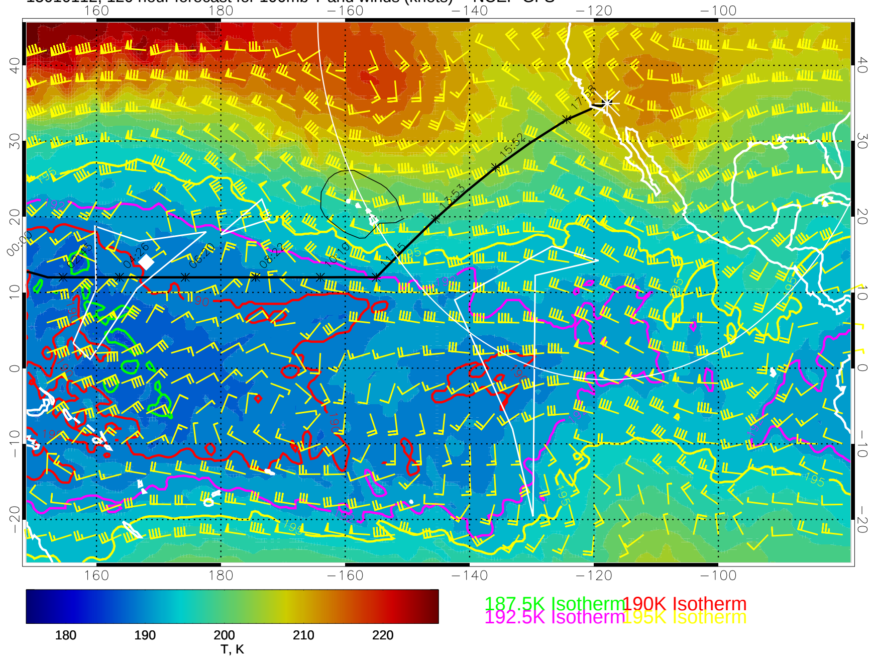
15010112, 120 hour forecast for 100mb T and winds (knots) -- NCEP GFS
