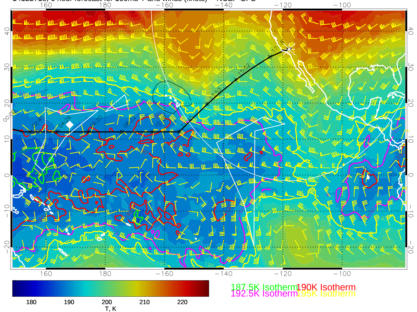
14122718, 6 hour forecast for 100mb T and winds (knots) -- NCEP GFS
