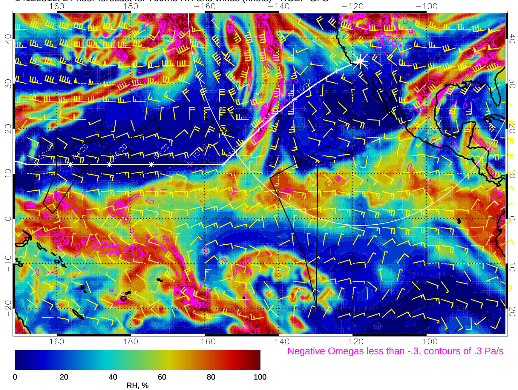
14122812, 24 hour forecast for 700mb RH and winds (knots) - NCEP GFS
