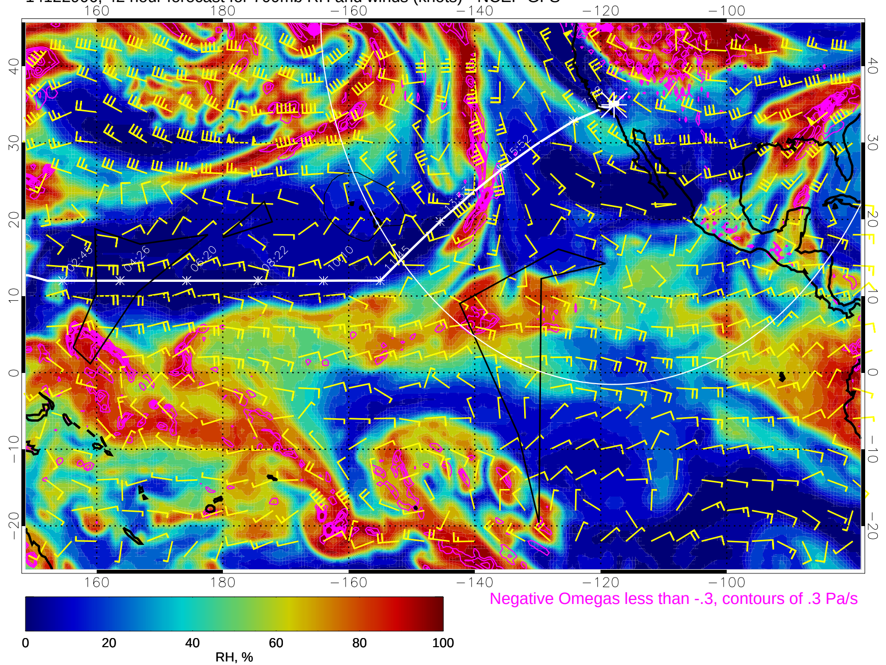
14122906, 42 hour forecast for 700mb RH and winds (knots) - NCEP GFS
