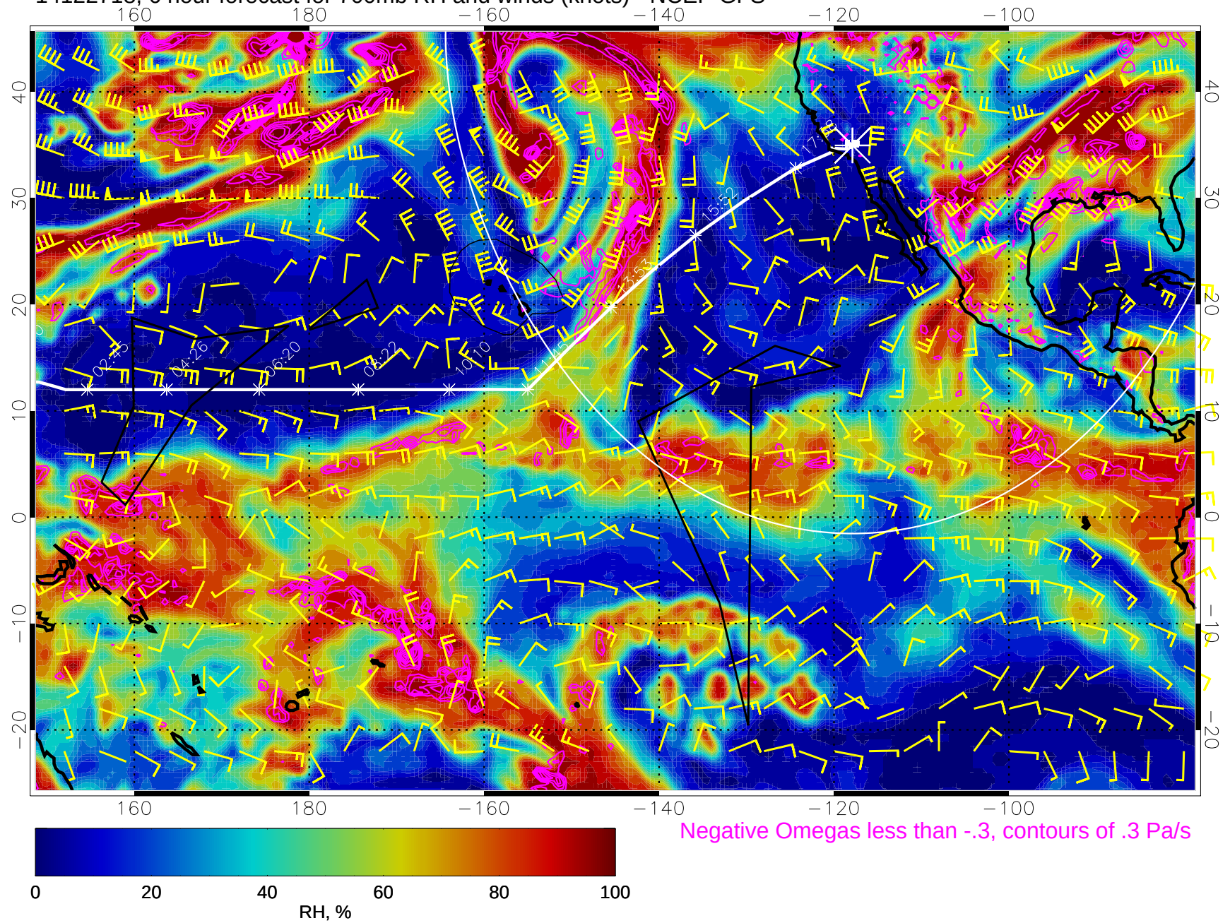
14122718, 6 hour forecast for 700mb RH and winds (knots) - NCEP GFS
