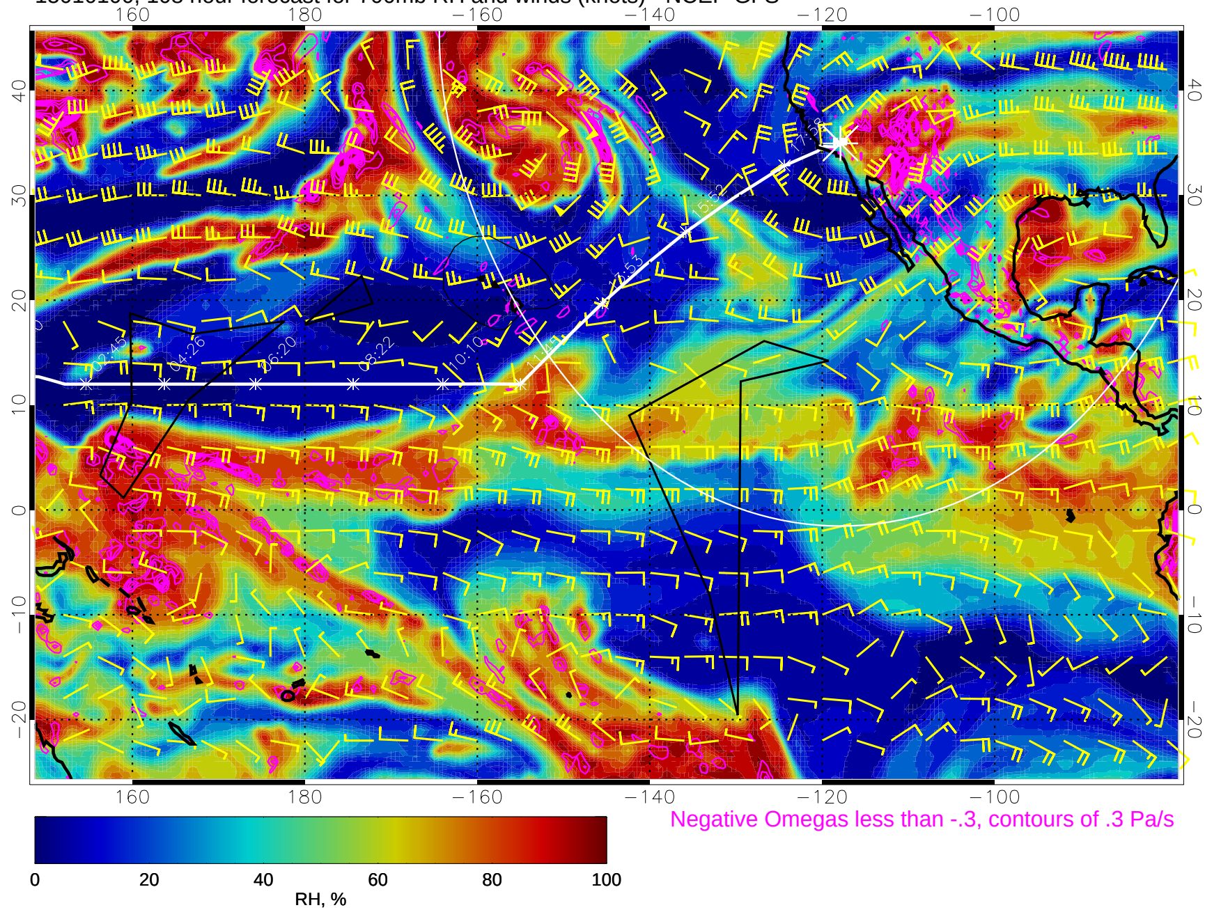
15010100, 108 hour forecast for 700mb RH and winds (knots) - NCEP GFS
