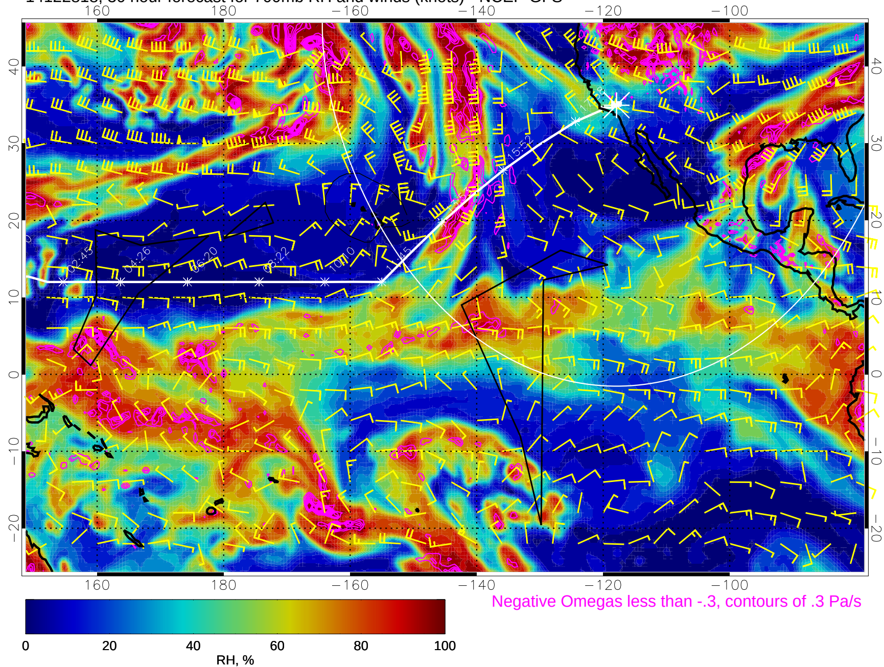
14122818, 30 hour forecast for 700mb RH and winds (knots) - NCEP GFS
