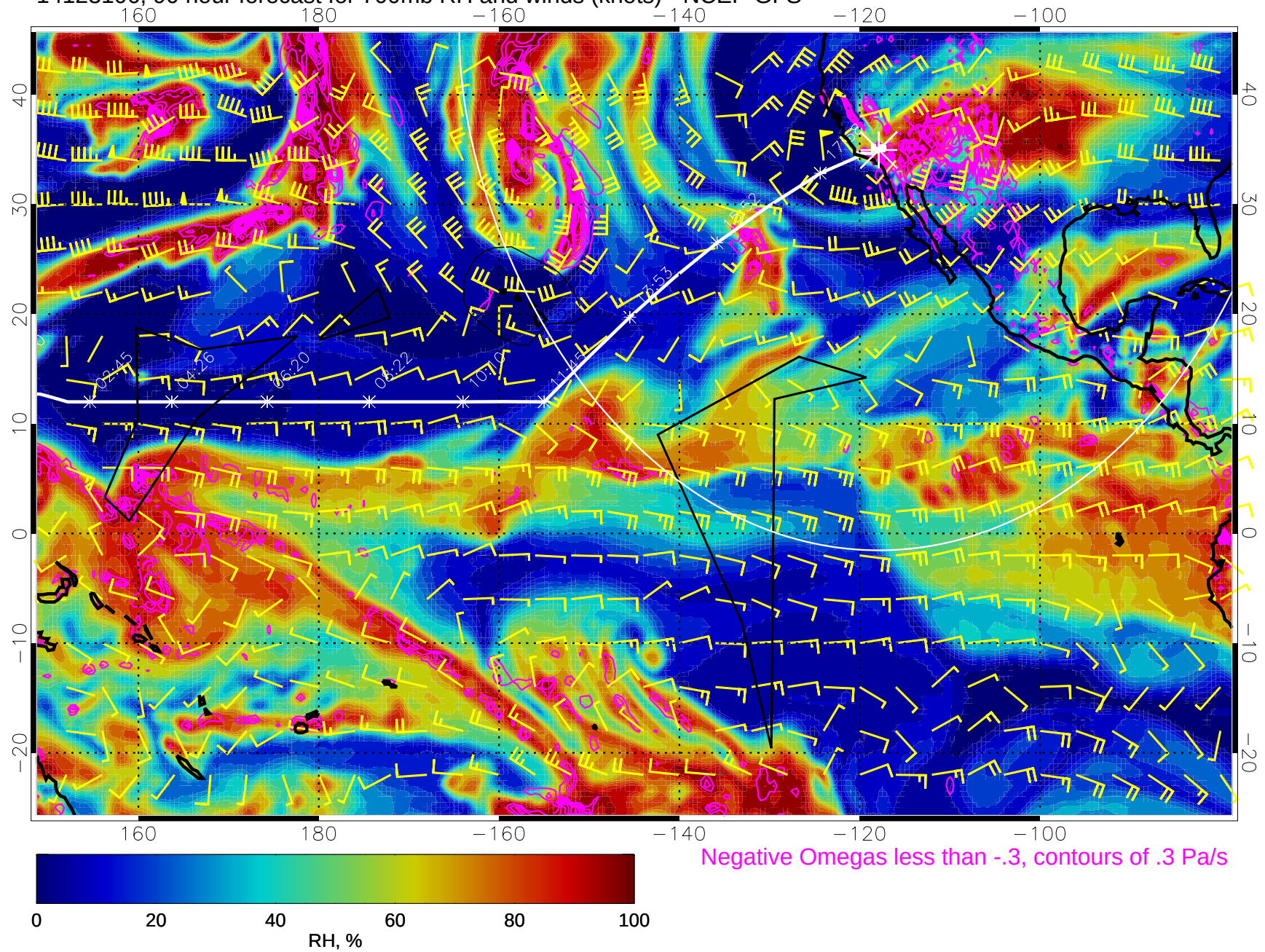
14123106, 90 hour forecast for 700mb RH and winds (knots) - NCEP GFS
