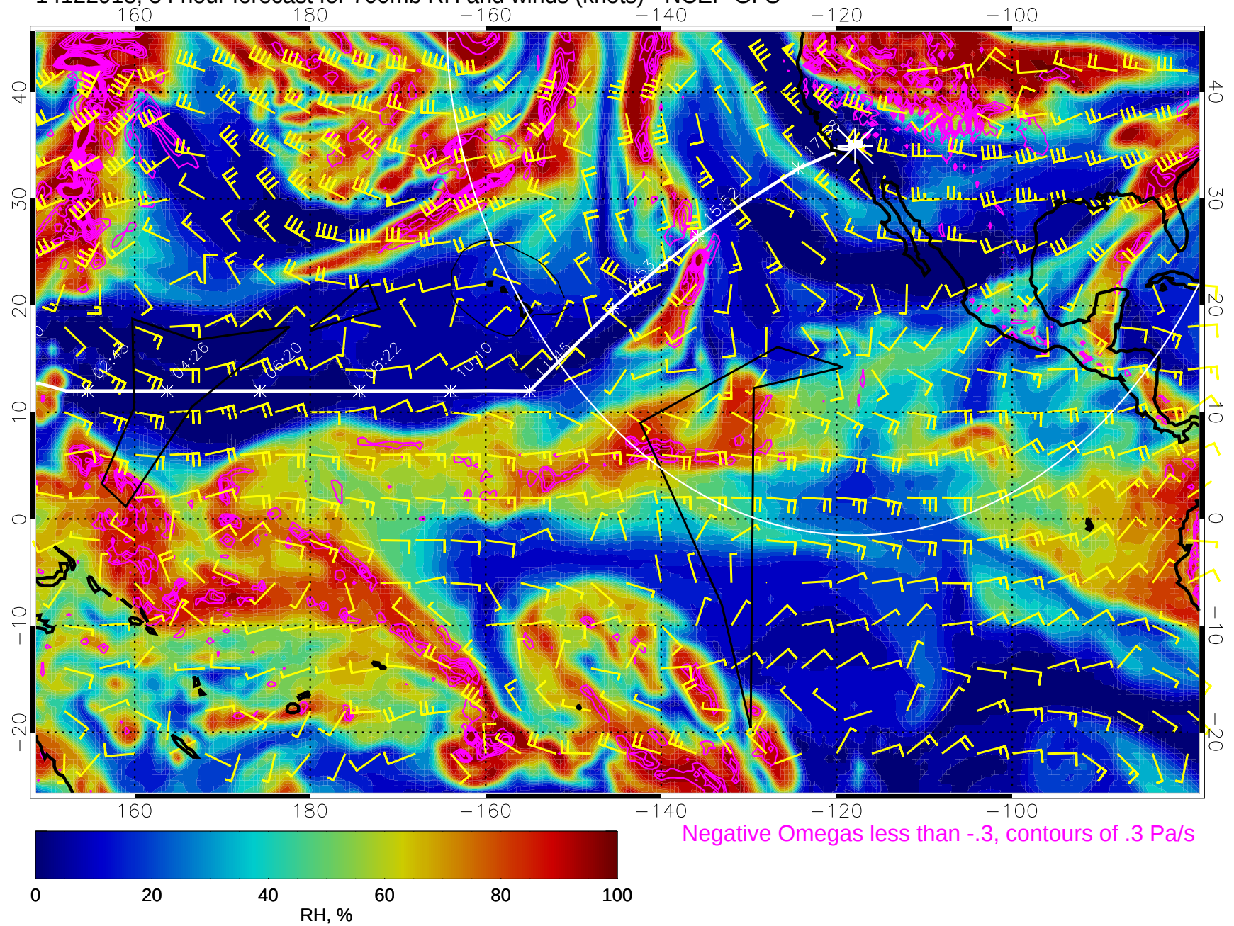
14122918, 54 hour forecast for 700mb RH and winds (knots) - NCEP GFS
