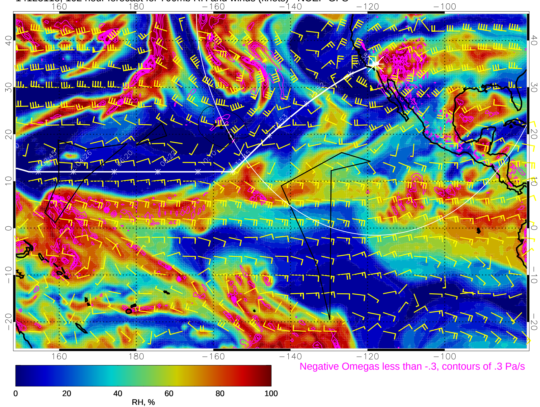
14123118, 102 hour forecast for 700mb RH and winds (knots) - NCEP GFS
