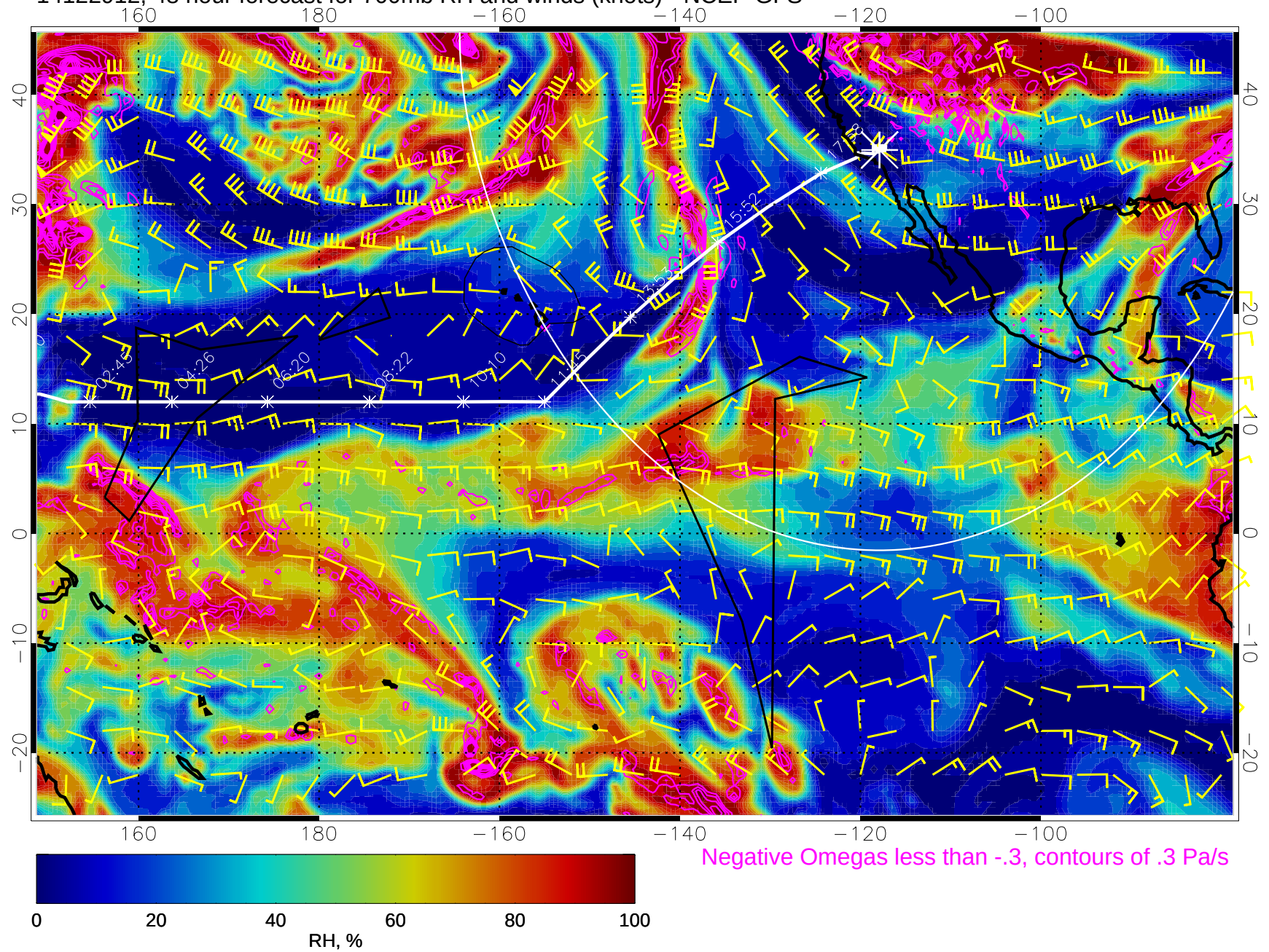
14122912, 48 hour forecast for 700mb RH and winds (knots) - NCEP GFS
