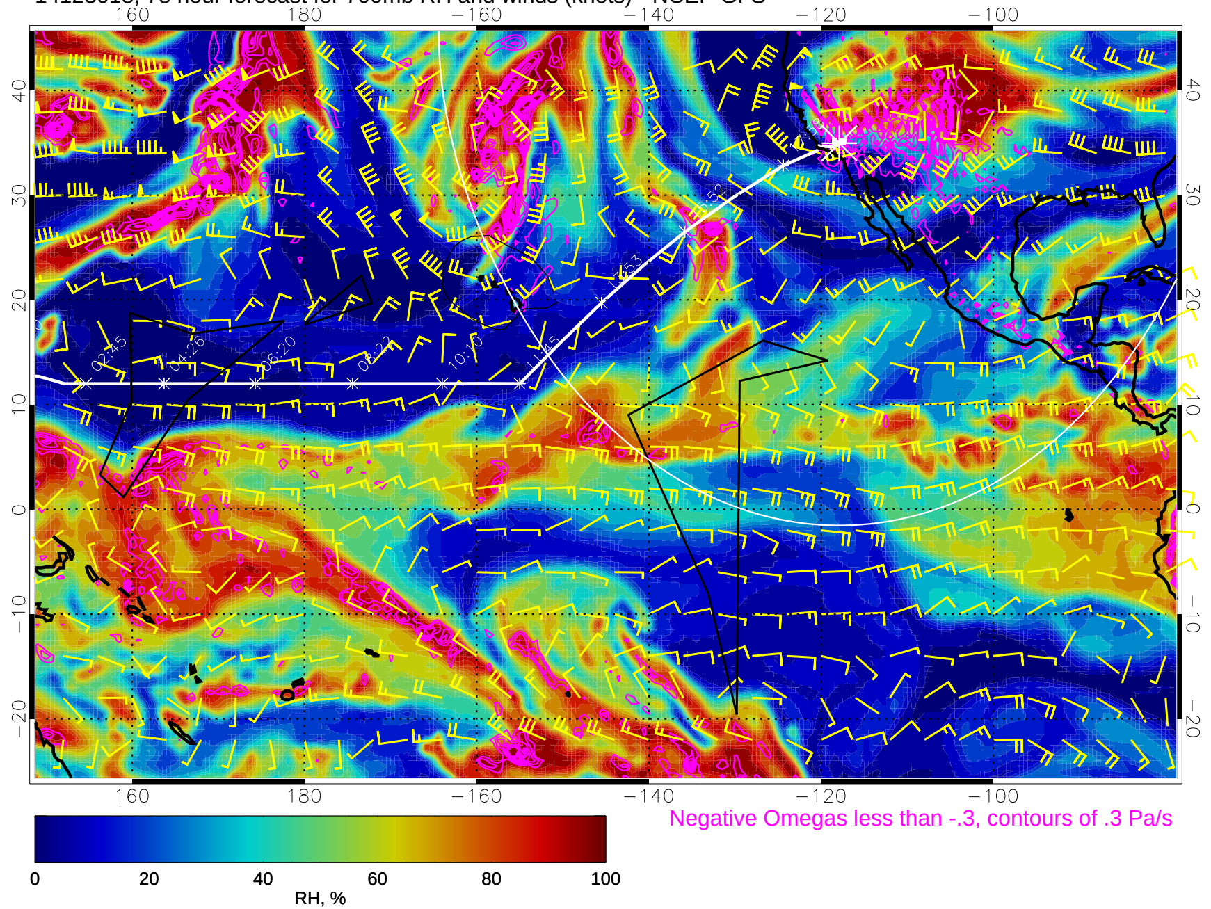
14123018, 78 hour forecast for 700mb RH and winds (knots) - NCEP GFS
