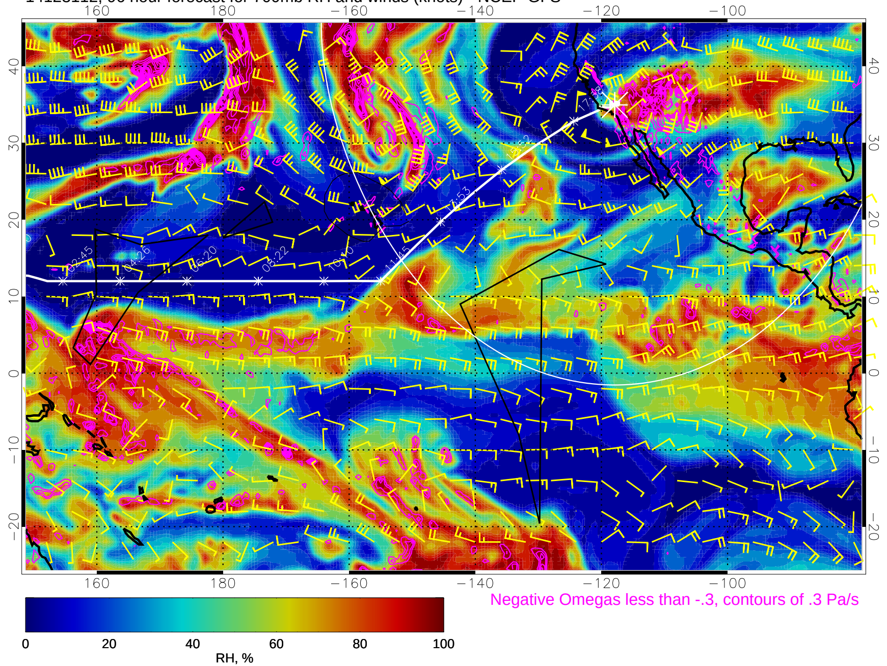
14123112, 96 hour forecast for 700mb RH and winds (knots) - NCEP GFS
