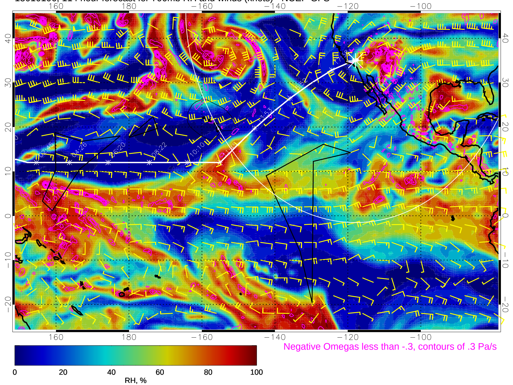
15010106, 114 hour forecast for 700mb RH and winds (knots) - NCEP GFS
