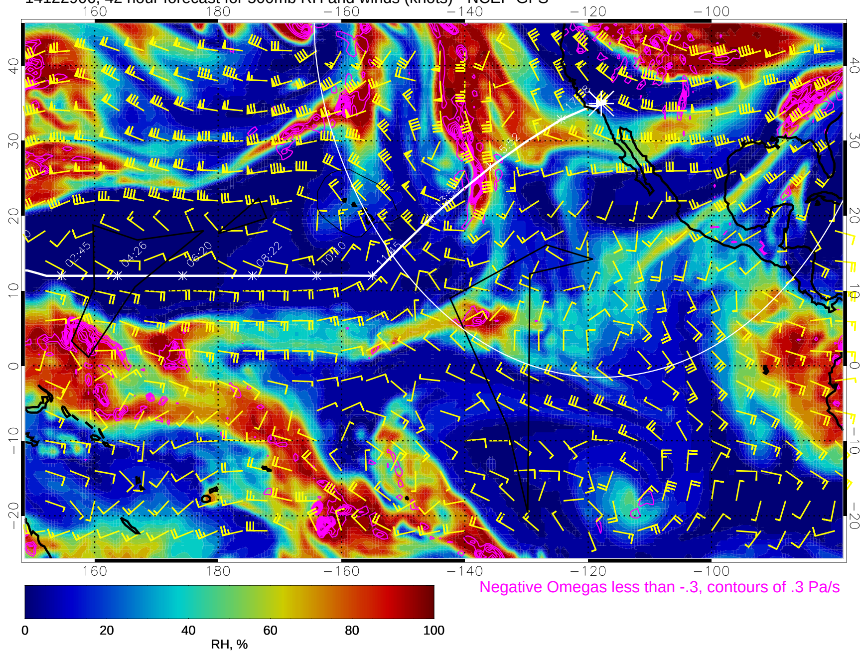
14122906, 42 hour forecast for 500mb RH and winds (knots) - NCEP GFS
