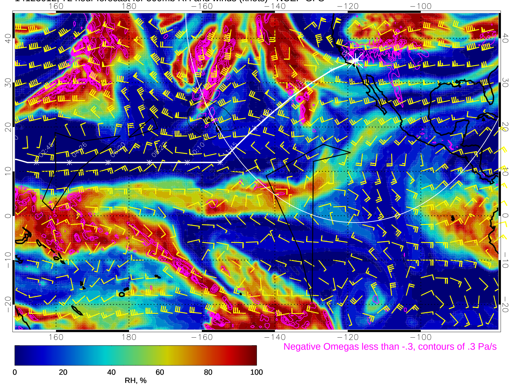
14123012, 72 hour forecast for 500mb RH and winds (knots) - NCEP GFS
