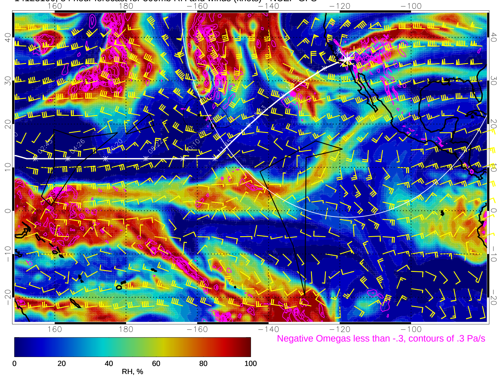
14123100, 84 hour forecast for 500mb RH and winds (knots) - NCEP GFS
