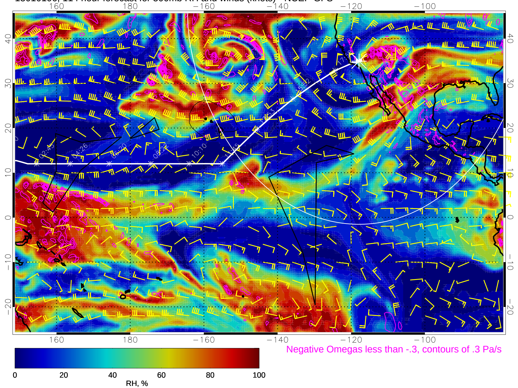
15010106, 114 hour forecast for 500mb RH and winds (knots) - NCEP GFS
