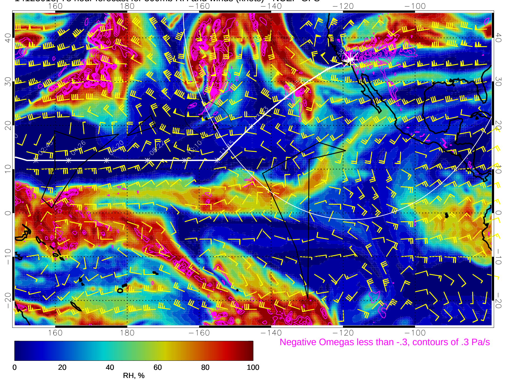
14123018, 78 hour forecast for 500mb RH and winds (knots) - NCEP GFS
