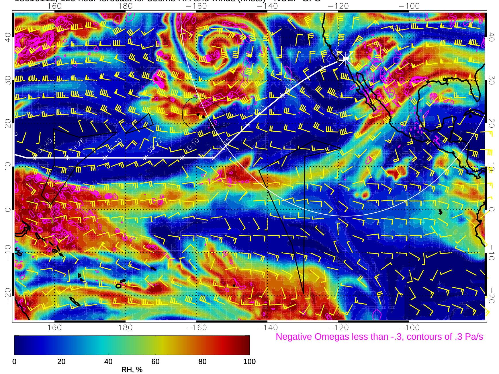
15010112, 120 hour forecast for 500mb RH and winds (knots) - NCEP GFS
