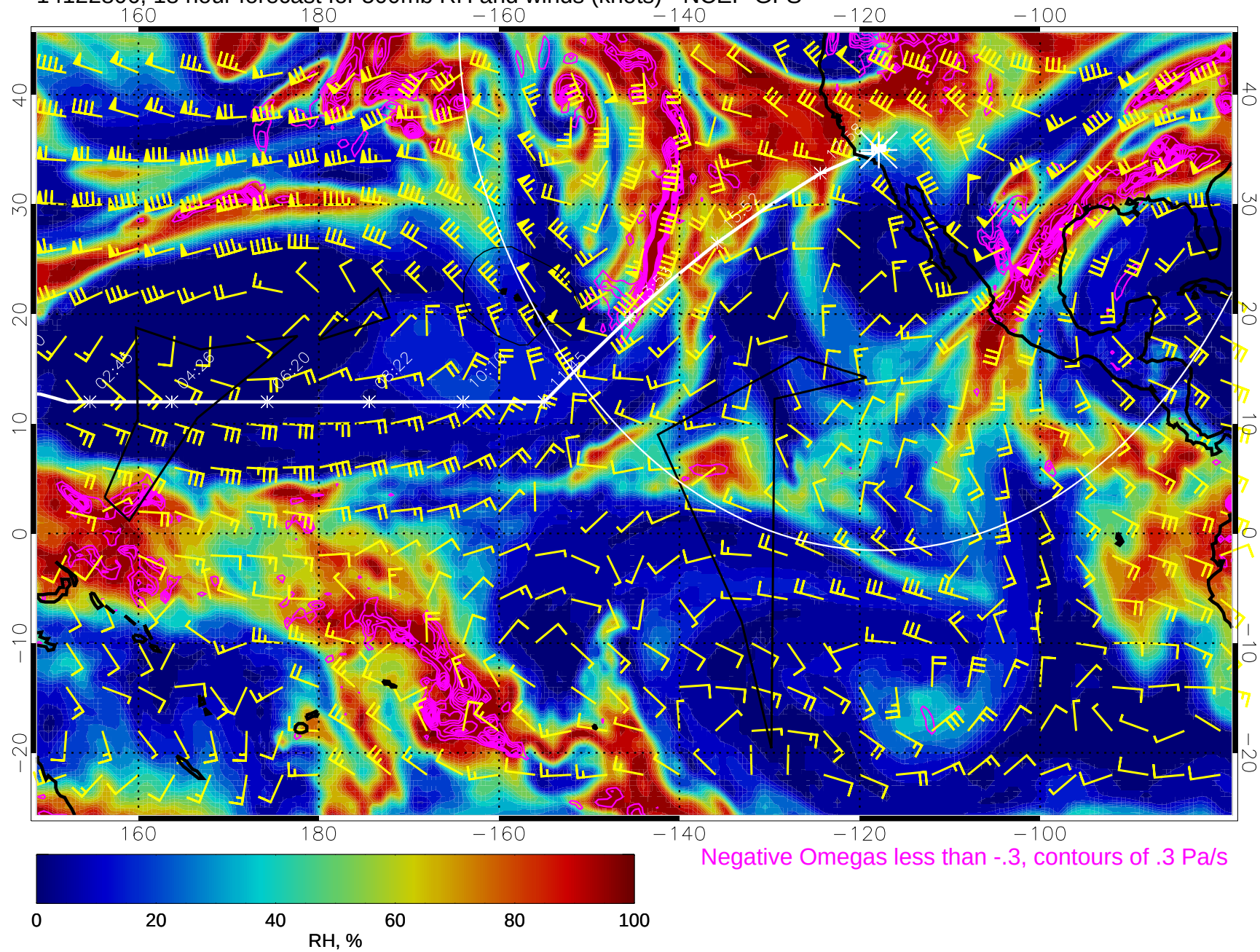
14122806, 18 hour forecast for 500mb RH and winds (knots) - NCEP GFS
