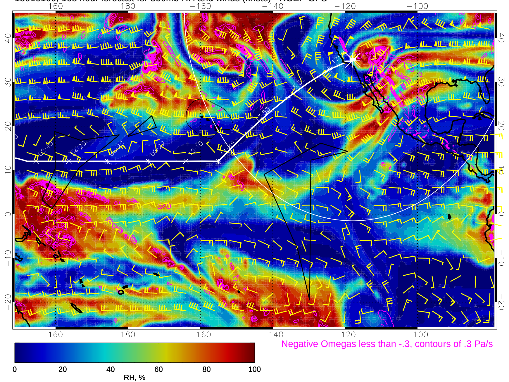
15010100, 108 hour forecast for 500mb RH and winds (knots) - NCEP GFS
