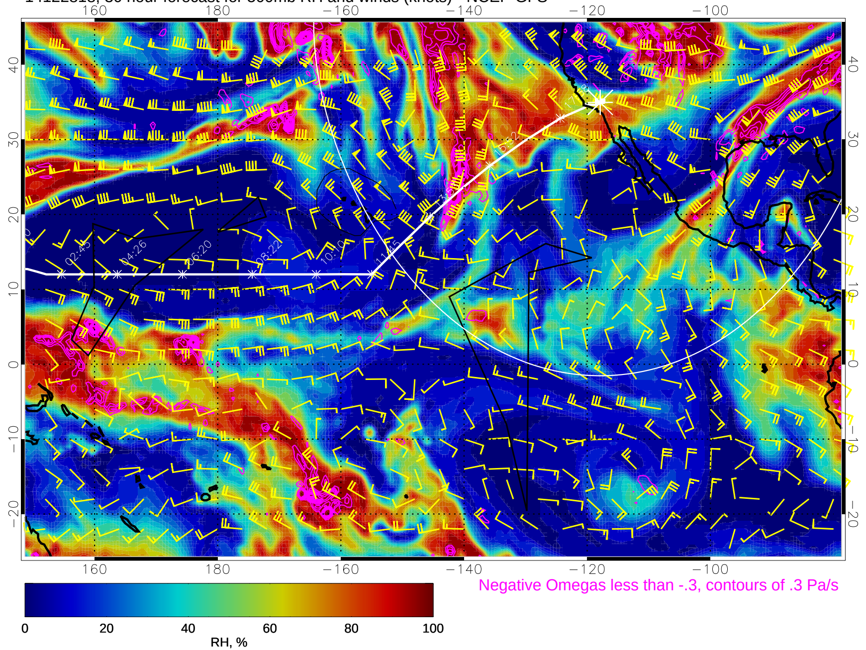
14122818, 30 hour forecast for 500mb RH and winds (knots) - NCEP GFS
