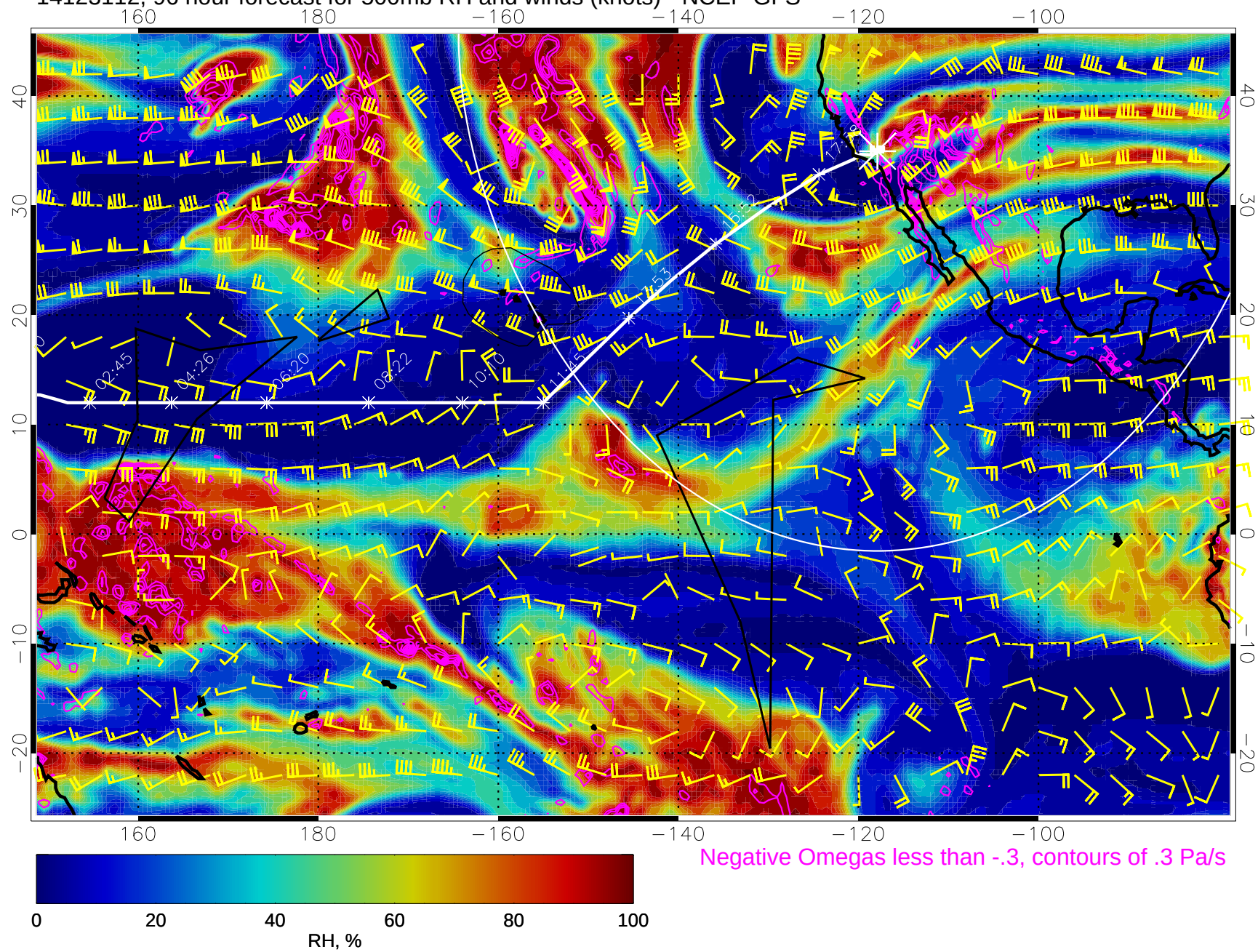
14123112, 96 hour forecast for 500mb RH and winds (knots) - NCEP GFS
