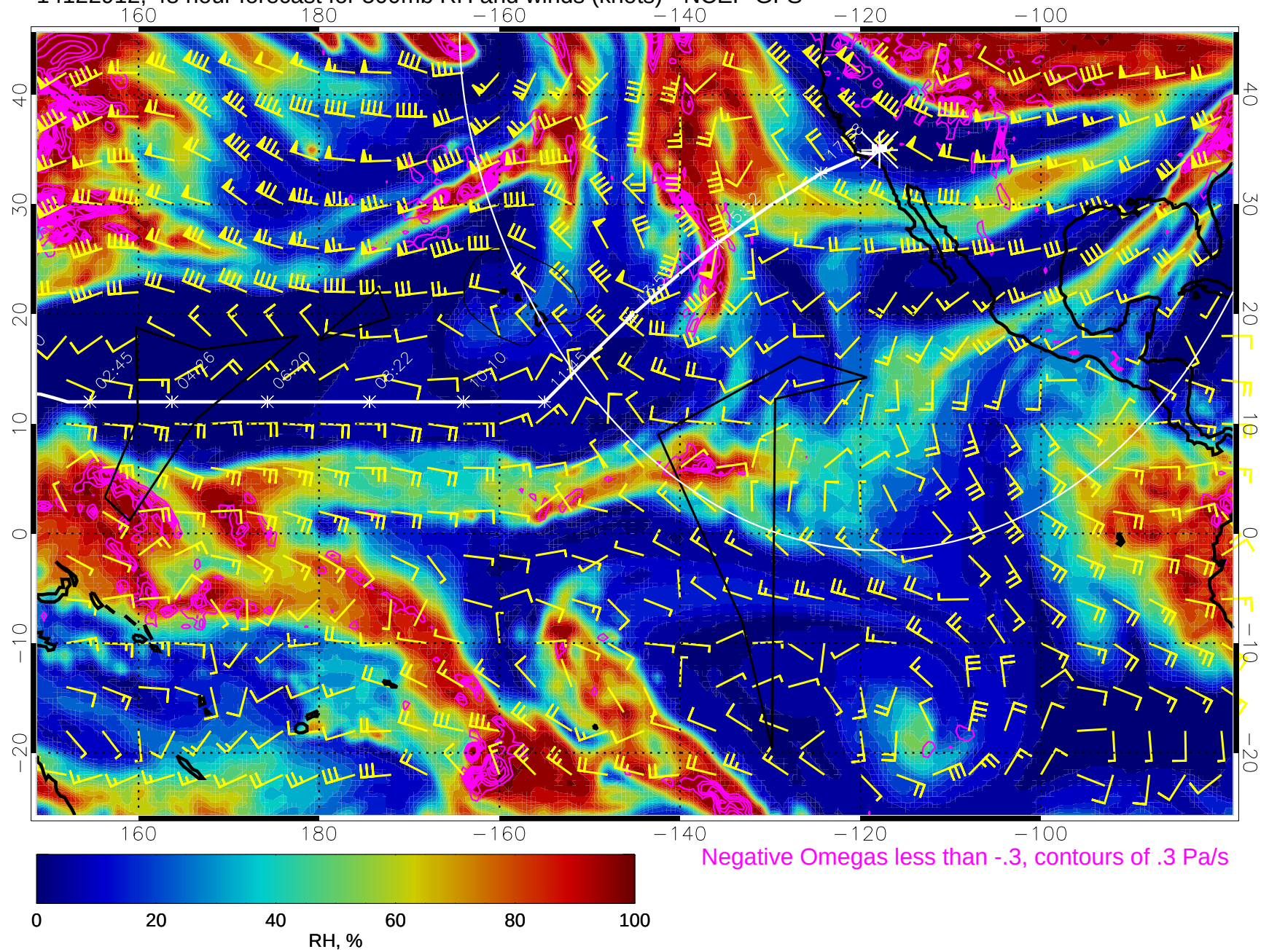
14122912, 48 hour forecast for 500mb RH and winds (knots) - NCEP GFS
