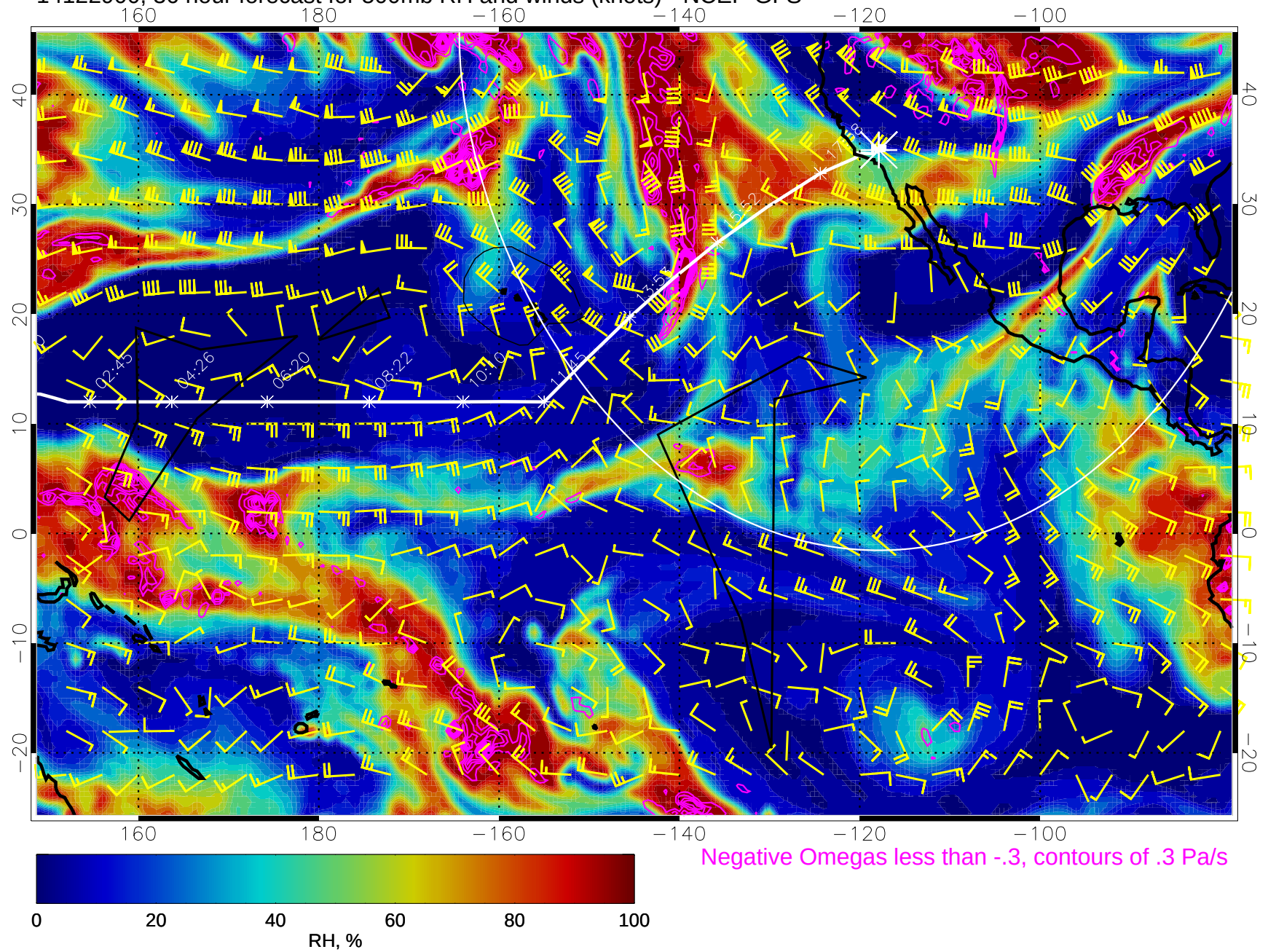
14122900, 36 hour forecast for 500mb RH and winds (knots) - NCEP GFS
