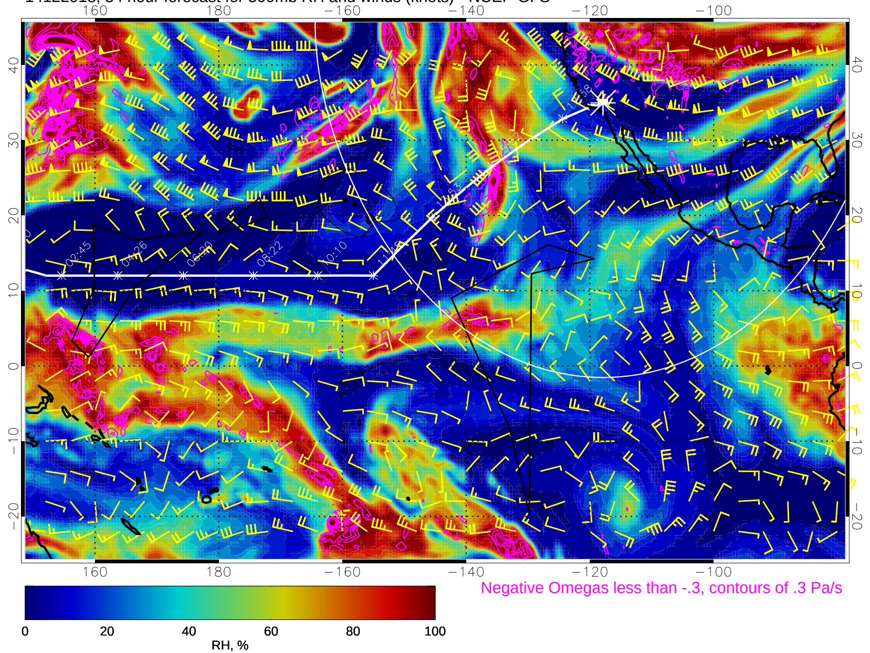
14122918, 54 hour forecast for 500mb RH and winds (knots) - NCEP GFS
