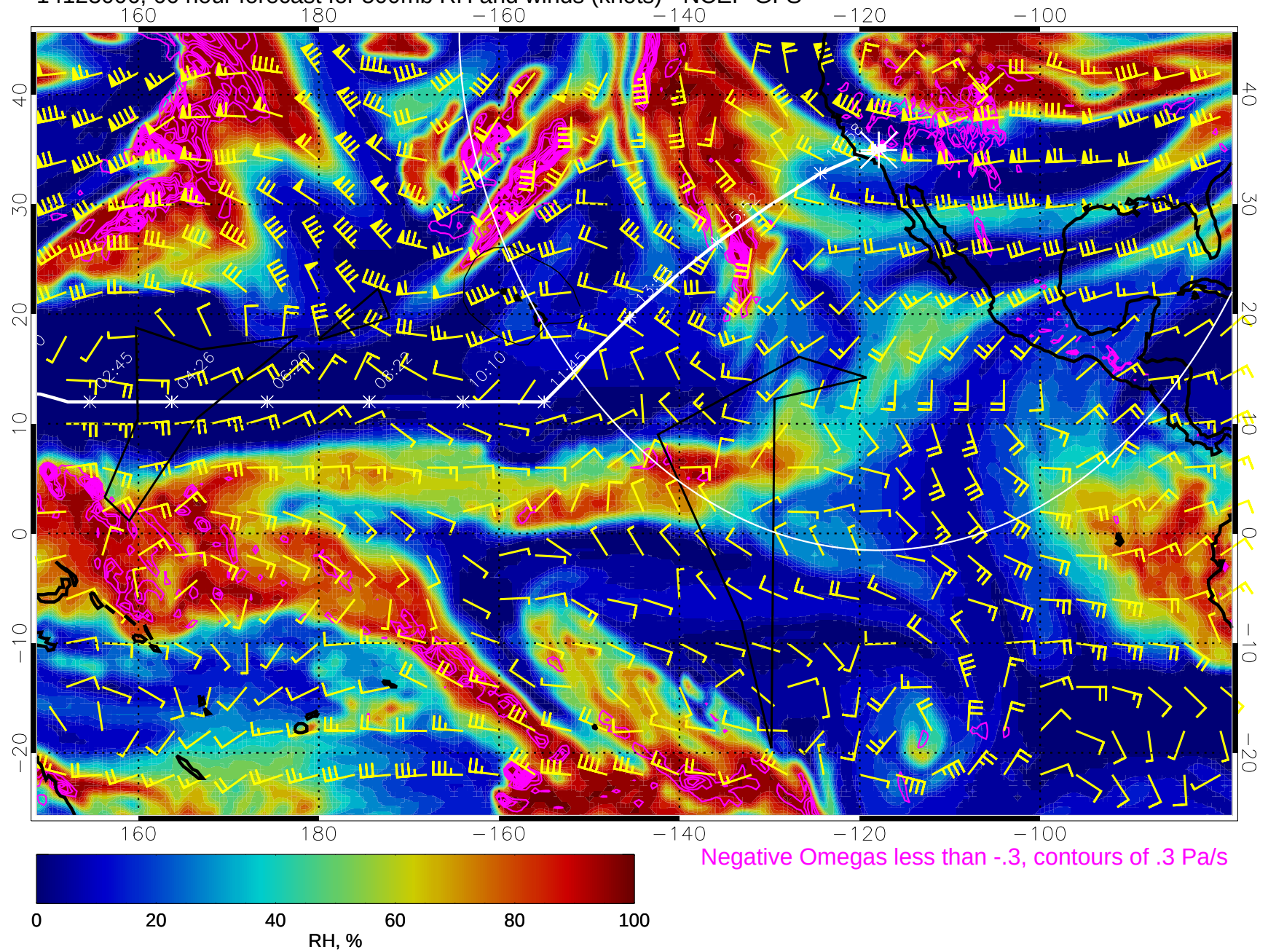
14123006, 66 hour forecast for 500mb RH and winds (knots) - NCEP GFS
