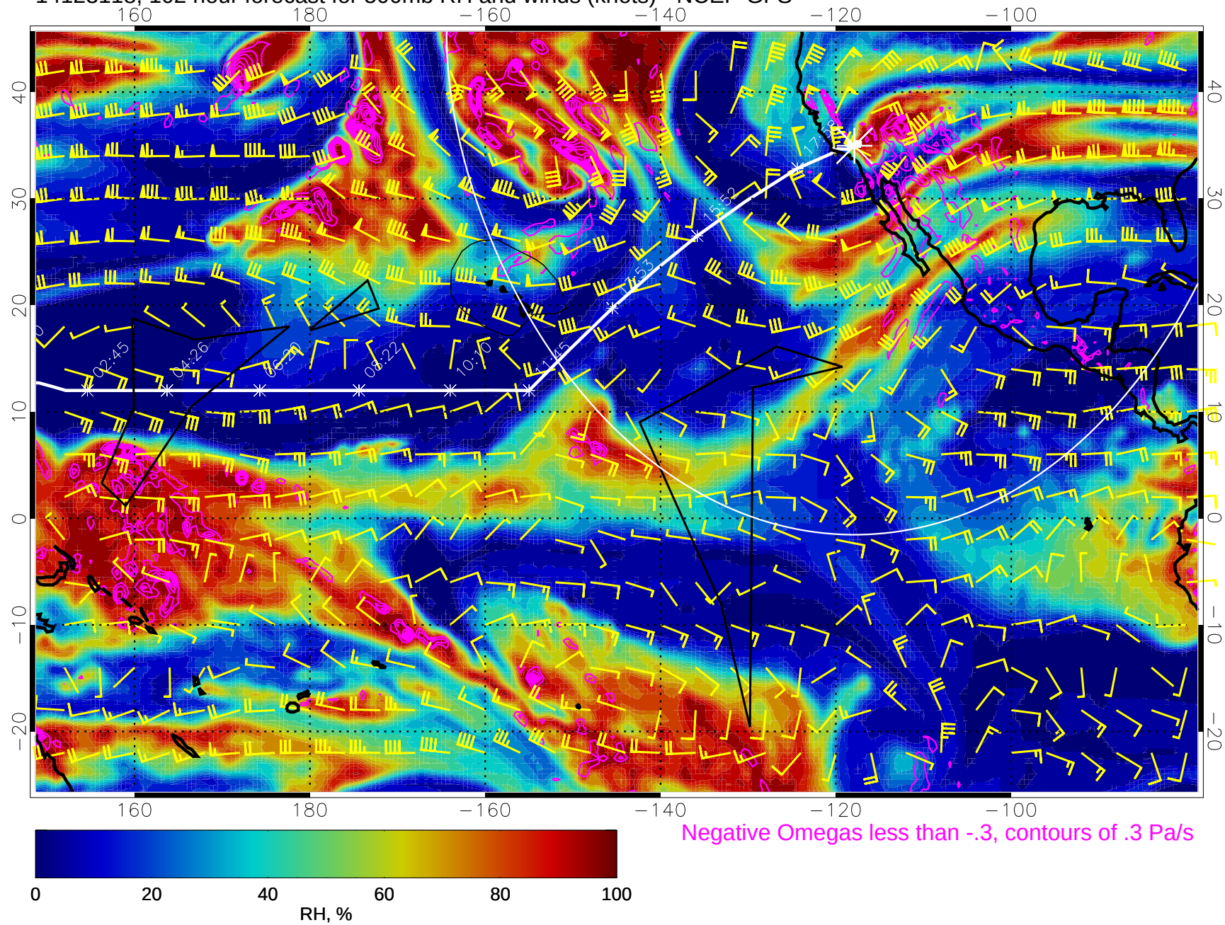
14123118, 102 hour forecast for 500mb RH and winds (knots) - NCEP GFS
