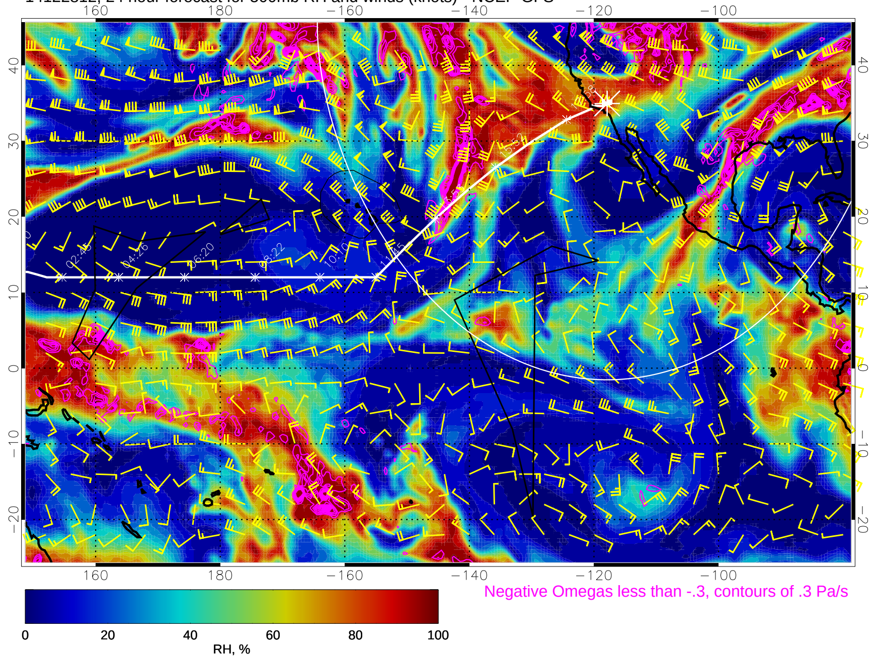
14122812, 24 hour forecast for 500mb RH and winds (knots) - NCEP GFS
