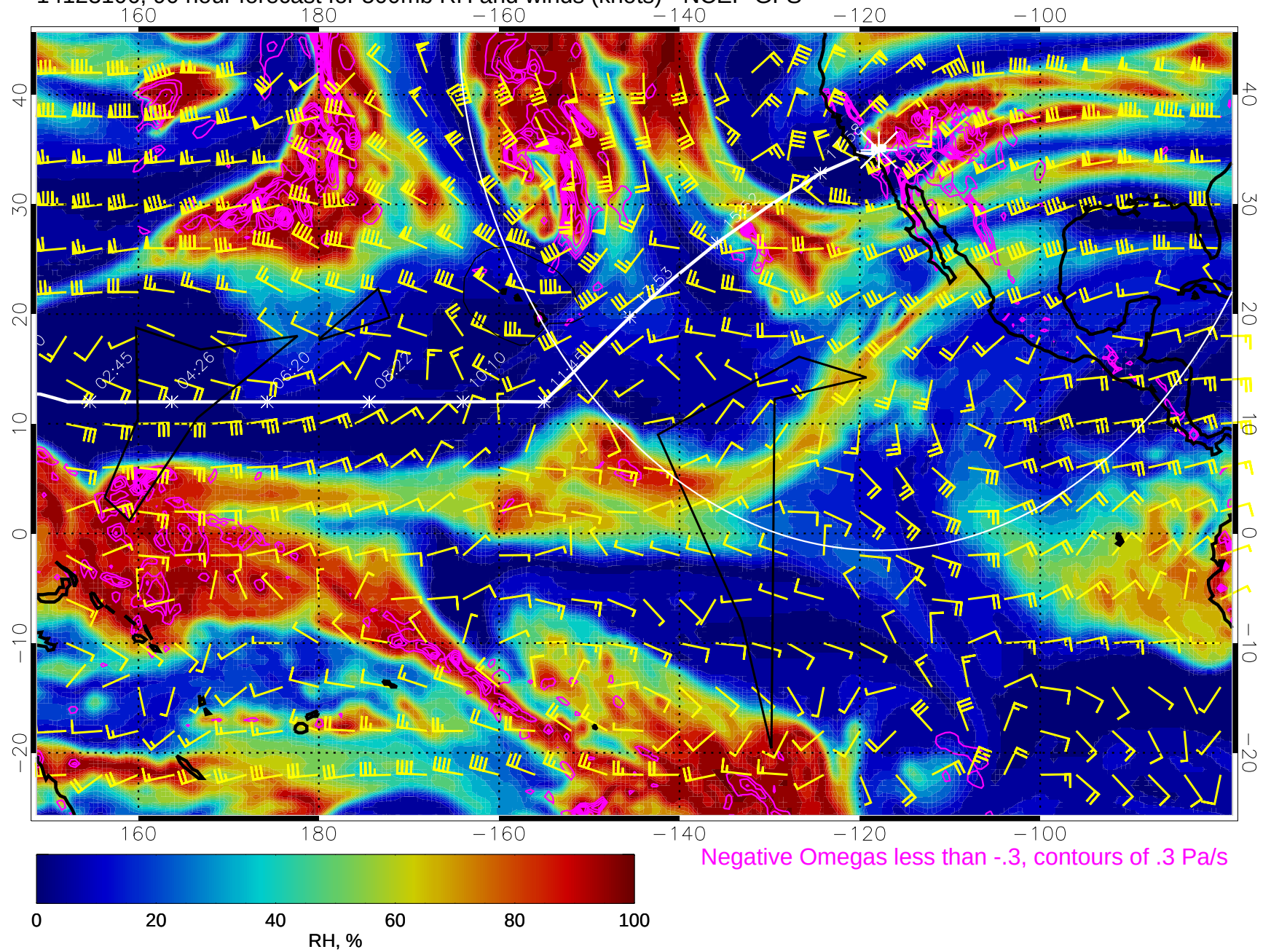
14123106, 90 hour forecast for 500mb RH and winds (knots) - NCEP GFS
