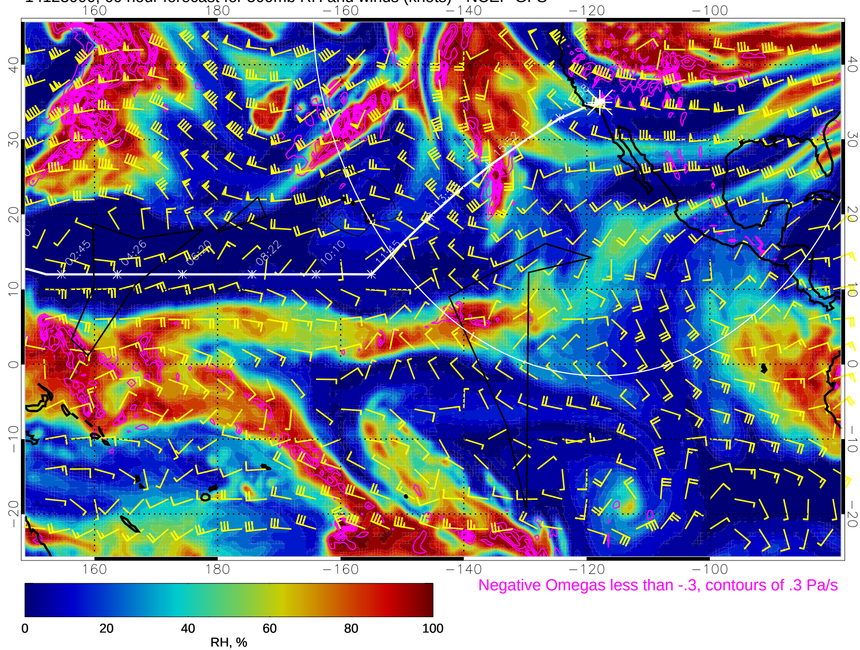
14123000, 60 hour forecast for 500mb RH and winds (knots) - NCEP GFS
