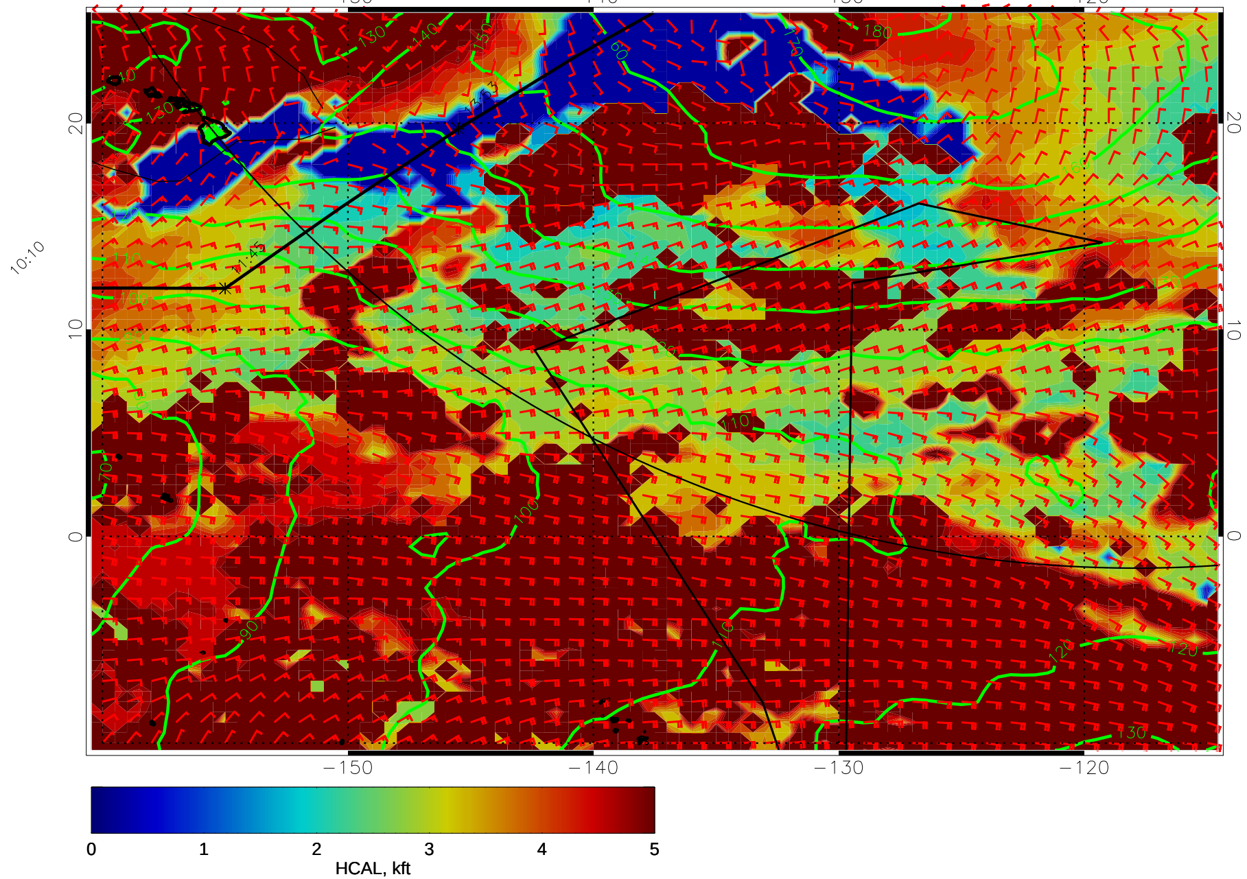
14123118, 102 hour forecast for HCAL, 1000mb Z, and winds (knots) -- NCEP GFS
