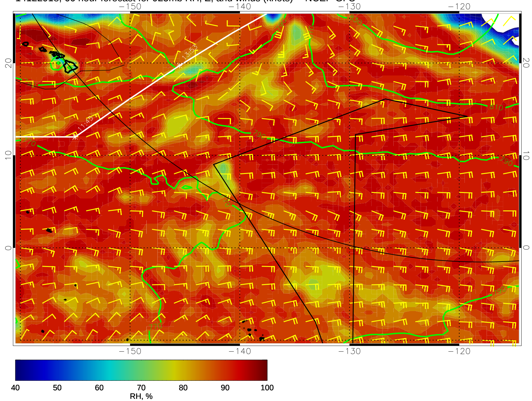
14122918, 66 hour forecast for 925mb RH, Z, and winds (knots) -- NCEP GFS
