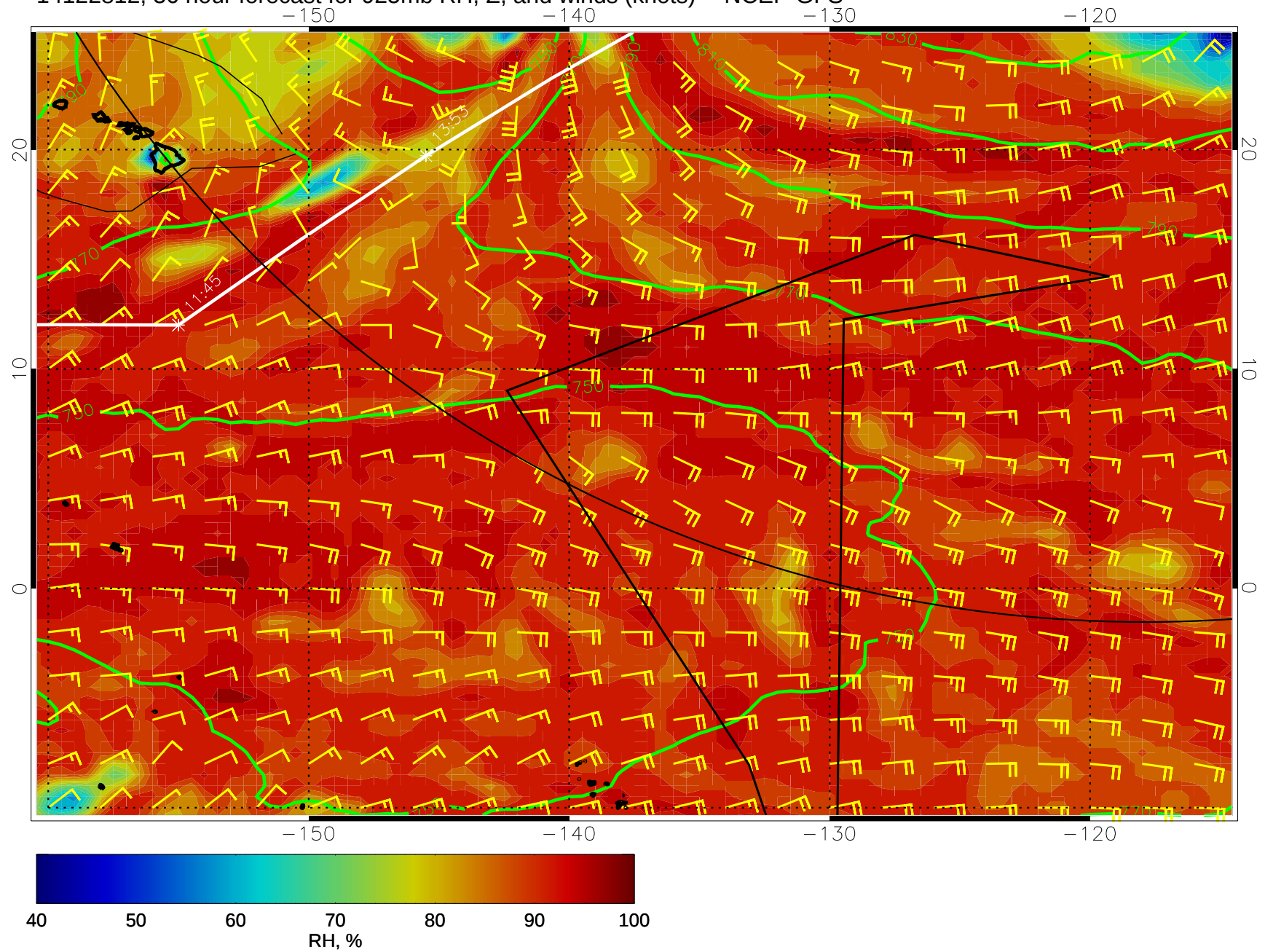
14122812, 36 hour forecast for 925mb RH, Z, and winds (knots) -- NCEP GFS
