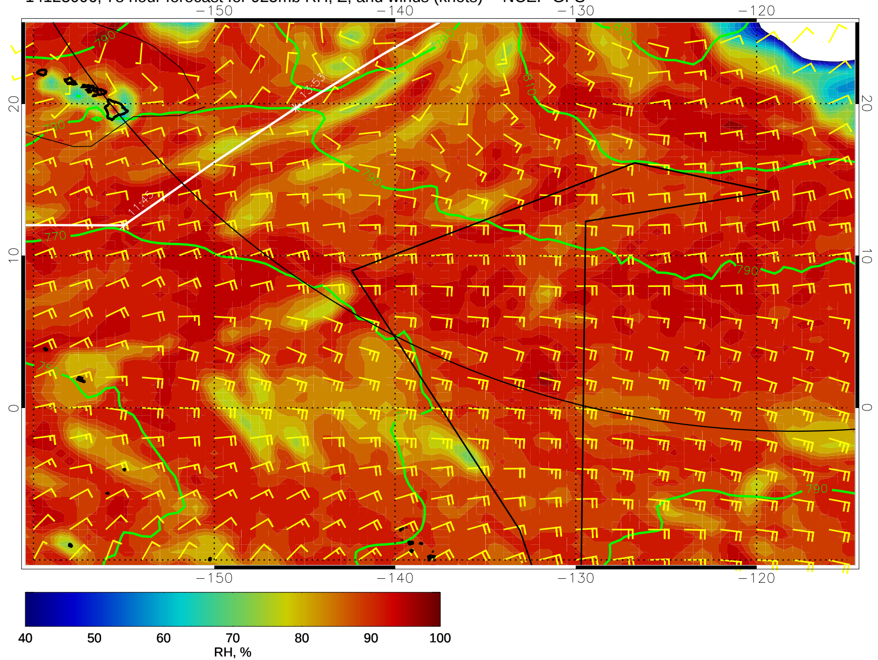
14123006, 78 hour forecast for 925mb RH, Z, and winds (knots) -- NCEP GFS
