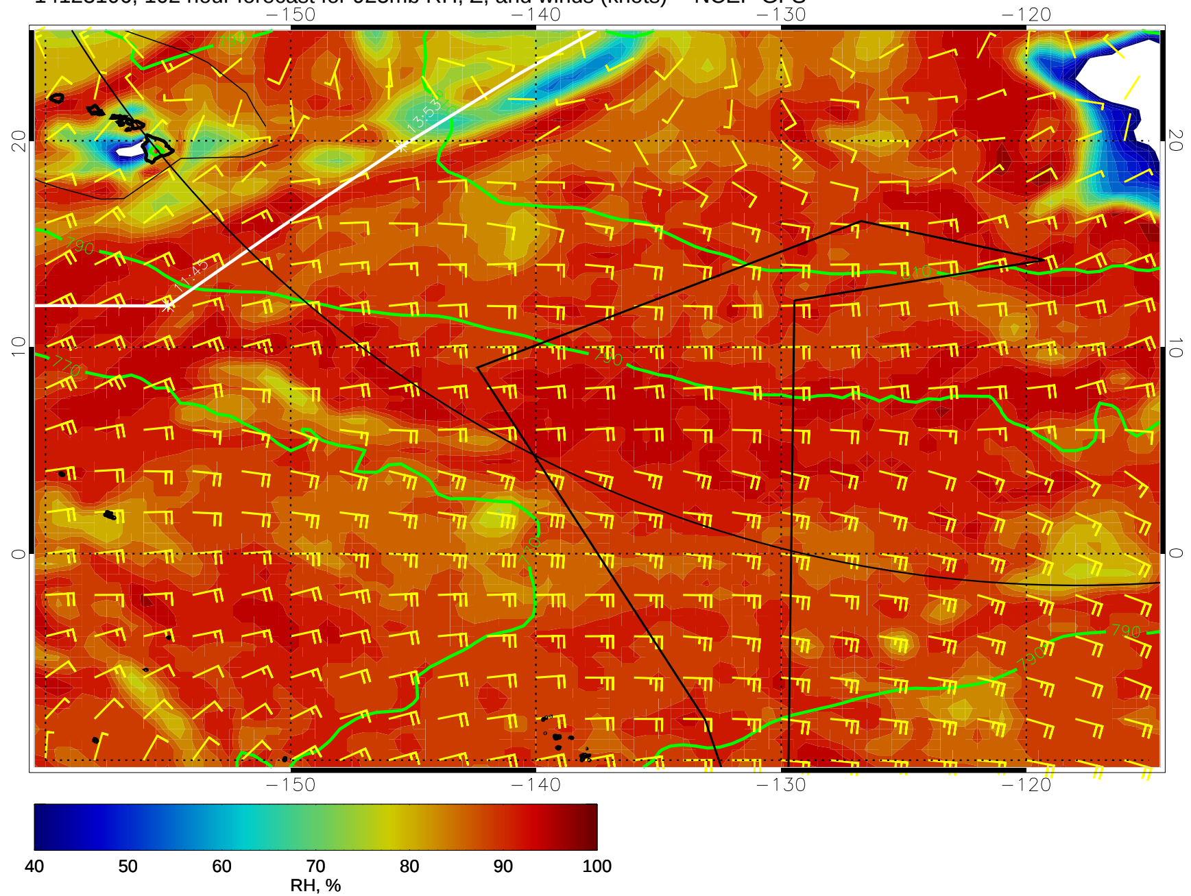
14123106, 102 hour forecast for 925mb RH, Z, and winds (knots) -- NCEP GFS
