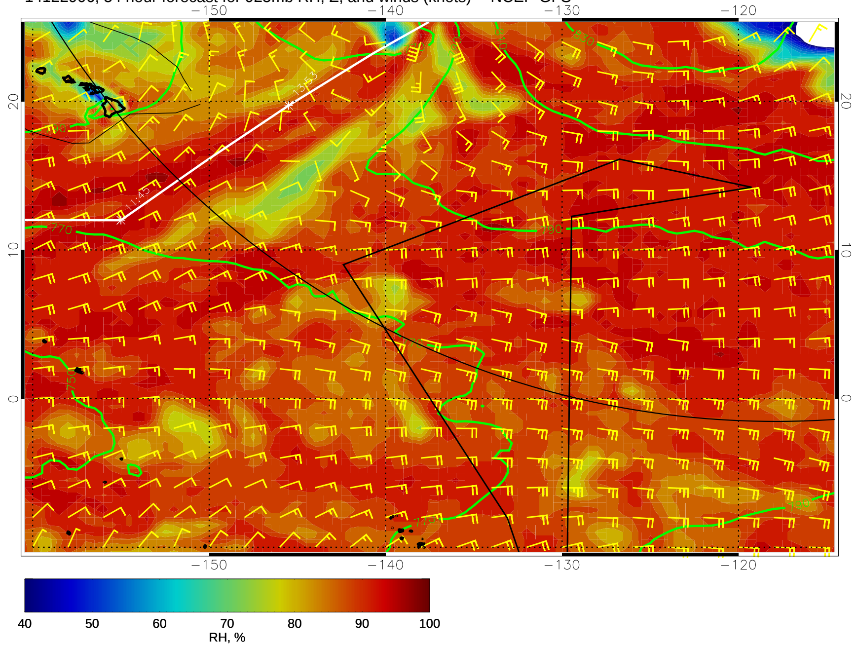
14122906, 54 hour forecast for 925mb RH, Z, and winds (knots) -- NCEP GFS
