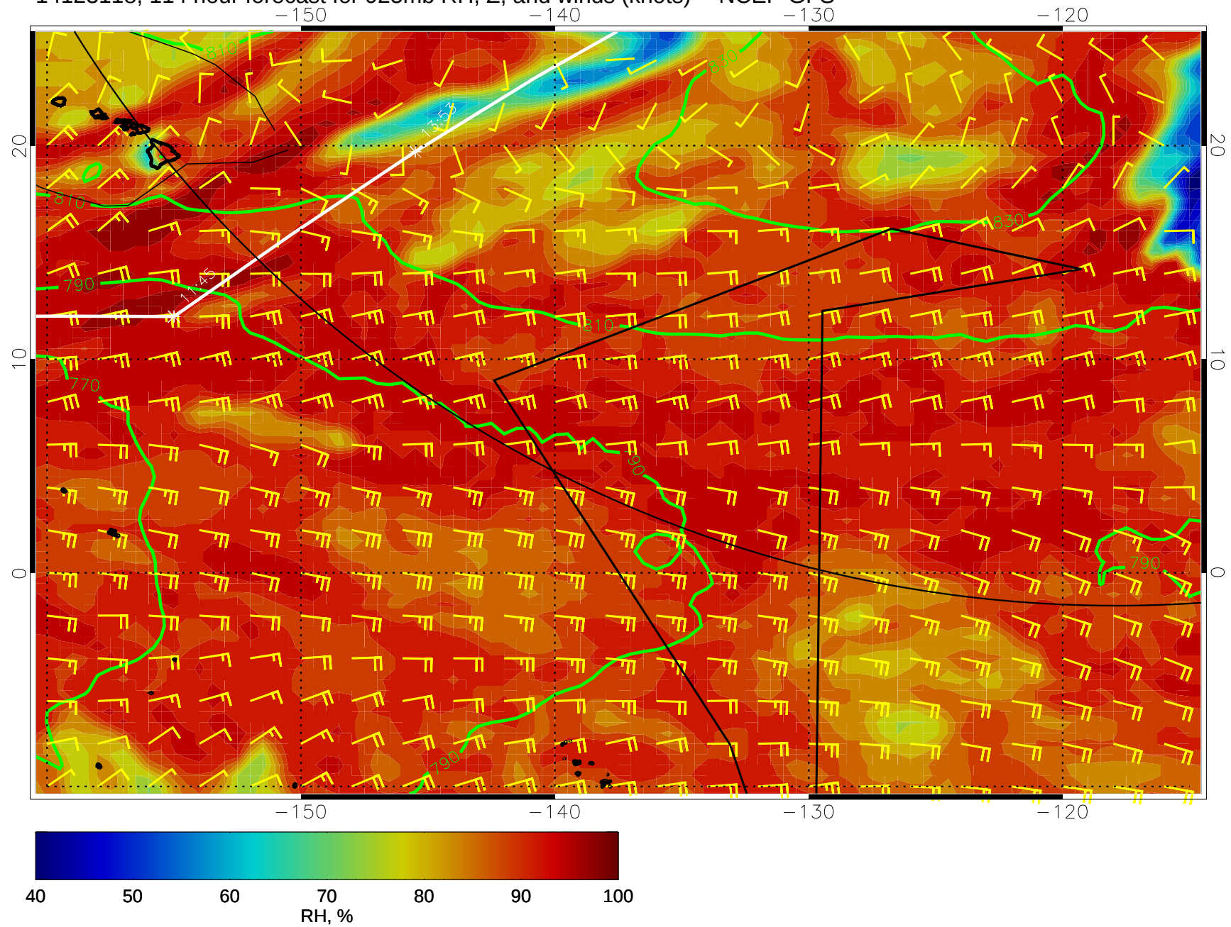
14123118, 114 hour forecast for 925mb RH, Z, and winds (knots) -- NCEP GFS
