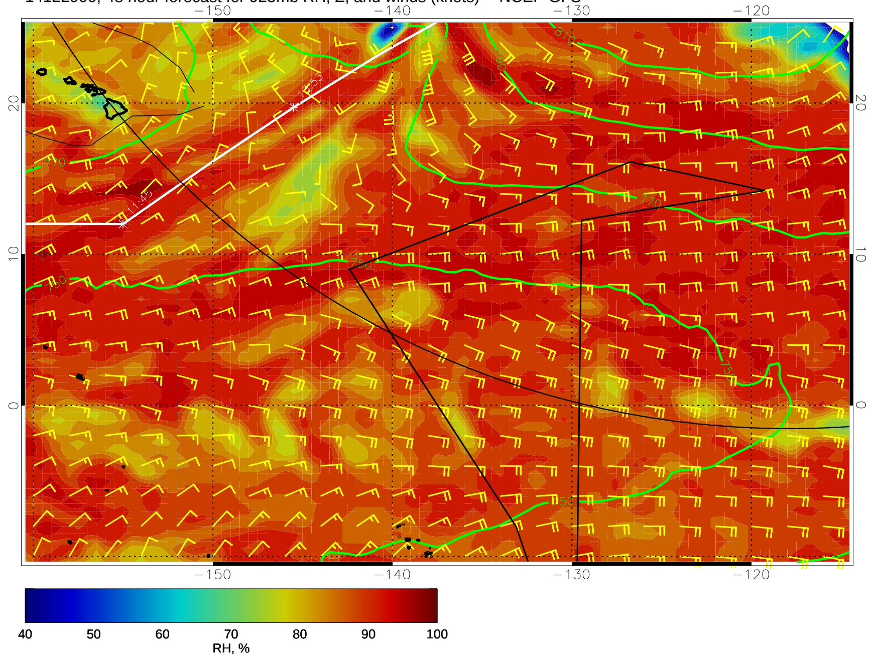
14122900, 48 hour forecast for 925mb RH, Z, and winds (knots) -- NCEP GFS
