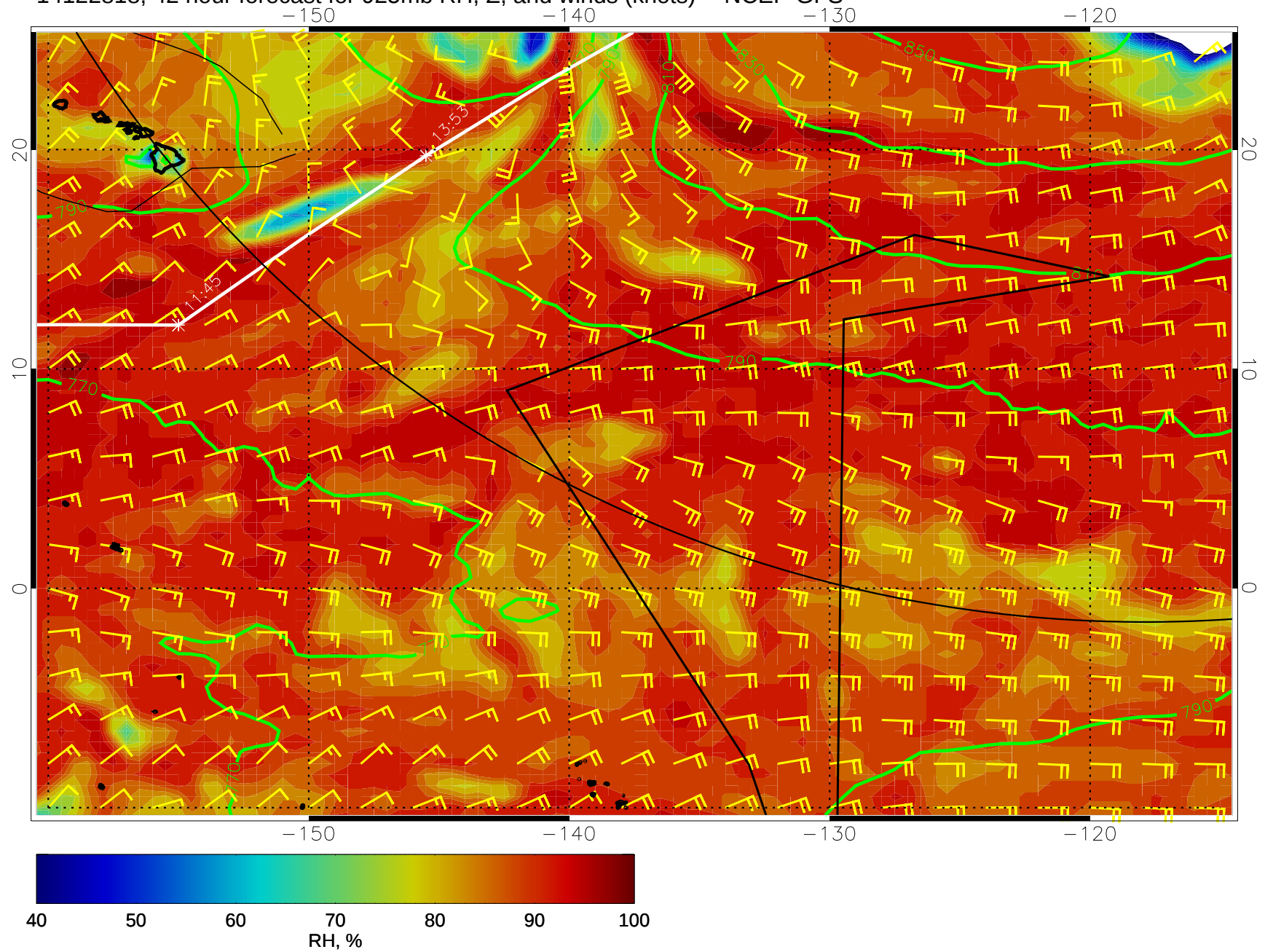
14122818, 42 hour forecast for 925mb RH, Z, and winds (knots) -- NCEP GFS
