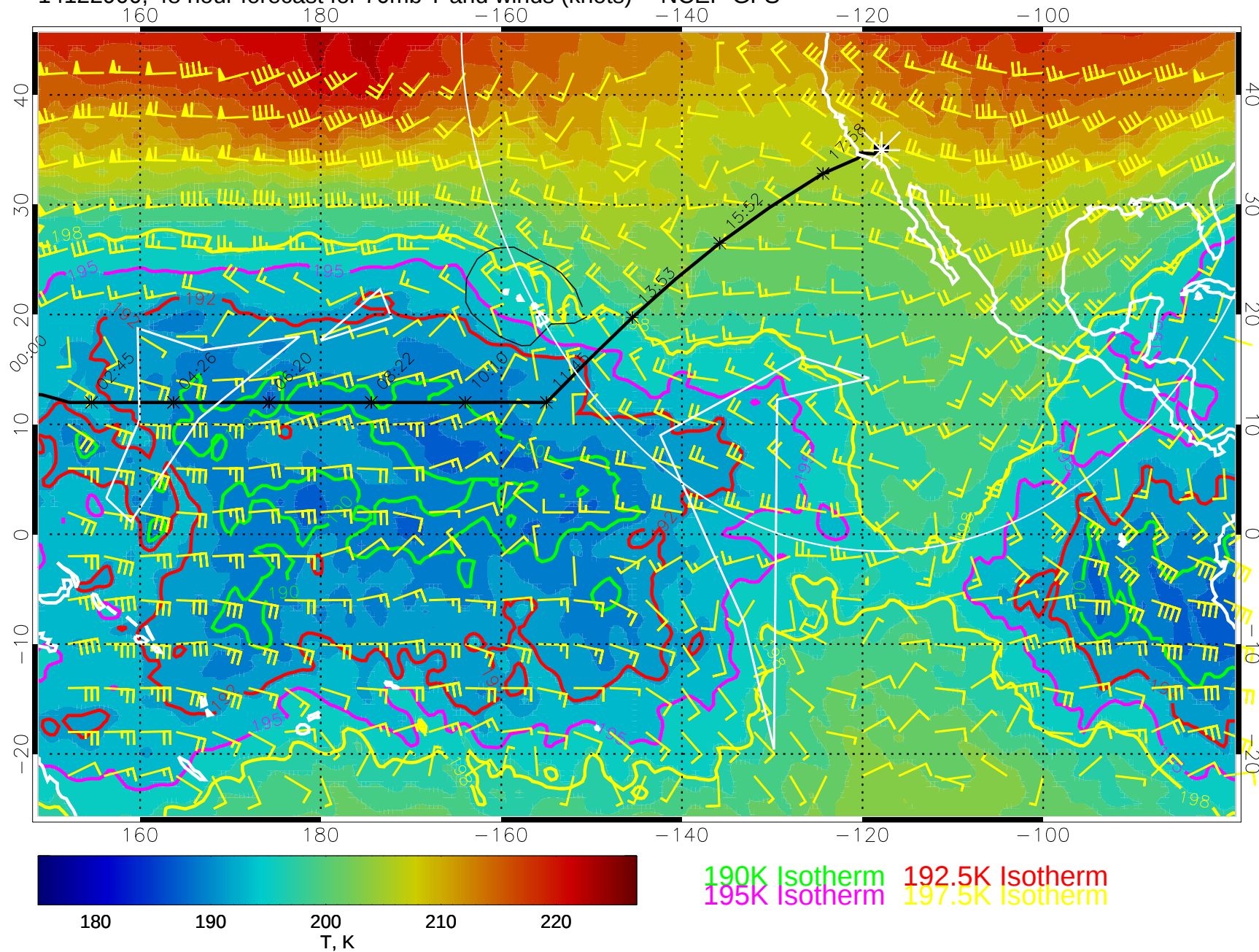
14122900, 48 hour forecast for 70mb T and winds (knots) -- NCEP GFS
