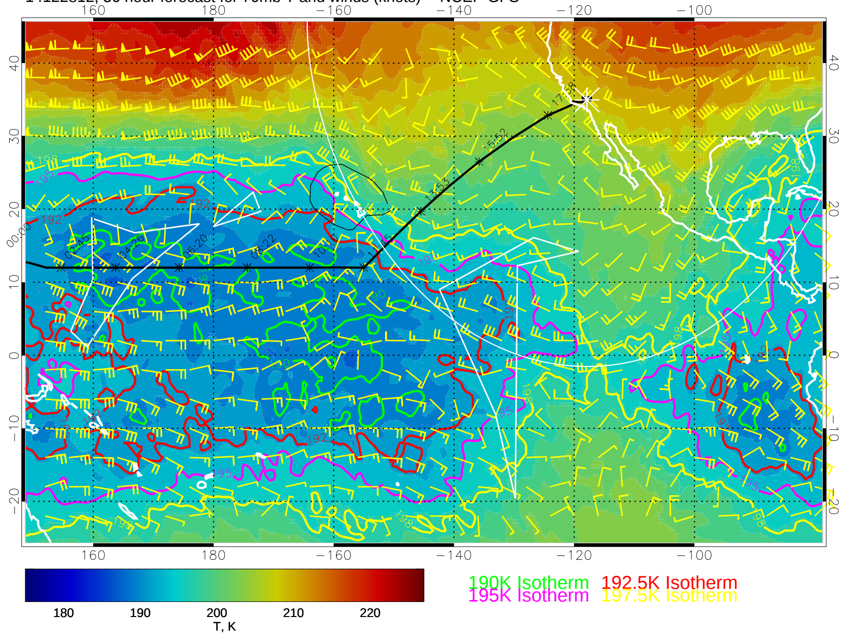
14122812, 36 hour forecast for 70mb T and winds (knots) -- NCEP GFS
