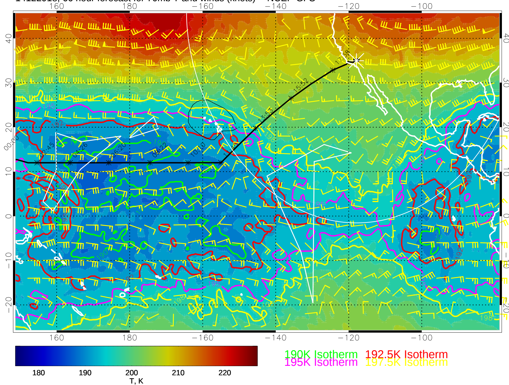
14122918, 66 hour forecast for 70mb T and winds (knots) -- NCEP GFS
