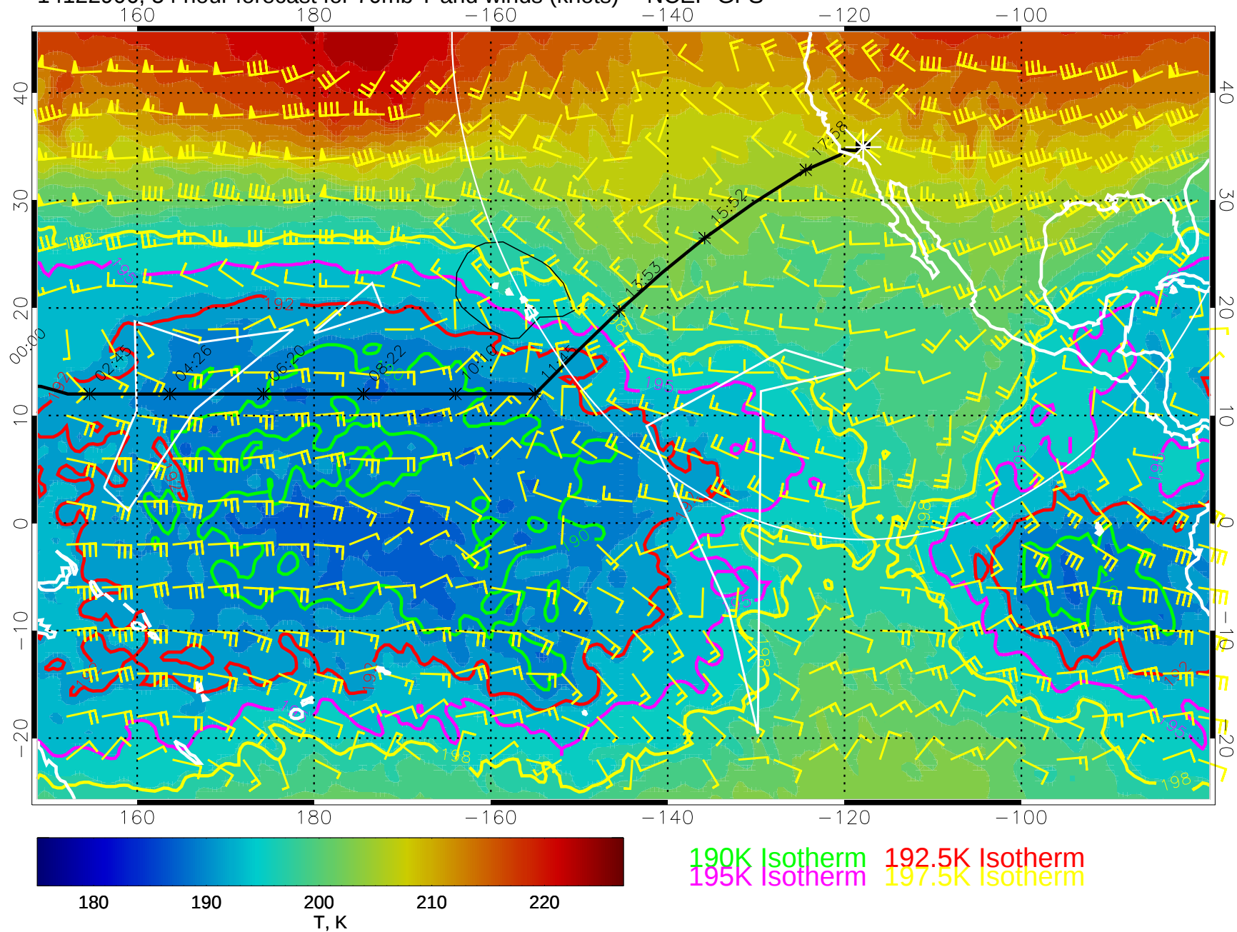
14122906, 54 hour forecast for 70mb T and winds (knots) -- NCEP GFS
