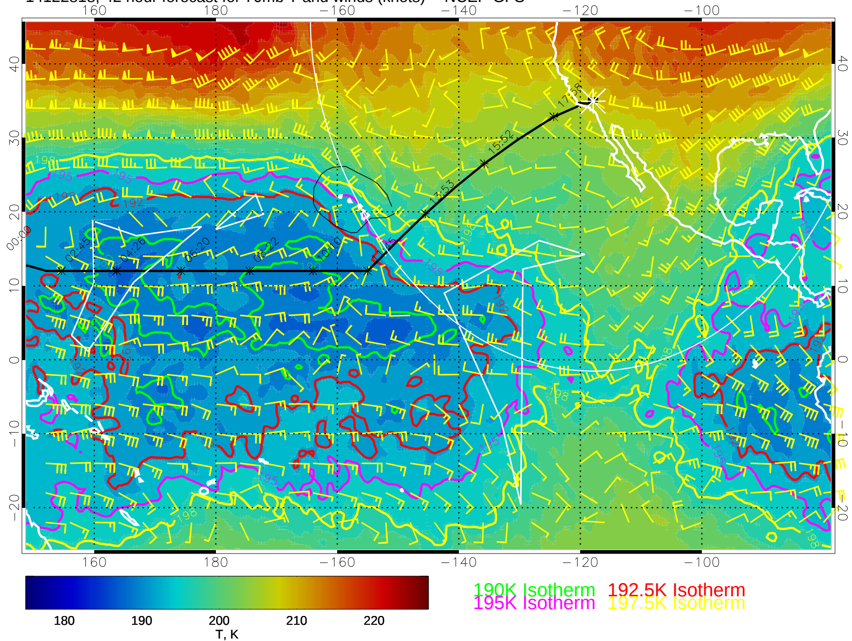
14122818, 42 hour forecast for 70mb T and winds (knots) -- NCEP GFS
