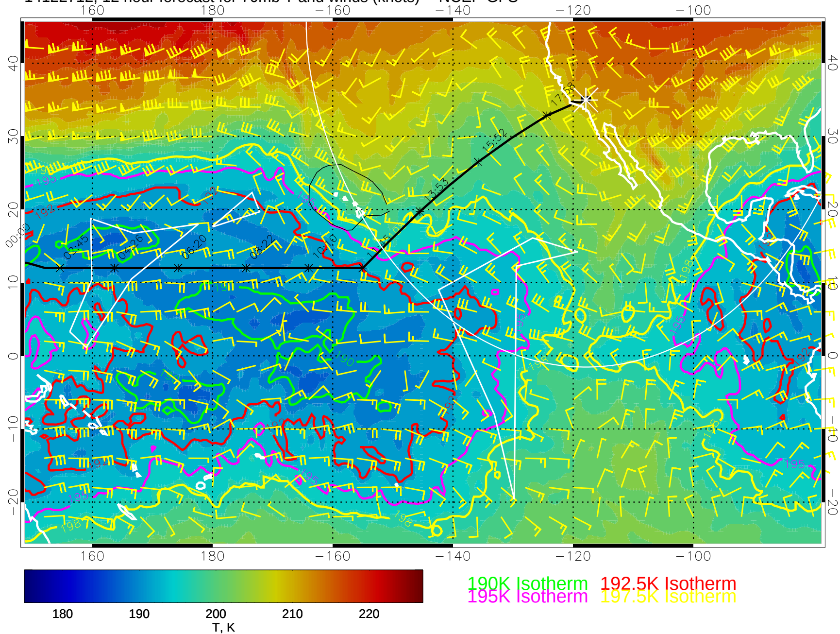
14122712, 12 hour forecast for 70mb T and winds (knots) -- NCEP GFS
