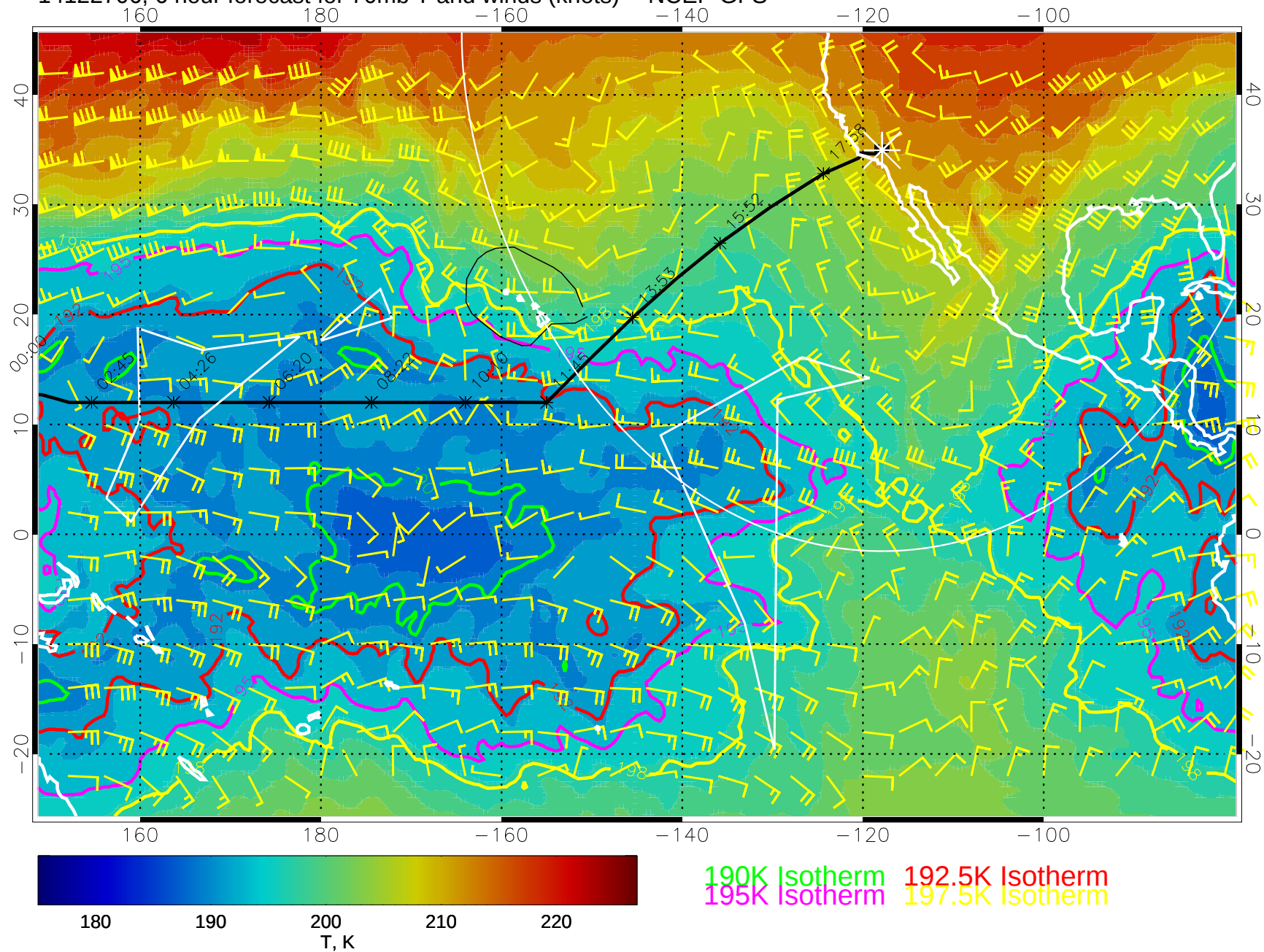
14122706, 6 hour forecast for 70mb T and winds (knots) -- NCEP GFS
