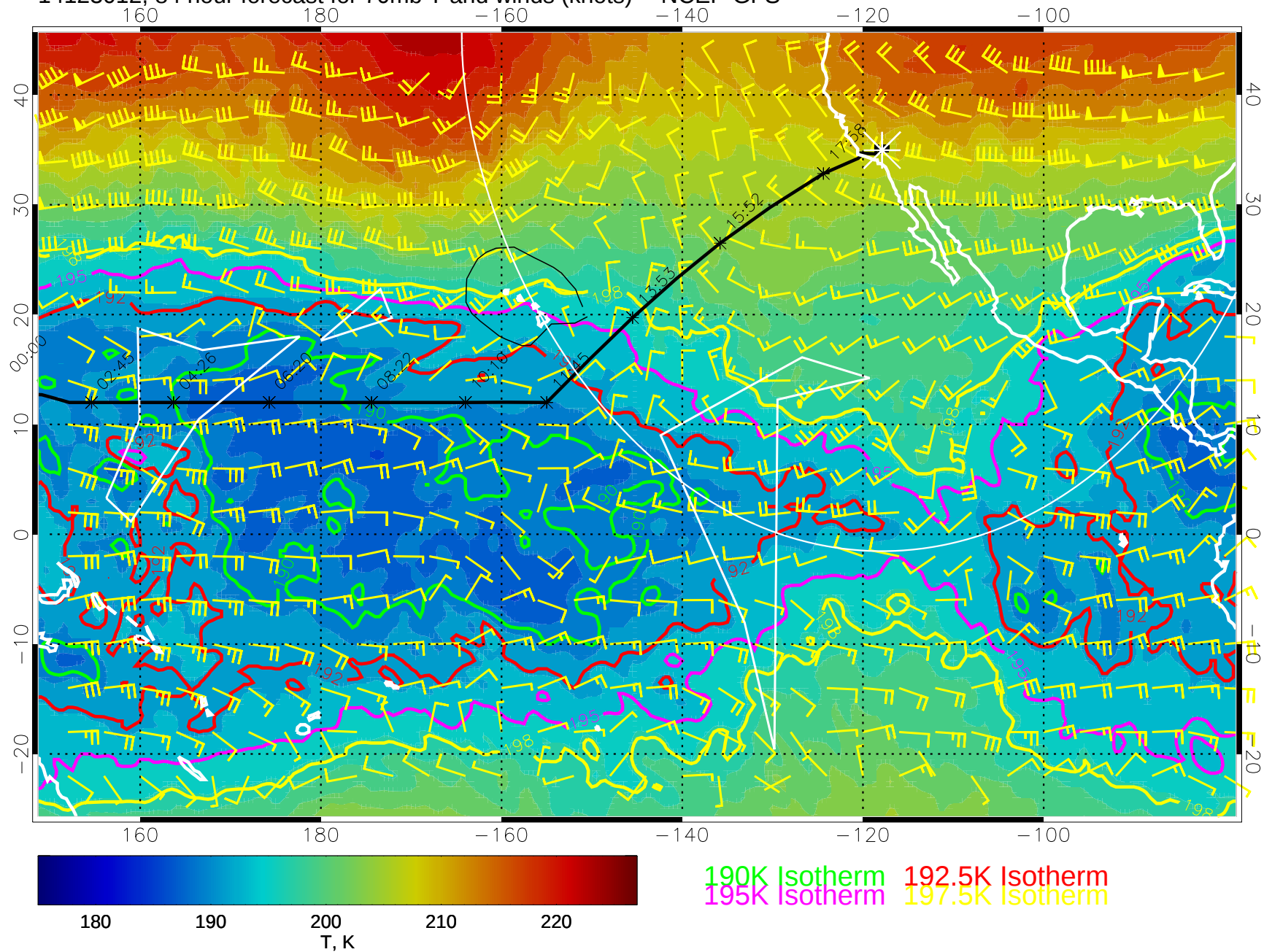
14123012, 84 hour forecast for 70mb T and winds (knots) -- NCEP GFS
