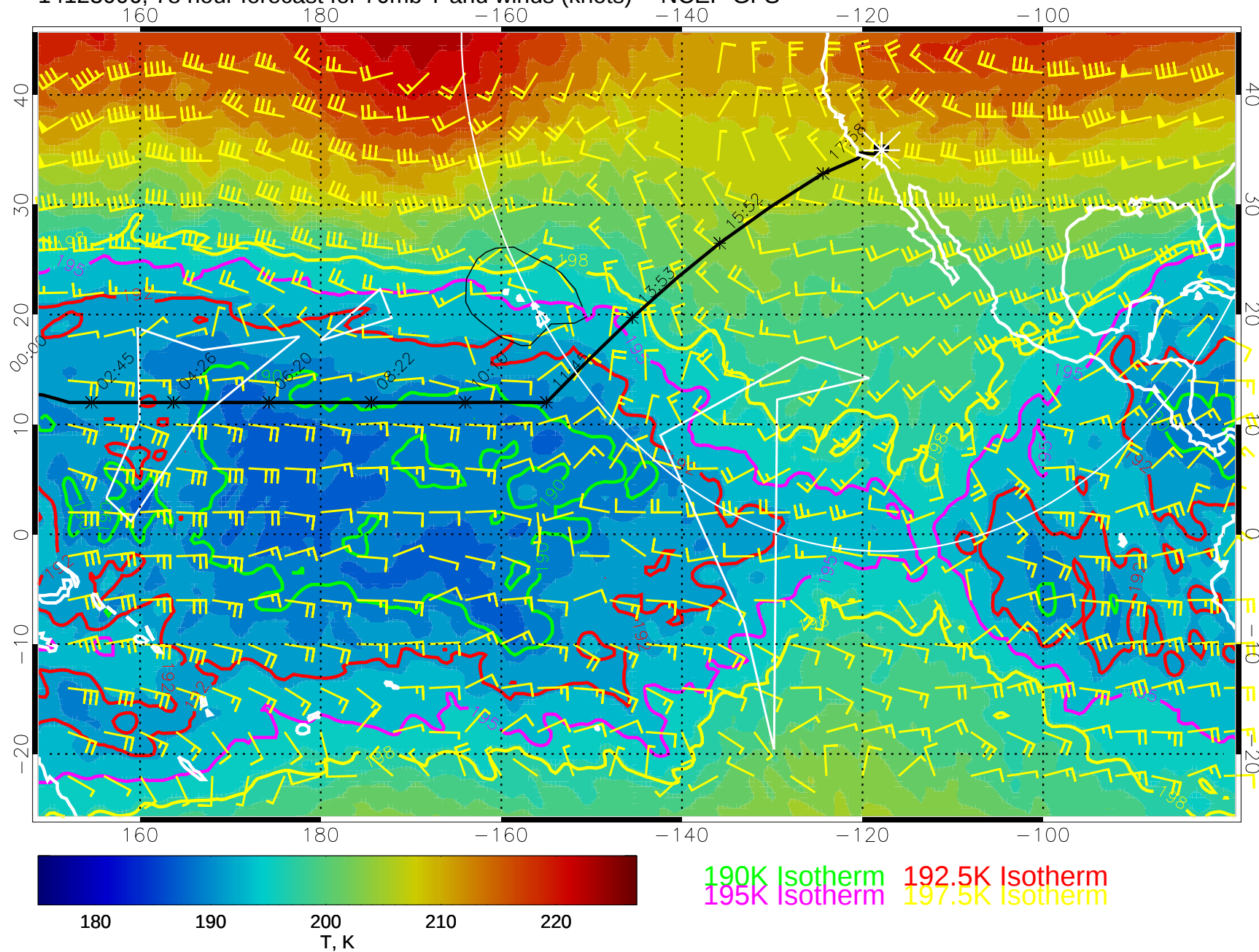
14123006, 78 hour forecast for 70mb T and winds (knots) -- NCEP GFS
