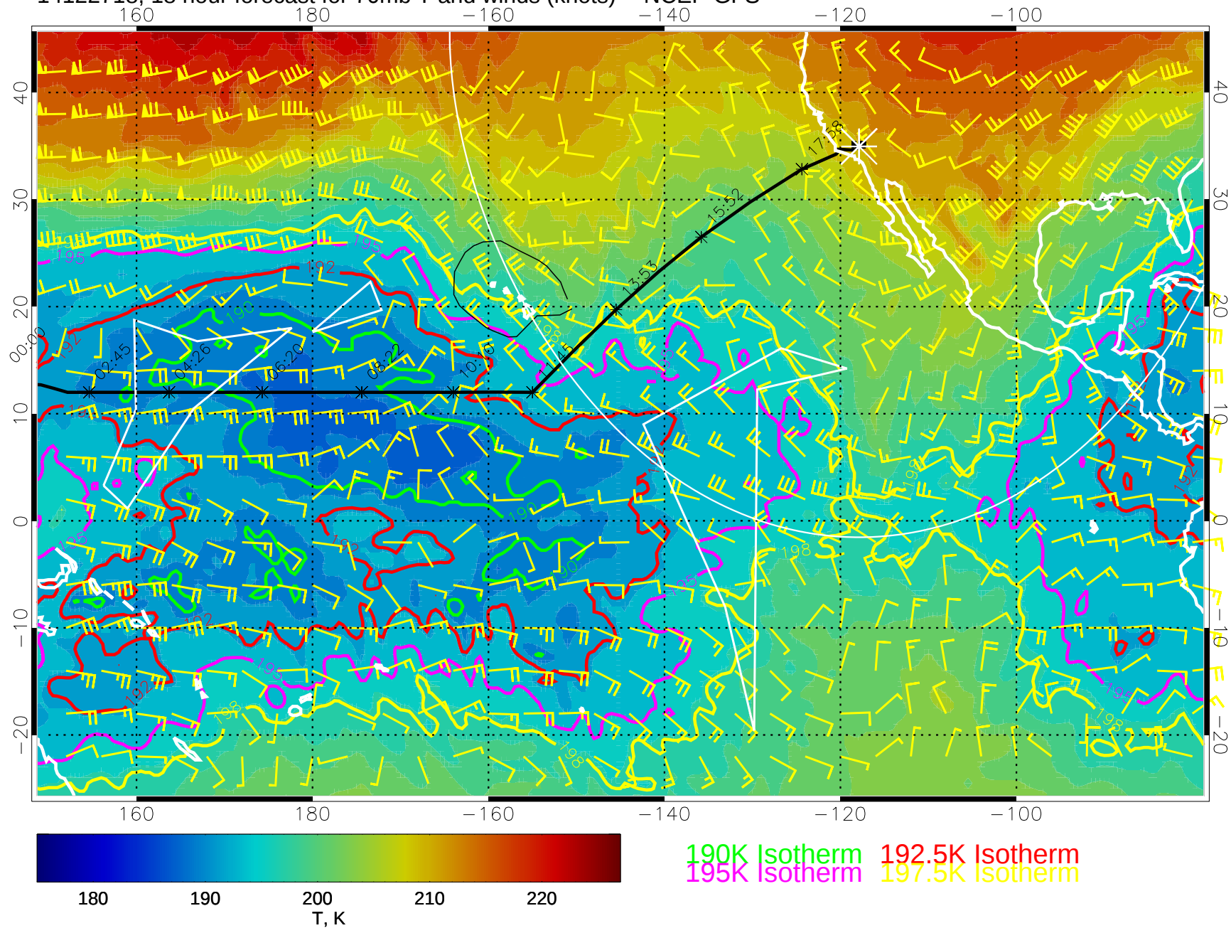
14122718, 18 hour forecast for 70mb T and winds (knots) -- NCEP GFS
