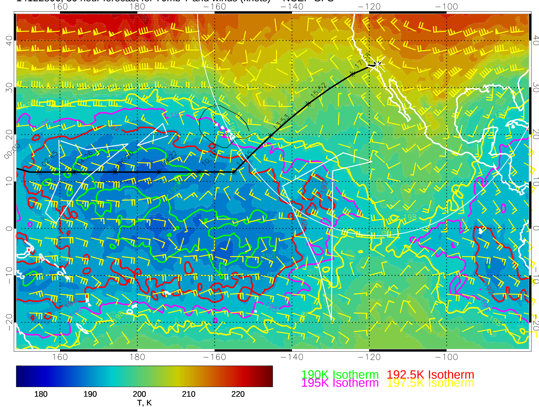
14122806, 30 hour forecast for 70mb T and winds (knots) -- NCEP GFS
