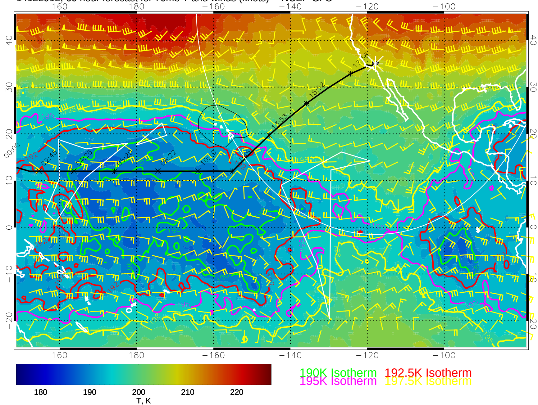
14122912, 60 hour forecast for 70mb T and winds (knots) -- NCEP GFS
