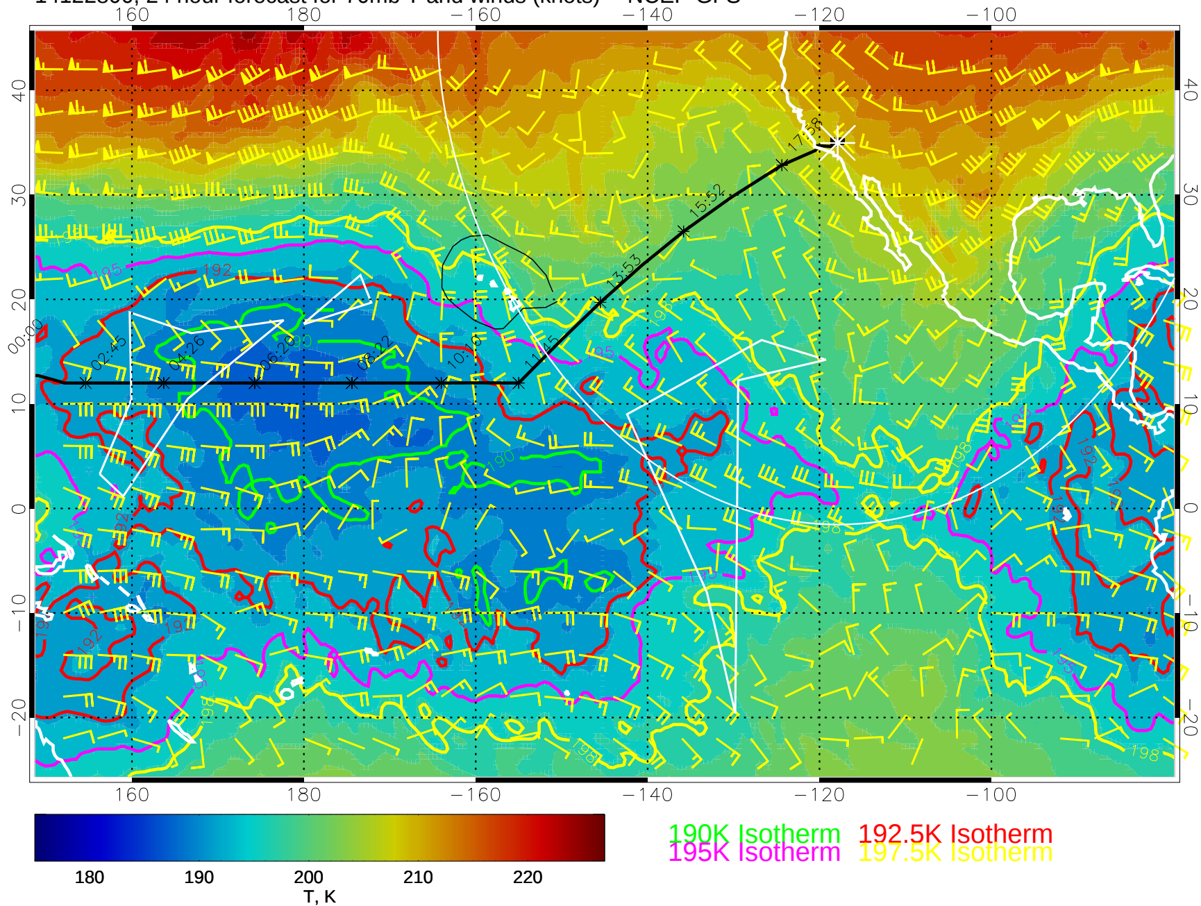
14122800, 24 hour forecast for 70mb T and winds (knots) -- NCEP GFS
