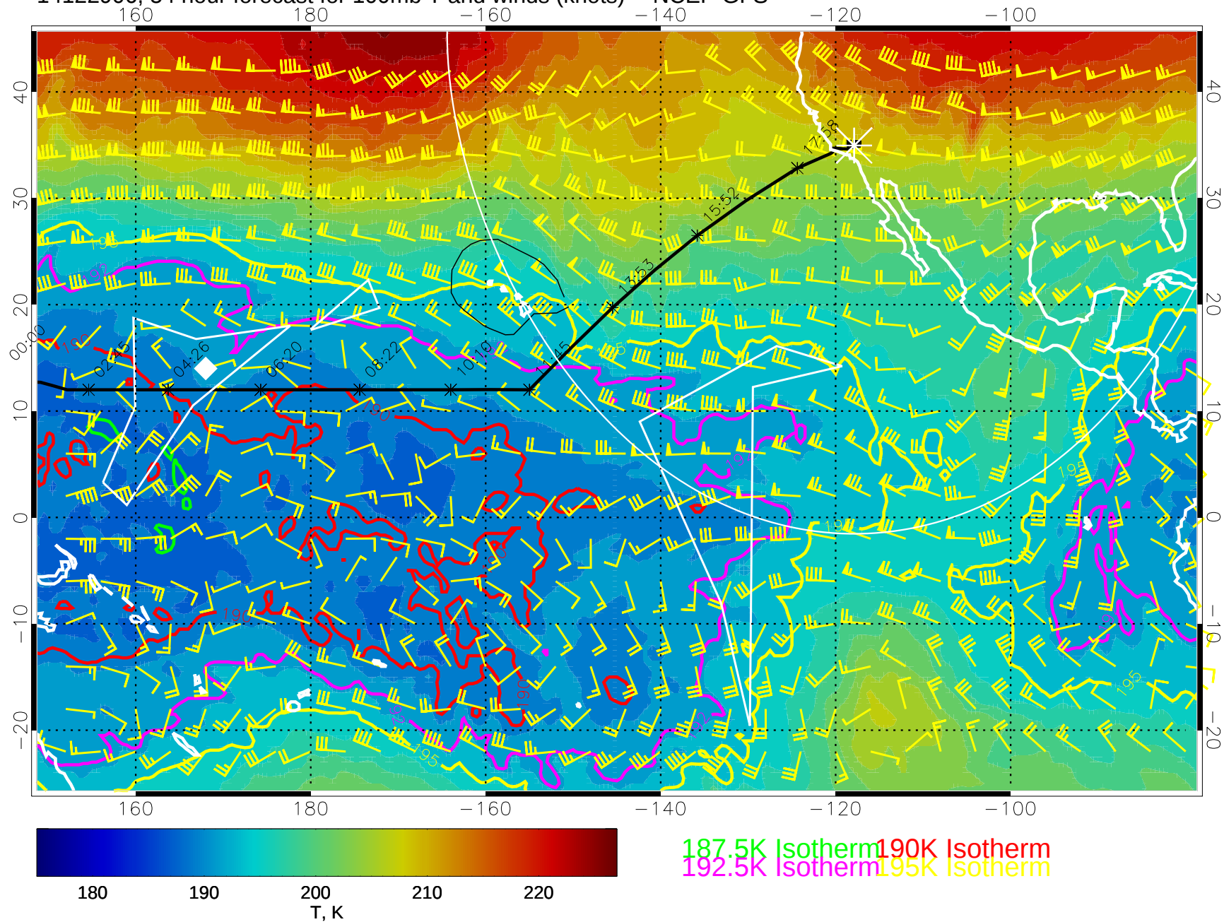
14122906, 54 hour forecast for 100mb T and winds (knots) -- NCEP GFS
