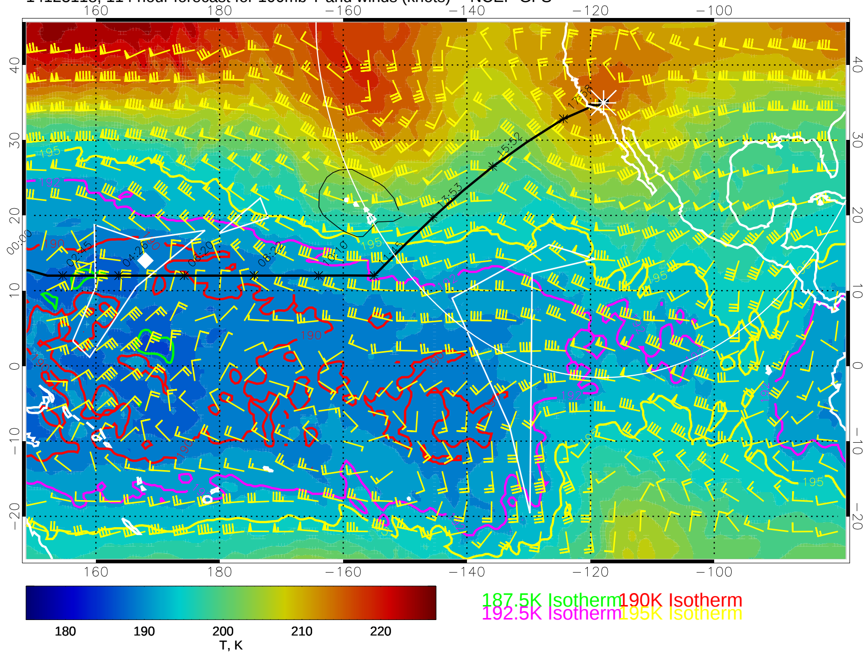
14123118, 114 hour forecast for 100mb T and winds (knots) -- NCEP GFS
