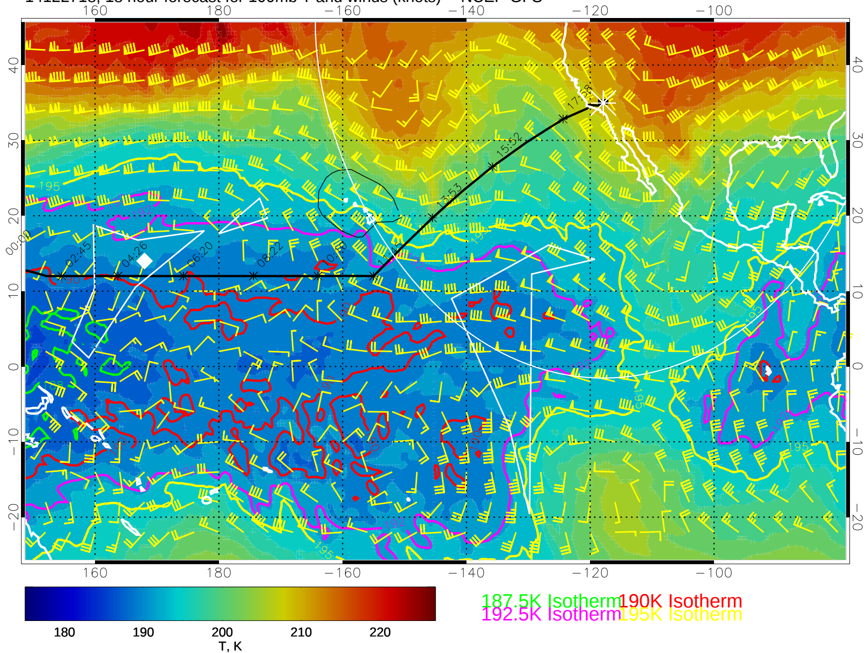
14122718, 18 hour forecast for 100mb T and winds (knots) -- NCEP GFS
