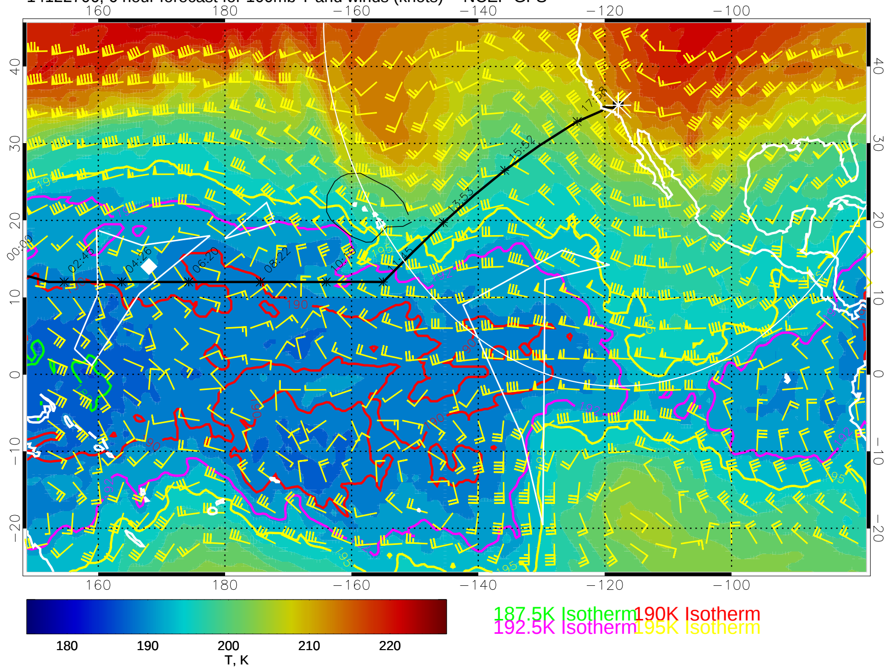
14122706, 6 hour forecast for 100mb T and winds (knots) -- NCEP GFS
