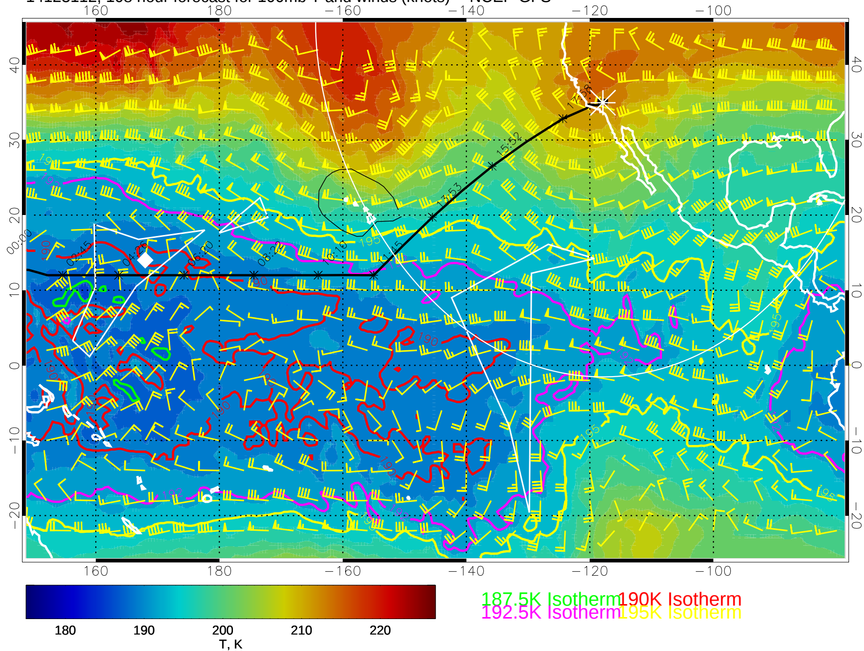
14123112, 108 hour forecast for 100mb T and winds (knots) -- NCEP GFS
