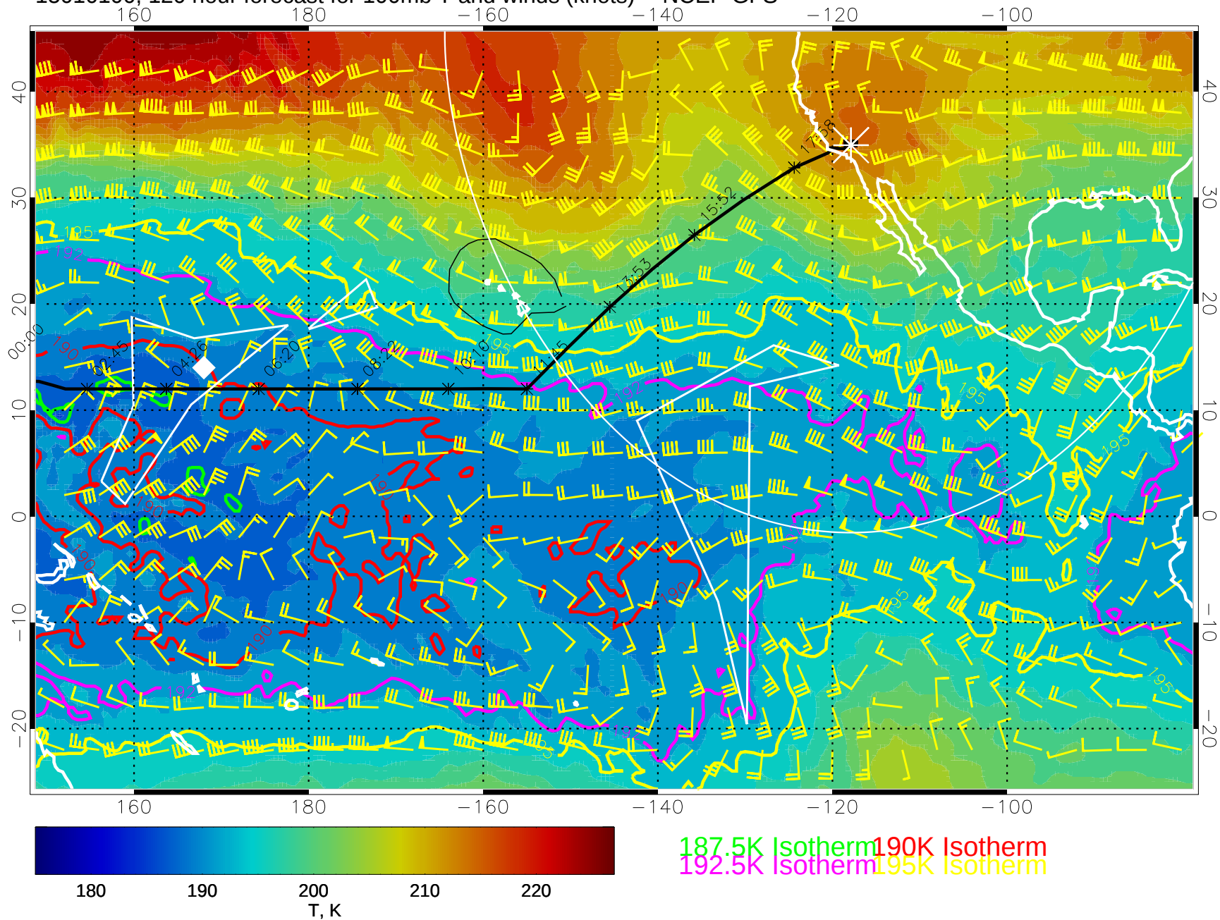
15010100, 120 hour forecast for 100mb T and winds (knots) -- NCEP GFS
