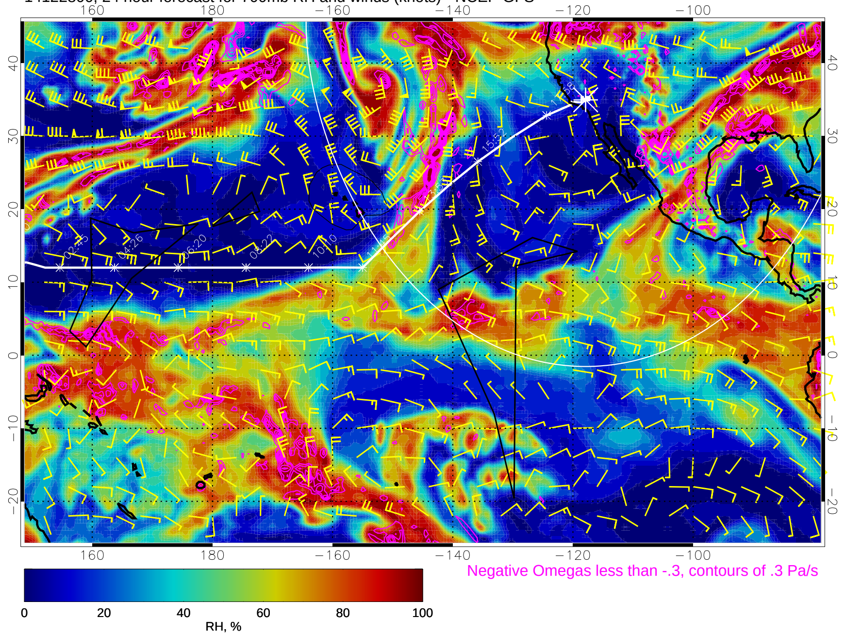
14122800, 24 hour forecast for 700mb RH and winds (knots) - NCEP GFS
