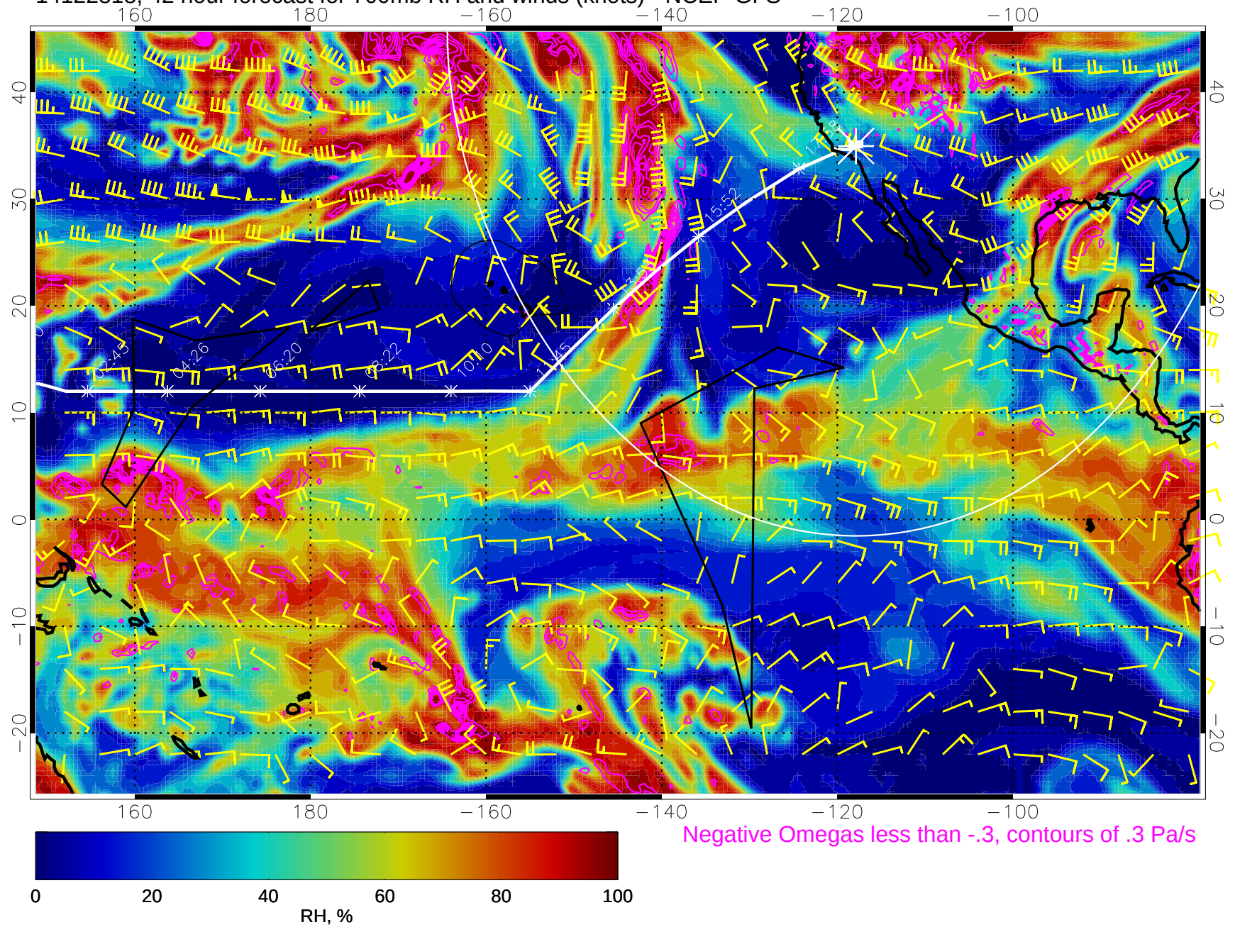
14122818, 42 hour forecast for 700mb RH and winds (knots) - NCEP GFS
