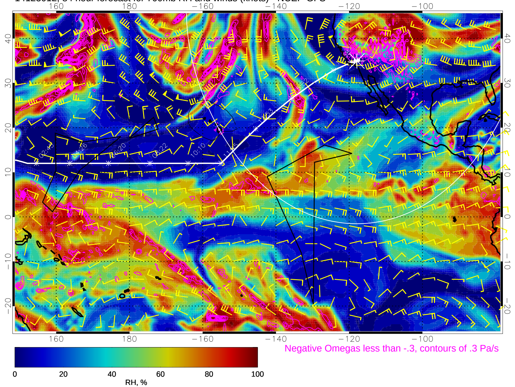
14123012, 84 hour forecast for 700mb RH and winds (knots) - NCEP GFS
