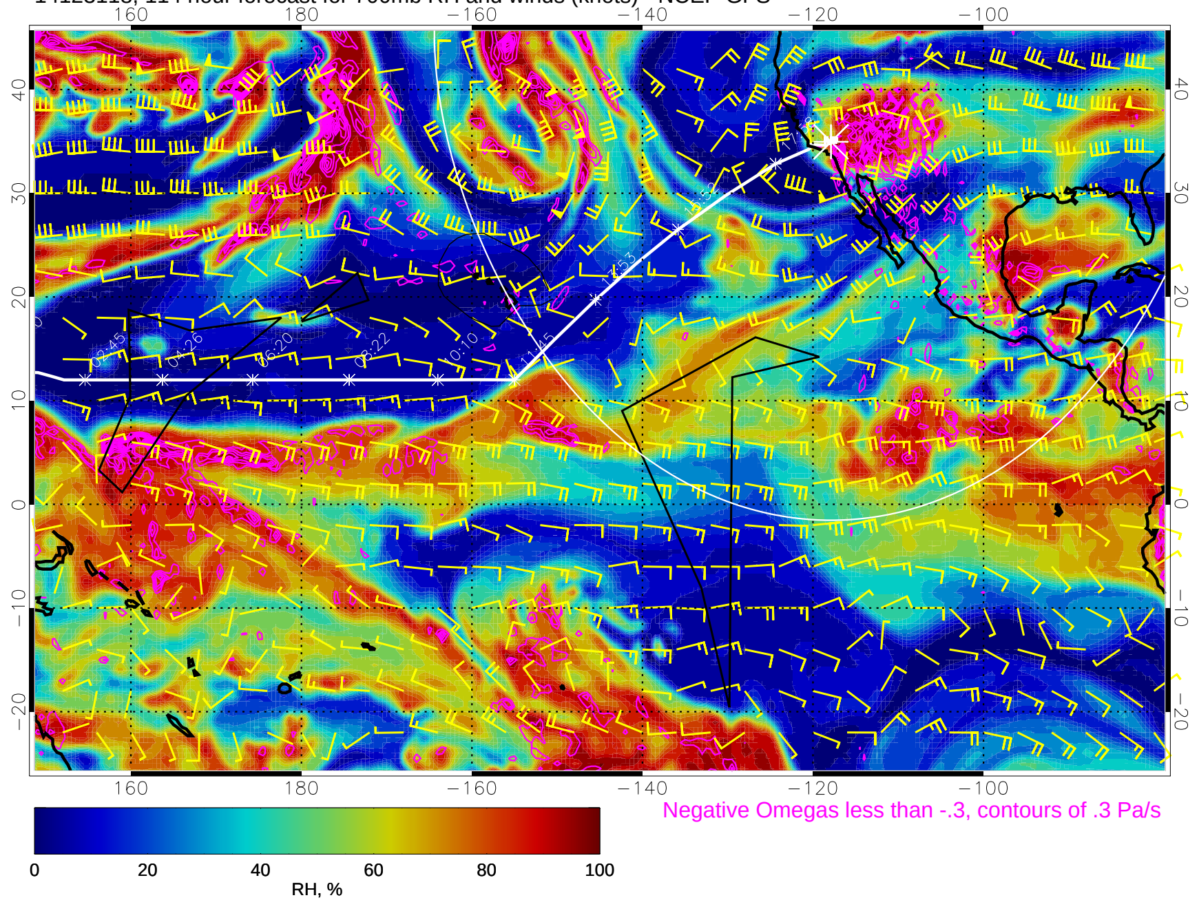
14123118, 114 hour forecast for 700mb RH and winds (knots) - NCEP GFS
