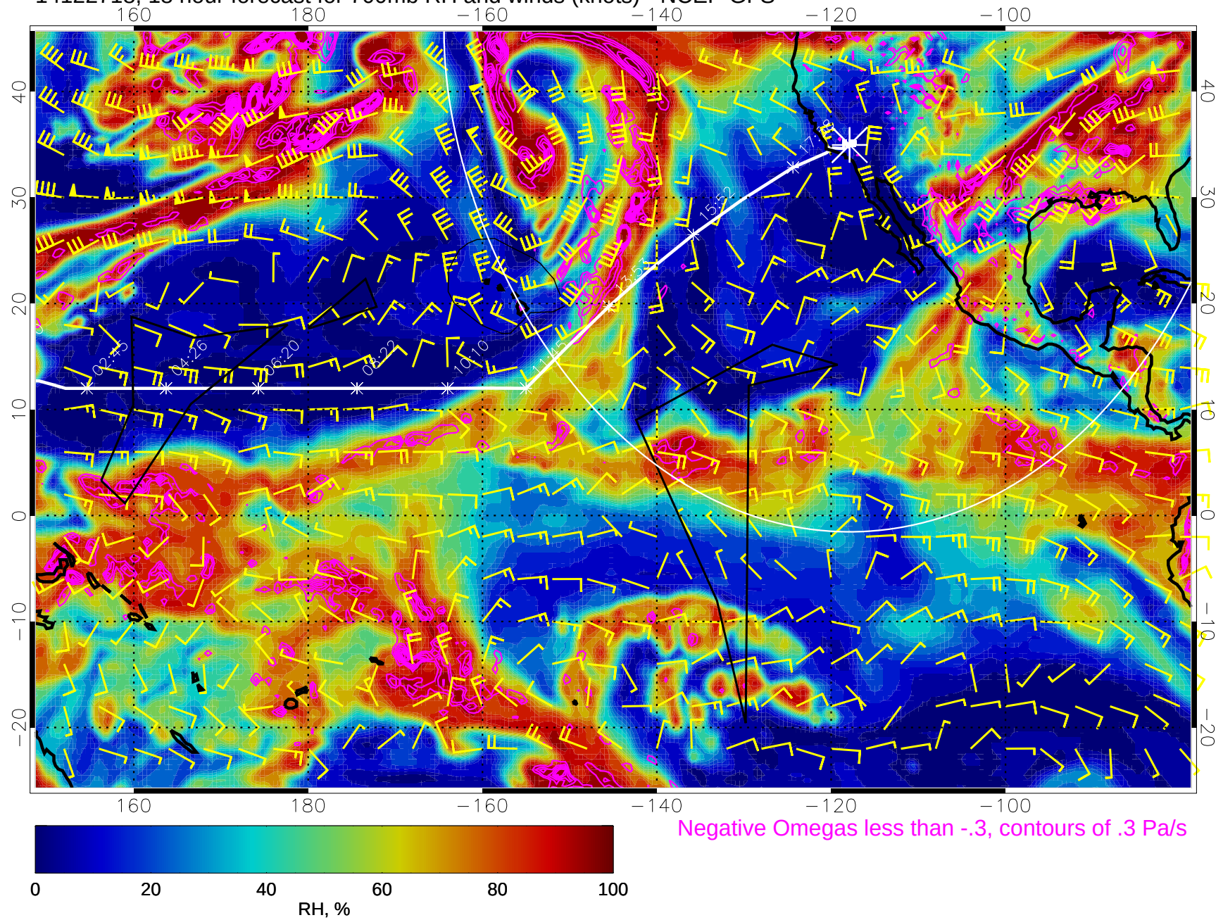
14122718, 18 hour forecast for 700mb RH and winds (knots) - NCEP GFS
