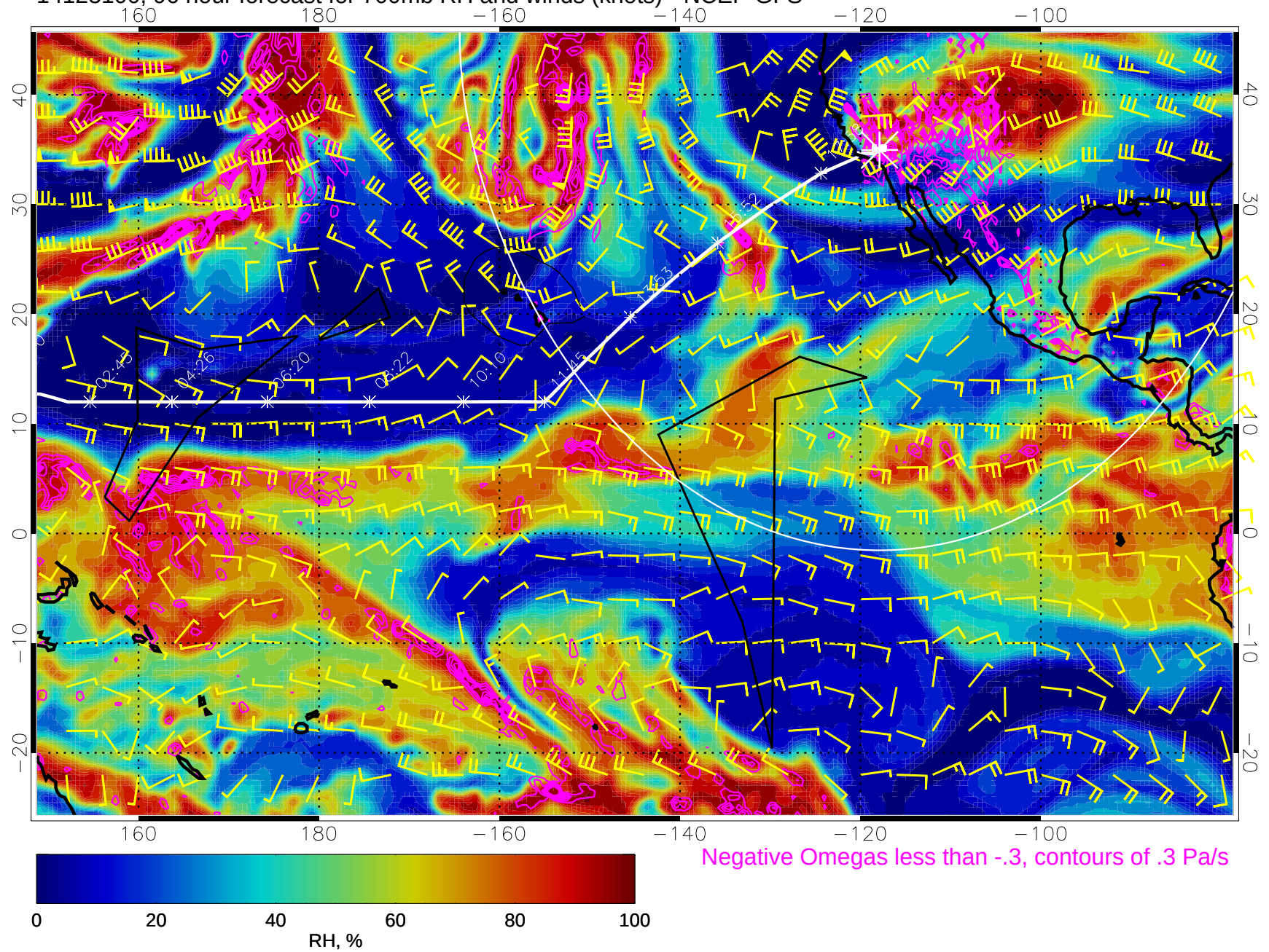
14123100, 96 hour forecast for 700mb RH and winds (knots) - NCEP GFS
