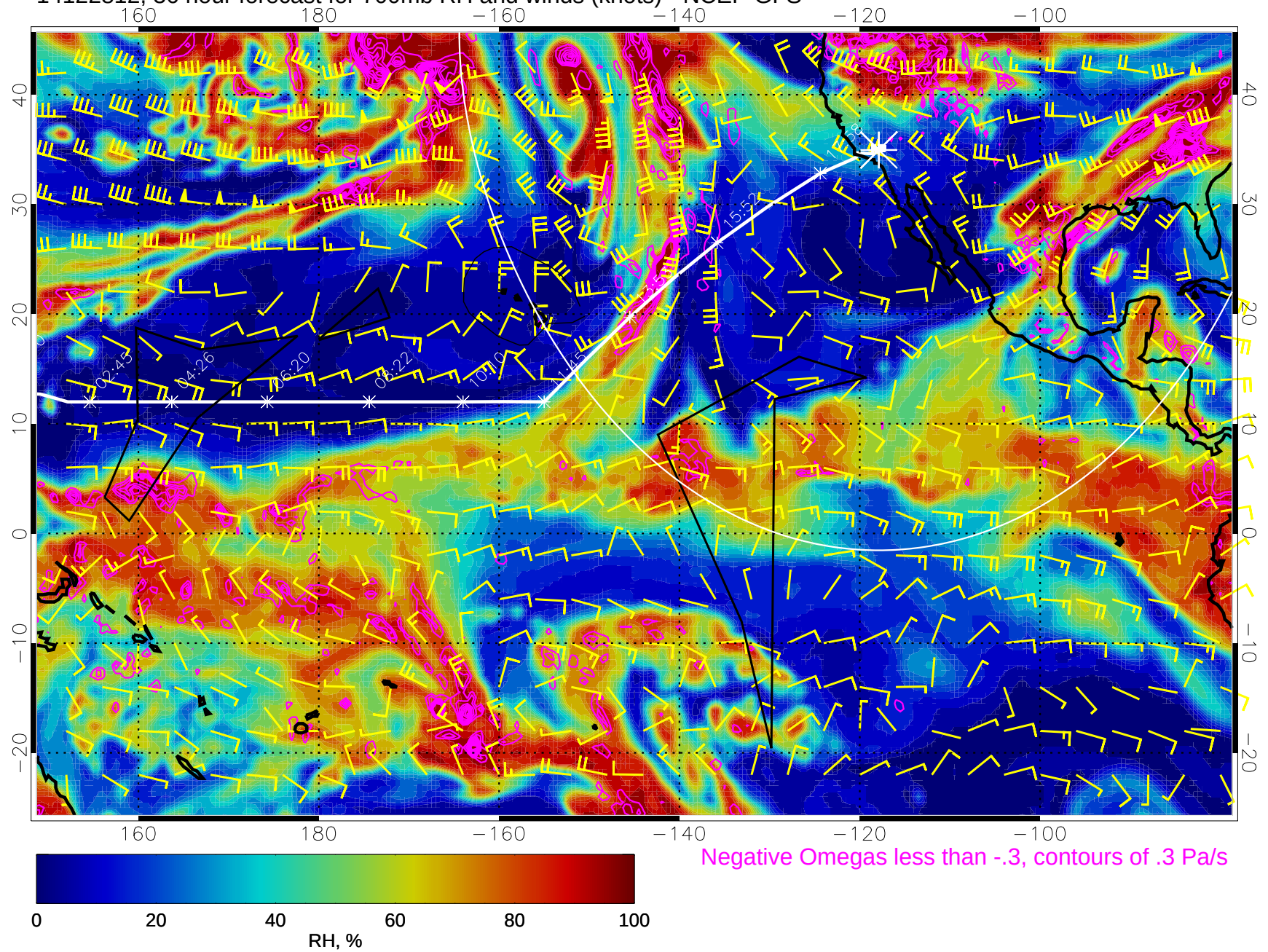
14122812, 36 hour forecast for 700mb RH and winds (knots) - NCEP GFS
