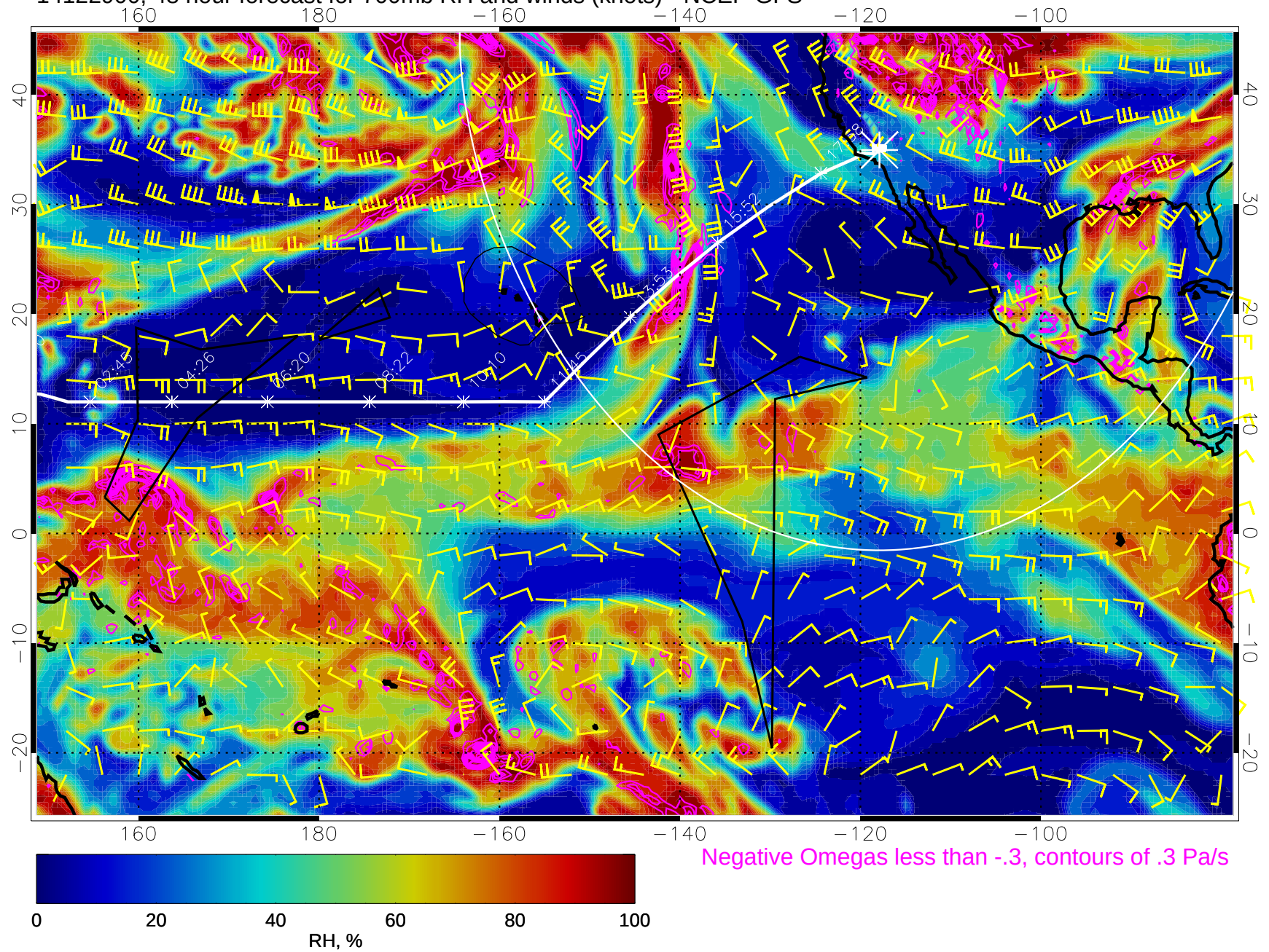
14122900, 48 hour forecast for 700mb RH and winds (knots) - NCEP GFS
