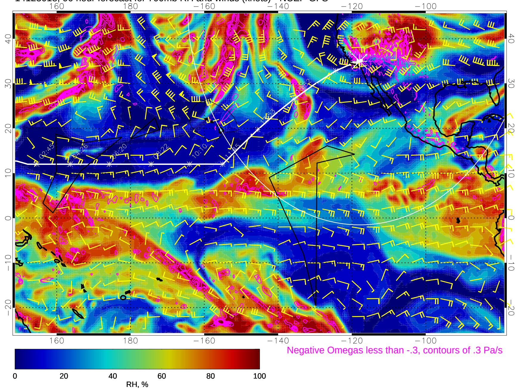
14123018, 90 hour forecast for 700mb RH and winds (knots) - NCEP GFS
