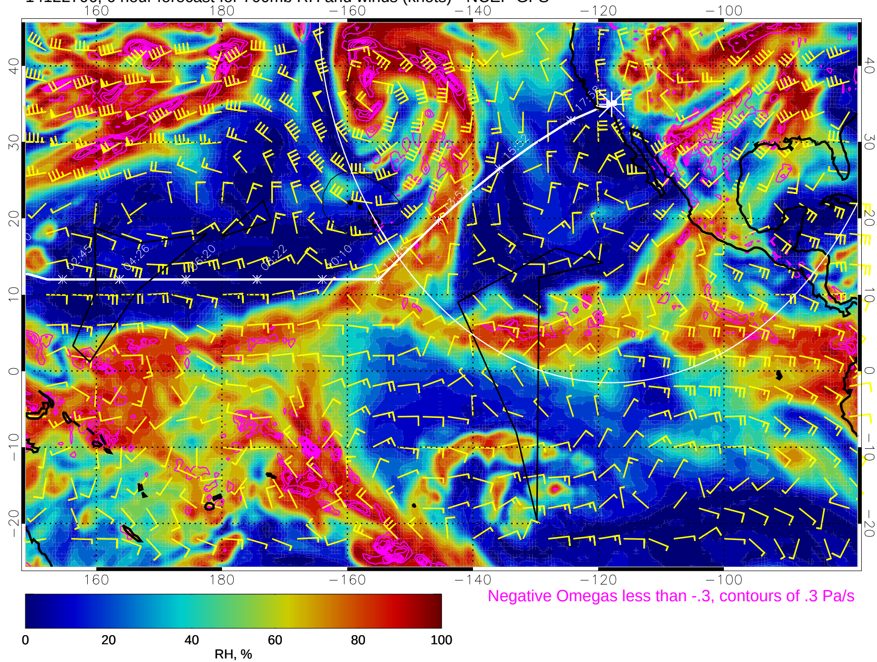
14122706, 6 hour forecast for 700mb RH and winds (knots) - NCEP GFS
