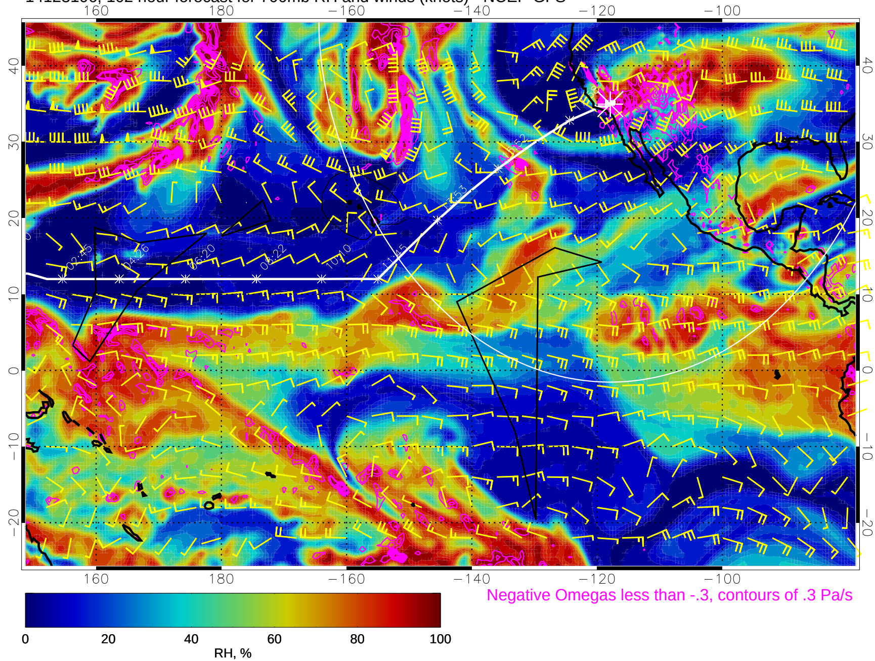
14123106, 102 hour forecast for 700mb RH and winds (knots) - NCEP GFS
