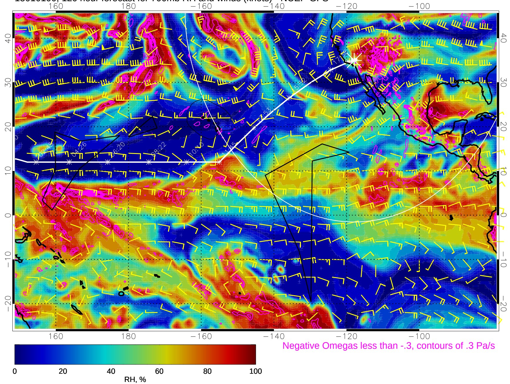
15010100, 120 hour forecast for 700mb RH and winds (knots) - NCEP GFS
