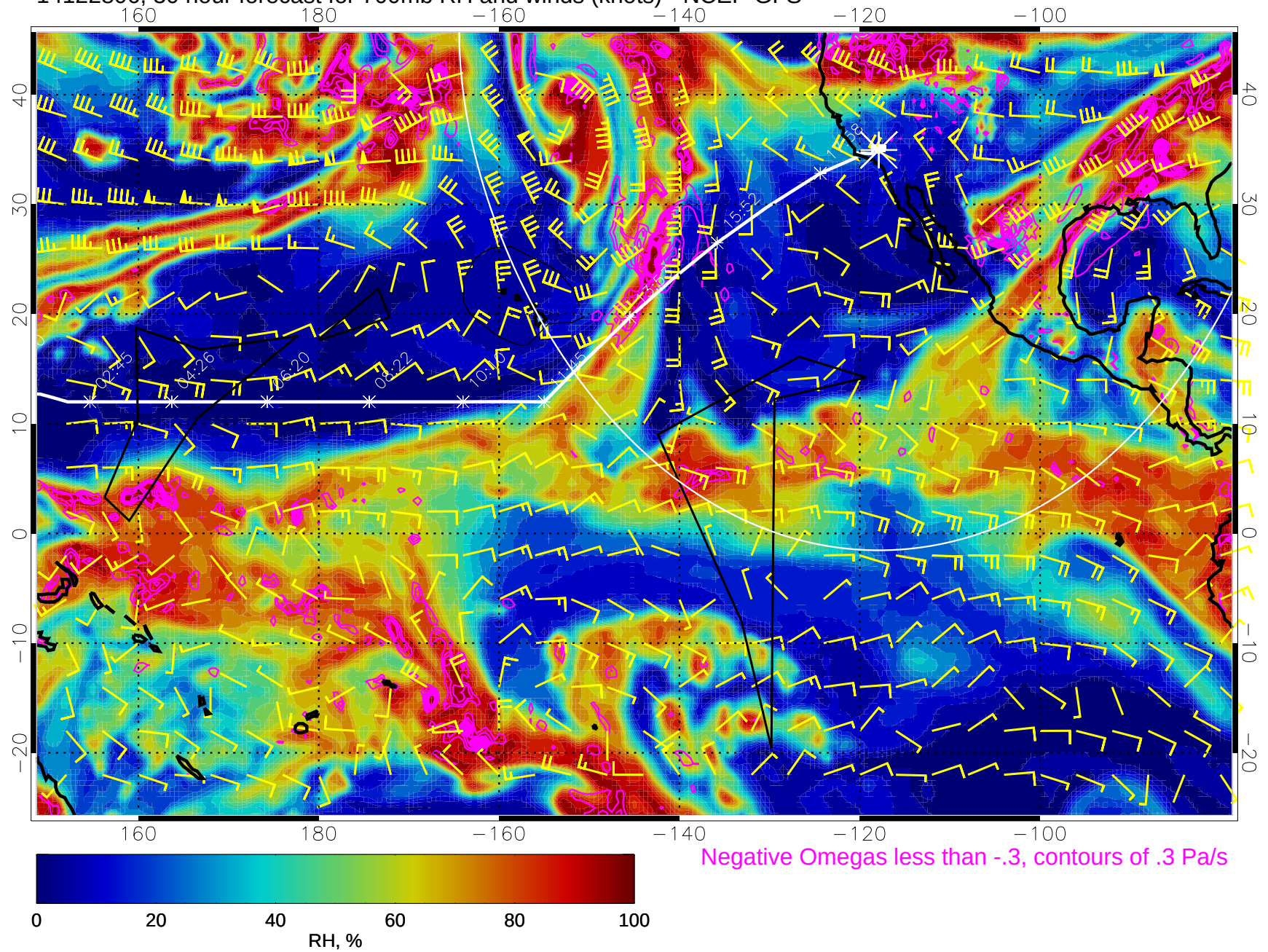
14122806, 30 hour forecast for 700mb RH and winds (knots) - NCEP GFS
