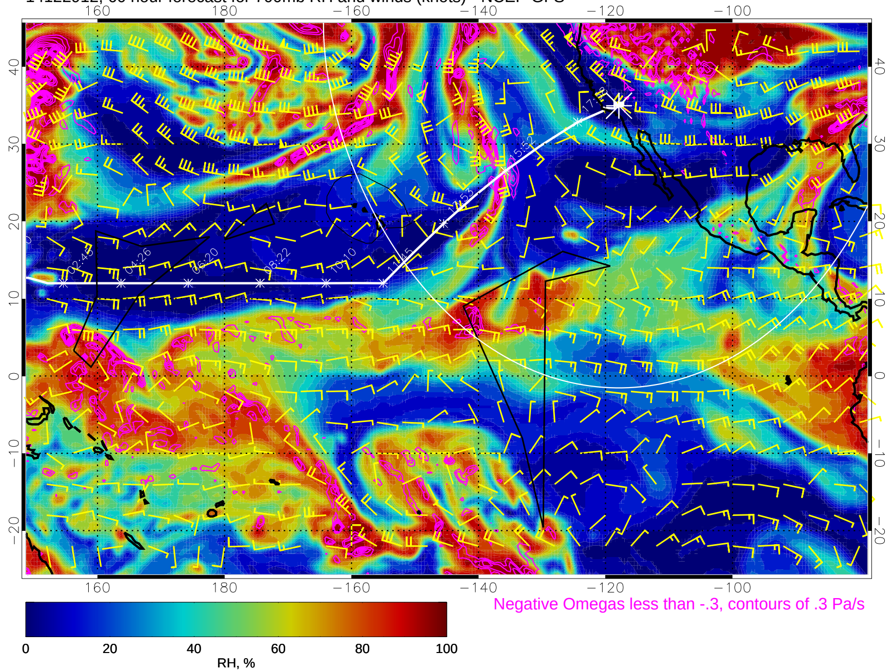
14122912, 60 hour forecast for 700mb RH and winds (knots) - NCEP GFS
