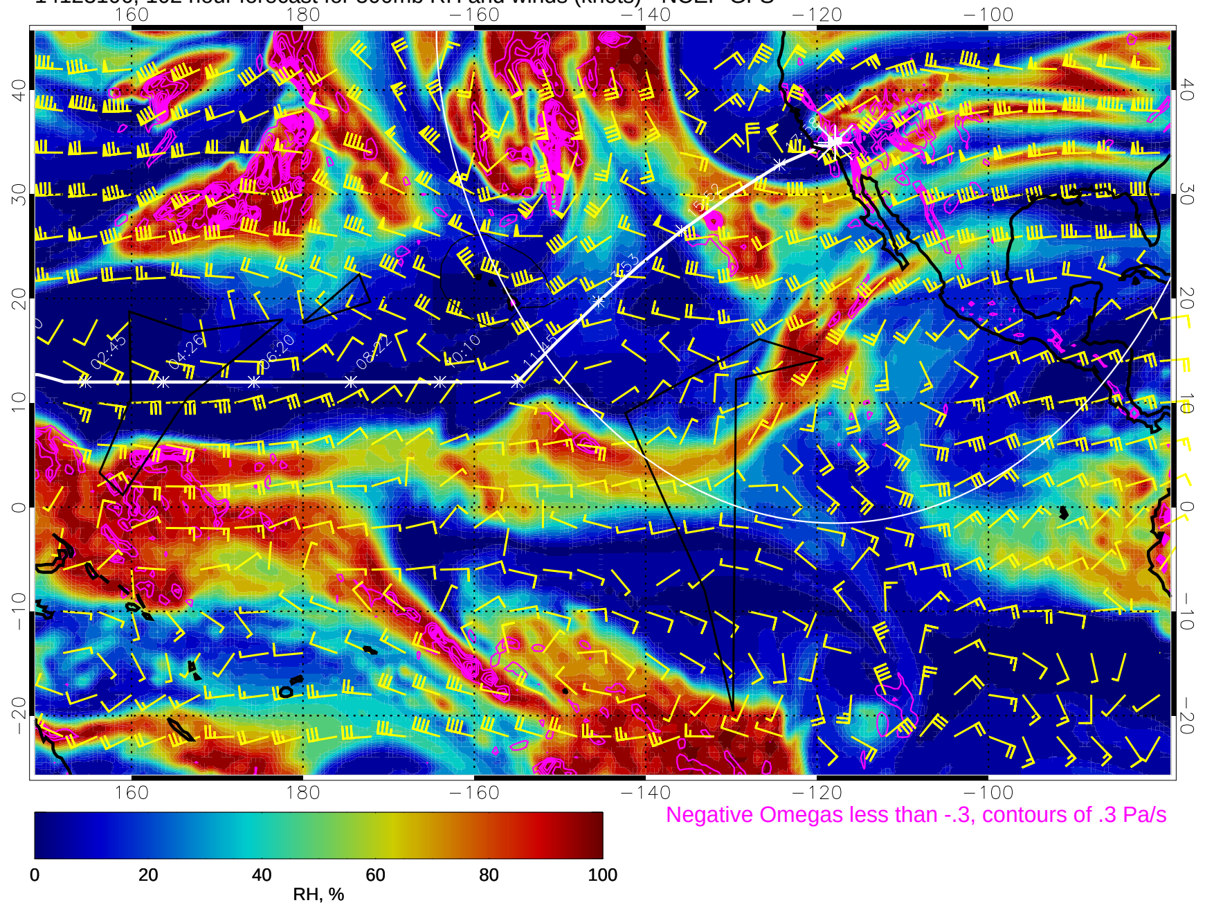
14123106, 102 hour forecast for 500mb RH and winds (knots) - NCEP GFS
