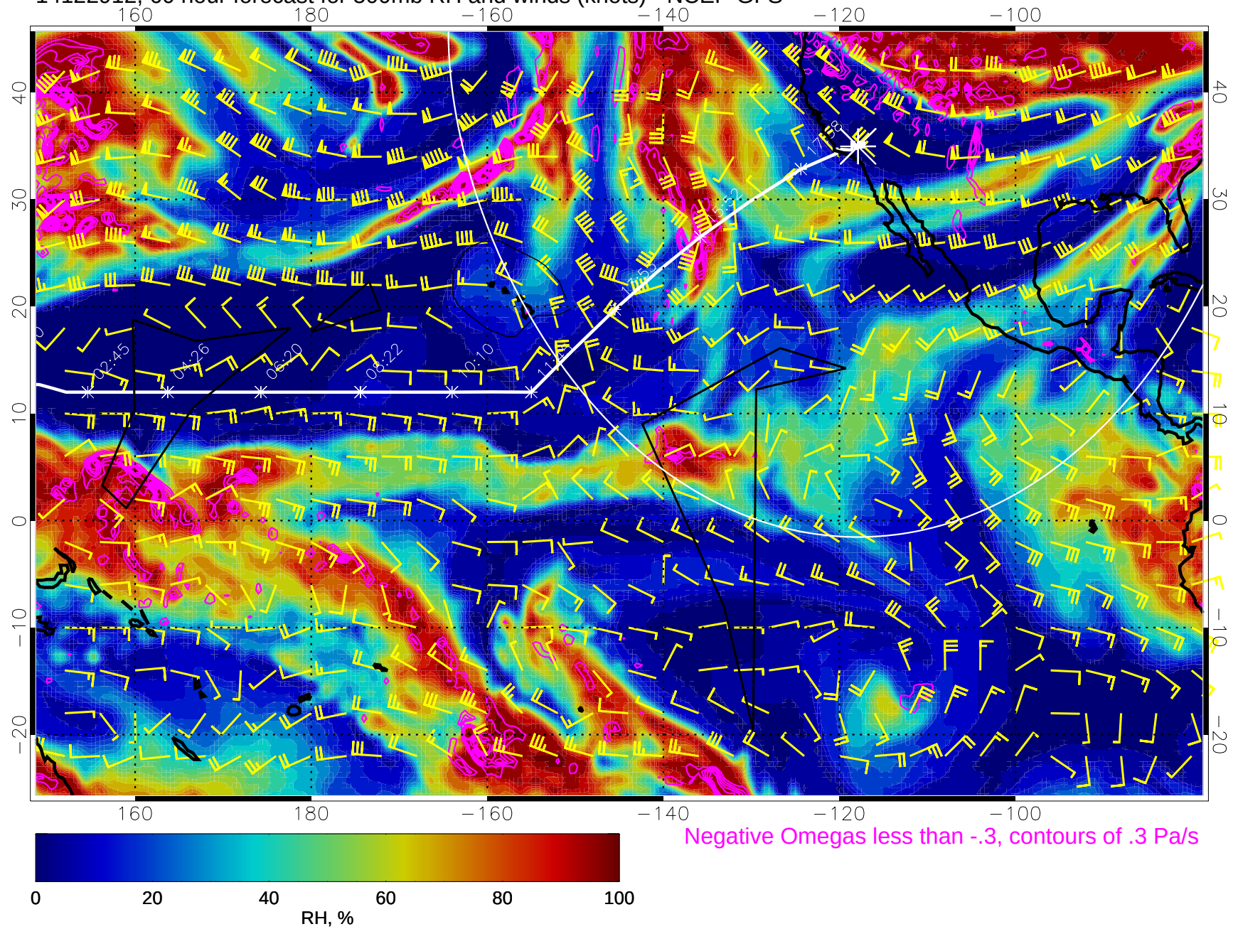
14122912, 60 hour forecast for 500mb RH and winds (knots) - NCEP GFS
