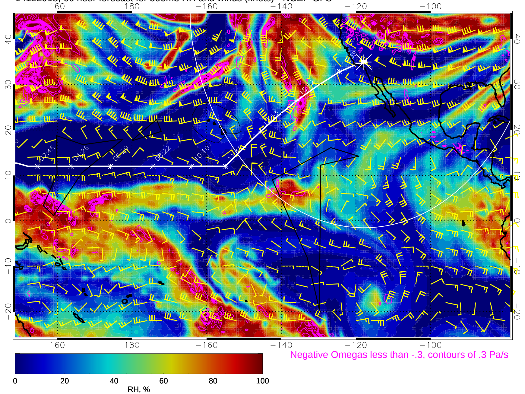
14122918, 66 hour forecast for 500mb RH and winds (knots) - NCEP GFS
