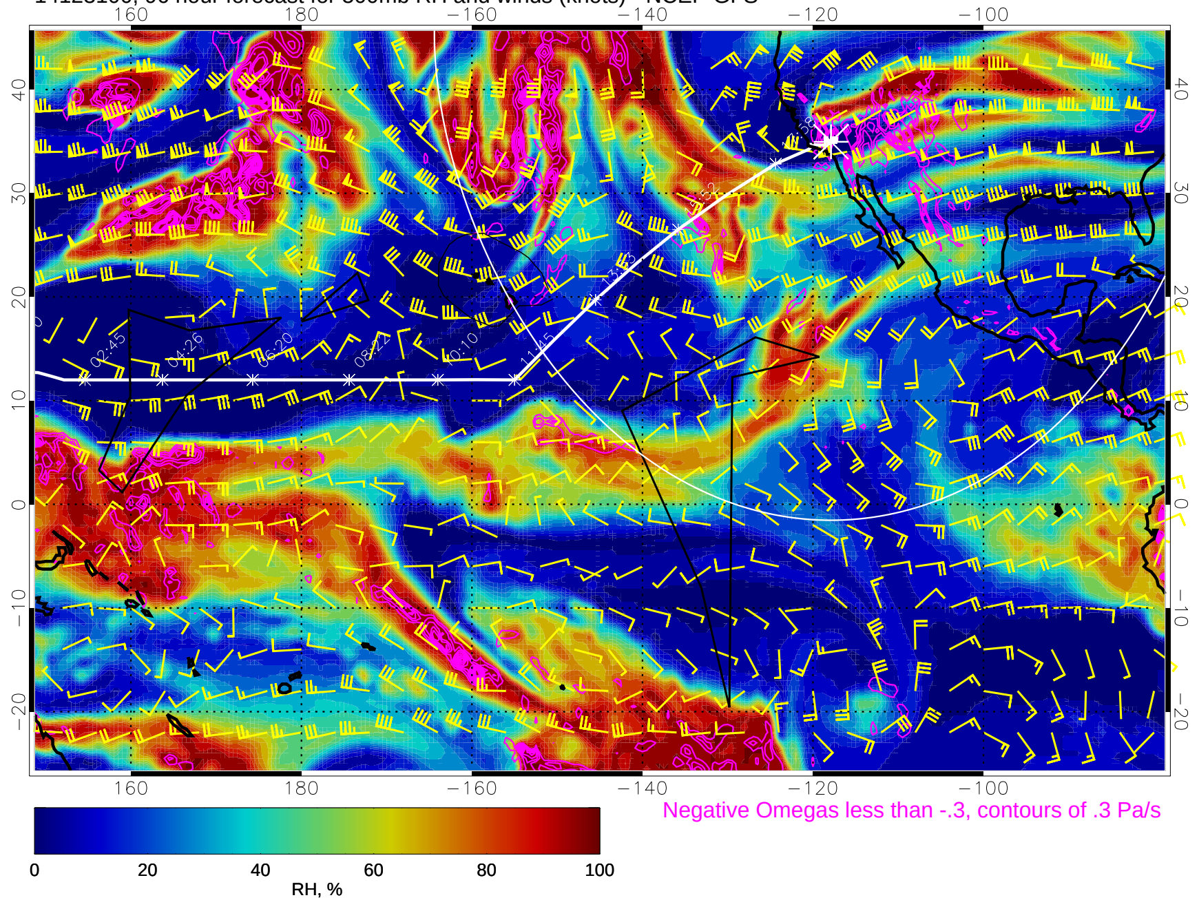
14123100, 96 hour forecast for 500mb RH and winds (knots) - NCEP GFS
