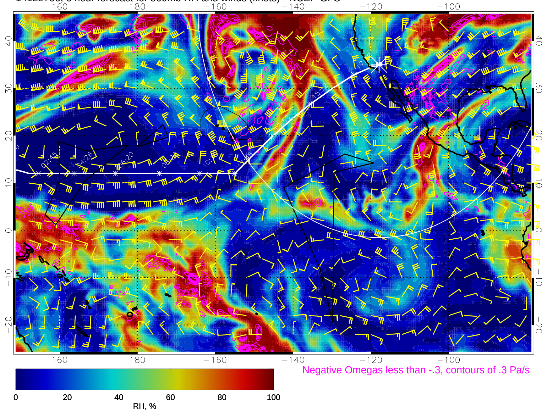
14122706, 6 hour forecast for 500mb RH and winds (knots) - NCEP GFS
