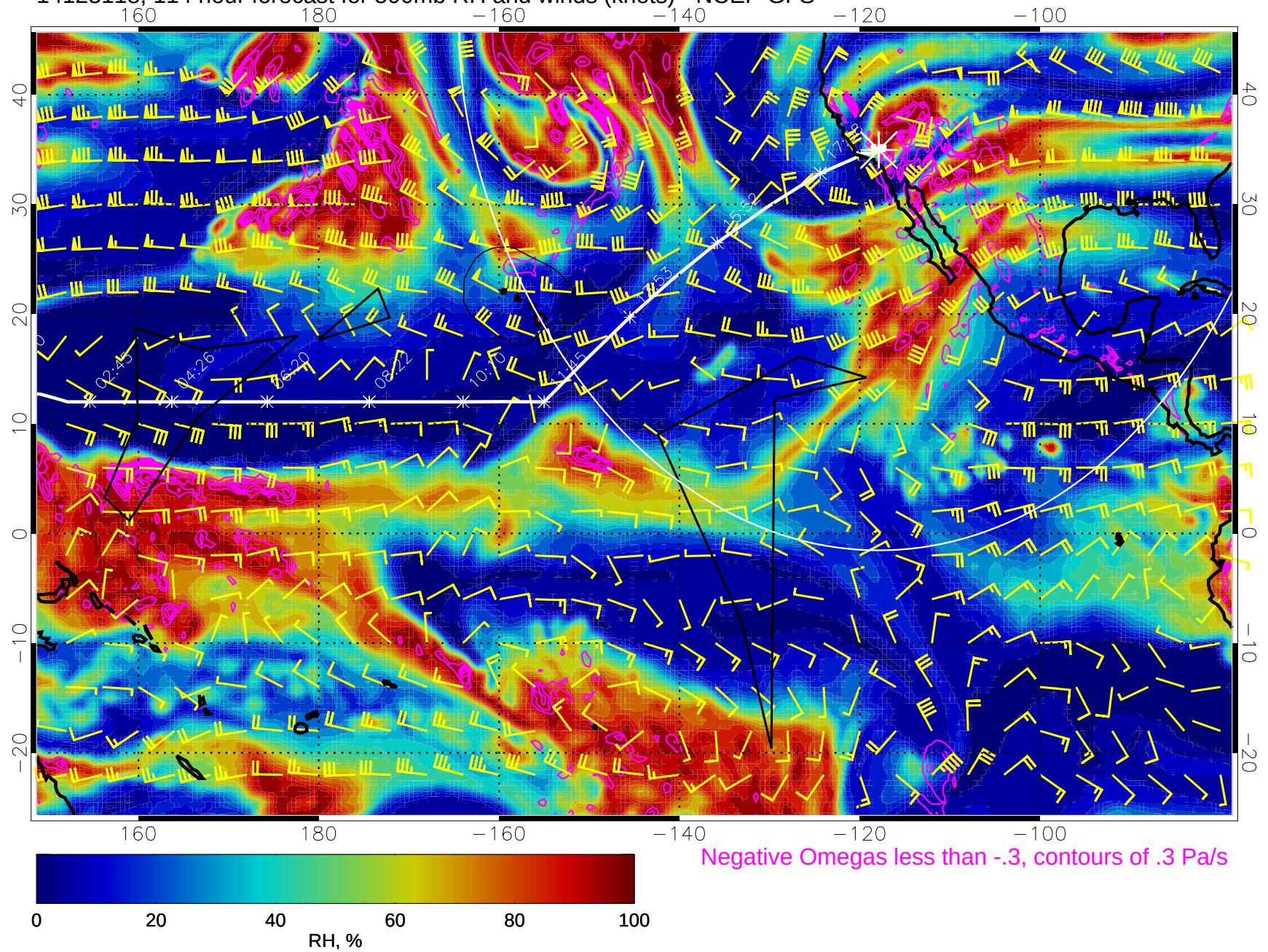
14123118, 114 hour forecast for 500mb RH and winds (knots) - NCEP GFS
