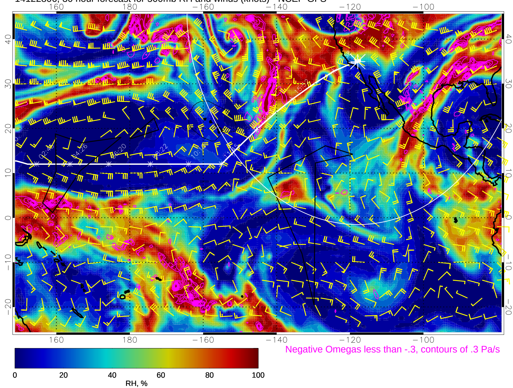
14122806, 30 hour forecast for 500mb RH and winds (knots) - NCEP GFS
