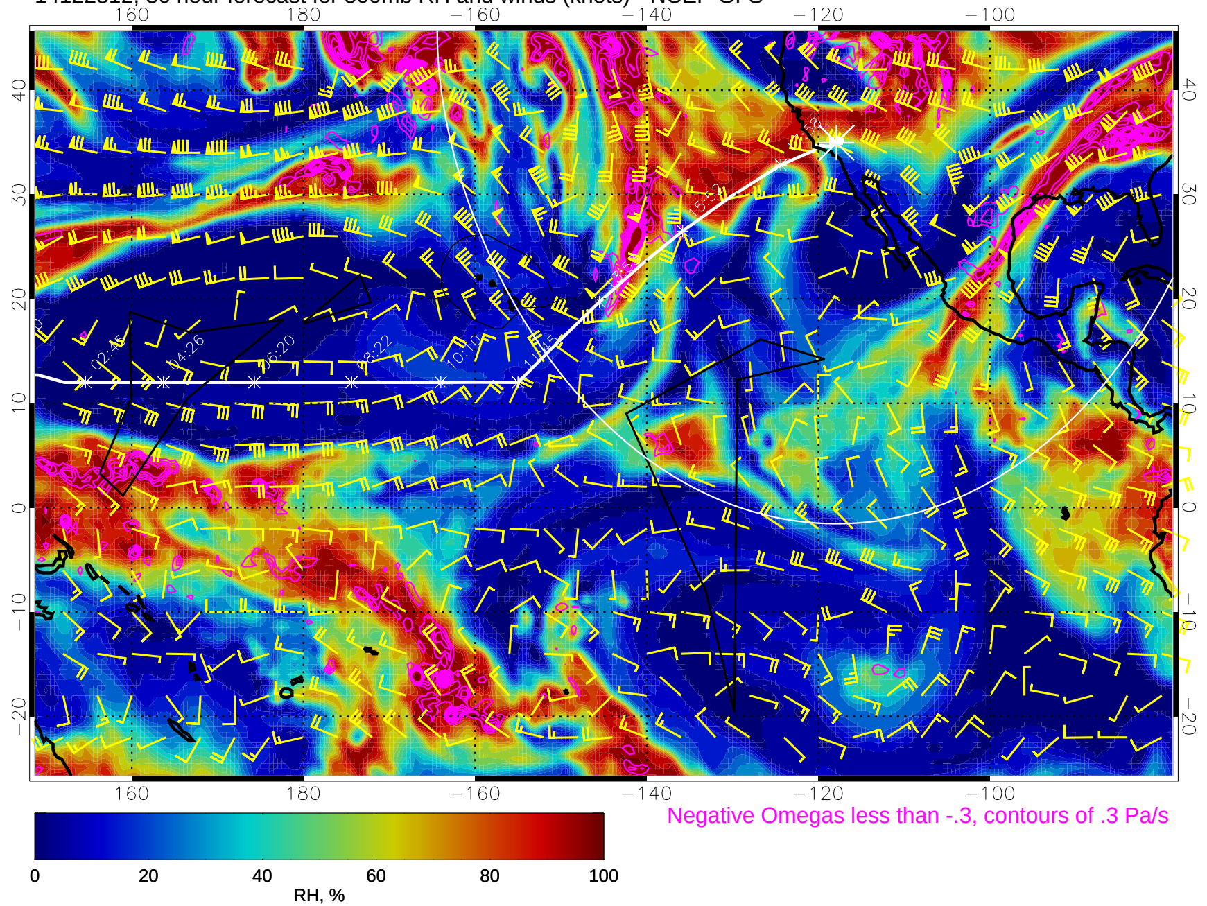
14122812, 36 hour forecast for 500mb RH and winds (knots) - NCEP GFS
