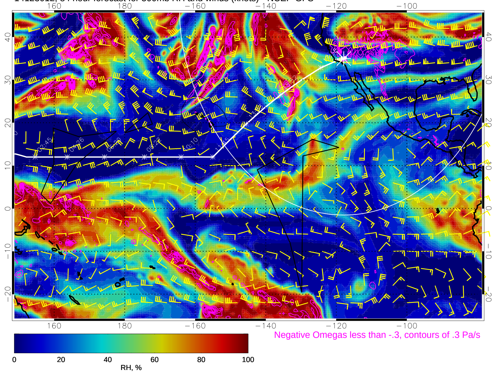
14123012, 84 hour forecast for 500mb RH and winds (knots) - NCEP GFS
