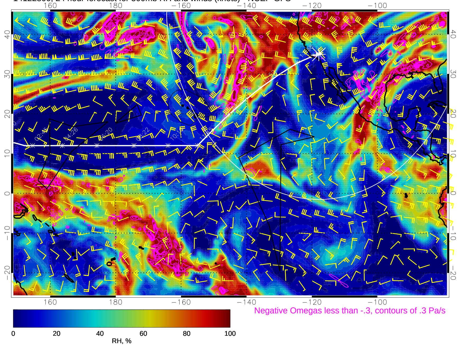
14122800, 24 hour forecast for 500mb RH and winds (knots) - NCEP GFS
