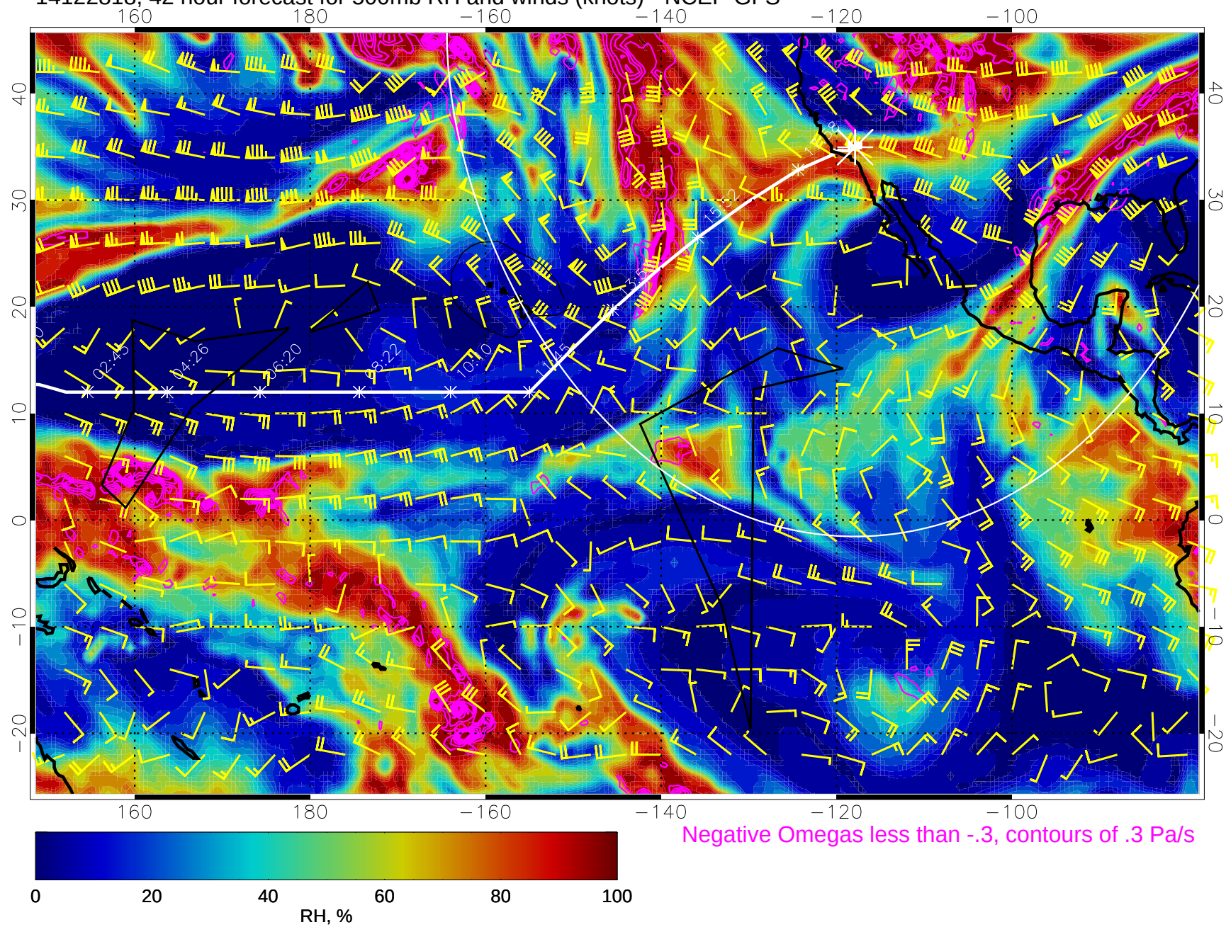
14122818, 42 hour forecast for 500mb RH and winds (knots) - NCEP GFS
