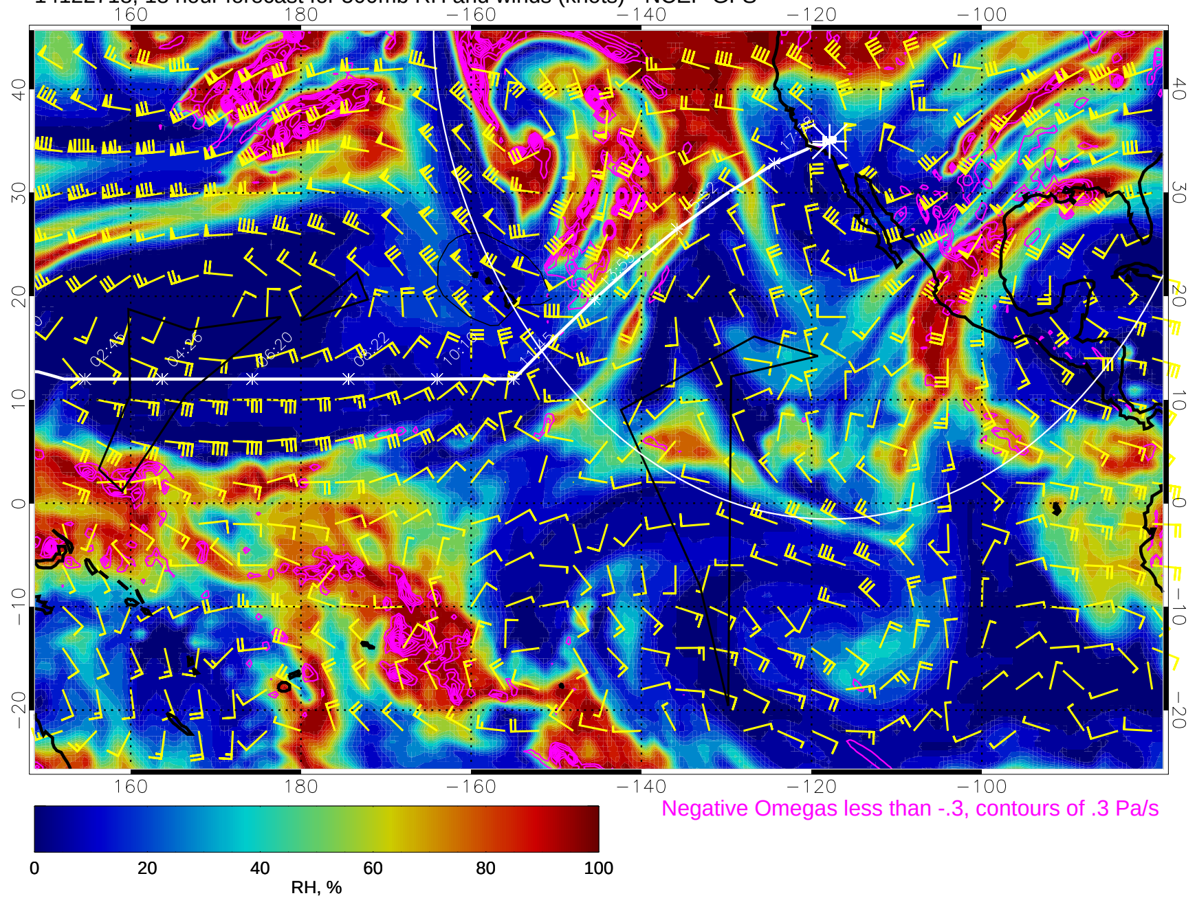
14122718, 18 hour forecast for 500mb RH and winds (knots) - NCEP GFS
