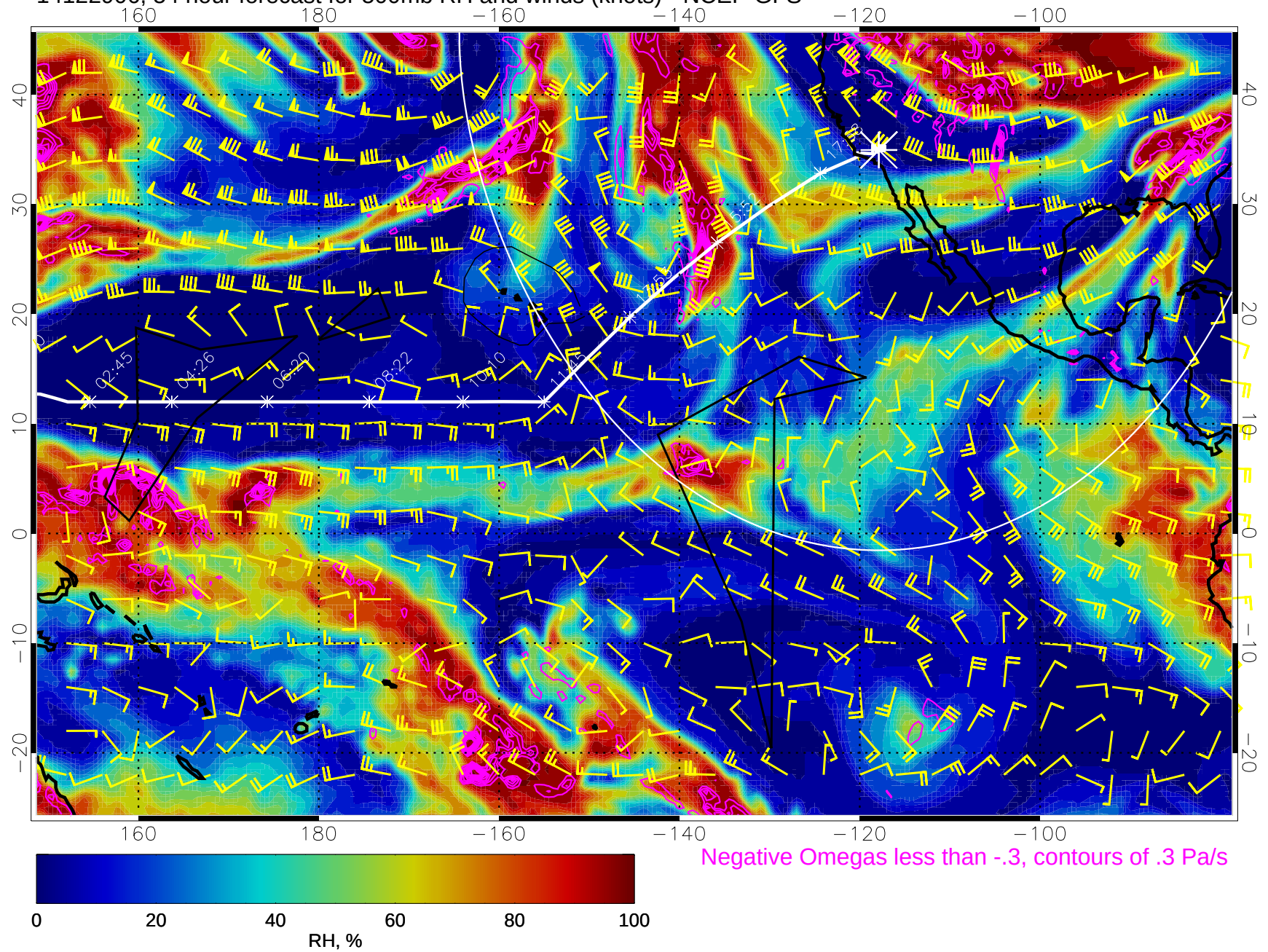
14122906, 54 hour forecast for 500mb RH and winds (knots) - NCEP GFS
