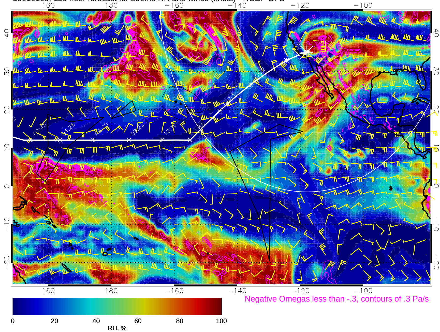
15010100, 120 hour forecast for 500mb RH and winds (knots) - NCEP GFS
