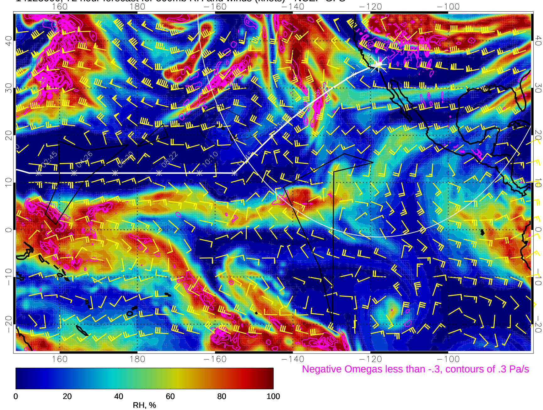
14123000, 72 hour forecast for 500mb RH and winds (knots) - NCEP GFS
