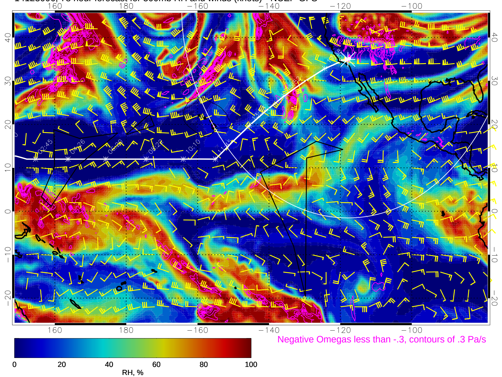
14123006, 78 hour forecast for 500mb RH and winds (knots) - NCEP GFS
