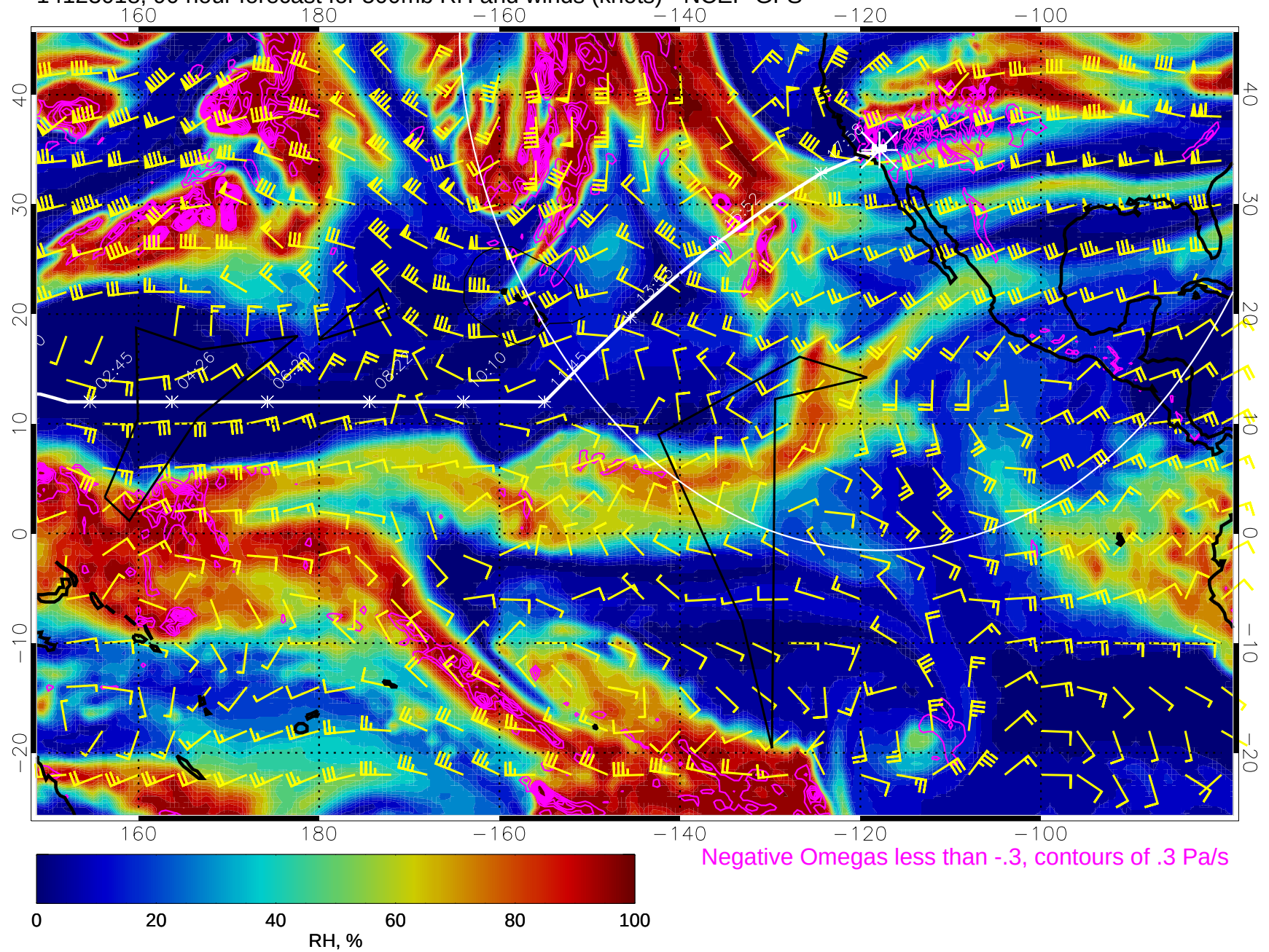
14123018, 90 hour forecast for 500mb RH and winds (knots) - NCEP GFS
