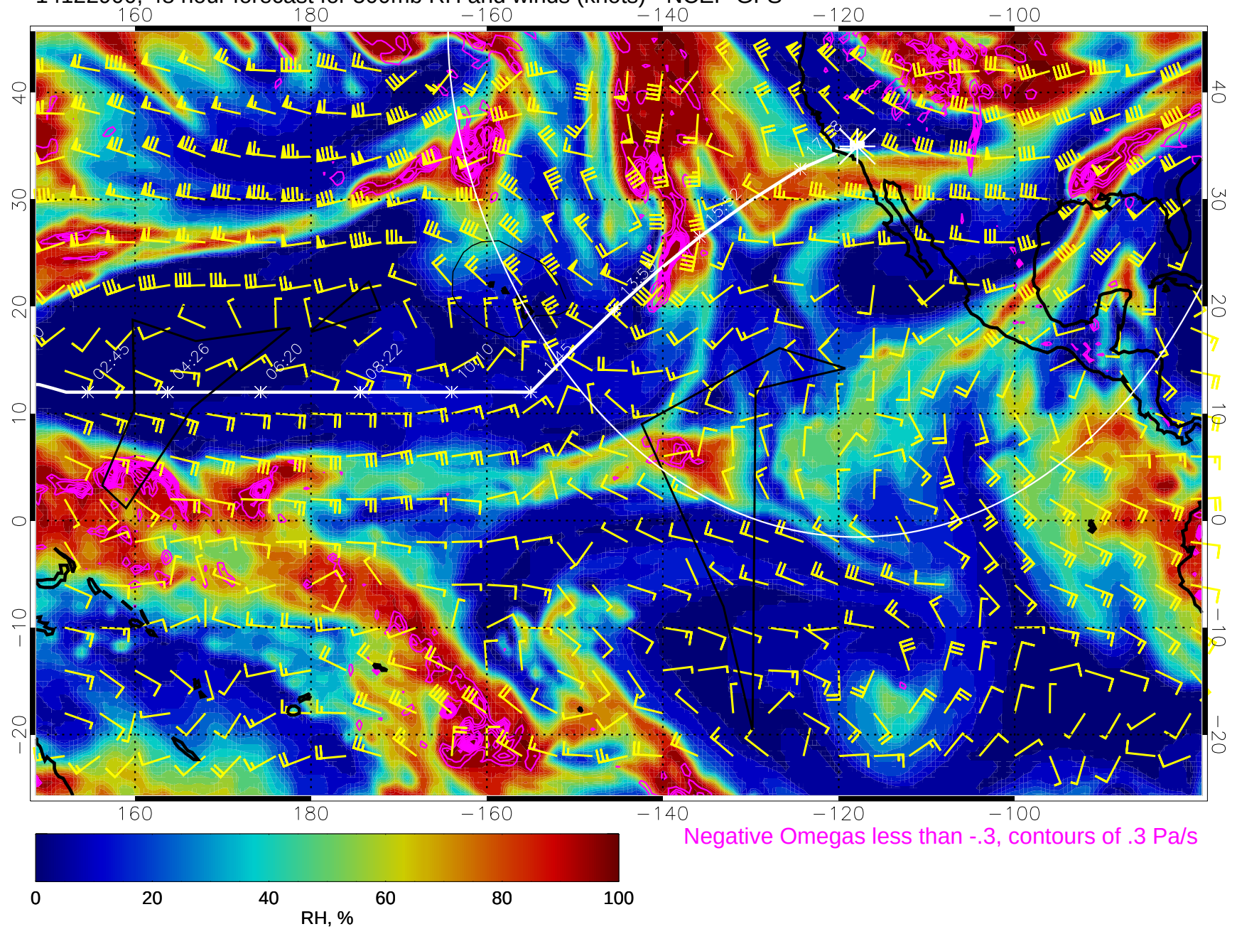
14122900, 48 hour forecast for 500mb RH and winds (knots) - NCEP GFS
