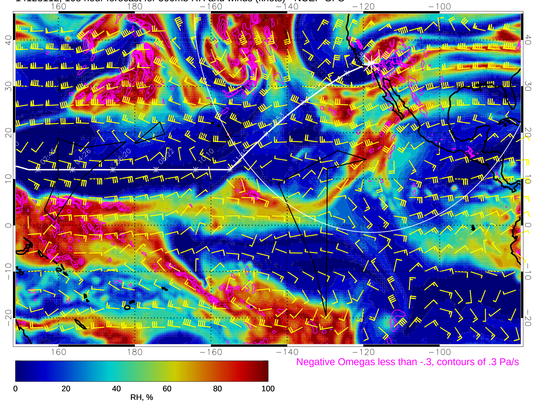
14123112, 108 hour forecast for 500mb RH and winds (knots) - NCEP GFS
