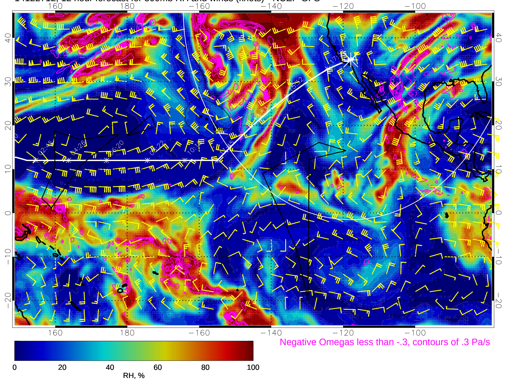
14122712, 12 hour forecast for 500mb RH and winds (knots) - NCEP GFS
