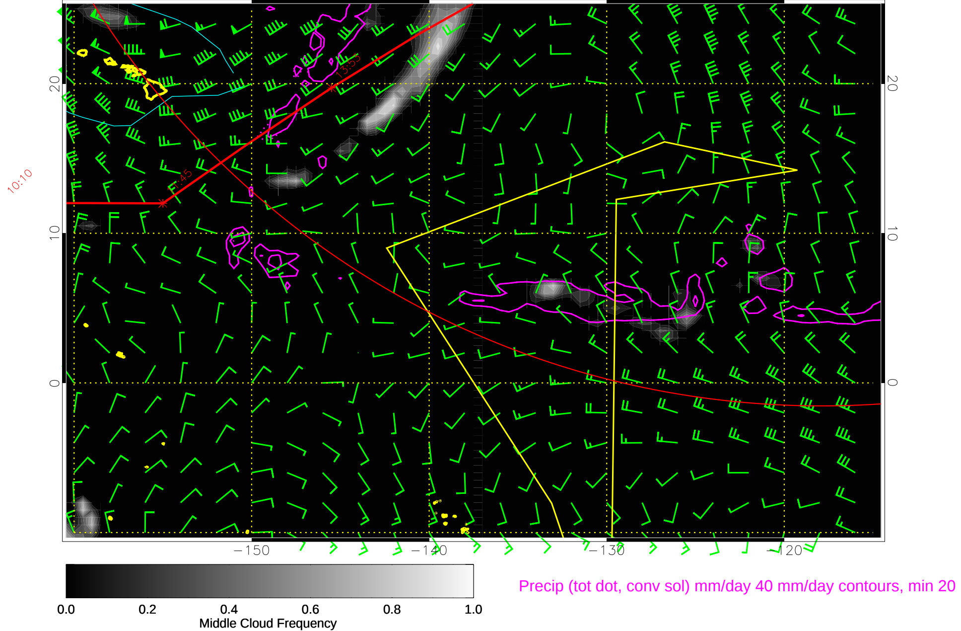
14122706, 6 hour forecast for 500mb winds (knots) and Middle Cloud Frequency -- NCEP GFS
