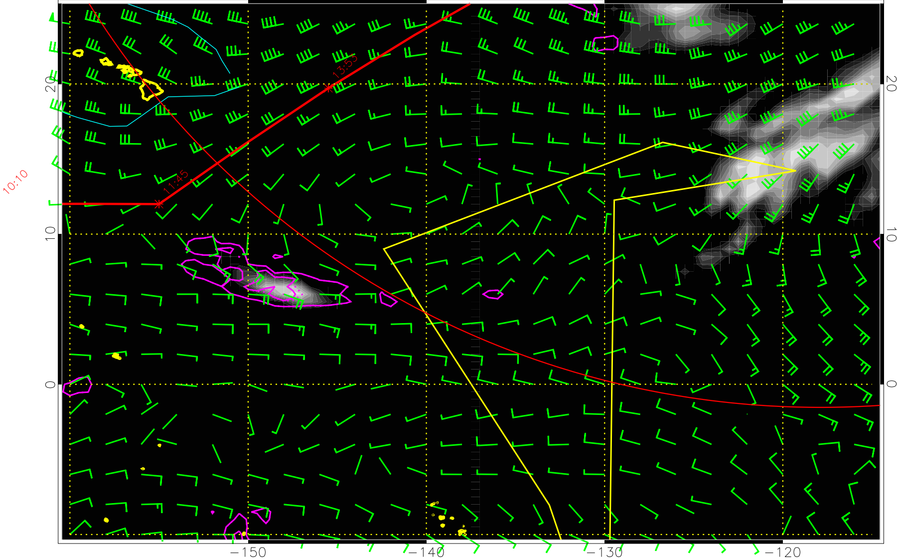
14123112, 108 hour forecast for 500mb winds (knots) and Middle Cloud Frequency -- NCEP GFS
