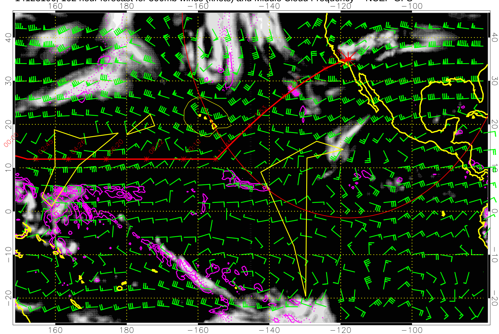
14123106, 102 hour forecast for 500mb winds (knots) and Middle Cloud Frequency -- NCEP GFS
