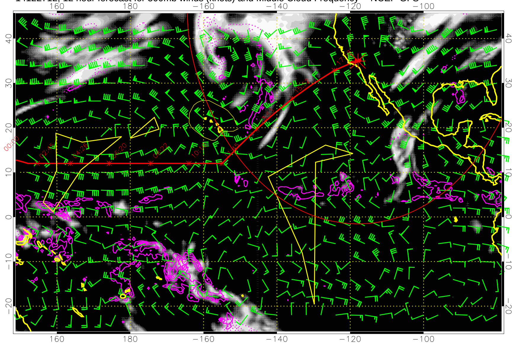
14122712, 12 hour forecast for 500mb winds (knots) and Middle Cloud Frequency -- NCEP GFS
