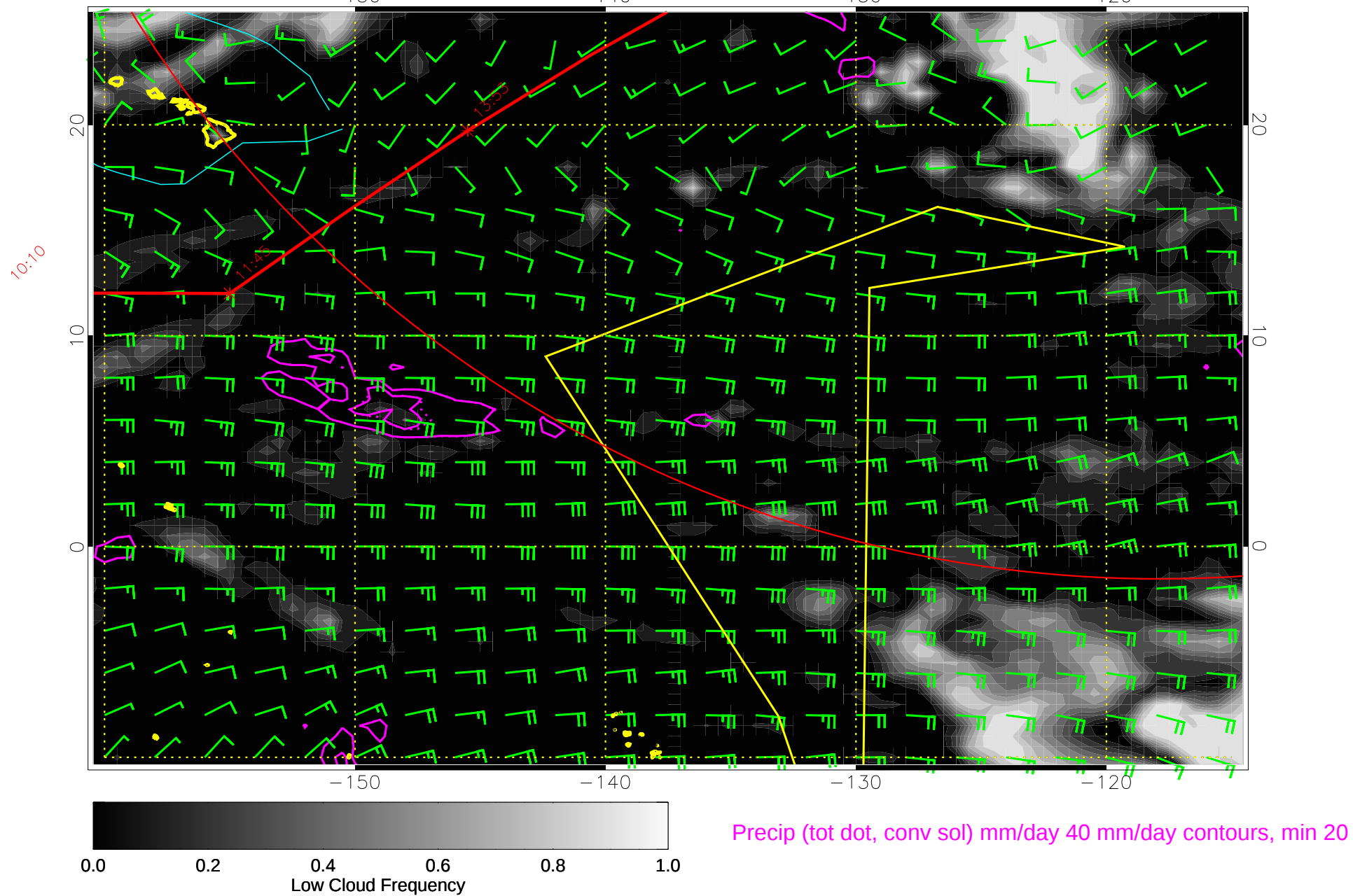
14123112, 108 hour forecast for 850mb winds (knots) and Low Cloud Frequency -- NCEP GFS
