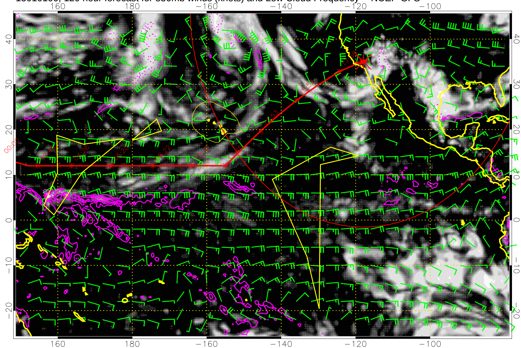
15010100, 120 hour forecast for 850mb winds (knots) and Low Cloud Frequency -- NCEP GFS
