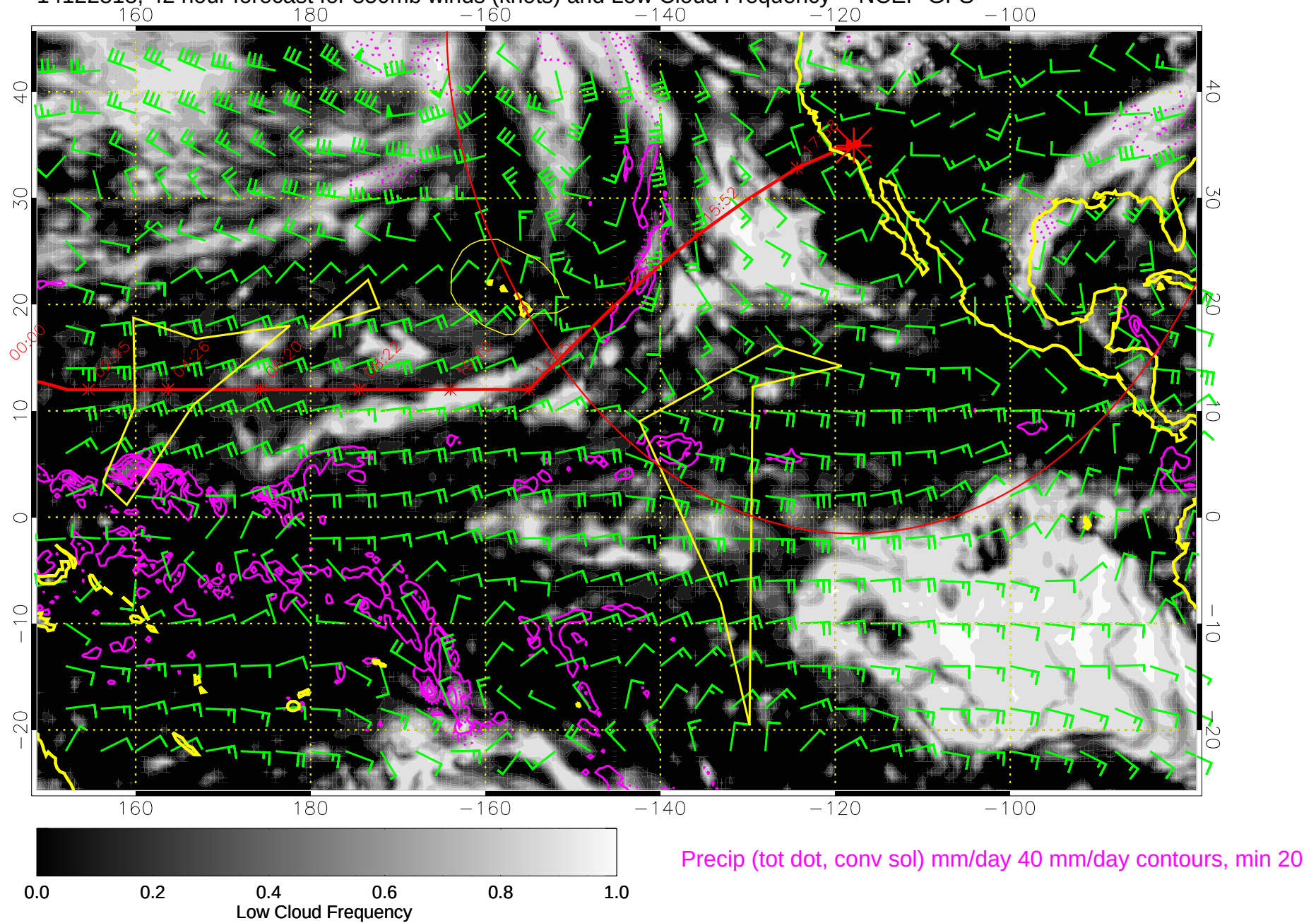
14122818, 42 hour forecast for 850mb winds (knots) and Low Cloud Frequency -- NCEP GFS
