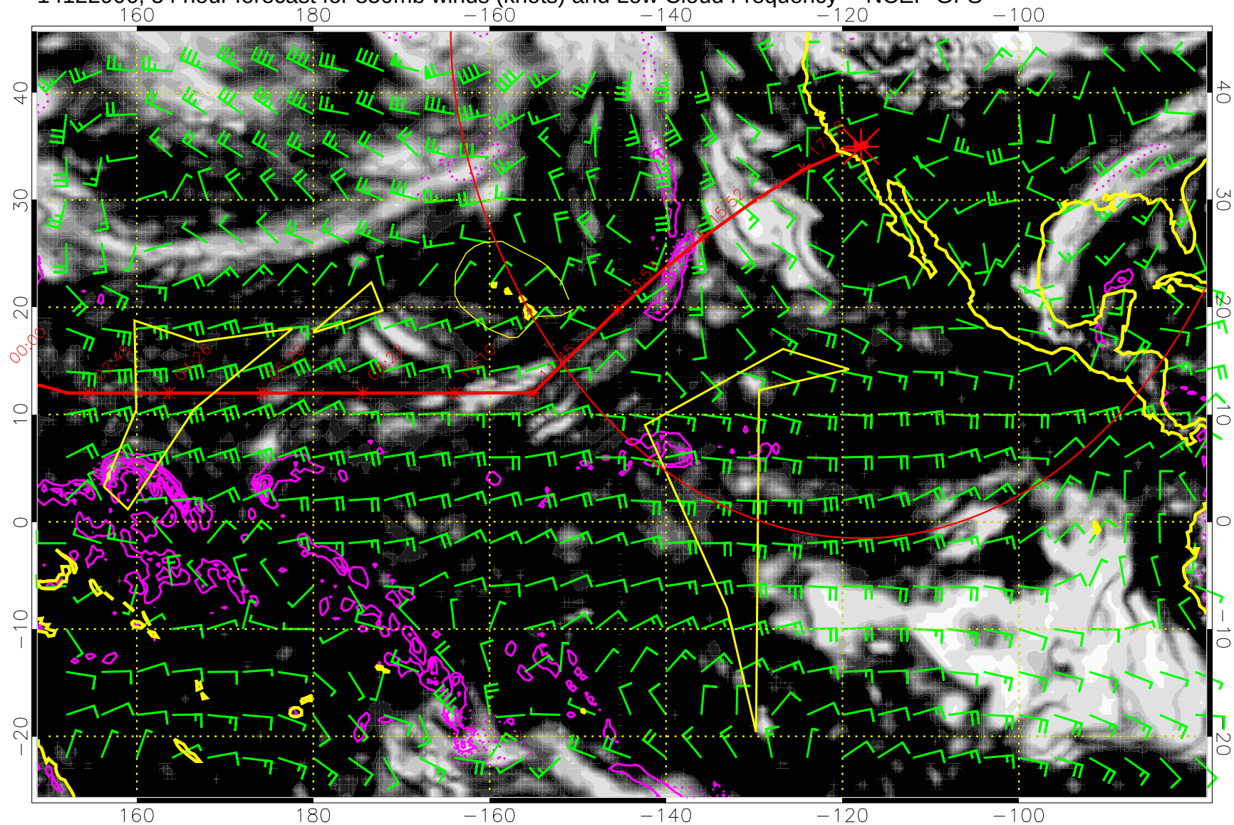
14122906, 54 hour forecast for 850mb winds (knots) and Low Cloud Frequency -- NCEP GFS
