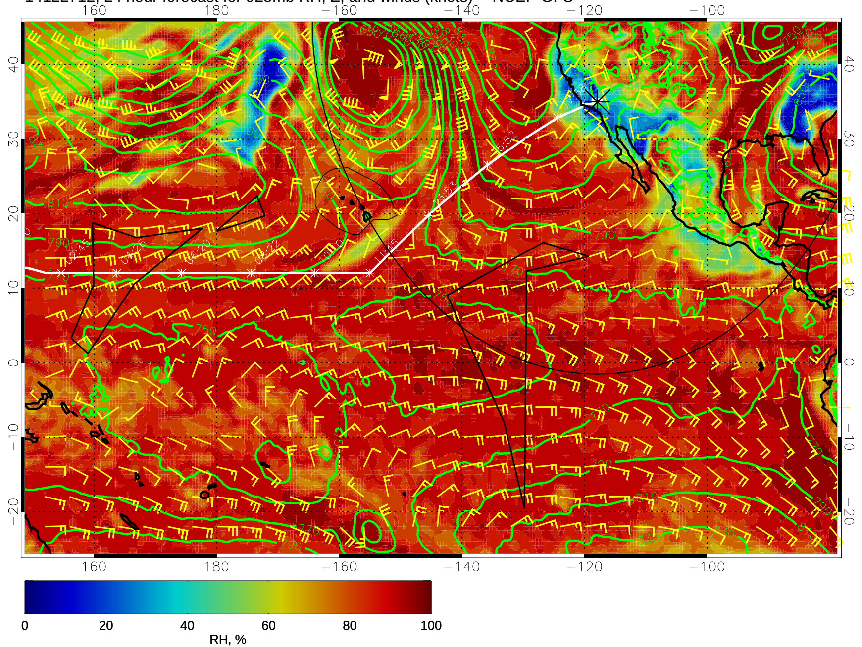
14122712, 24 hour forecast for 925mb RH, Z, and winds (knots) -- NCEP GFS
