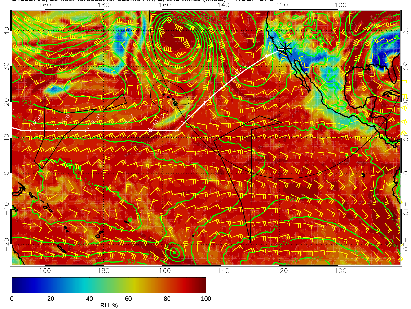
14122706, 18 hour forecast for 925mb RH, Z, and winds (knots) -- NCEP GFS
