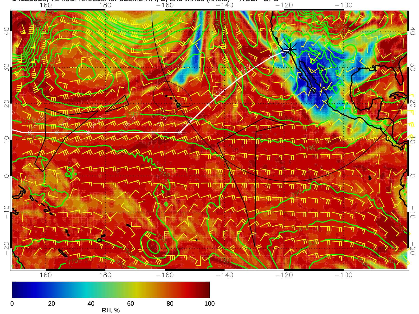
14122918, 78 hour forecast for 925mb RH, Z, and winds (knots) -- NCEP GFS
