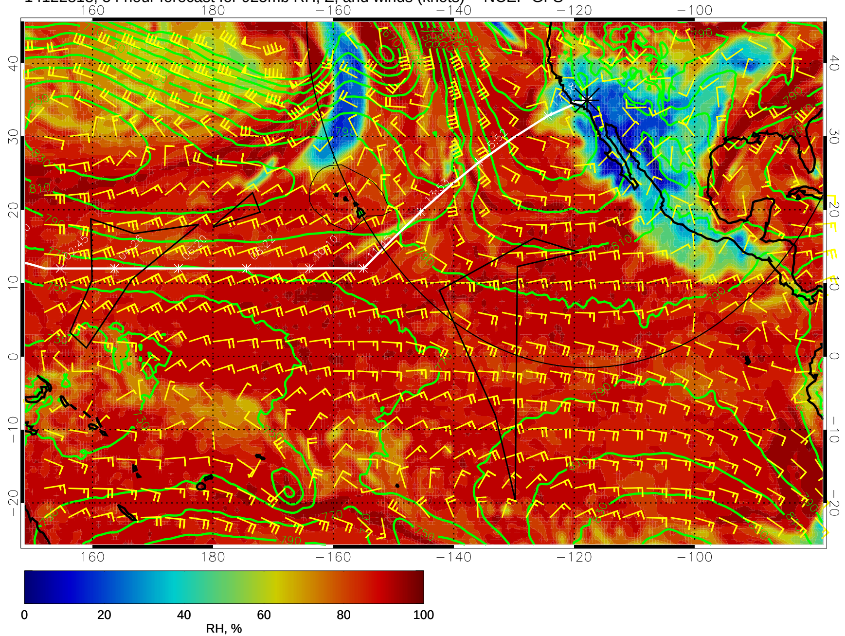
14122818, 54 hour forecast for 925mb RH, Z, and winds (knots) -- NCEP GFS
