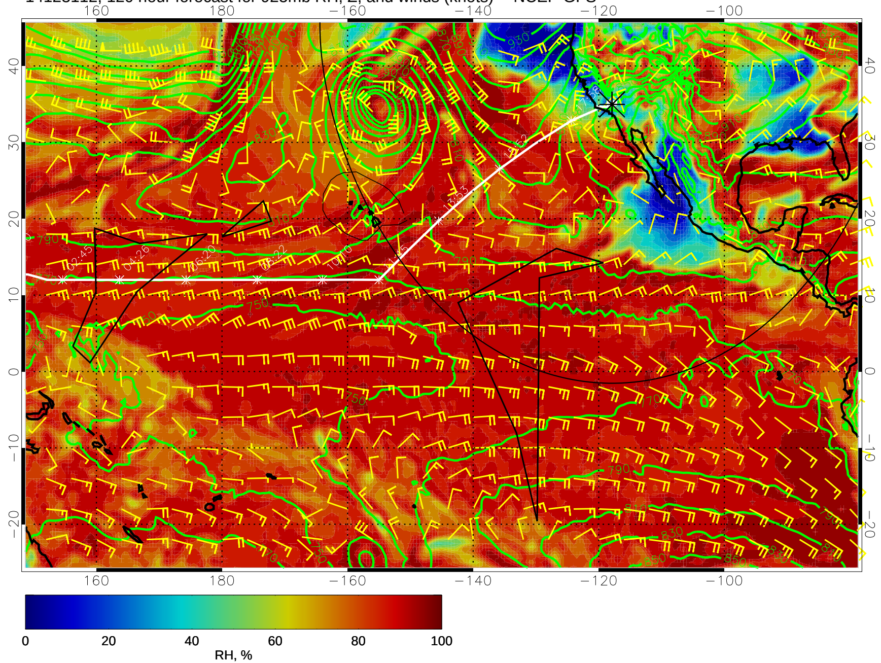
14123112, 120 hour forecast for 925mb RH, Z, and winds (knots) -- NCEP GFS
