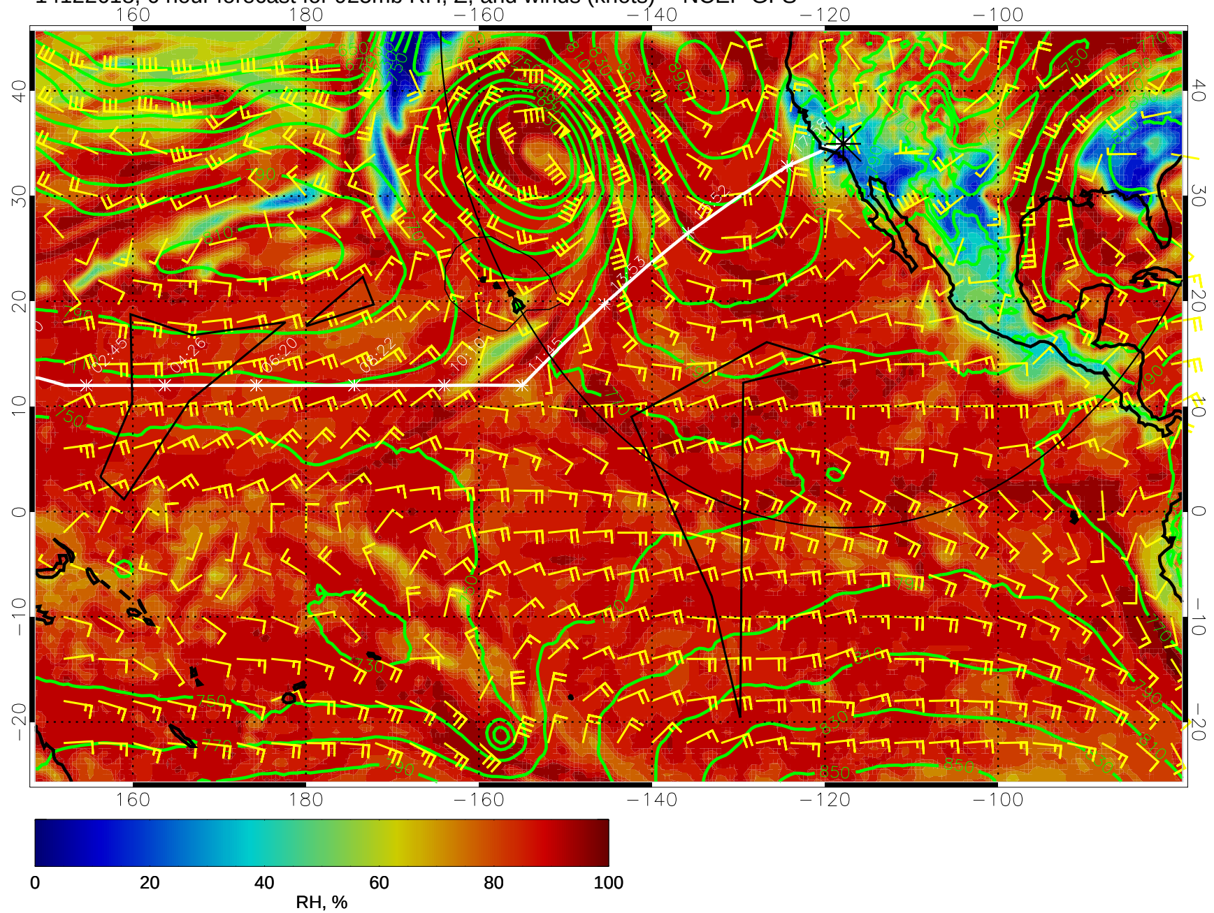
14122618, 6 hour forecast for 925mb RH, Z, and winds (knots) -- NCEP GFS
