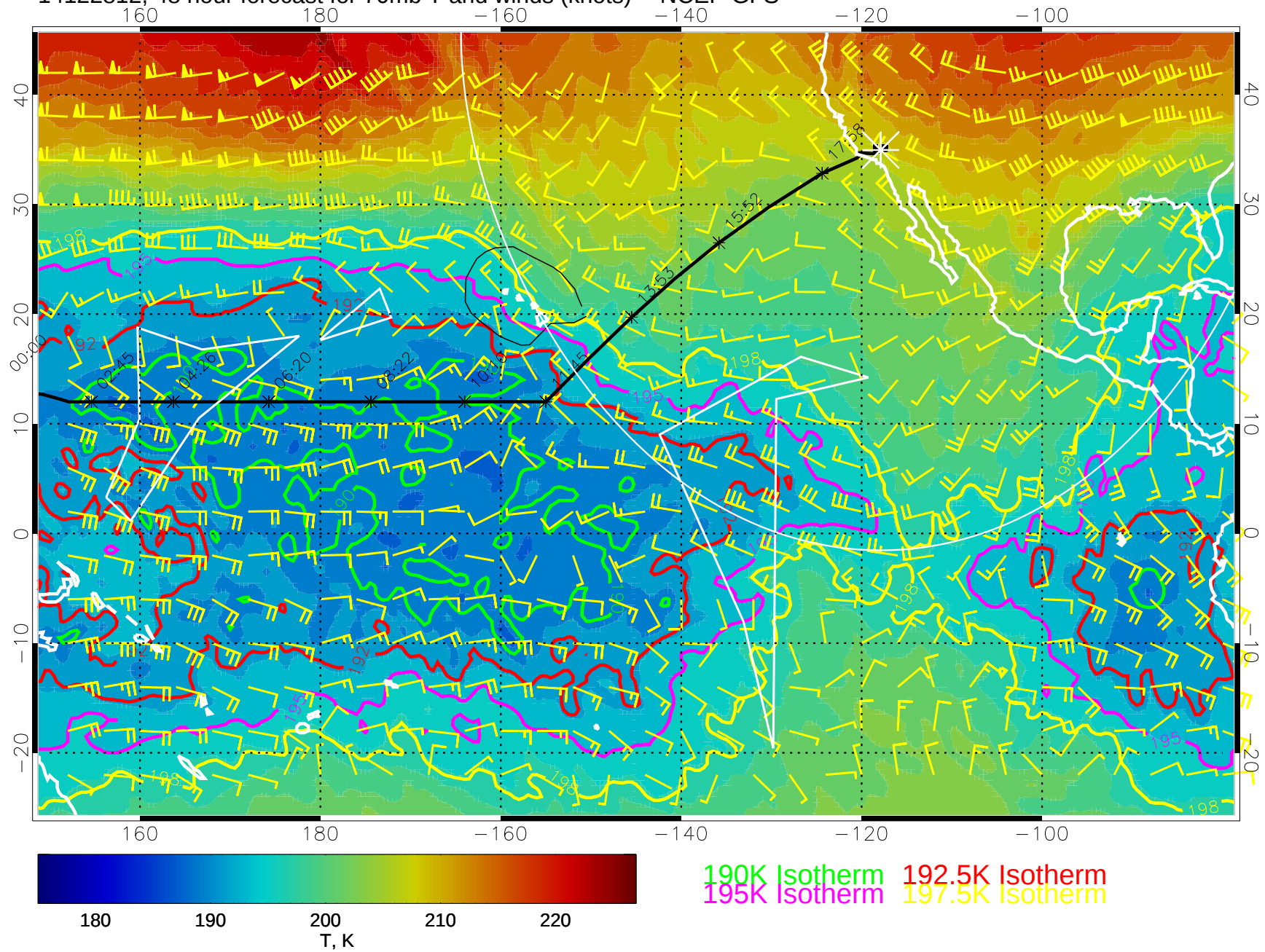
14122812, 48 hour forecast for 70mb T and winds (knots) -- NCEP GFS
