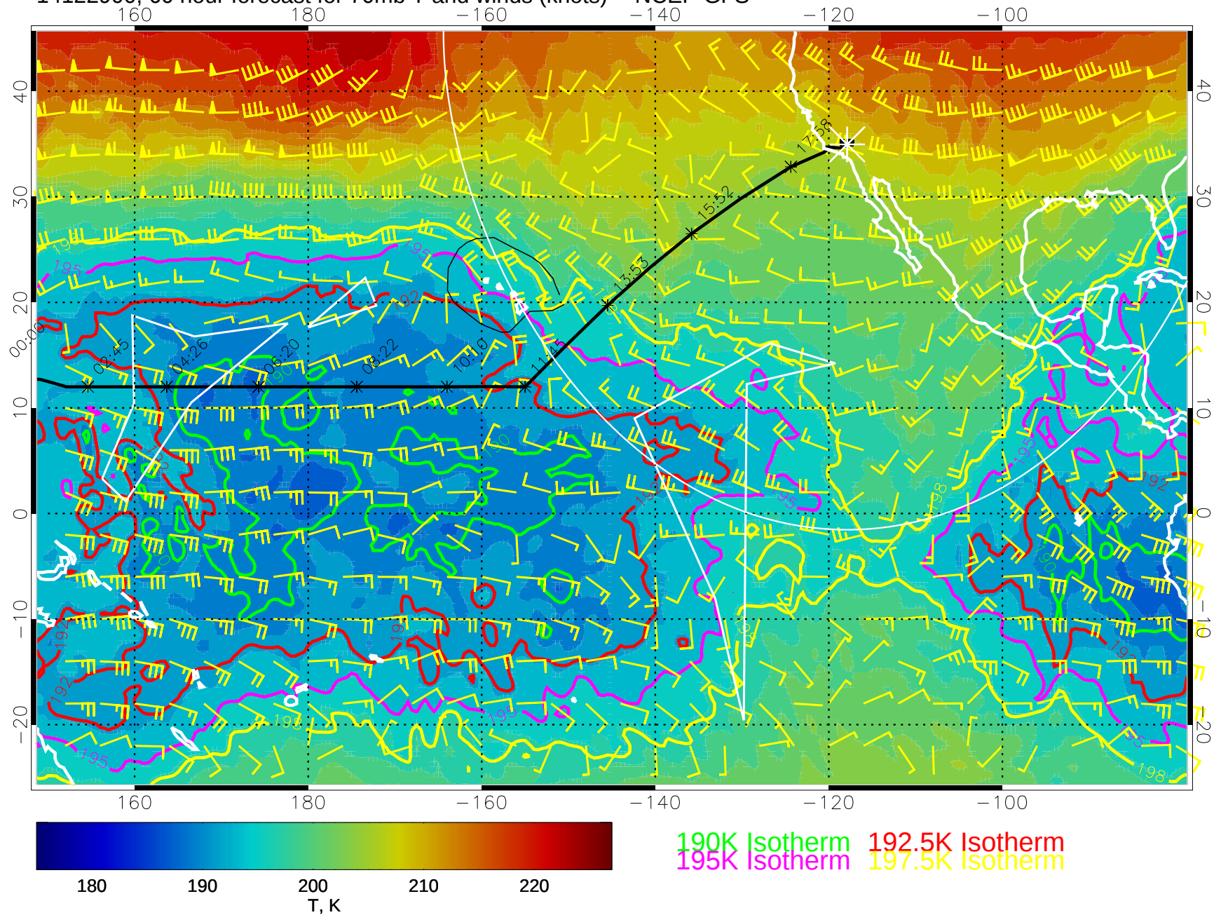
14122900, 60 hour forecast for 70mb T and winds (knots) -- NCEP GFS
