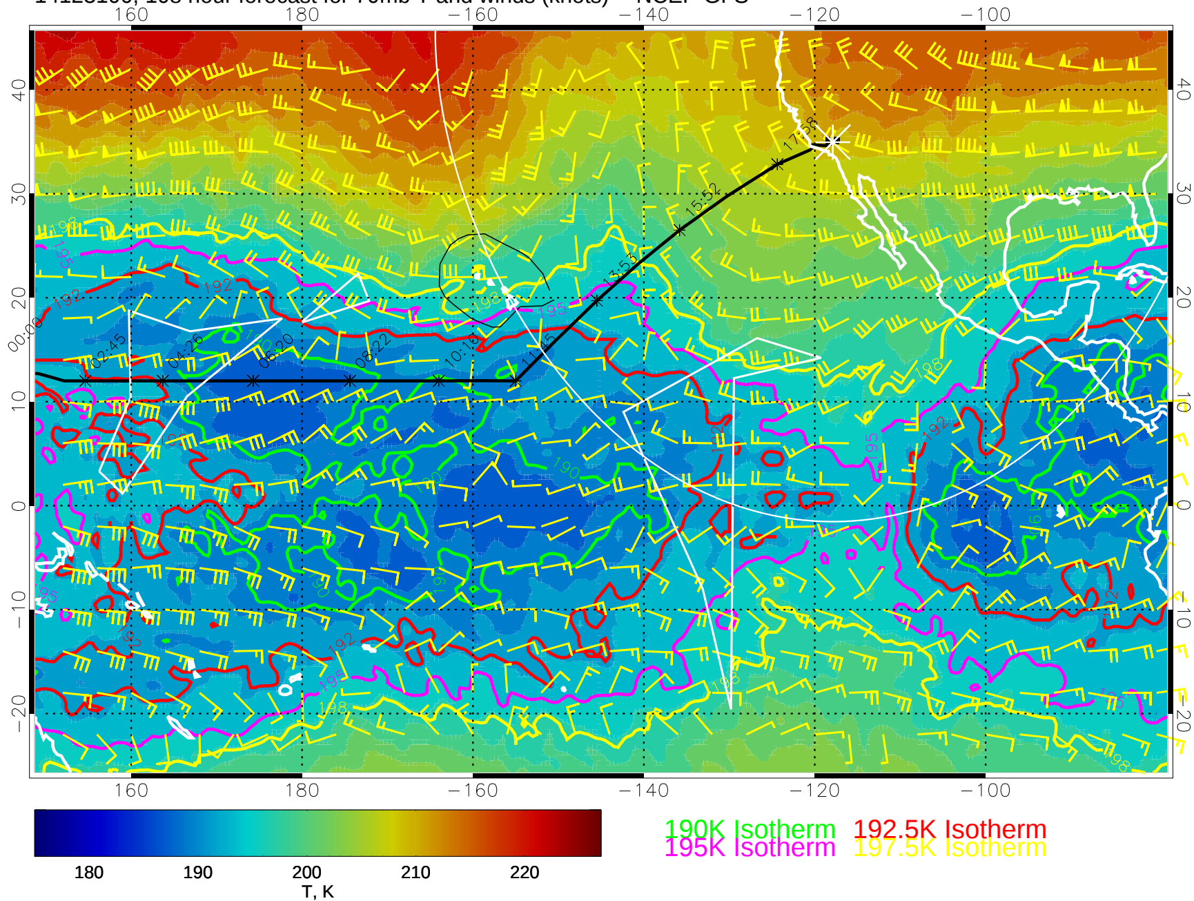
14123100, 108 hour forecast for 70mb T and winds (knots) -- NCEP GFS
