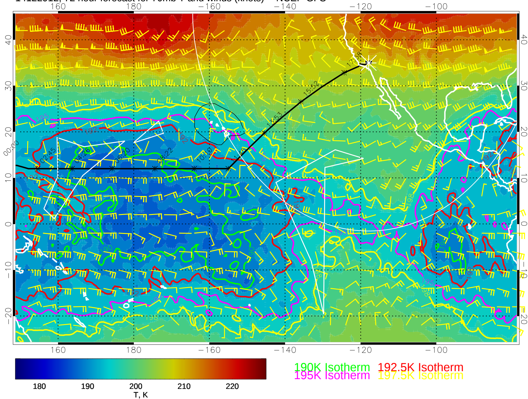
14122912, 72 hour forecast for 70mb T and winds (knots) -- NCEP GFS
