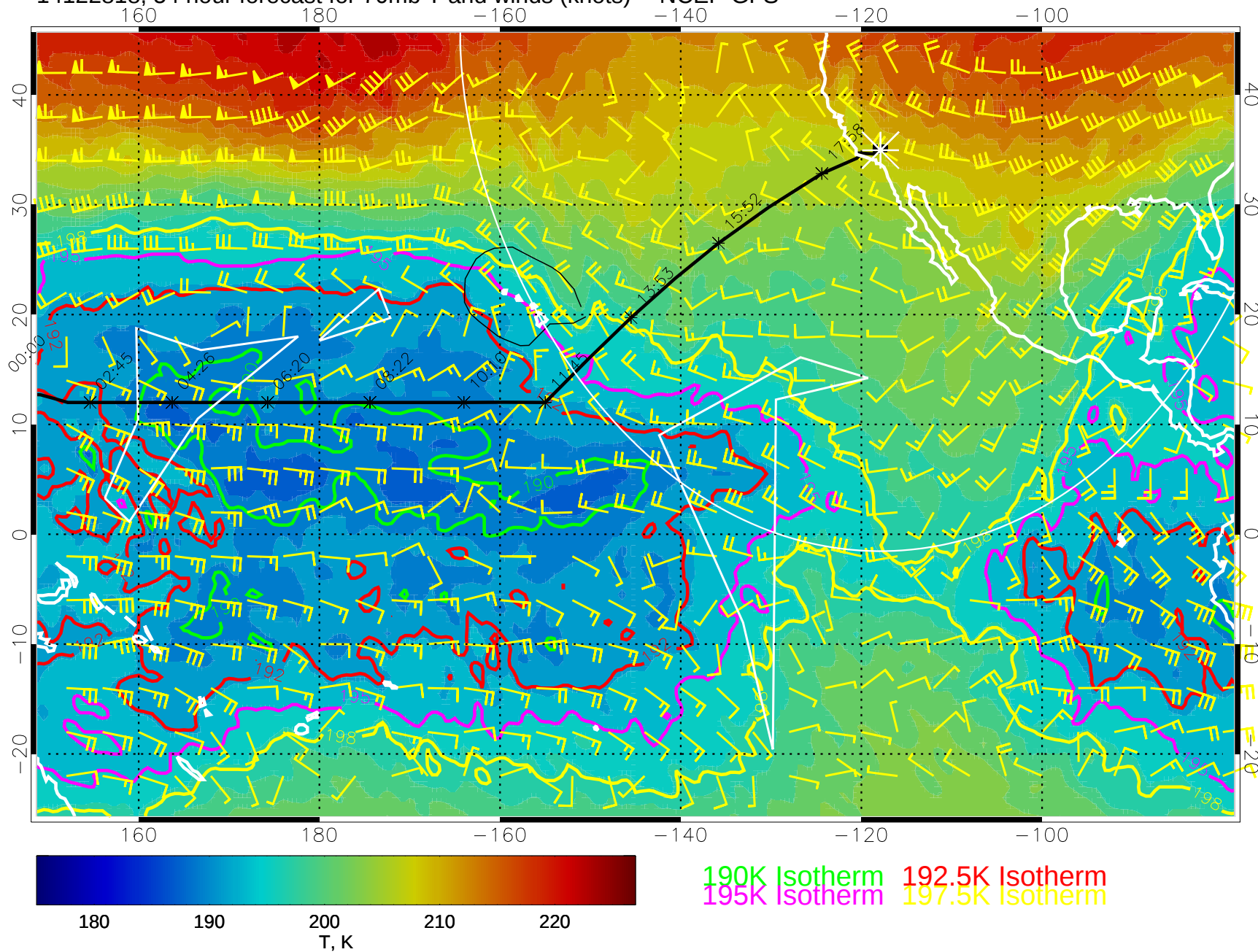
14122818, 54 hour forecast for 70mb T and winds (knots) -- NCEP GFS
