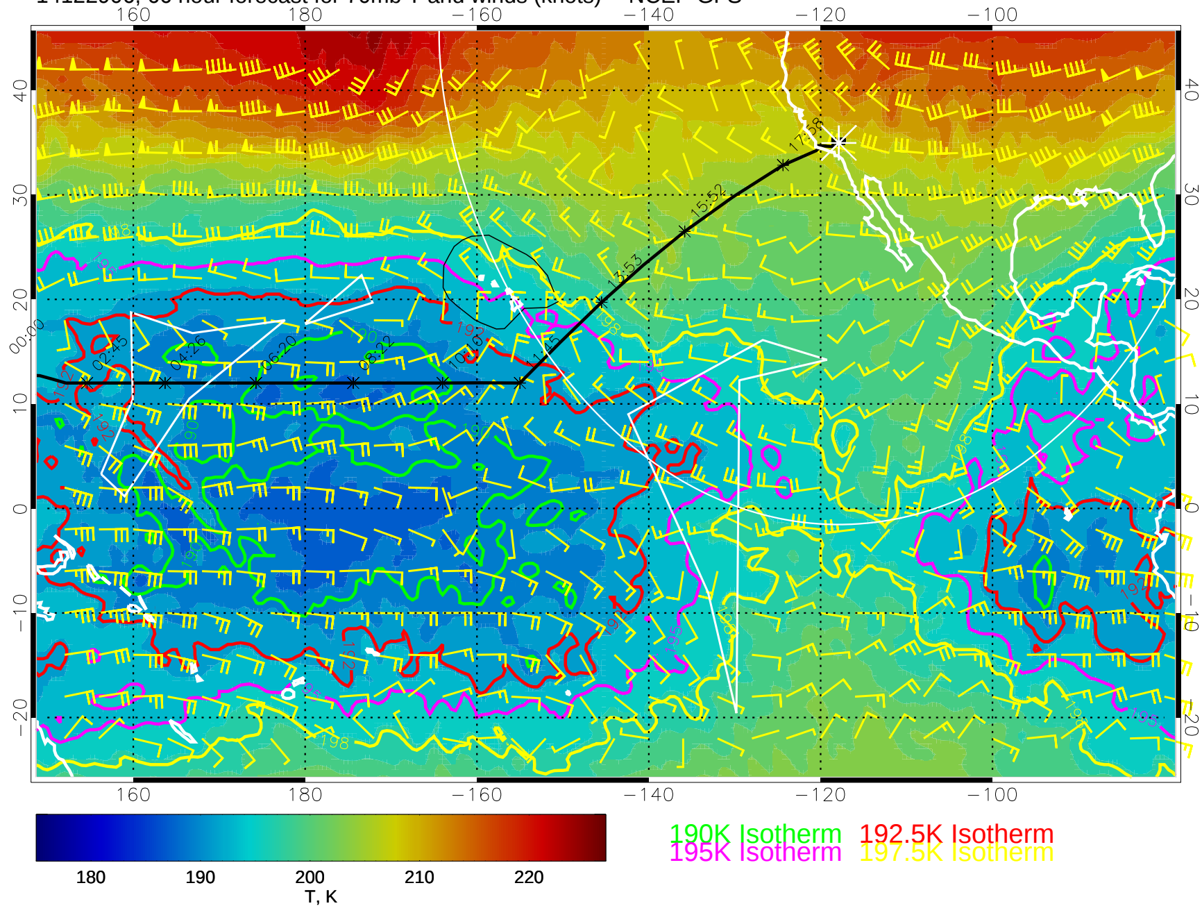
14122906, 66 hour forecast for 70mb T and winds (knots) -- NCEP GFS
