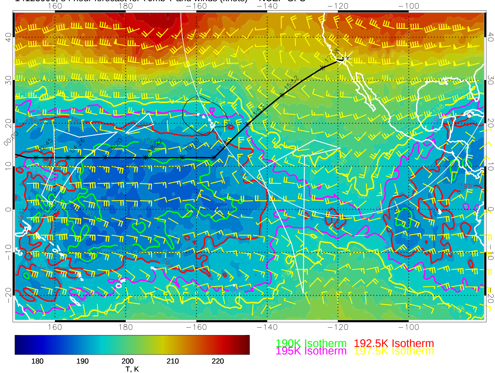
14123000, 84 hour forecast for 70mb T and winds (knots) -- NCEP GFS
