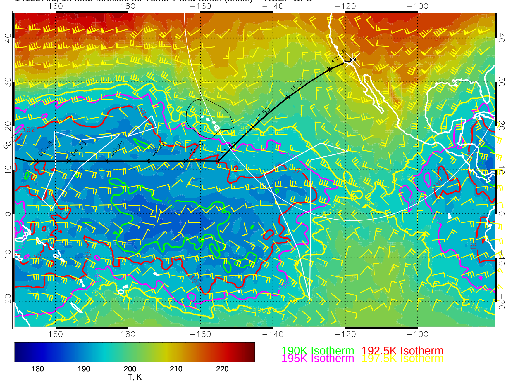
14122706, 18 hour forecast for 70mb T and winds (knots) -- NCEP GFS
