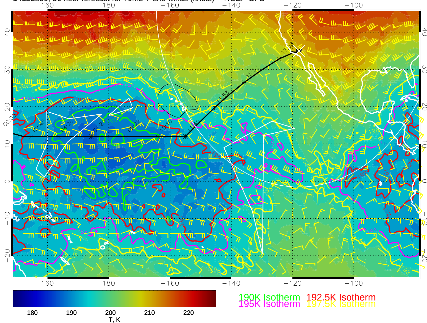
14122800, 36 hour forecast for 70mb T and winds (knots) -- NCEP GFS
