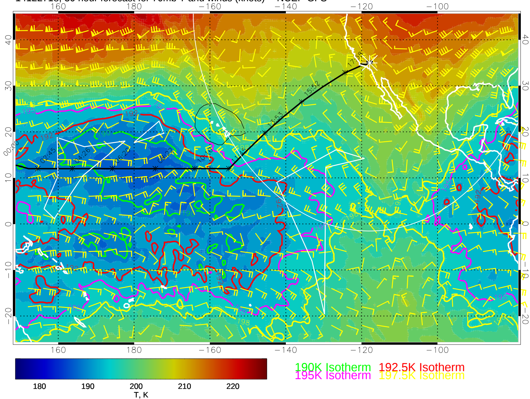
14122718, 30 hour forecast for 70mb T and winds (knots) -- NCEP GFS
