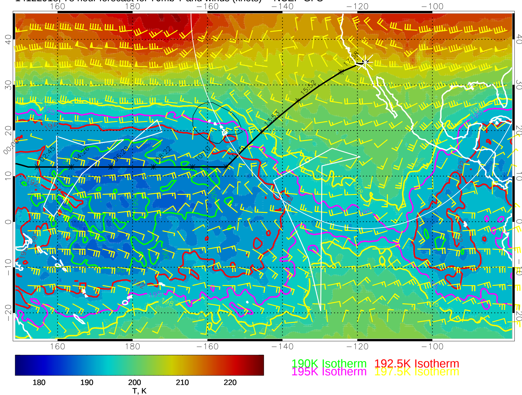
14122918, 78 hour forecast for 70mb T and winds (knots) -- NCEP GFS
