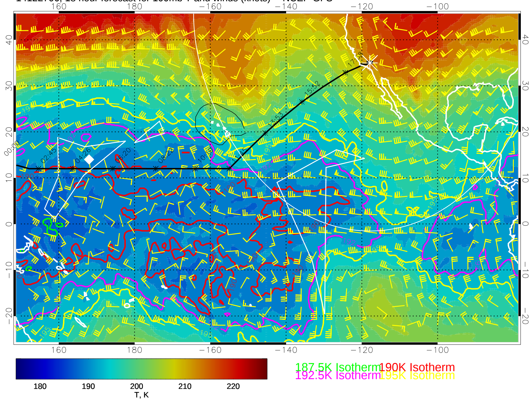
14122706, 18 hour forecast for 100mb T and winds (knots) -- NCEP GFS
