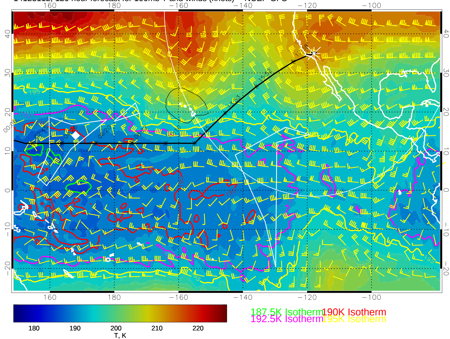
14123112, 120 hour forecast for 100mb T and winds (knots) -- NCEP GFS
