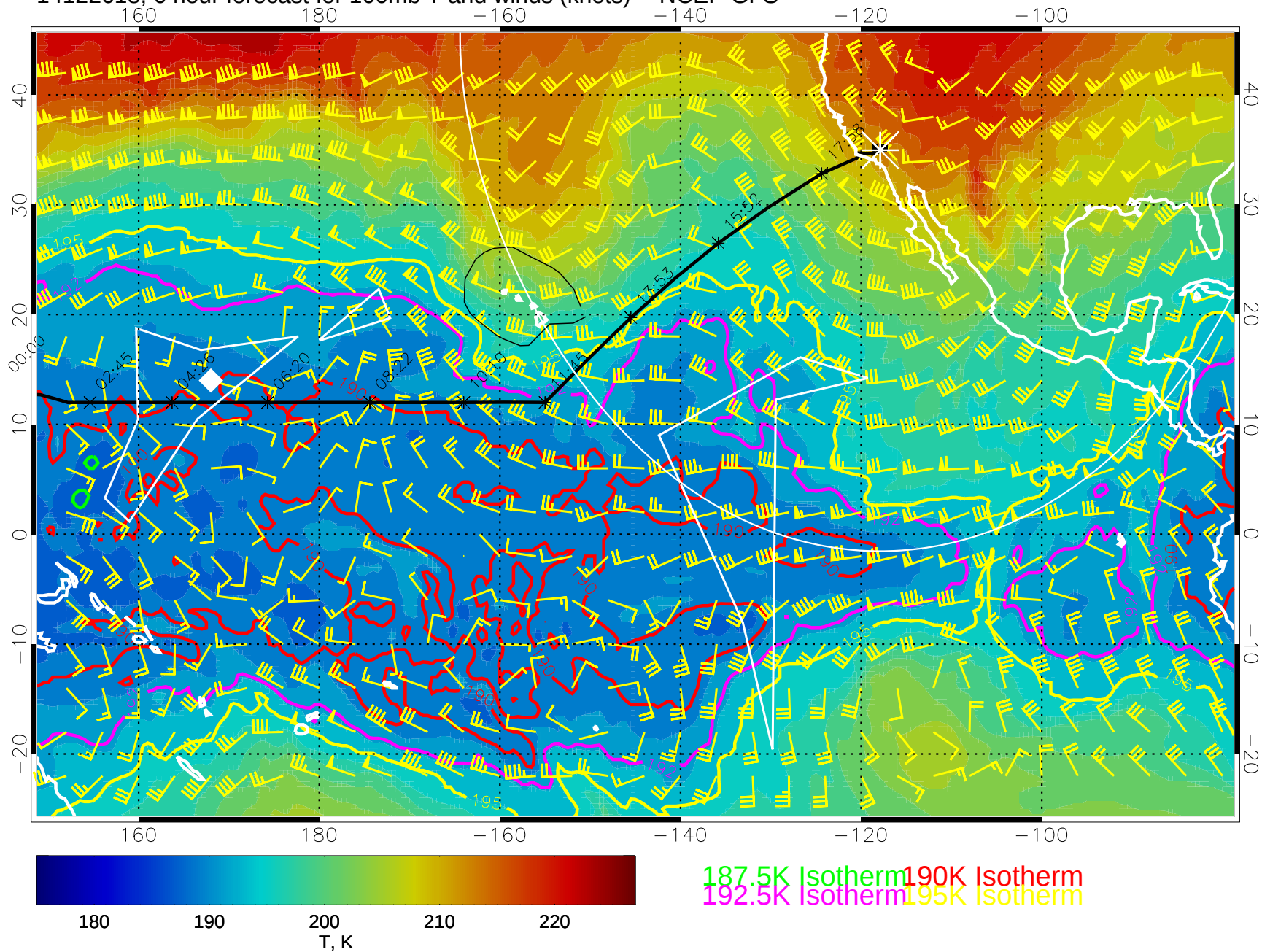
14122618, 6 hour forecast for 100mb T and winds (knots) -- NCEP GFS
