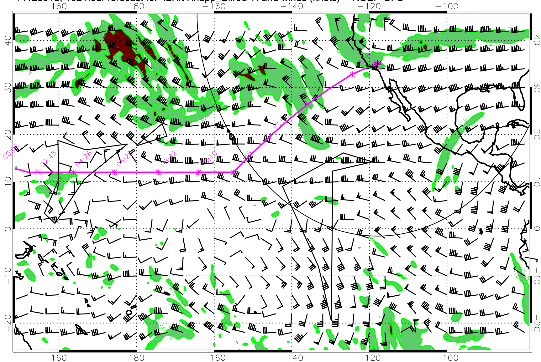
14123018, 102 hour forecast for 42Kft Knapp_Ellrod TI and winds (knots) -- NCEP GFS
