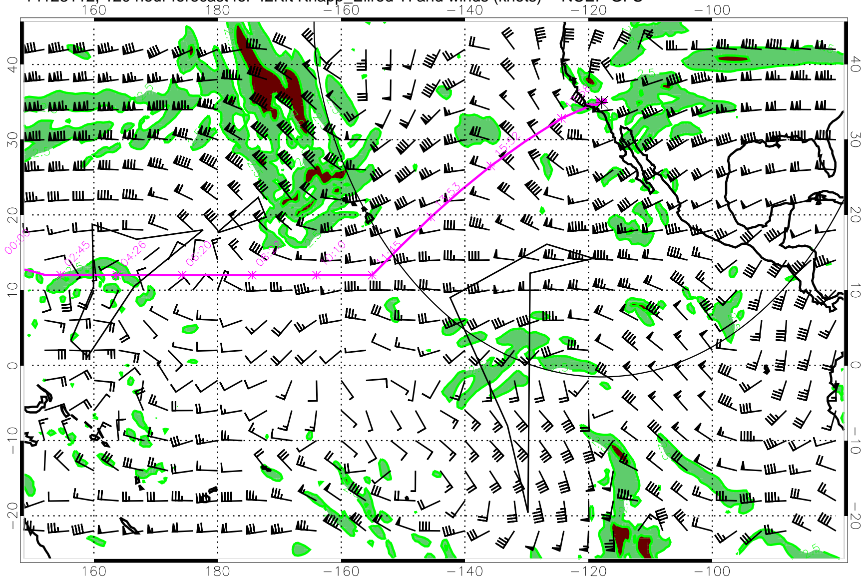
14123112, 120 hour forecast for 42Kft Knapp_Ellrod TI and winds (knots) -- NCEP GFS
