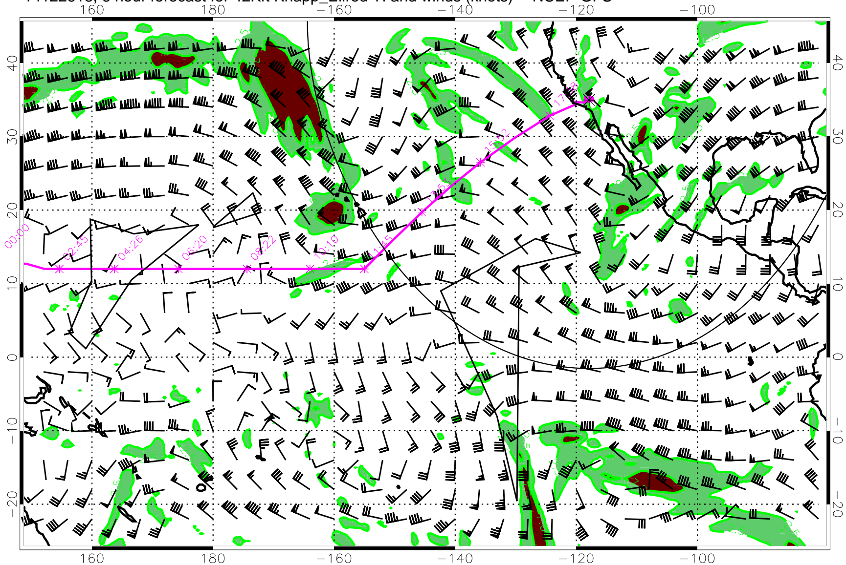
14122618, 6 hour forecast for 42Kft Knapp_Ellrod TI and winds (knots) -- NCEP GFS
