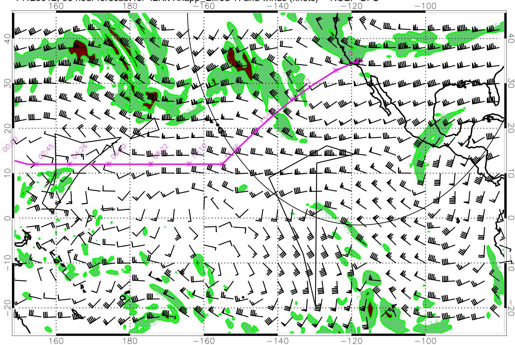
14123012, 96 hour forecast for 42Kft Knapp_Ellrod TI and winds (knots) -- NCEP GFS
