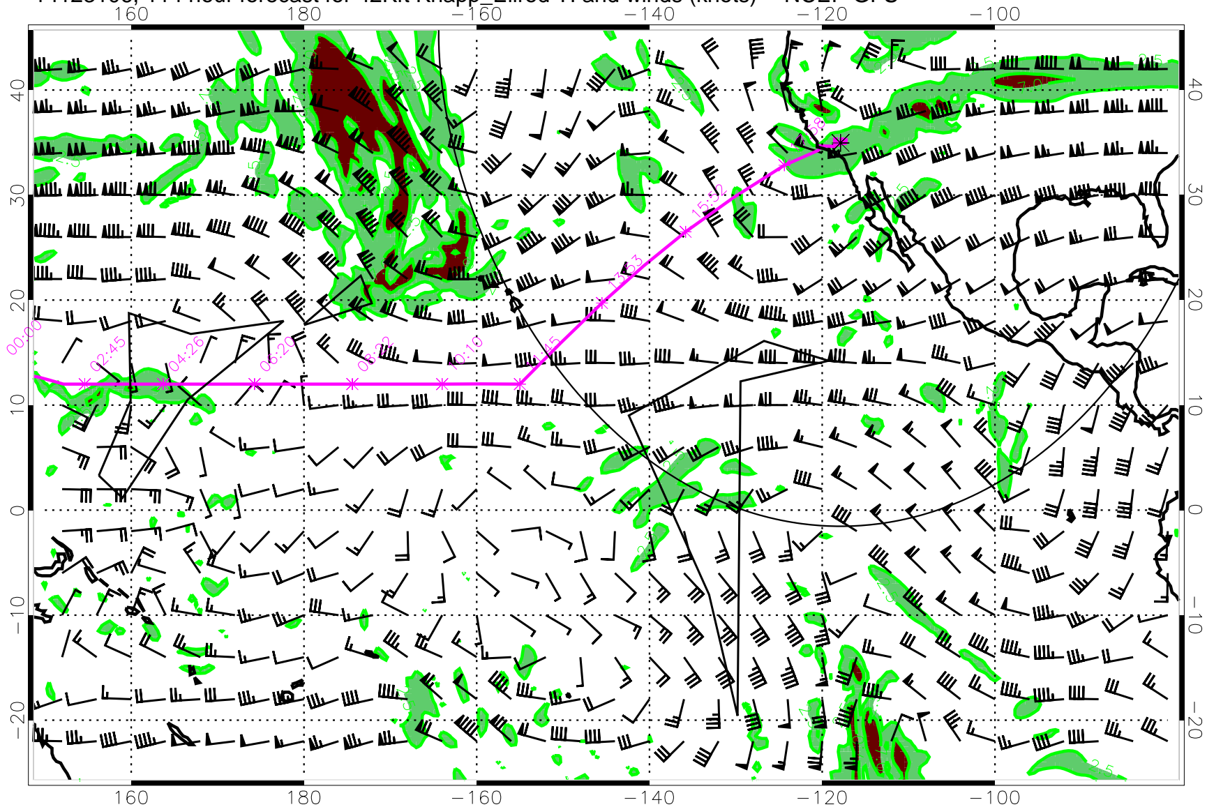
14123106, 114 hour forecast for 42Kft Knapp_Ellrod TI and winds (knots) -- NCEP GFS
