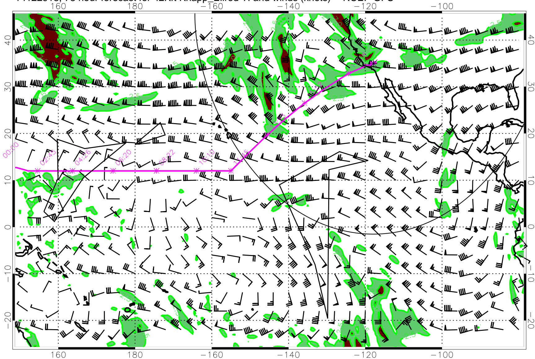
14122918, 78 hour forecast for 42Kft Knapp_Ellrod TI and winds (knots) -- NCEP GFS
