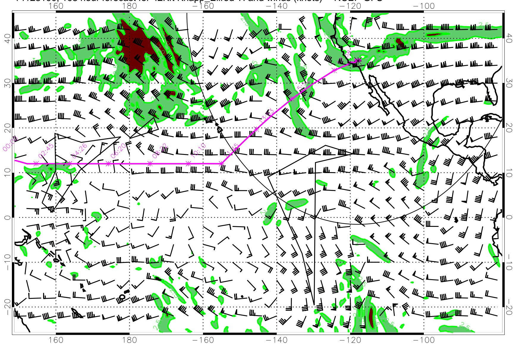
14123100, 108 hour forecast for 42Kft Knapp_Ellrod TI and winds (knots) -- NCEP GFS
