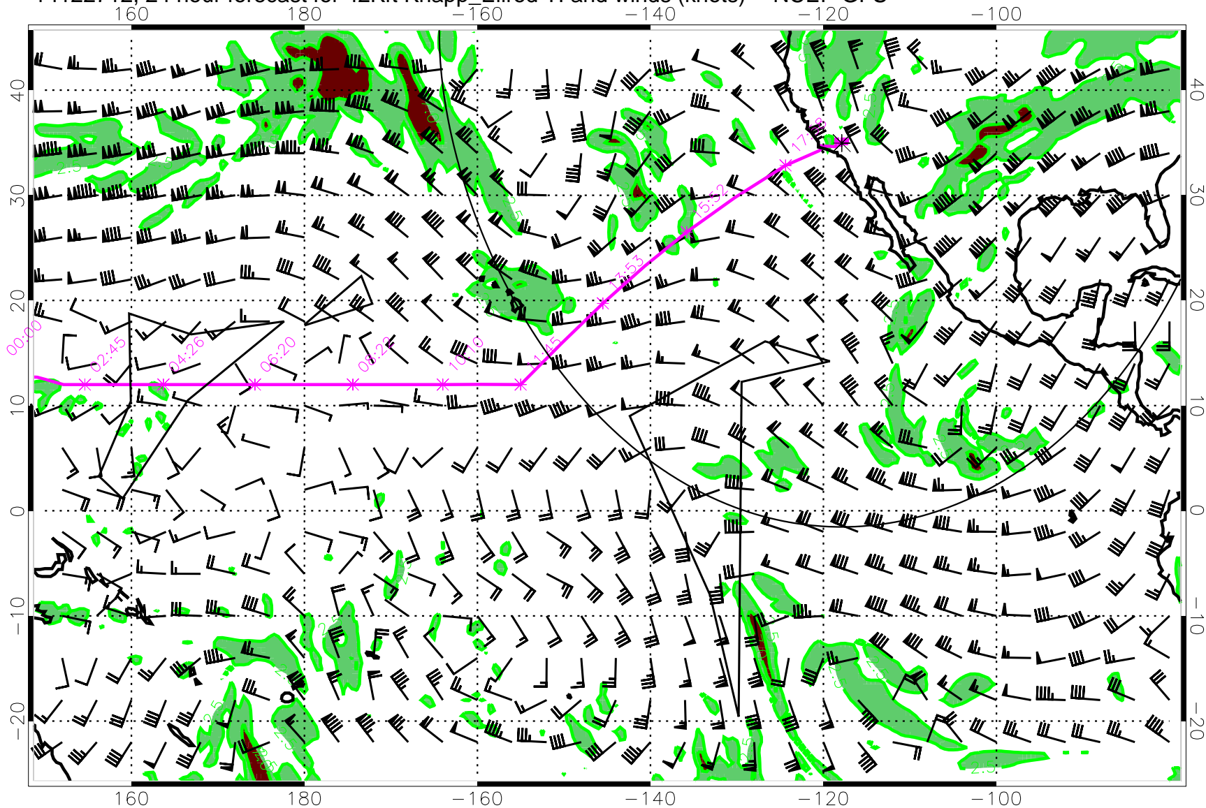
14122712, 24 hour forecast for 42Kft Knapp_Ellrod TI and winds (knots) -- NCEP GFS
