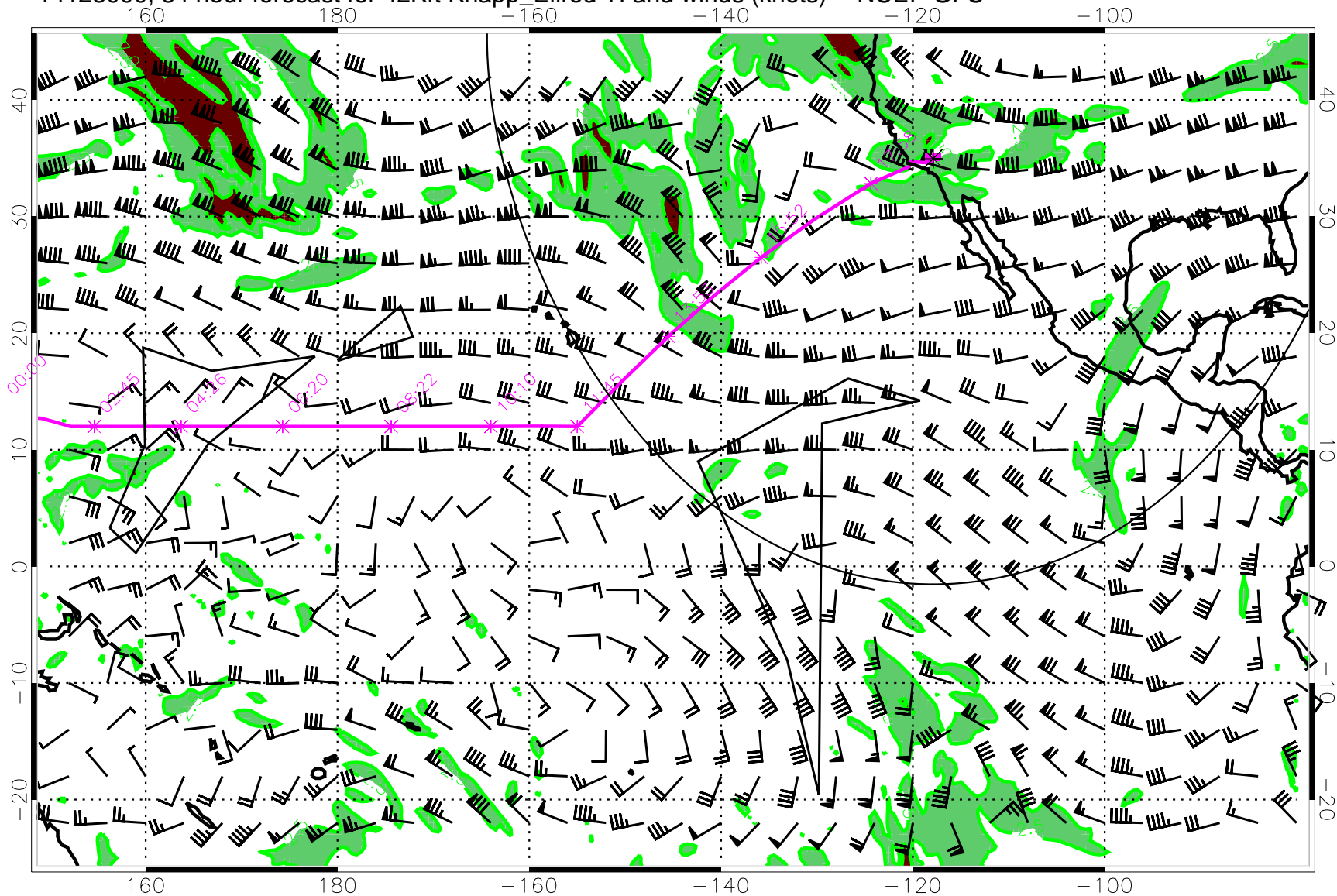
14123000, 84 hour forecast for 42Kft Knapp_Ellrod TI and winds (knots) -- NCEP GFS
