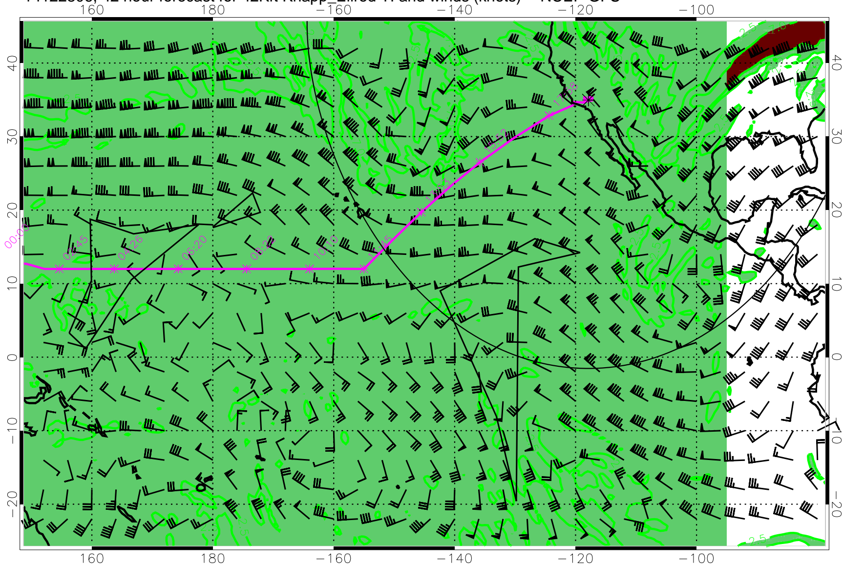
14122806, 42 hour forecast for 42Kft Knapp_Ellrod TI and winds (knots) -- NCEP GFS
