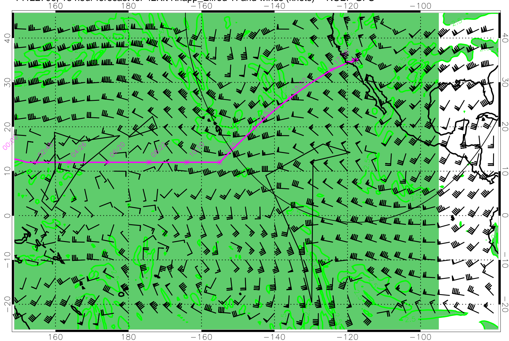
14122706, 18 hour forecast for 42Kft Knapp_Ellrod TI and winds (knots) -- NCEP GFS
