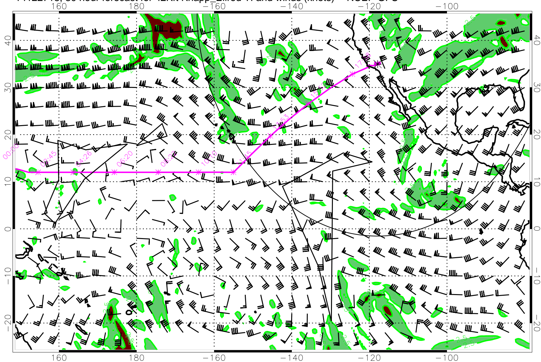
14122718, 30 hour forecast for 42Kft Knapp_Ellrod TI and winds (knots) -- NCEP GFS
