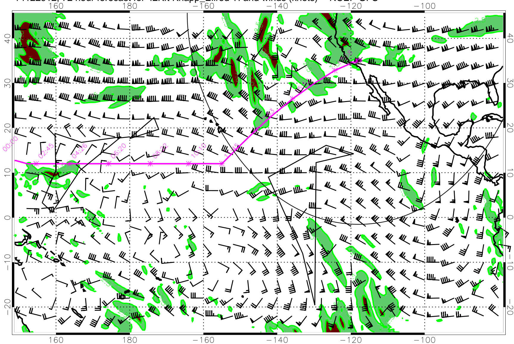
14122912, 72 hour forecast for 42Kft Knapp_Ellrod TI and winds (knots) -- NCEP GFS
