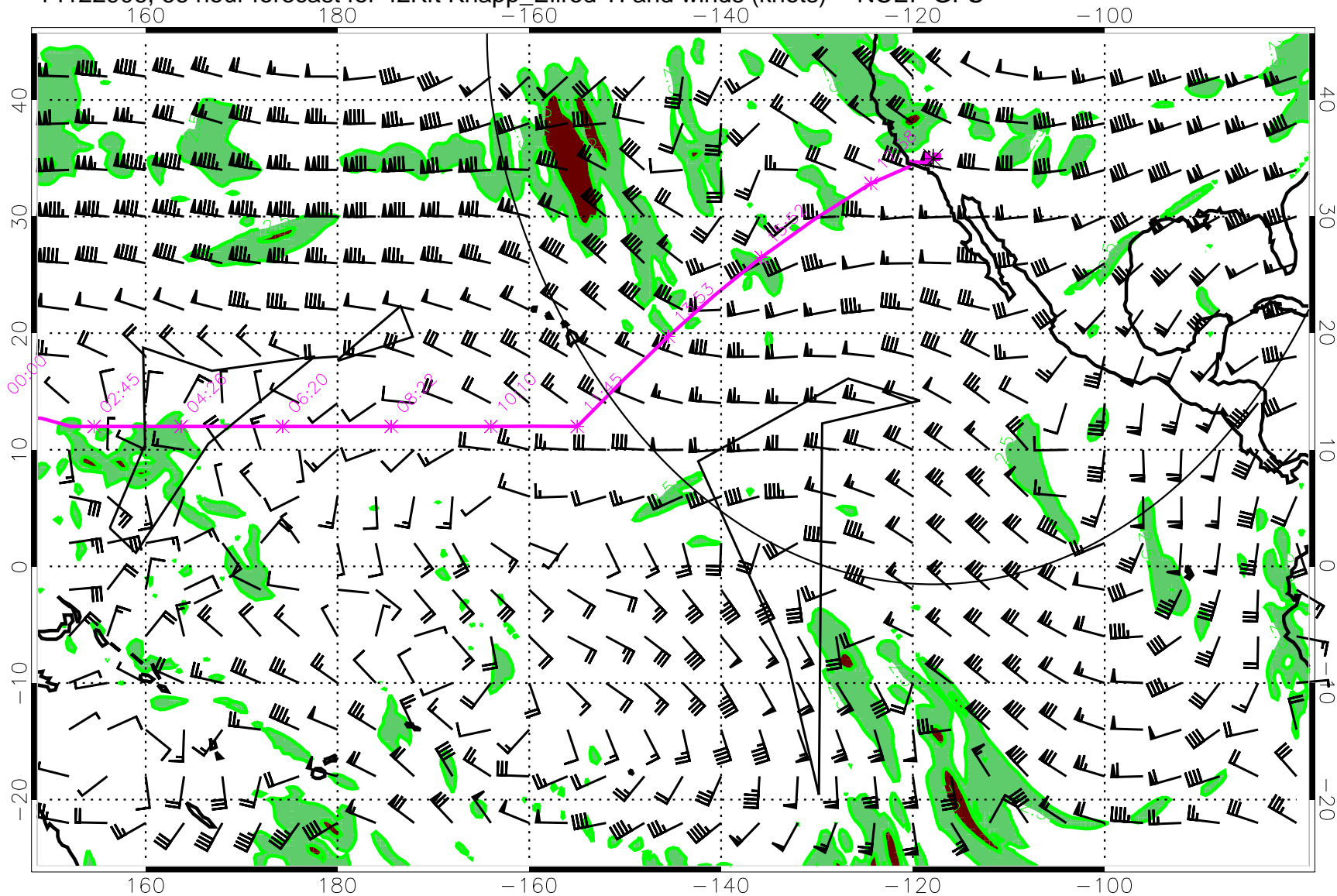
14122906, 66 hour forecast for 42Kft Knapp_Ellrod TI and winds (knots) -- NCEP GFS
