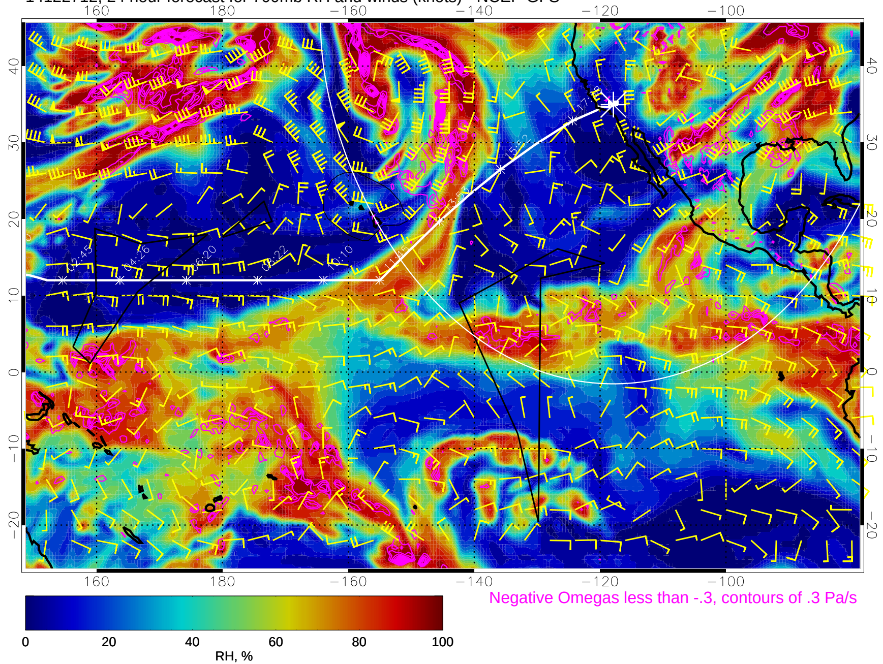
14122712, 24 hour forecast for 700mb RH and winds (knots) - NCEP GFS
