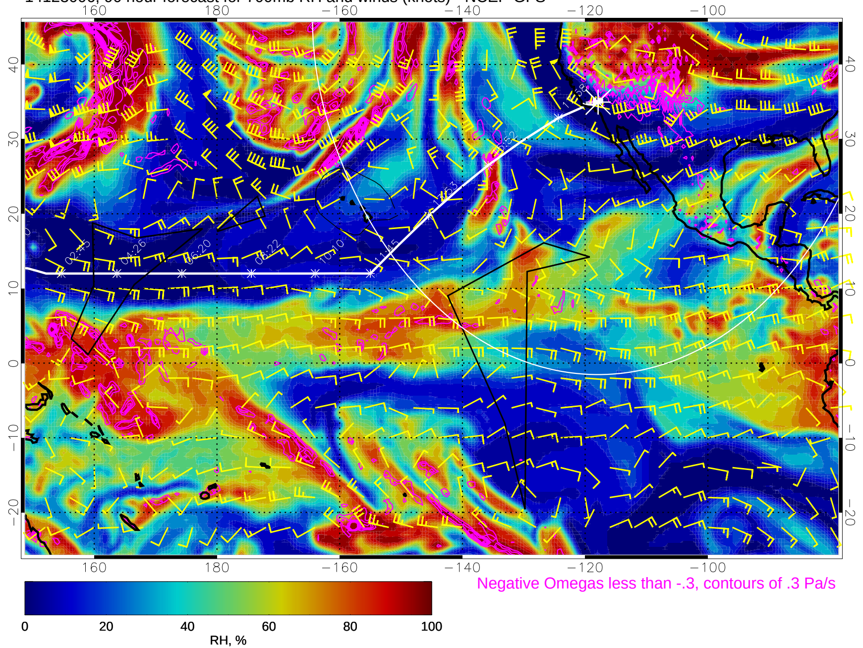
14123006, 90 hour forecast for 700mb RH and winds (knots) - NCEP GFS
