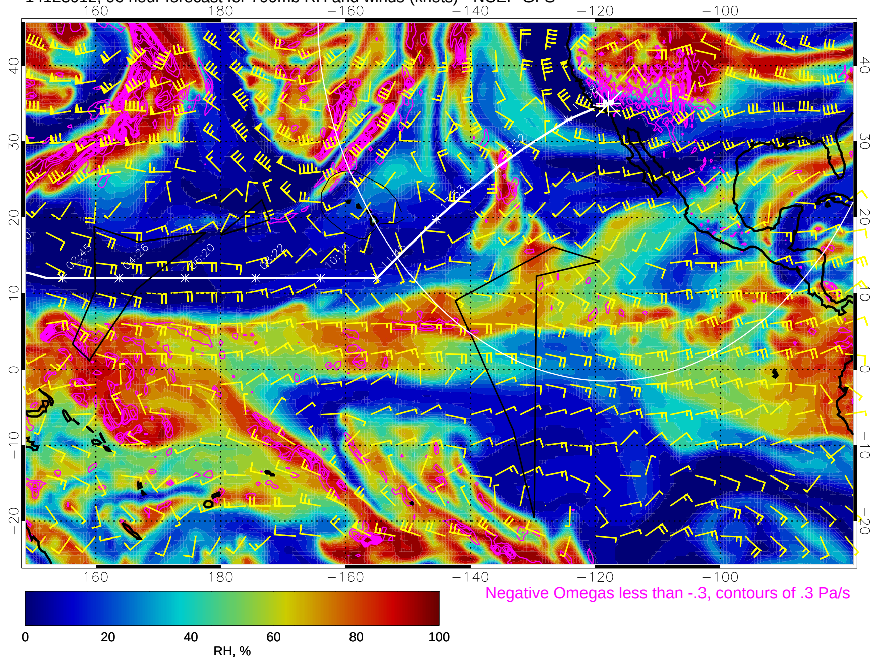
14123012, 96 hour forecast for 700mb RH and winds (knots) - NCEP GFS
