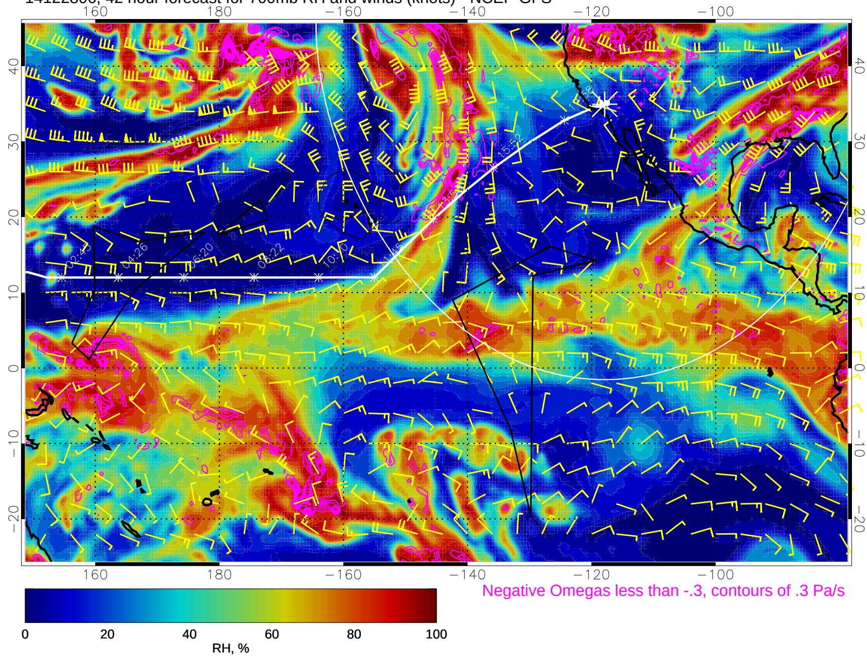
14122806, 42 hour forecast for 700mb RH and winds (knots) - NCEP GFS
