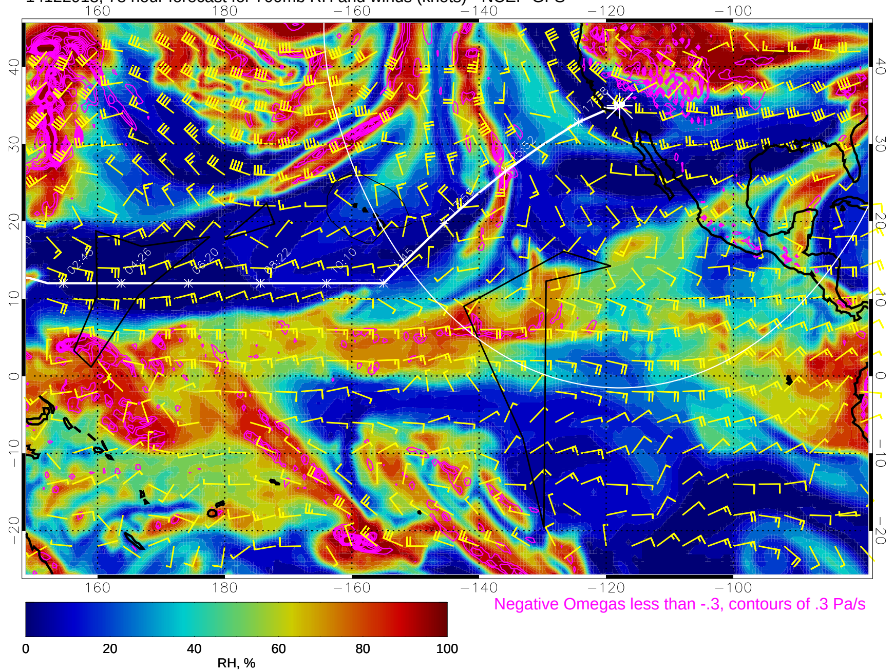
14122918, 78 hour forecast for 700mb RH and winds (knots) - NCEP GFS
