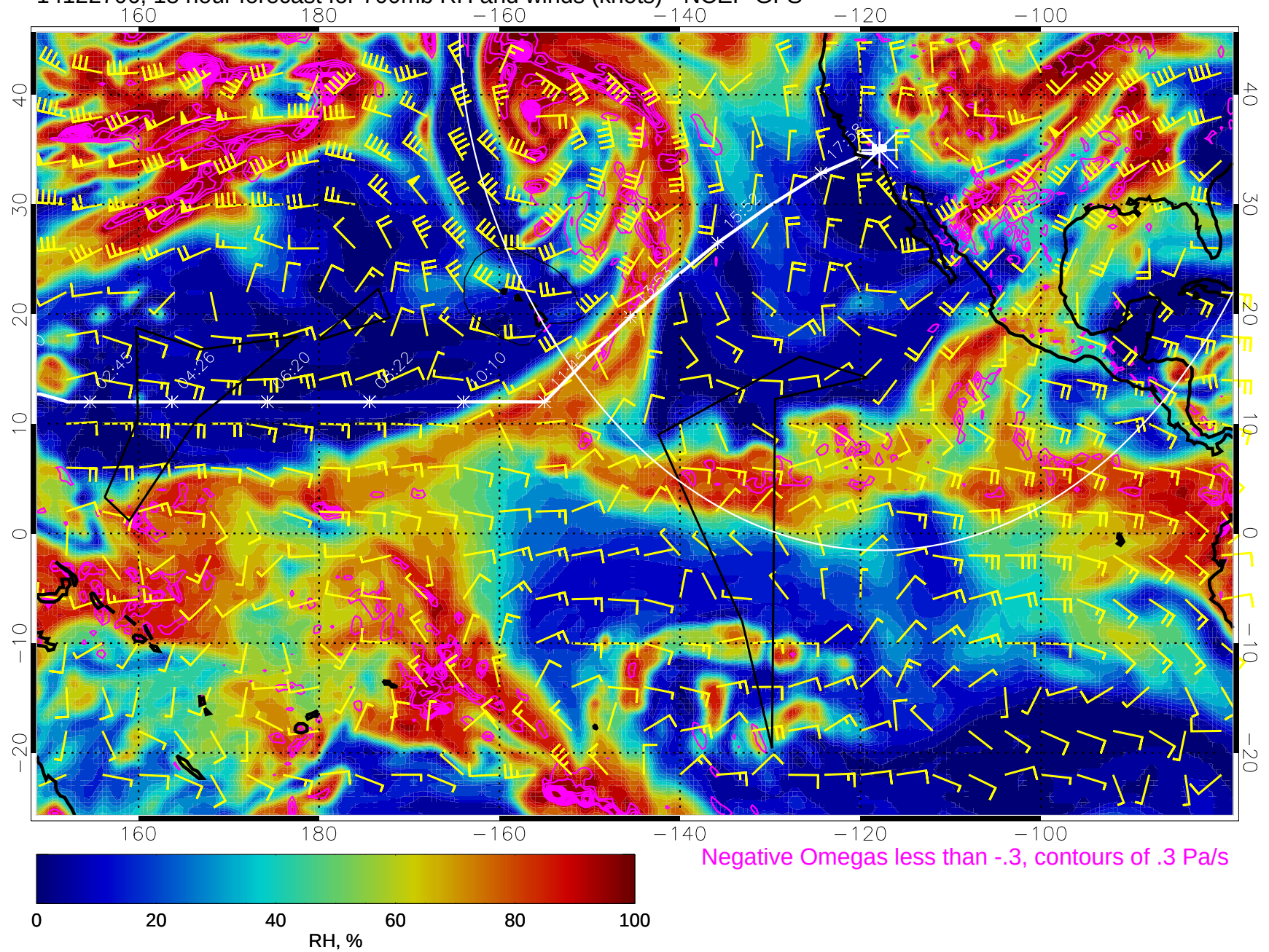
14122706, 18 hour forecast for 700mb RH and winds (knots) - NCEP GFS
