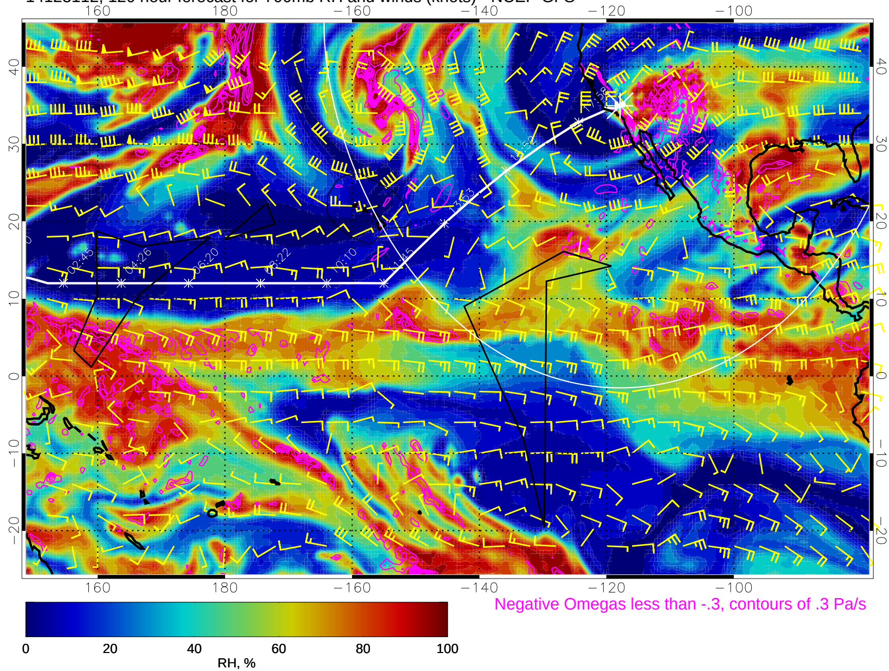
14123112, 120 hour forecast for 700mb RH and winds (knots) - NCEP GFS
