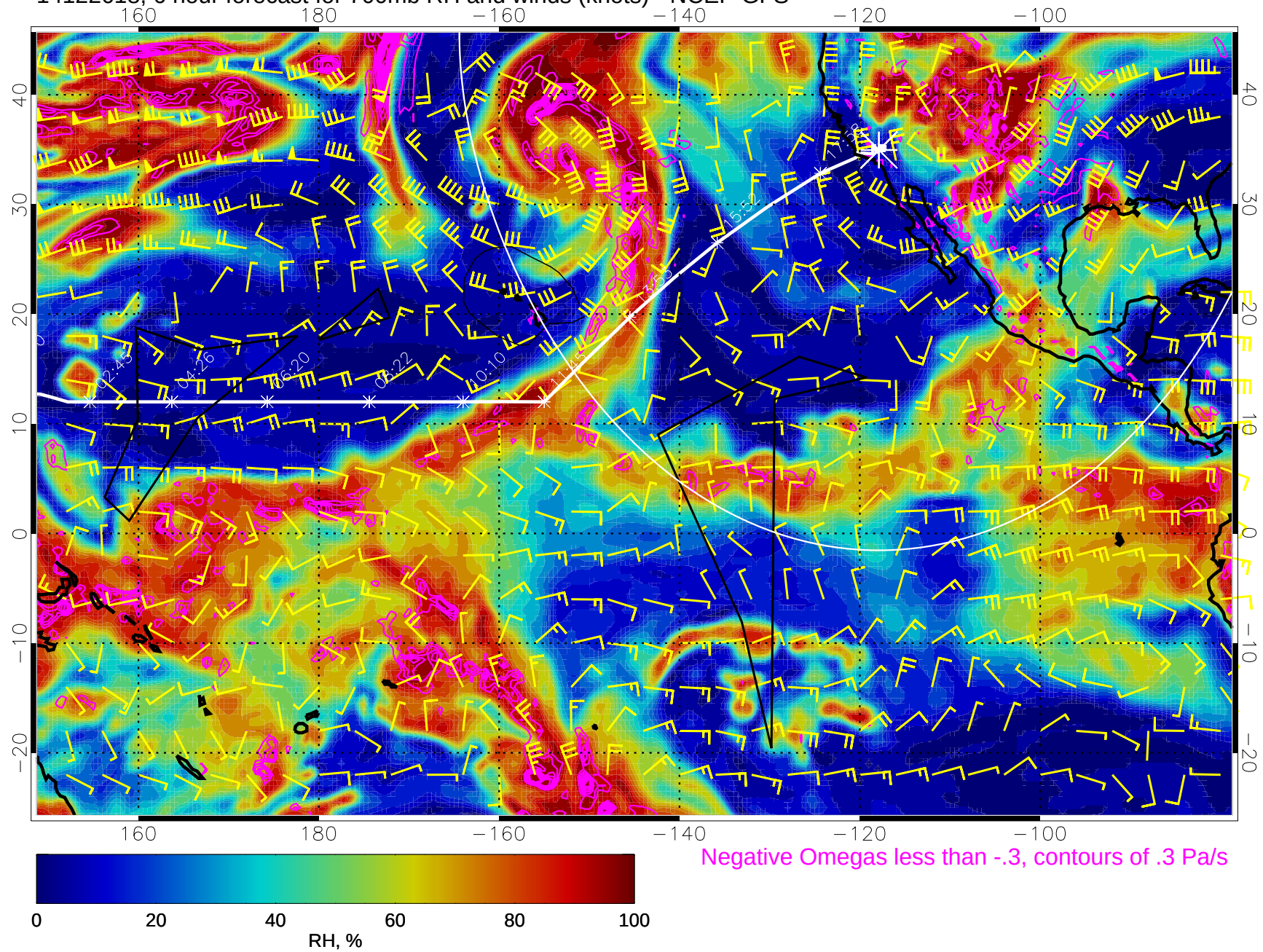
14122618, 6 hour forecast for 700mb RH and winds (knots) - NCEP GFS
