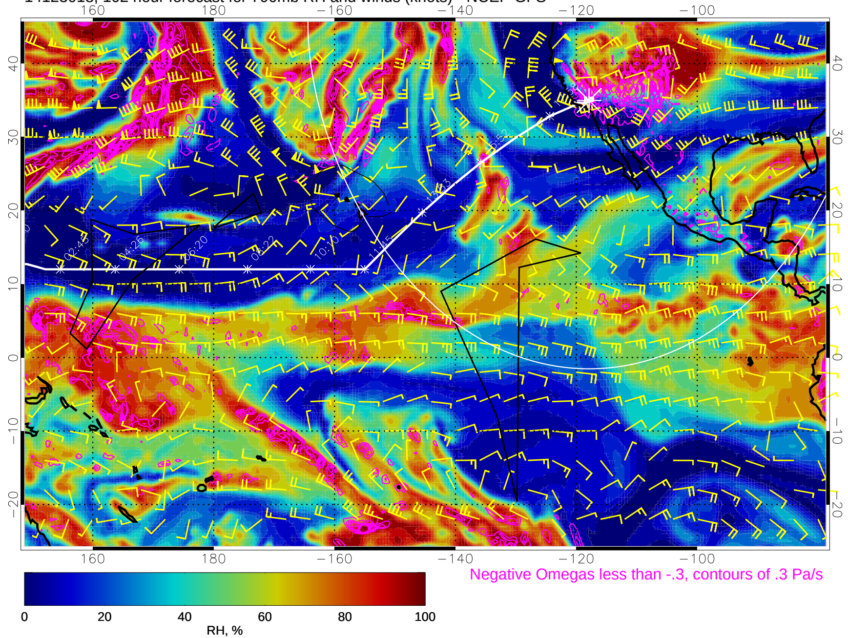
14123018, 102 hour forecast for 700mb RH and winds (knots) - NCEP GFS
