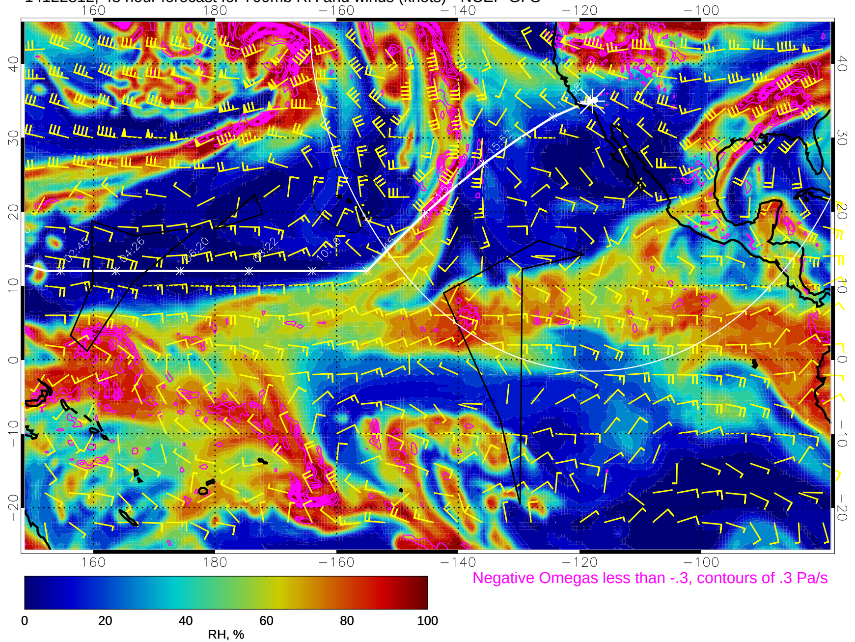
14122812, 48 hour forecast for 700mb RH and winds (knots) - NCEP GFS
