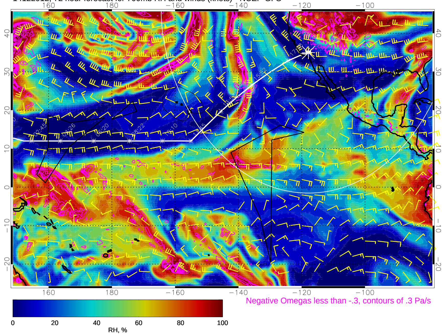
14122912, 72 hour forecast for 700mb RH and winds (knots) - NCEP GFS
