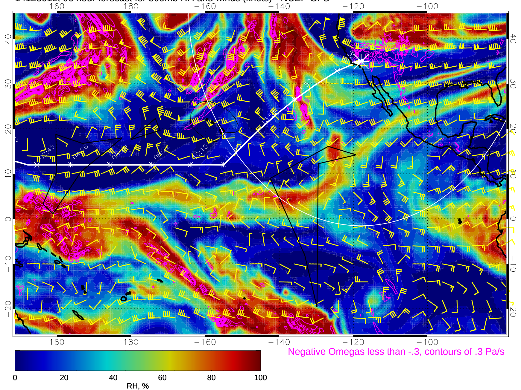
14123012, 96 hour forecast for 500mb RH and winds (knots) - NCEP GFS
