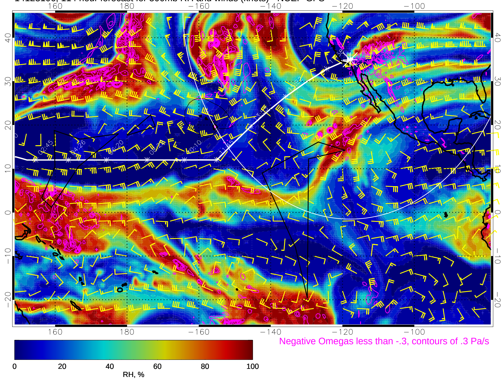
14123106, 114 hour forecast for 500mb RH and winds (knots) - NCEP GFS
