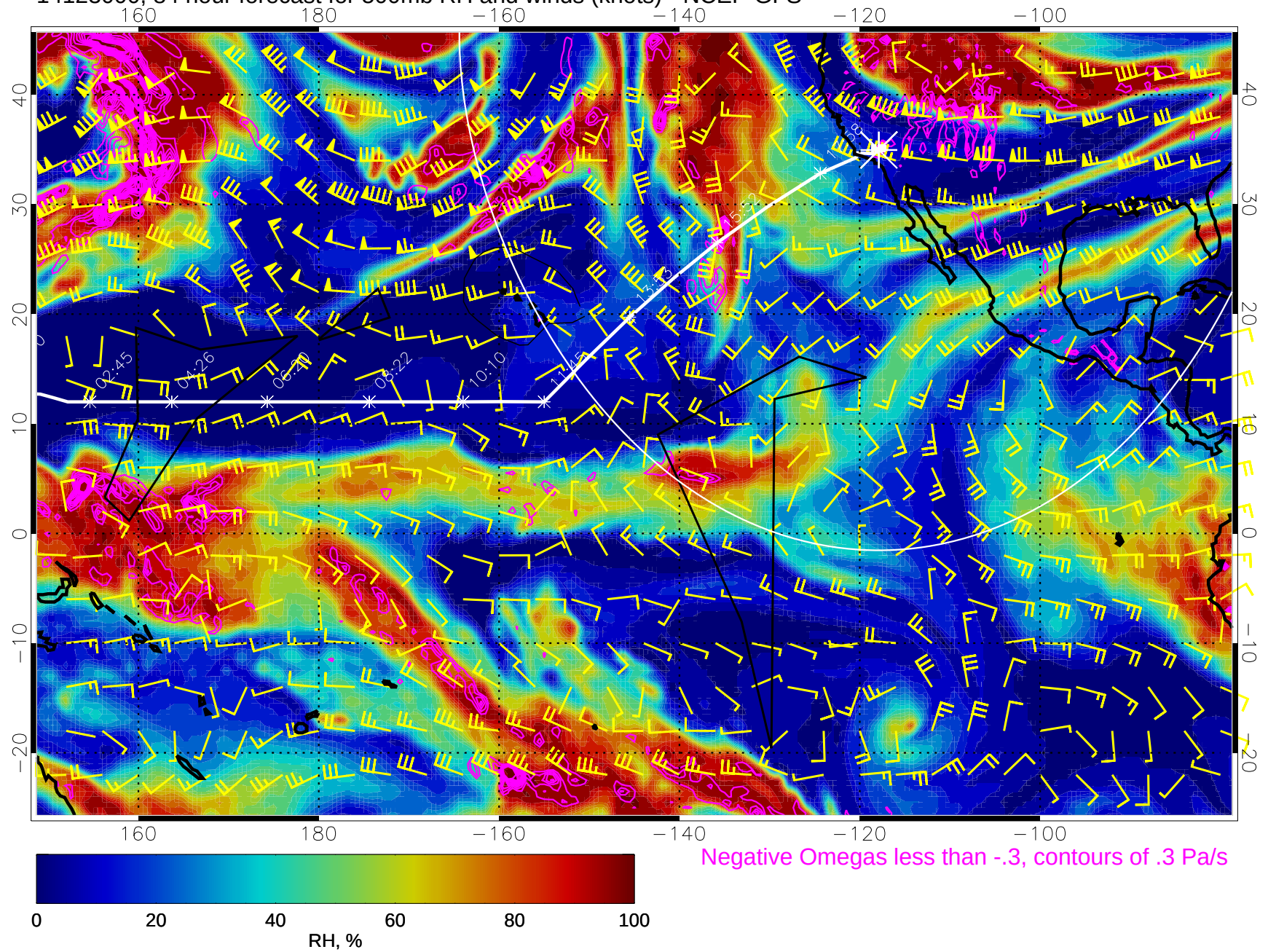
14123000, 84 hour forecast for 500mb RH and winds (knots) - NCEP GFS
