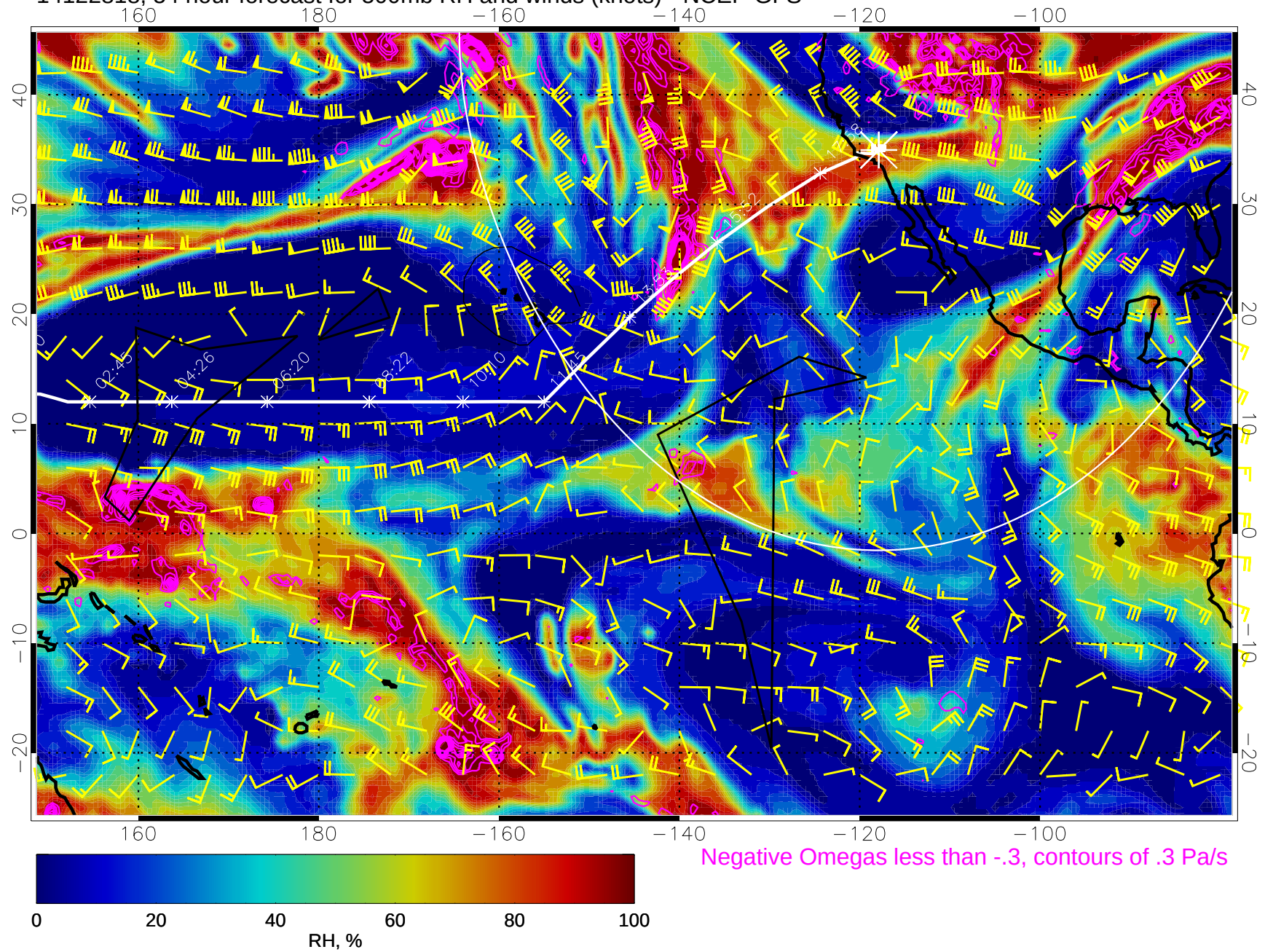
14122818, 54 hour forecast for 500mb RH and winds (knots) - NCEP GFS
