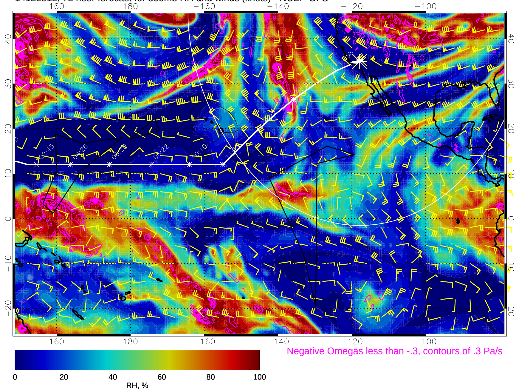
14122912, 72 hour forecast for 500mb RH and winds (knots) - NCEP GFS
