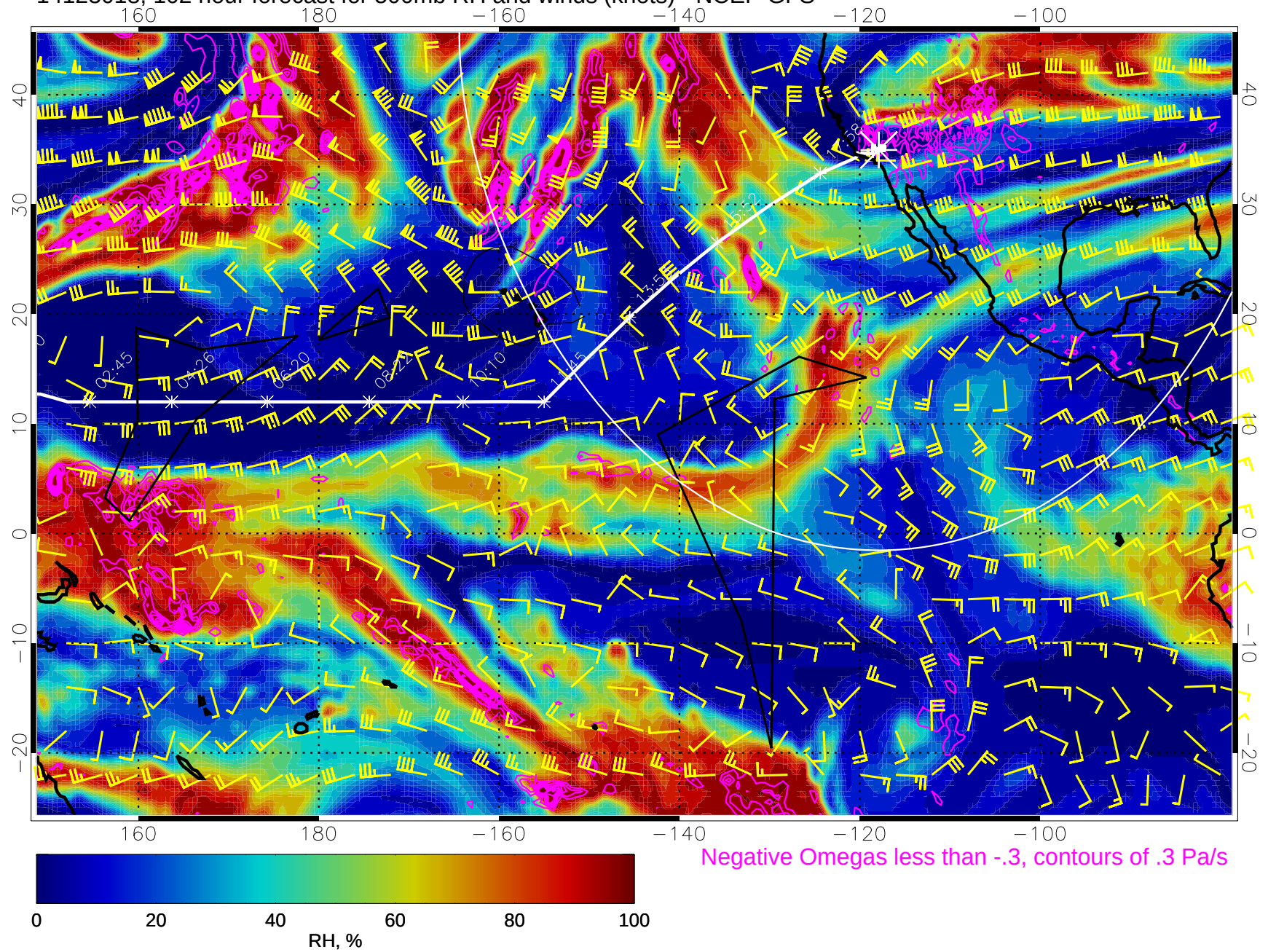
14123018, 102 hour forecast for 500mb RH and winds (knots) - NCEP GFS
