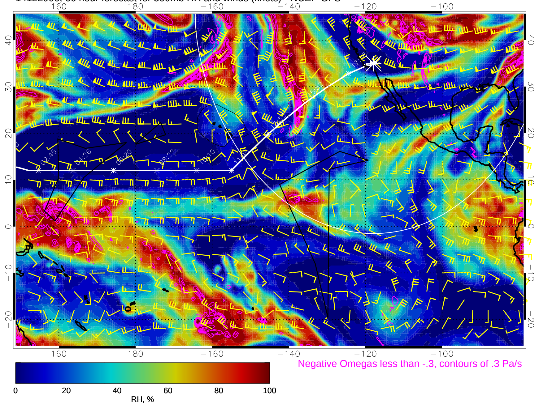
14122906, 66 hour forecast for 500mb RH and winds (knots) - NCEP GFS
