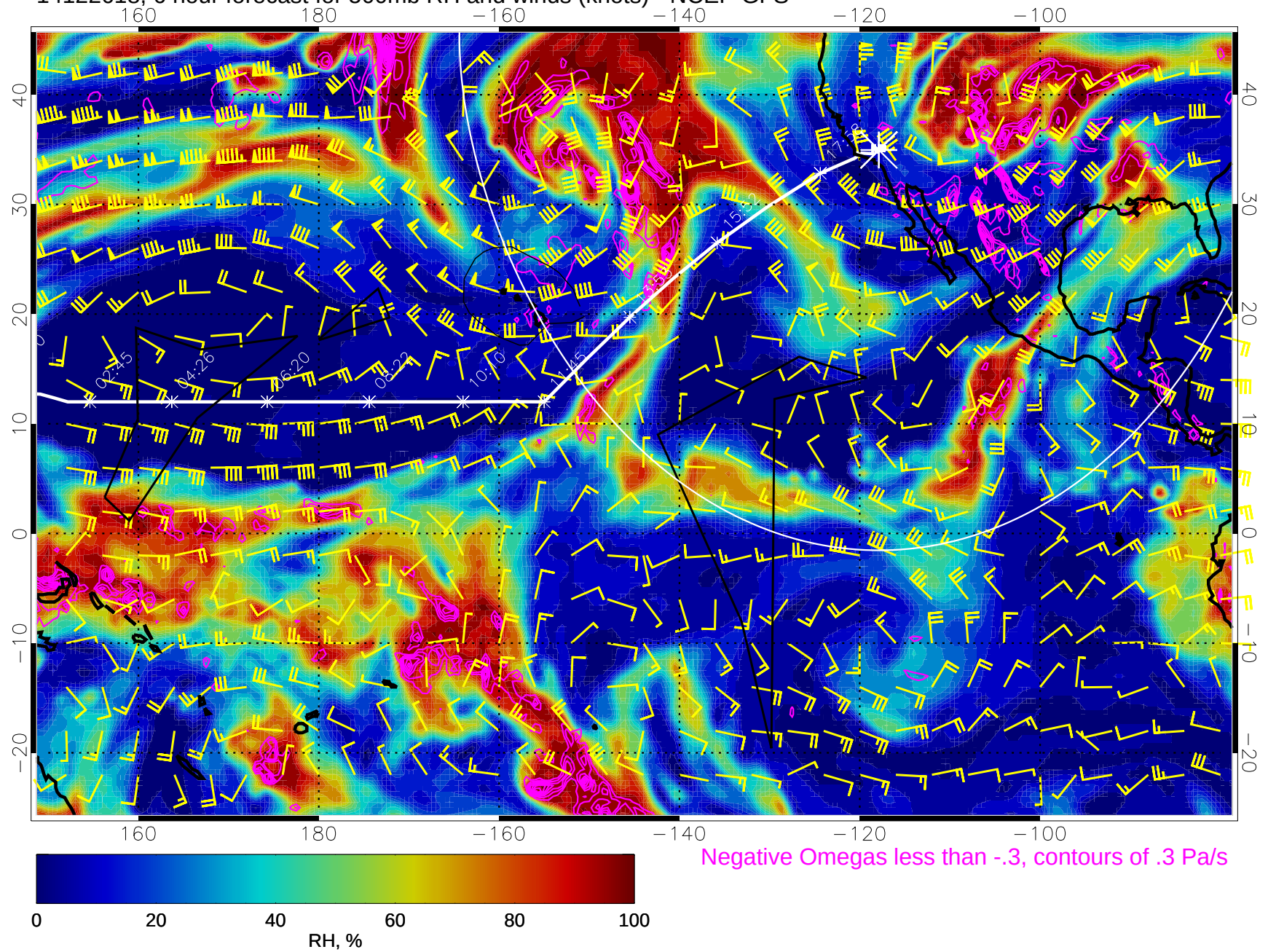
14122618, 6 hour forecast for 500mb RH and winds (knots) - NCEP GFS
