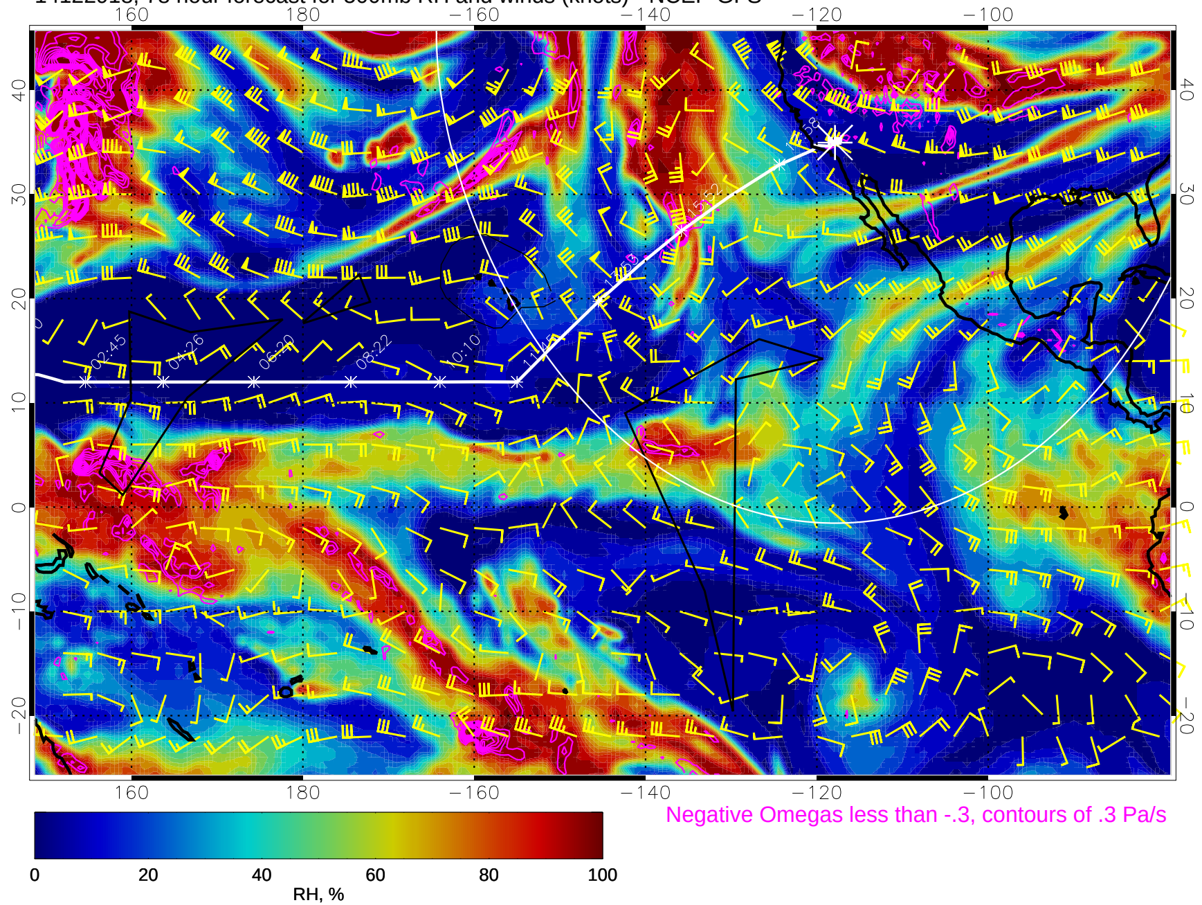
14122918, 78 hour forecast for 500mb RH and winds (knots) - NCEP GFS
