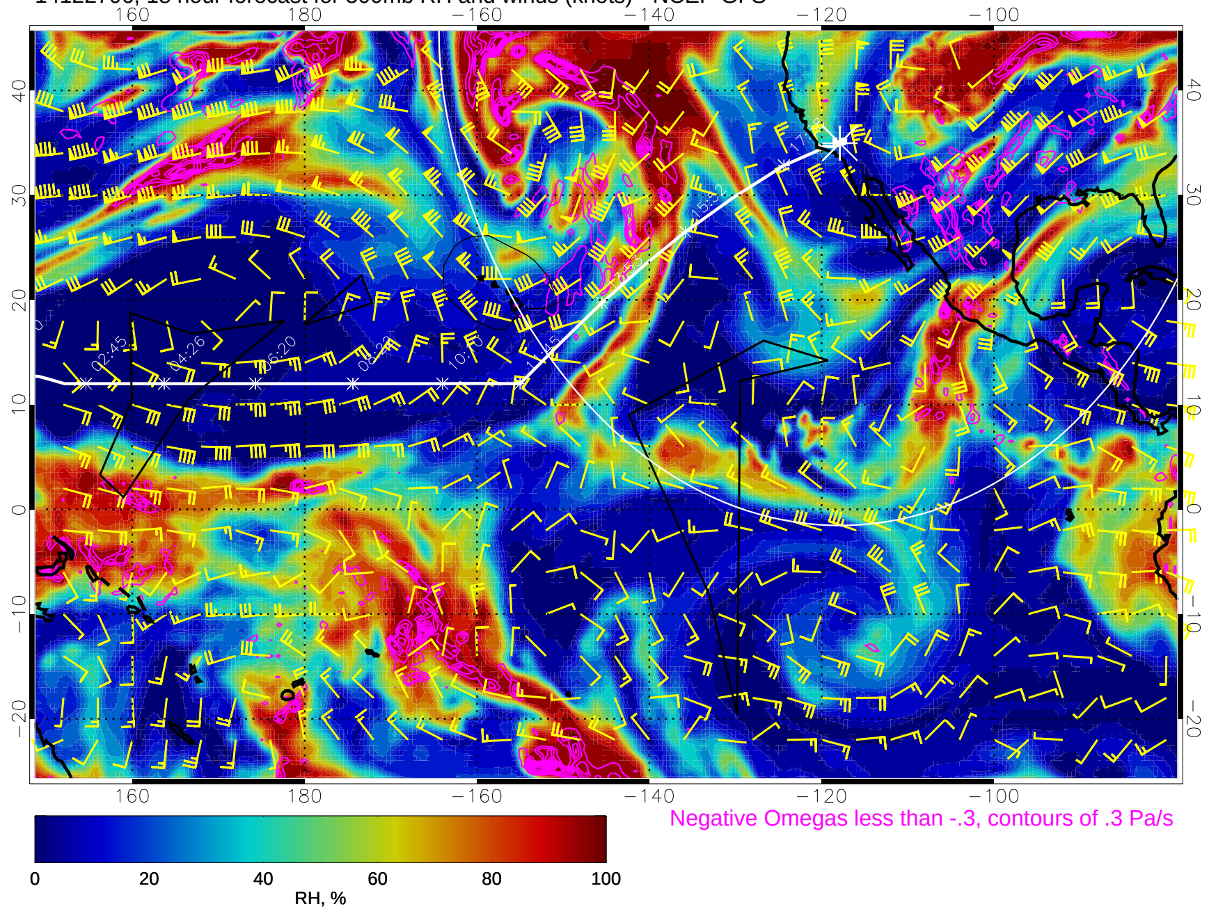
14122706, 18 hour forecast for 500mb RH and winds (knots) - NCEP GFS
