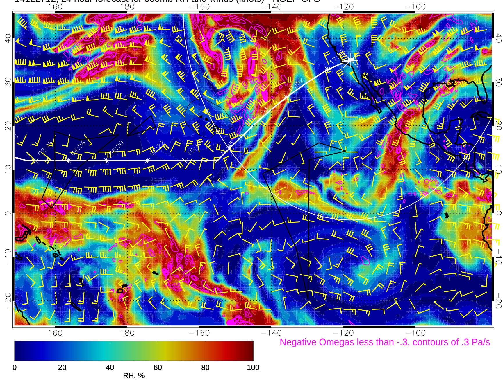
14122712, 24 hour forecast for 500mb RH and winds (knots) - NCEP GFS
