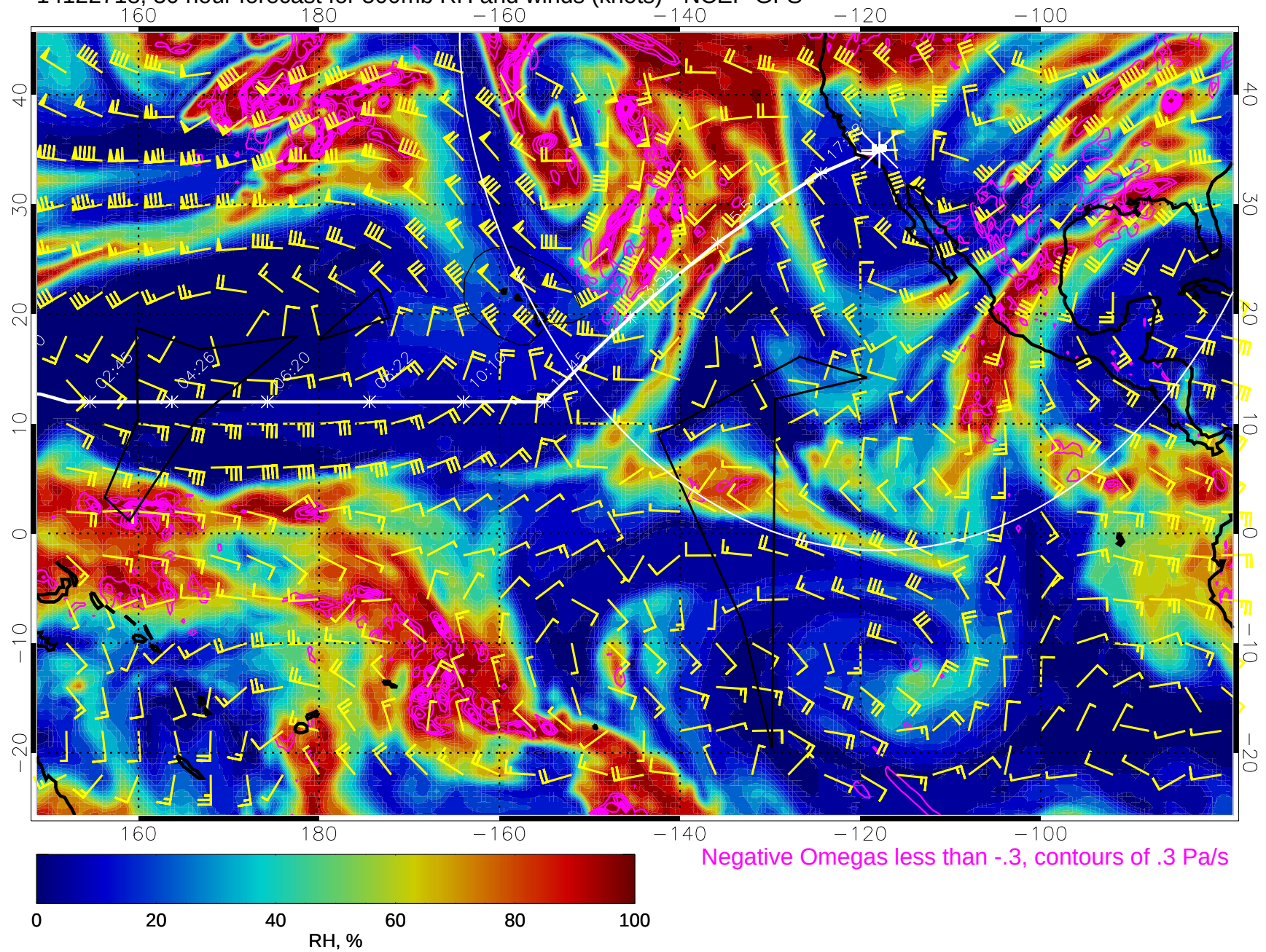
14122718, 30 hour forecast for 500mb RH and winds (knots) - NCEP GFS
