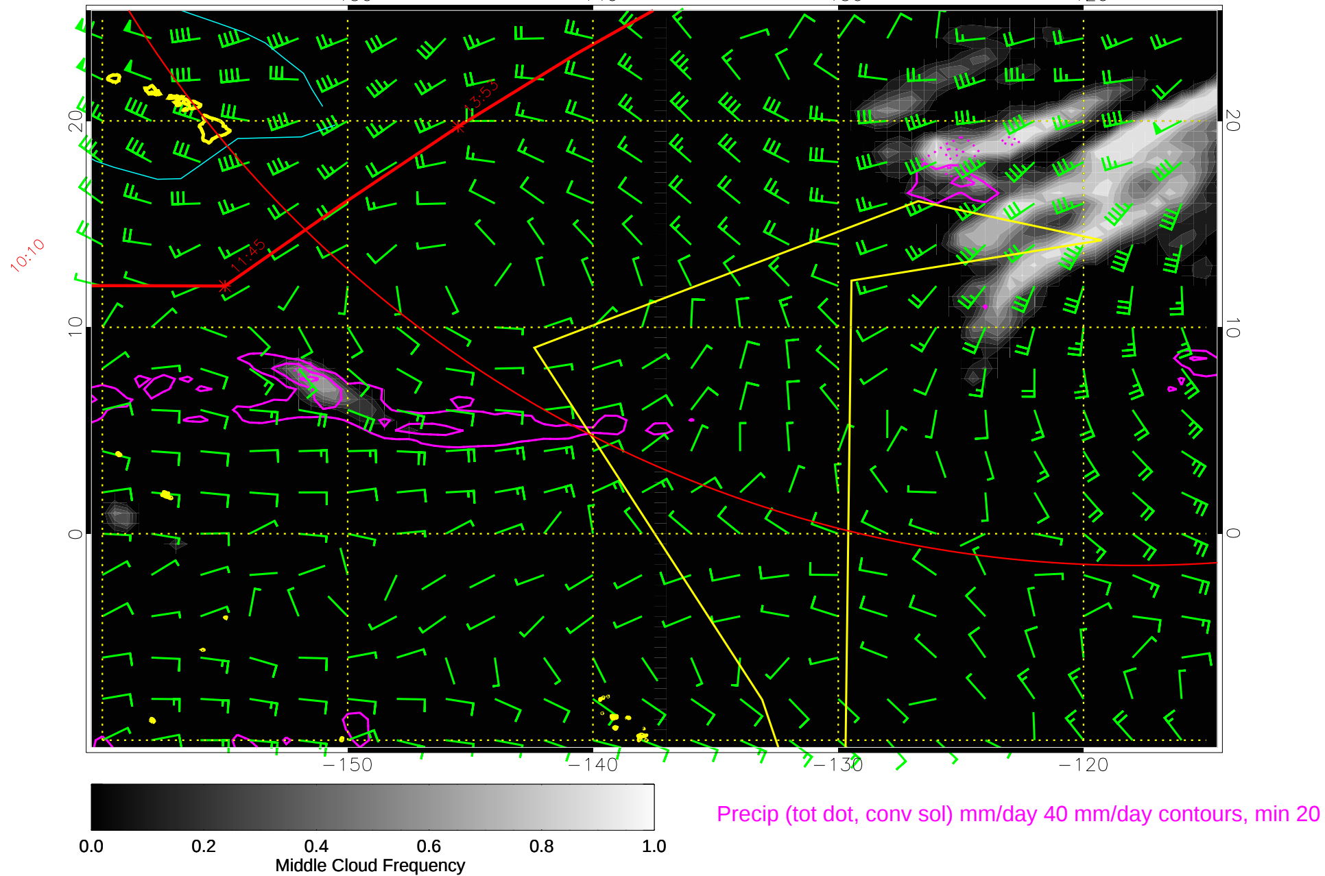
14123112, 120 hour forecast for 500mb winds (knots) and Middle Cloud Frequency -- NCEP GFS
