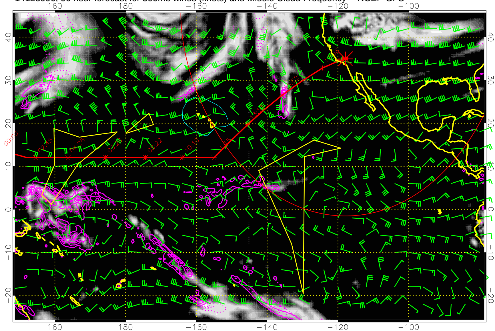
14123006, 90 hour forecast for 500mb winds (knots) and Middle Cloud Frequency -- NCEP GFS
