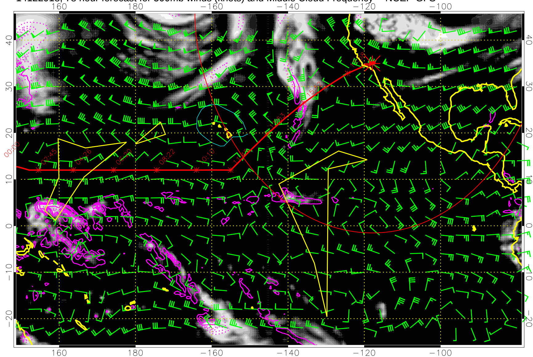
14122918, 78 hour forecast for 500mb winds (knots) and Middle Cloud Frequency -- NCEP GFS
