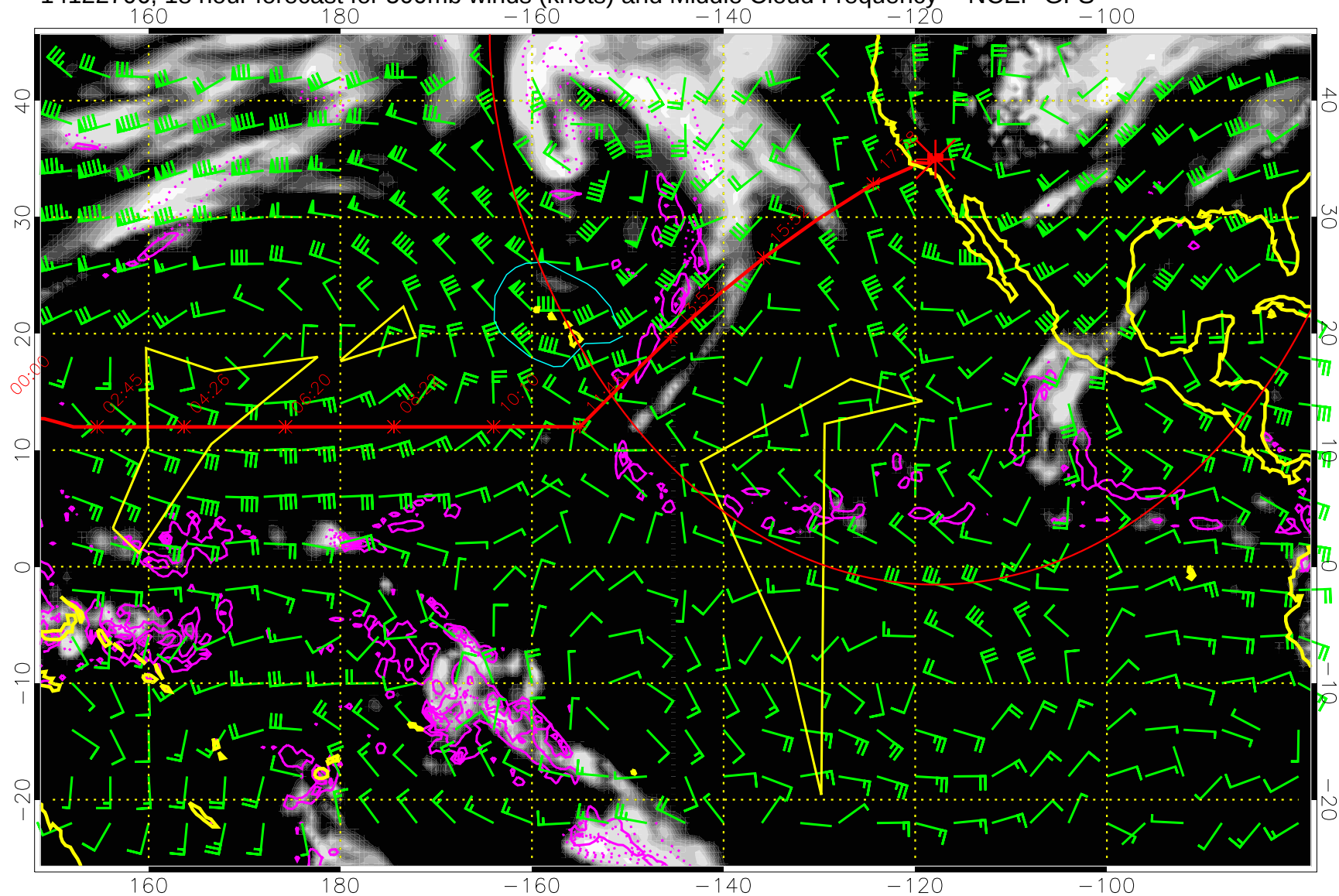
14122706, 18 hour forecast for 500mb winds (knots) and Middle Cloud Frequency -- NCEP GFS
