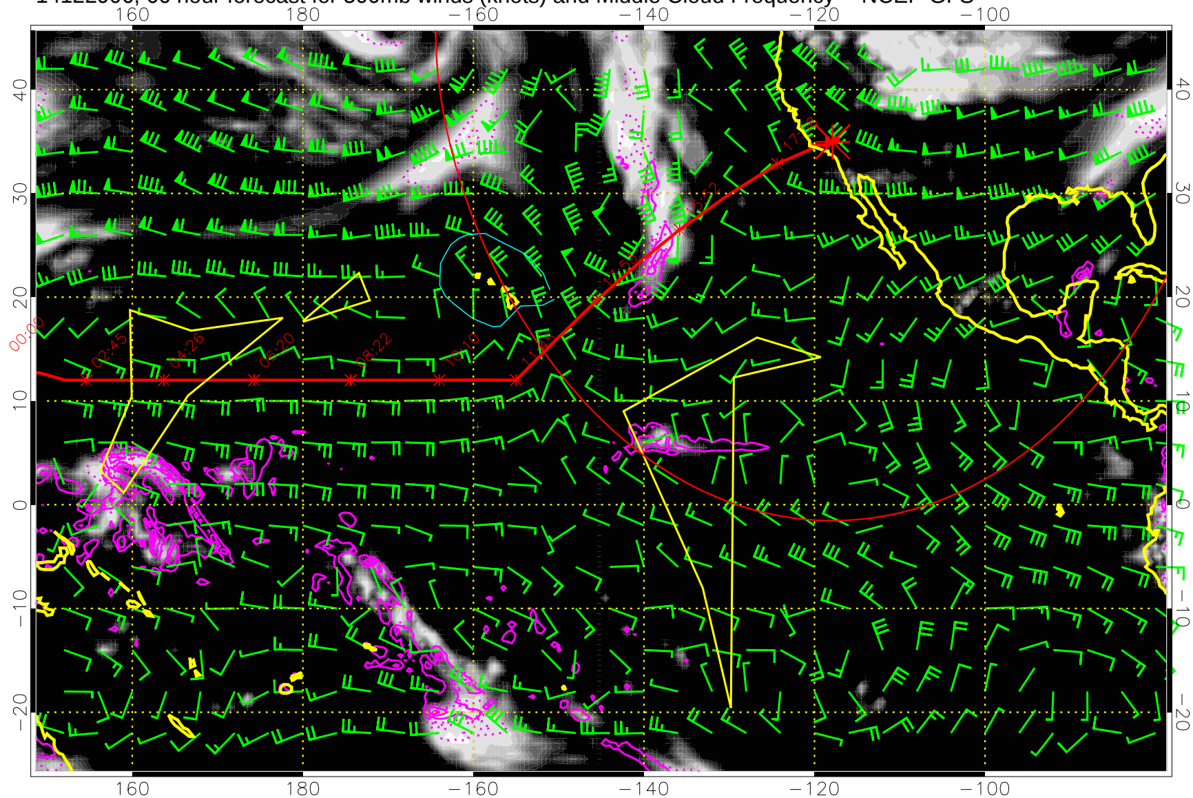
14122906, 66 hour forecast for 500mb winds (knots) and Middle Cloud Frequency -- NCEP GFS
