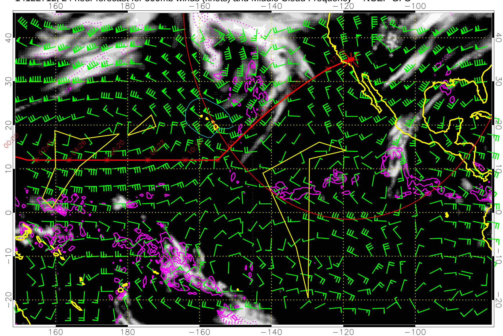
14122712, 24 hour forecast for 500mb winds (knots) and Middle Cloud Frequency -- NCEP GFS
