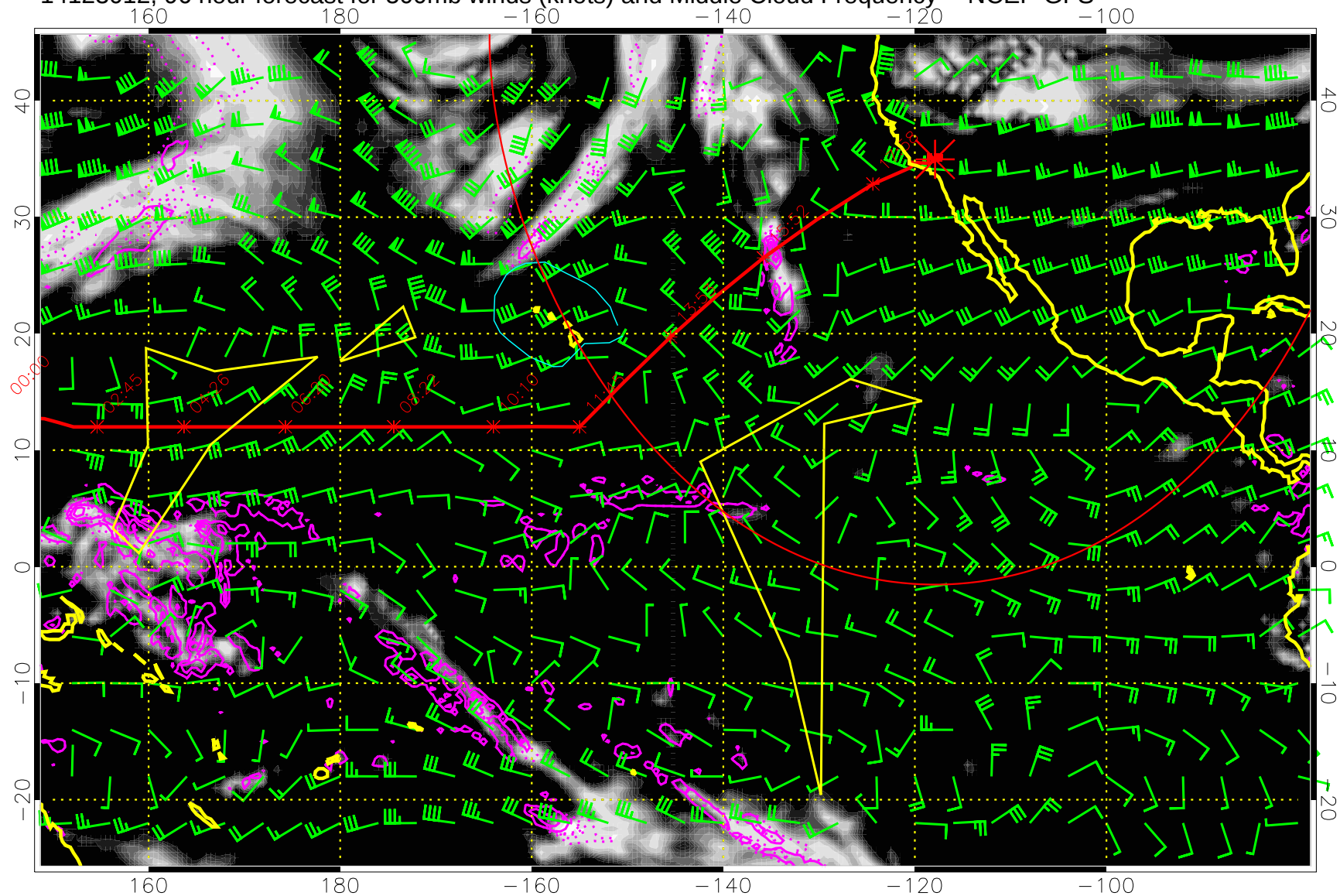
14123012, 96 hour forecast for 500mb winds (knots) and Middle Cloud Frequency -- NCEP GFS
