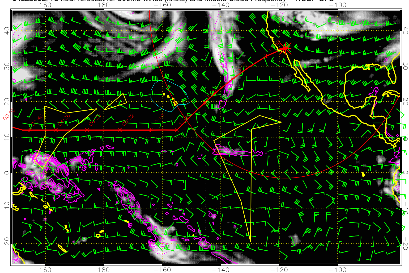
14122912, 72 hour forecast for 500mb winds (knots) and Middle Cloud Frequency -- NCEP GFS
