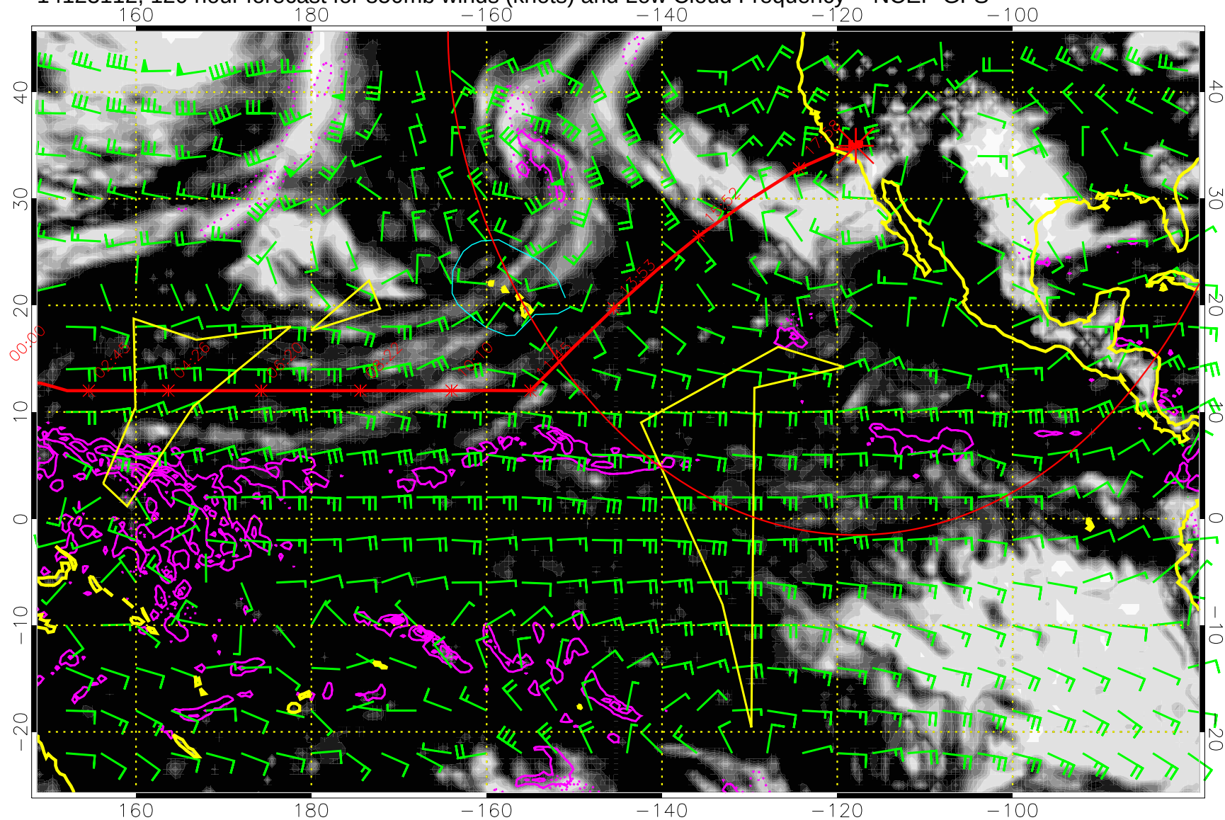
14123112, 120 hour forecast for 850mb winds (knots) and Low Cloud Frequency -- NCEP GFS
