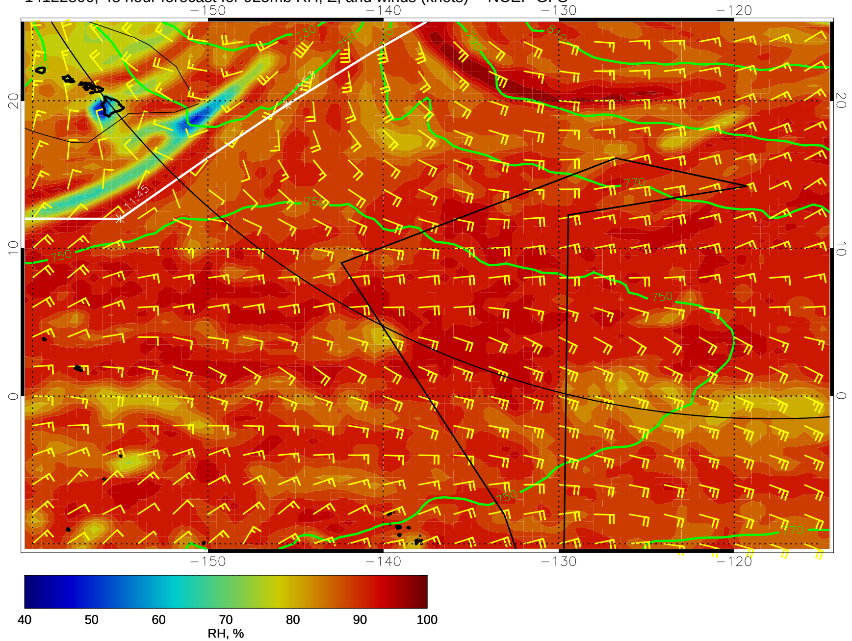
14122800, 48 hour forecast for 925mb RH, Z, and winds (knots) -- NCEP GFS
