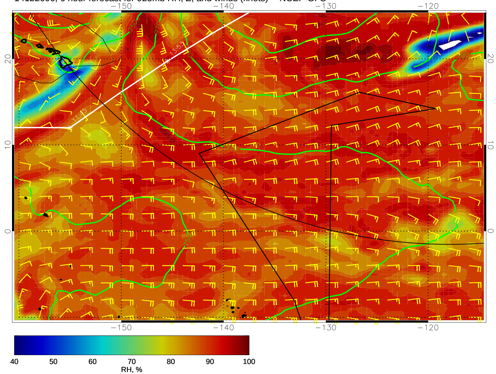
14122606, 6 hour forecast for 925mb RH, Z, and winds (knots) -- NCEP GFS
