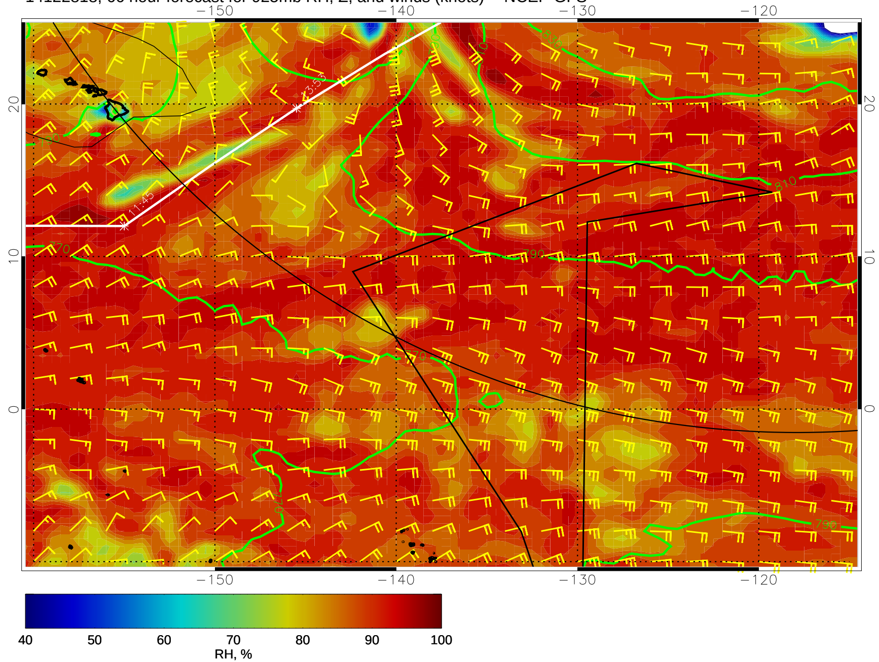
14122818, 66 hour forecast for 925mb RH, Z, and winds (knots) -- NCEP GFS
