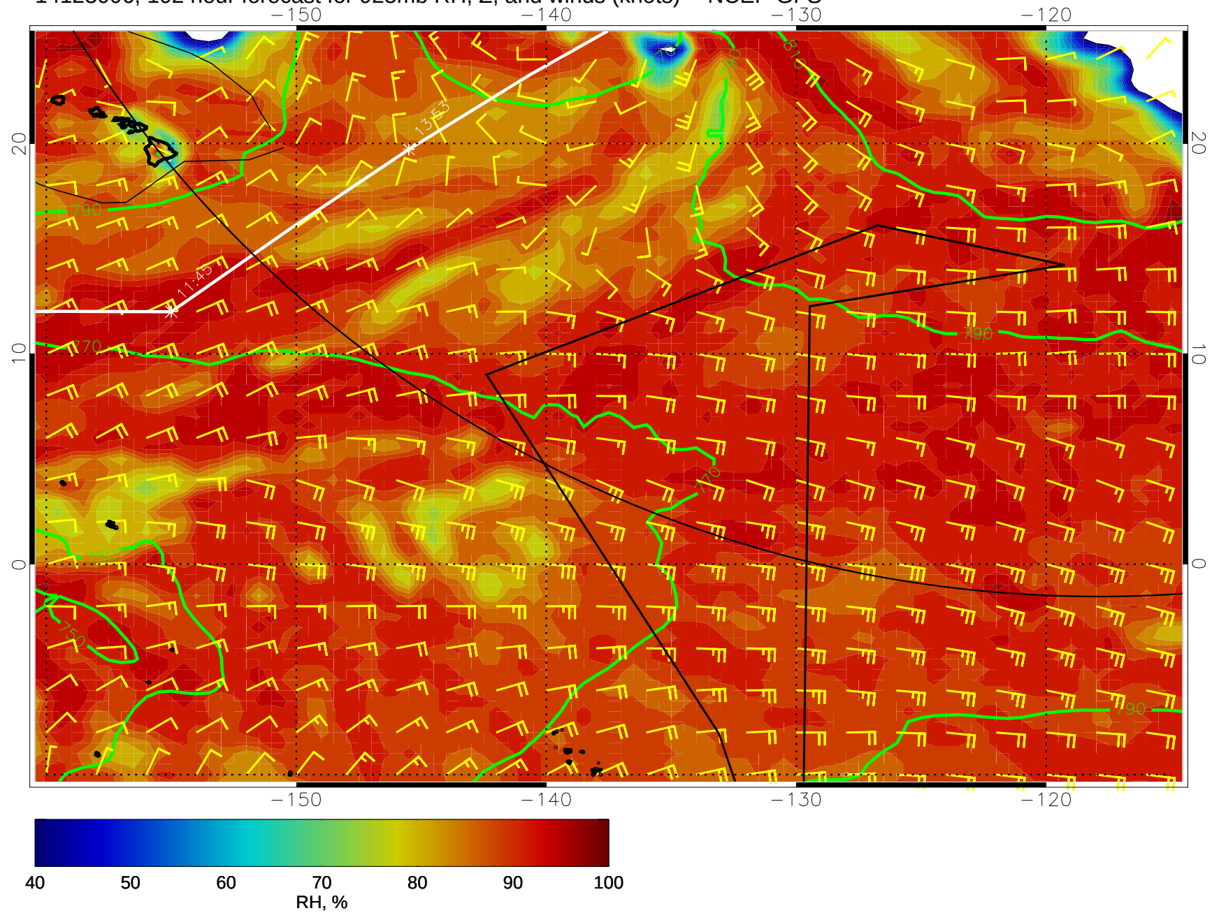
14123006, 102 hour forecast for 925mb RH, Z, and winds (knots) -- NCEP GFS
