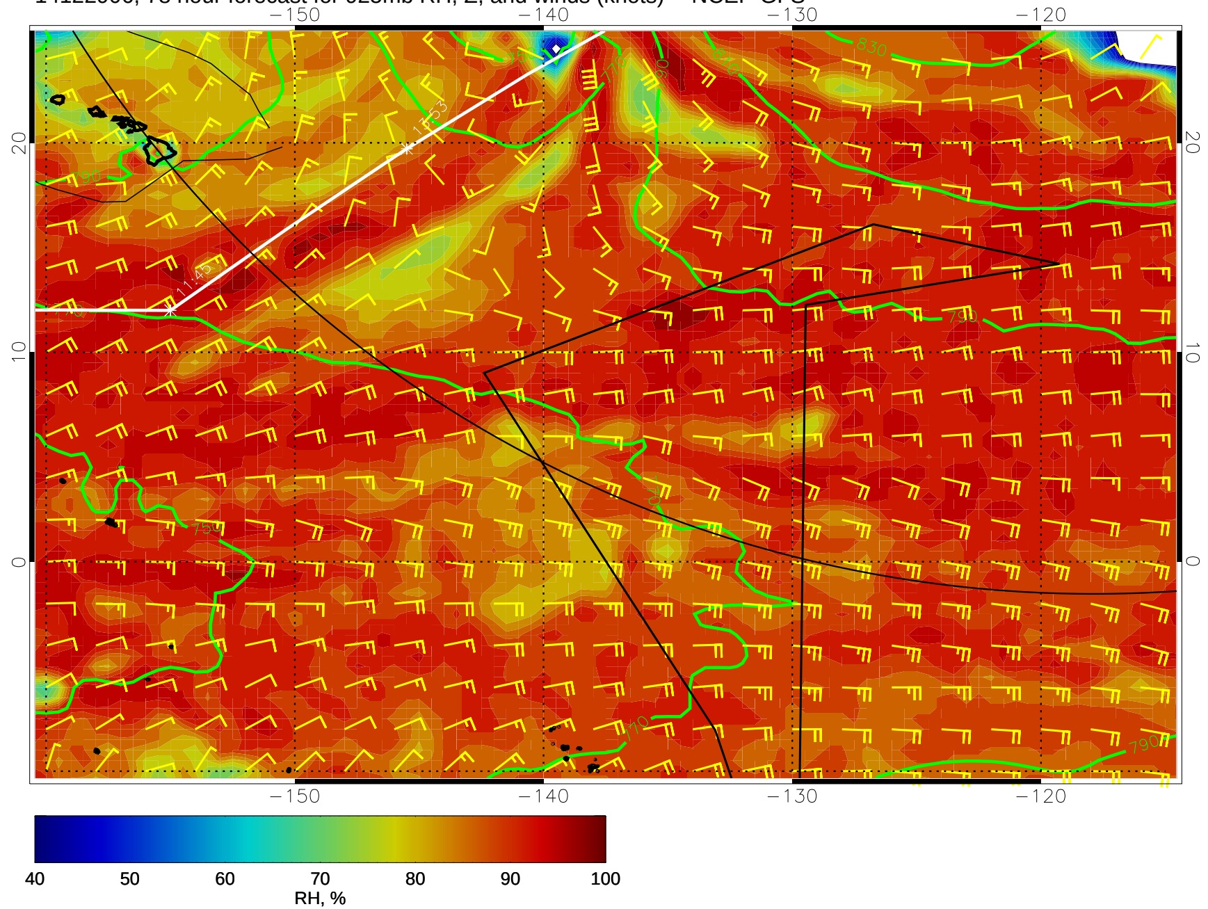
14122906, 78 hour forecast for 925mb RH, Z, and winds (knots) -- NCEP GFS
