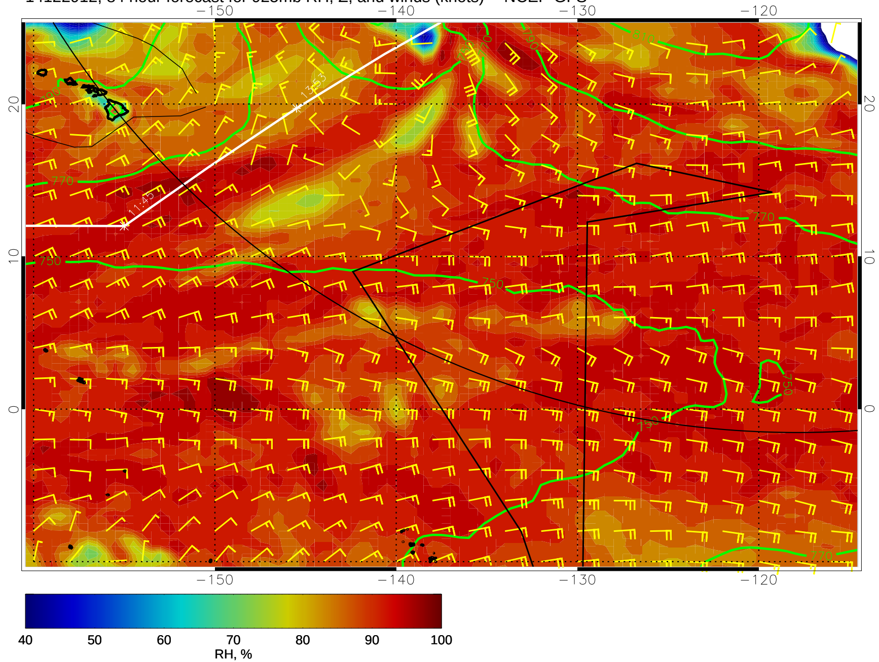
14122912, 84 hour forecast for 925mb RH, Z, and winds (knots) -- NCEP GFS
