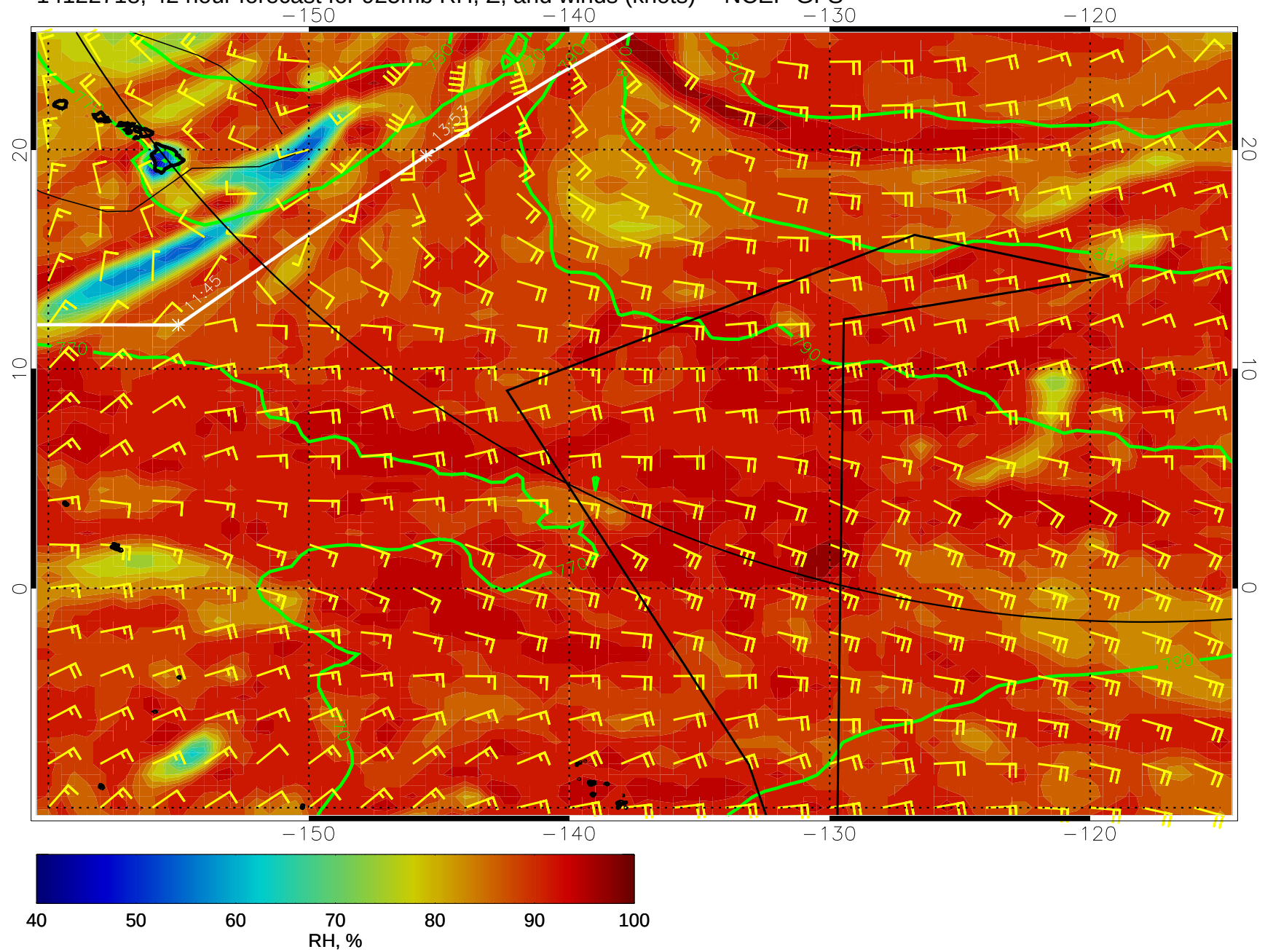
14122718, 42 hour forecast for 925mb RH, Z, and winds (knots) -- NCEP GFS
