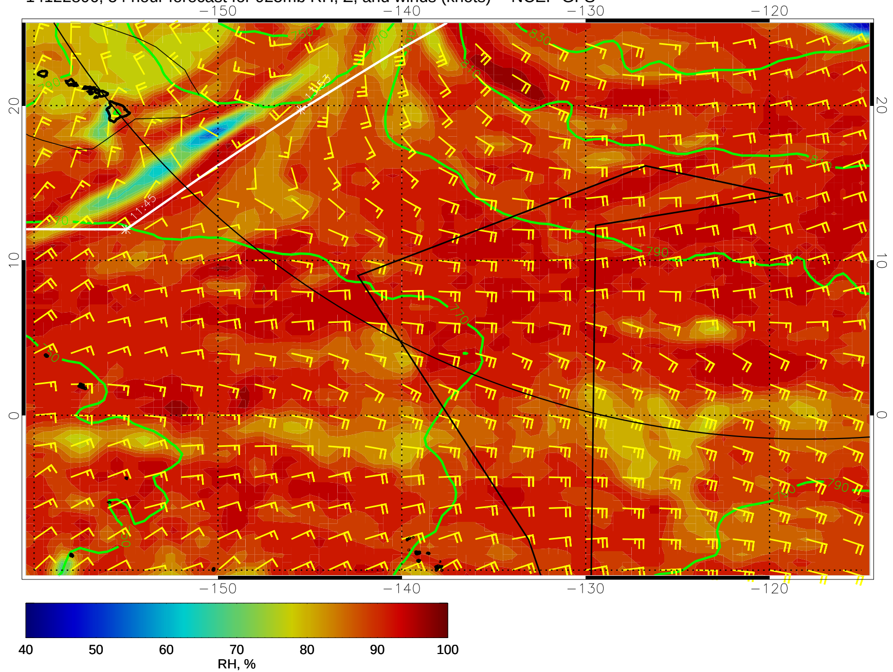
14122806, 54 hour forecast for 925mb RH, Z, and winds (knots) -- NCEP GFS
