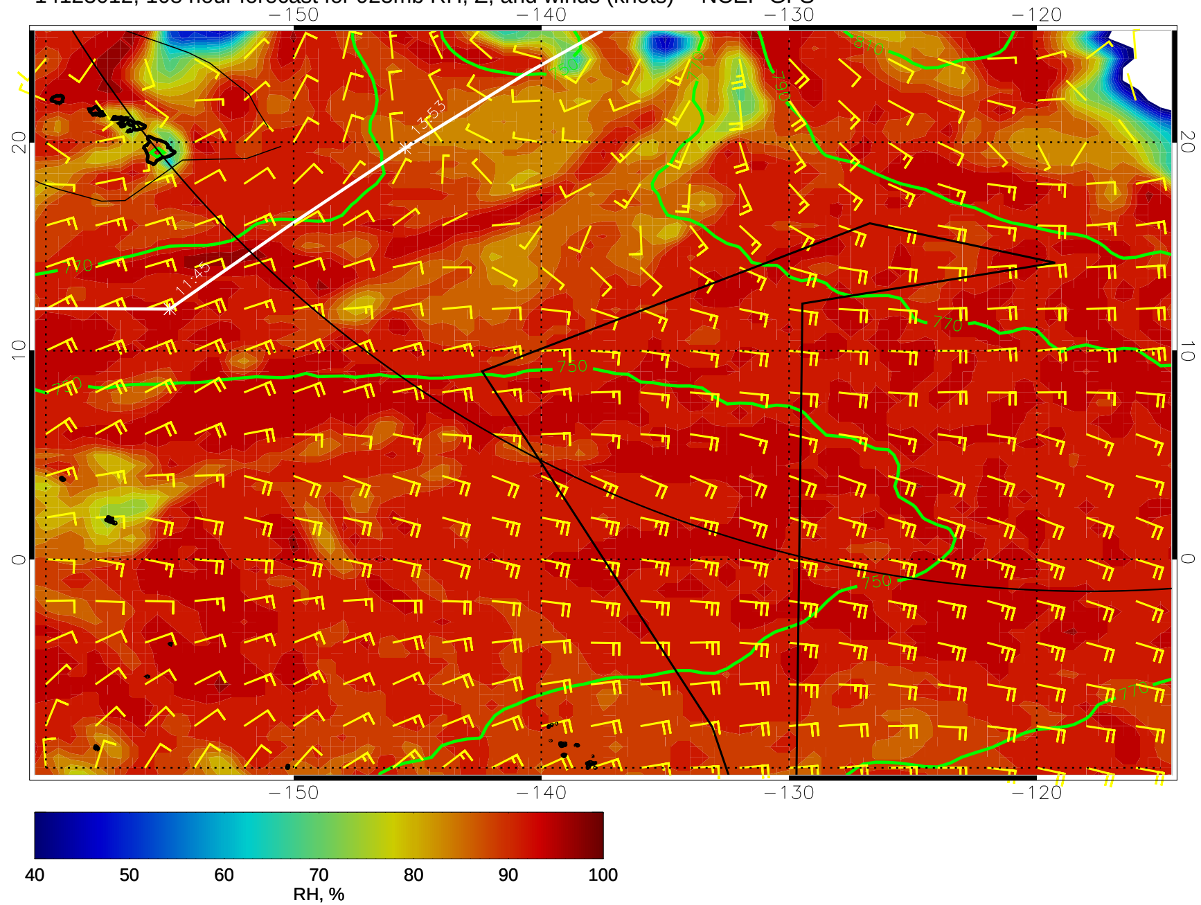
14123012, 108 hour forecast for 925mb RH, Z, and winds (knots) -- NCEP GFS
