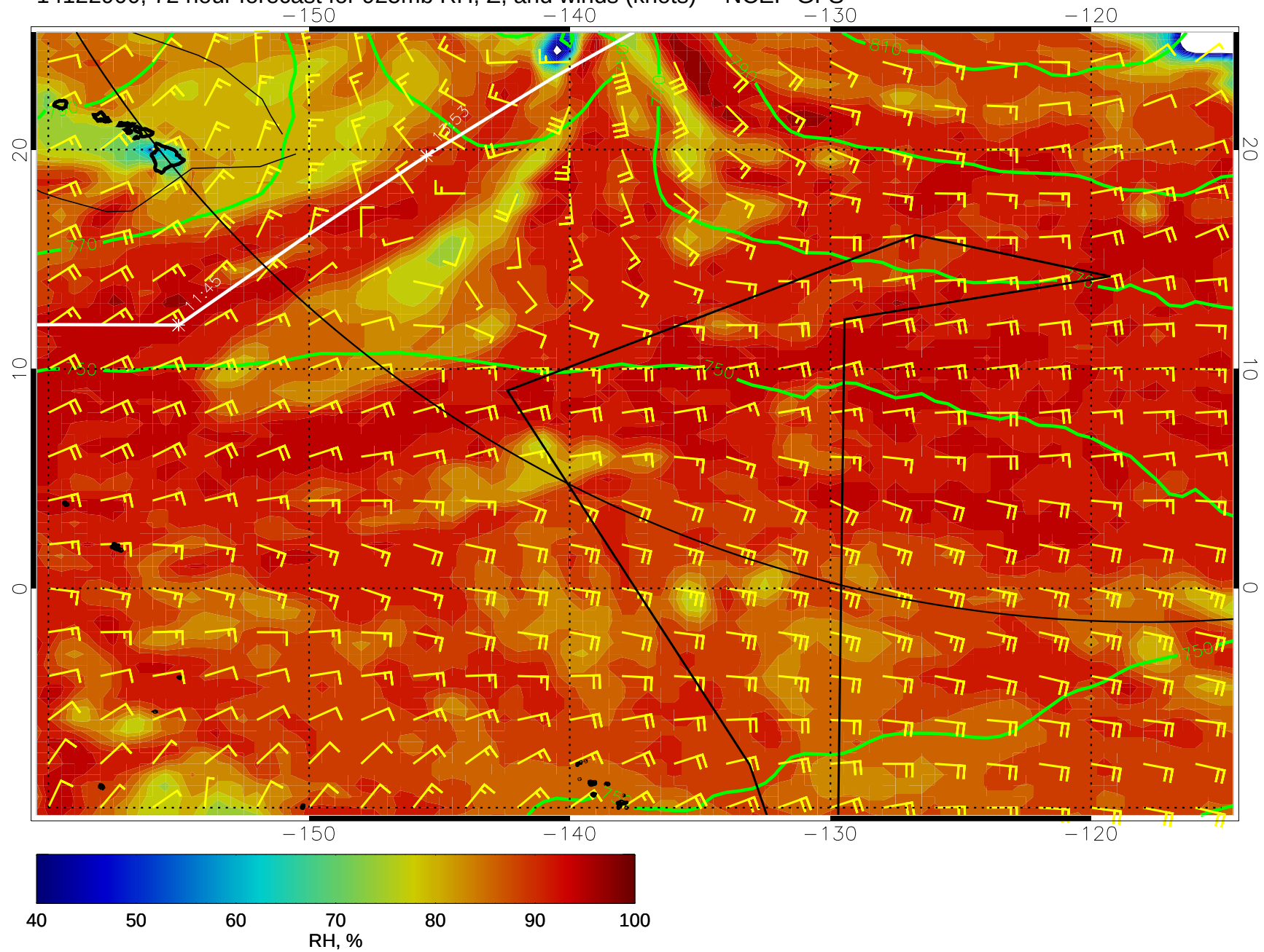
14122900, 72 hour forecast for 925mb RH, Z, and winds (knots) -- NCEP GFS
