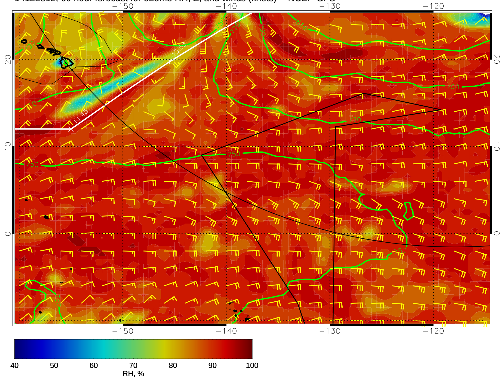
14122812, 60 hour forecast for 925mb RH, Z, and winds (knots) -- NCEP GFS
