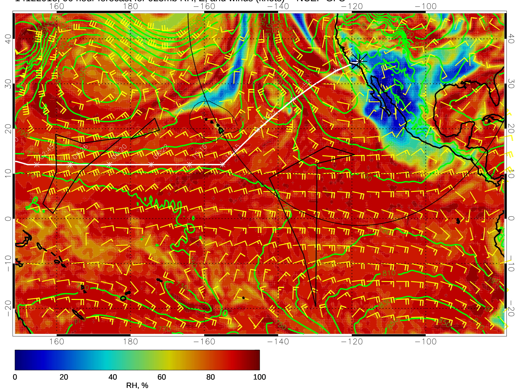
14122918, 90 hour forecast for 925mb RH, Z, and winds (knots) -- NCEP GFS
