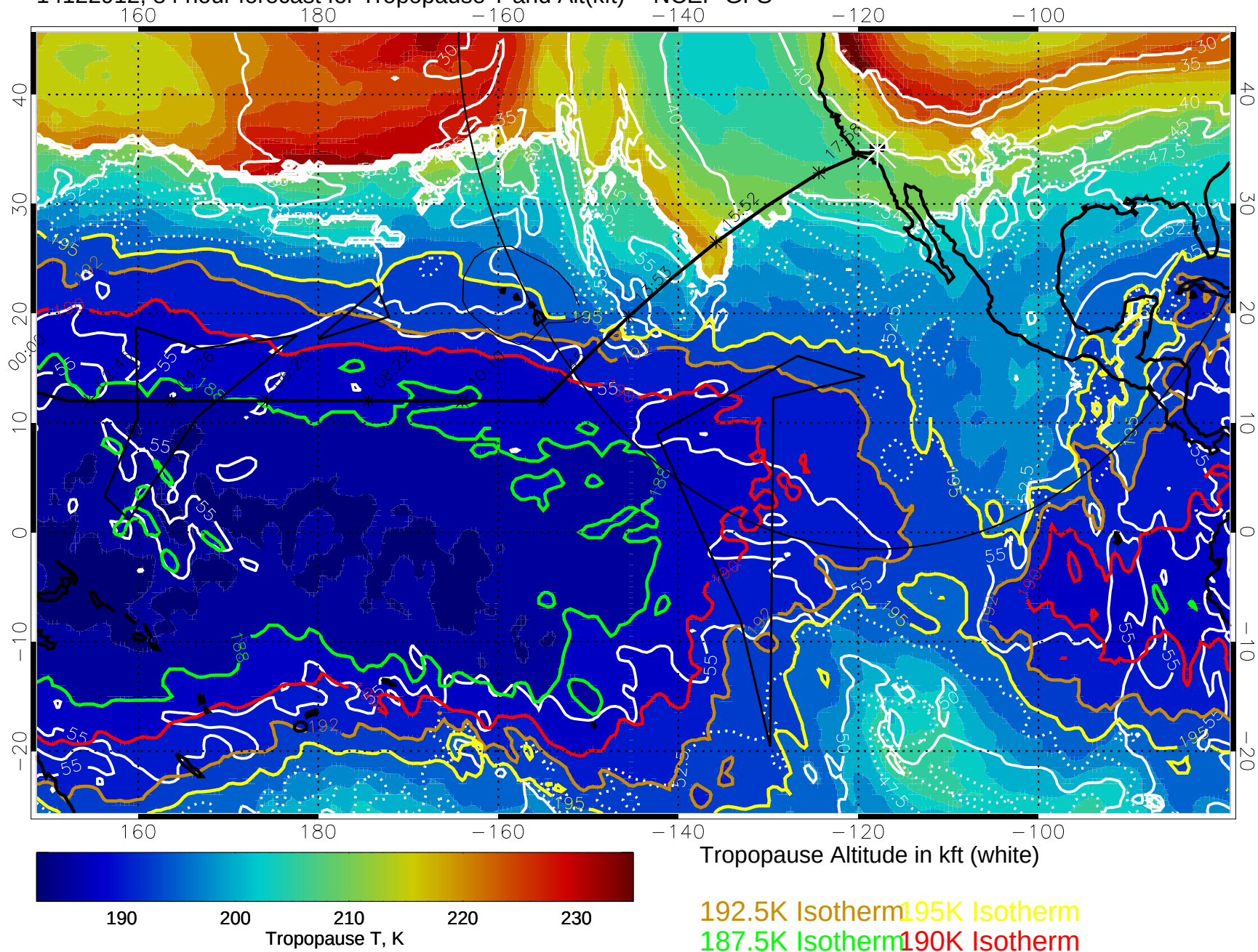
14122912, 84 hour forecast for Tropopause T and Alt(kft) -- NCEP GFS
