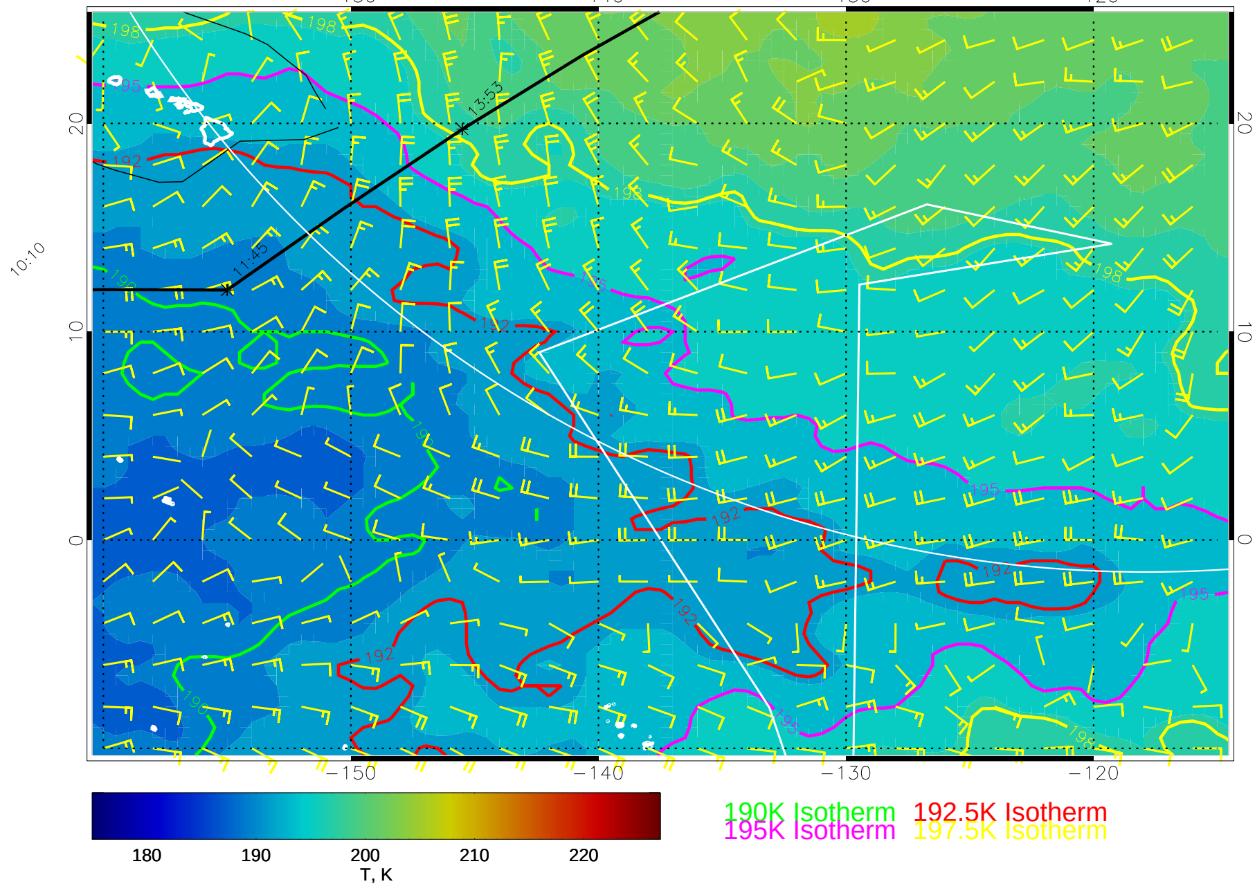
14123006, 102 hour forecast for 70mb T and winds (knots) -- NCEP GFS
