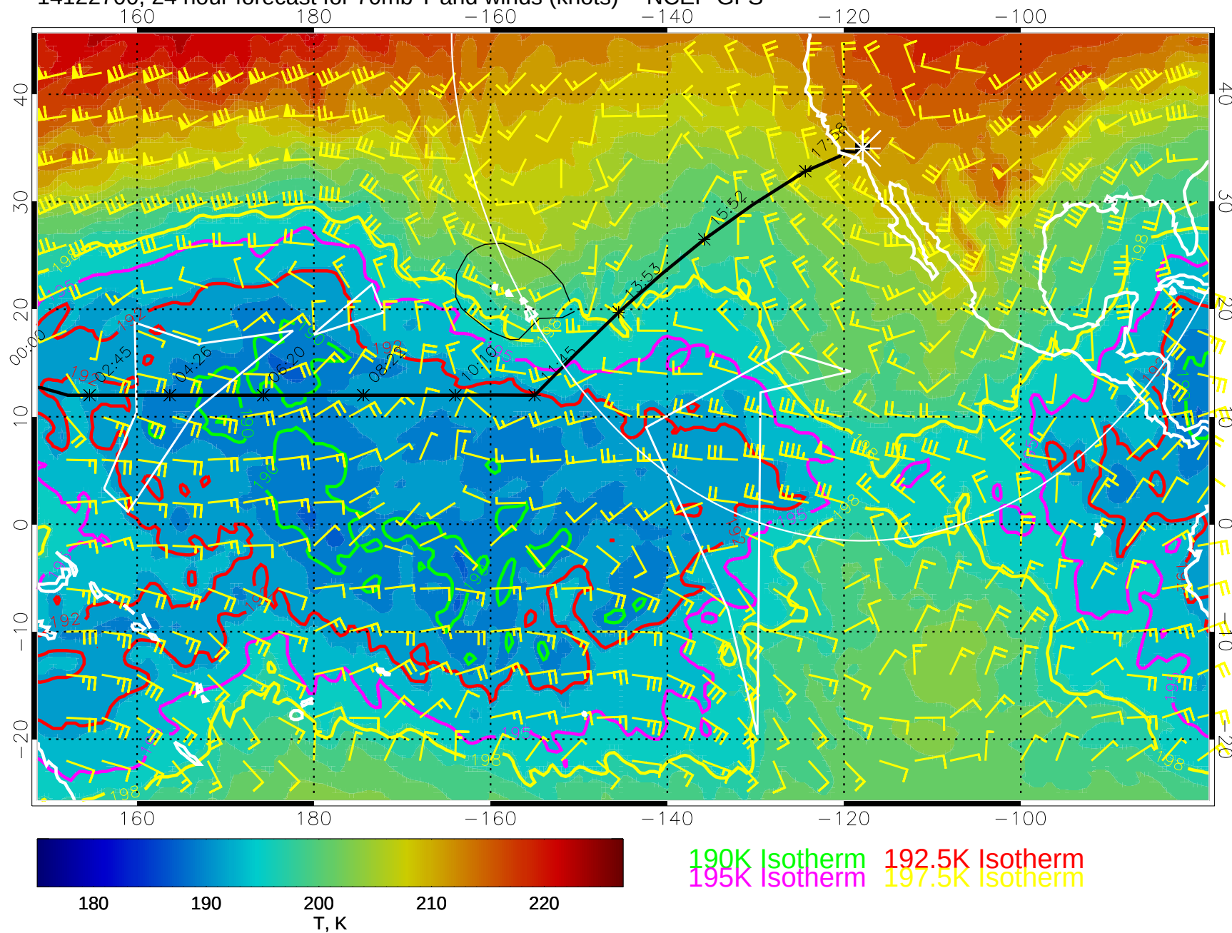
14122700, 24 hour forecast for 70mb T and winds (knots) -- NCEP GFS
