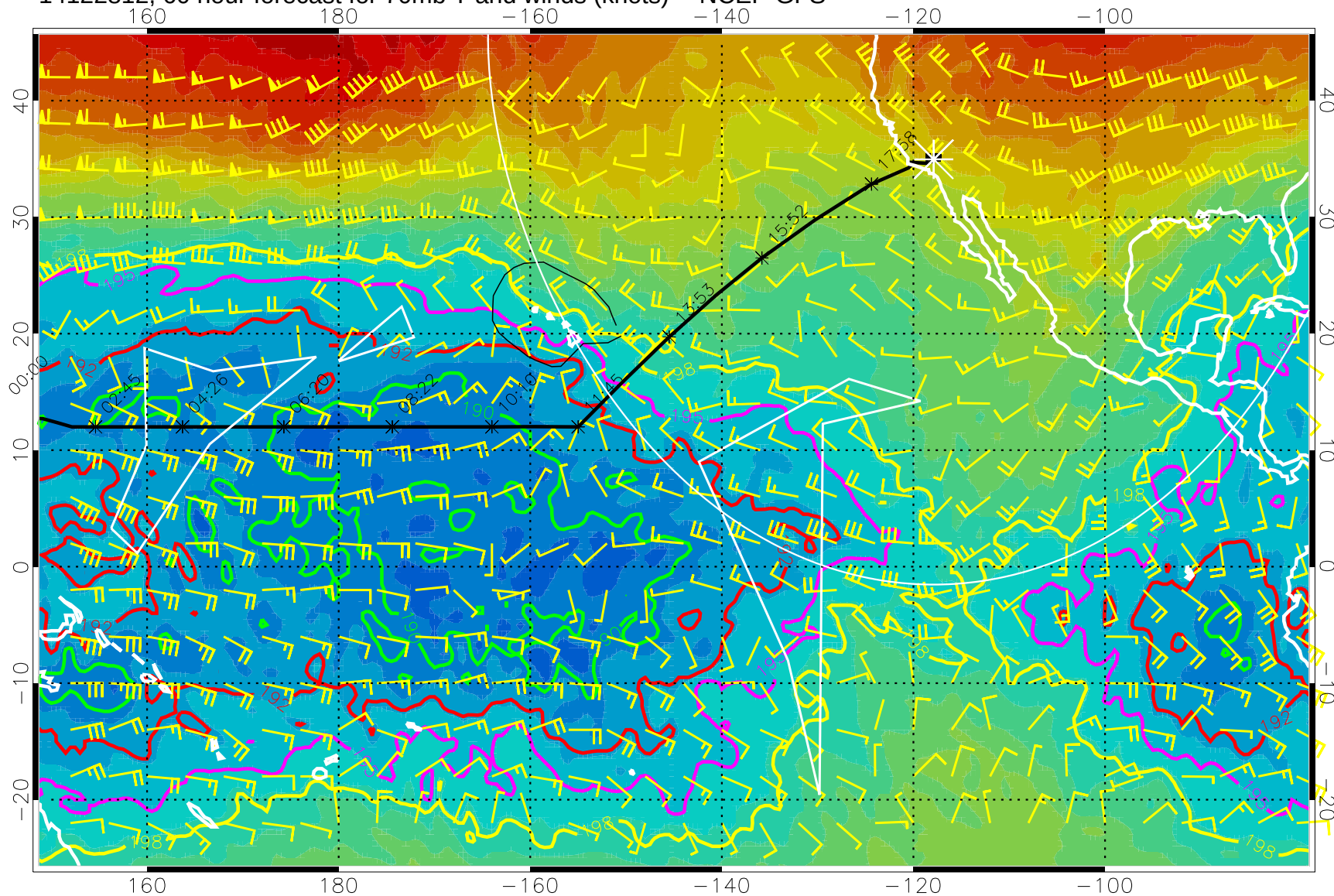
14122812, 60 hour forecast for 70mb T and winds (knots) -- NCEP GFS
