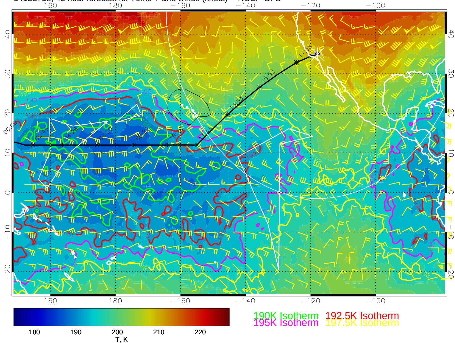
14122718, 42 hour forecast for 70mb T and winds (knots) -- NCEP GFS
