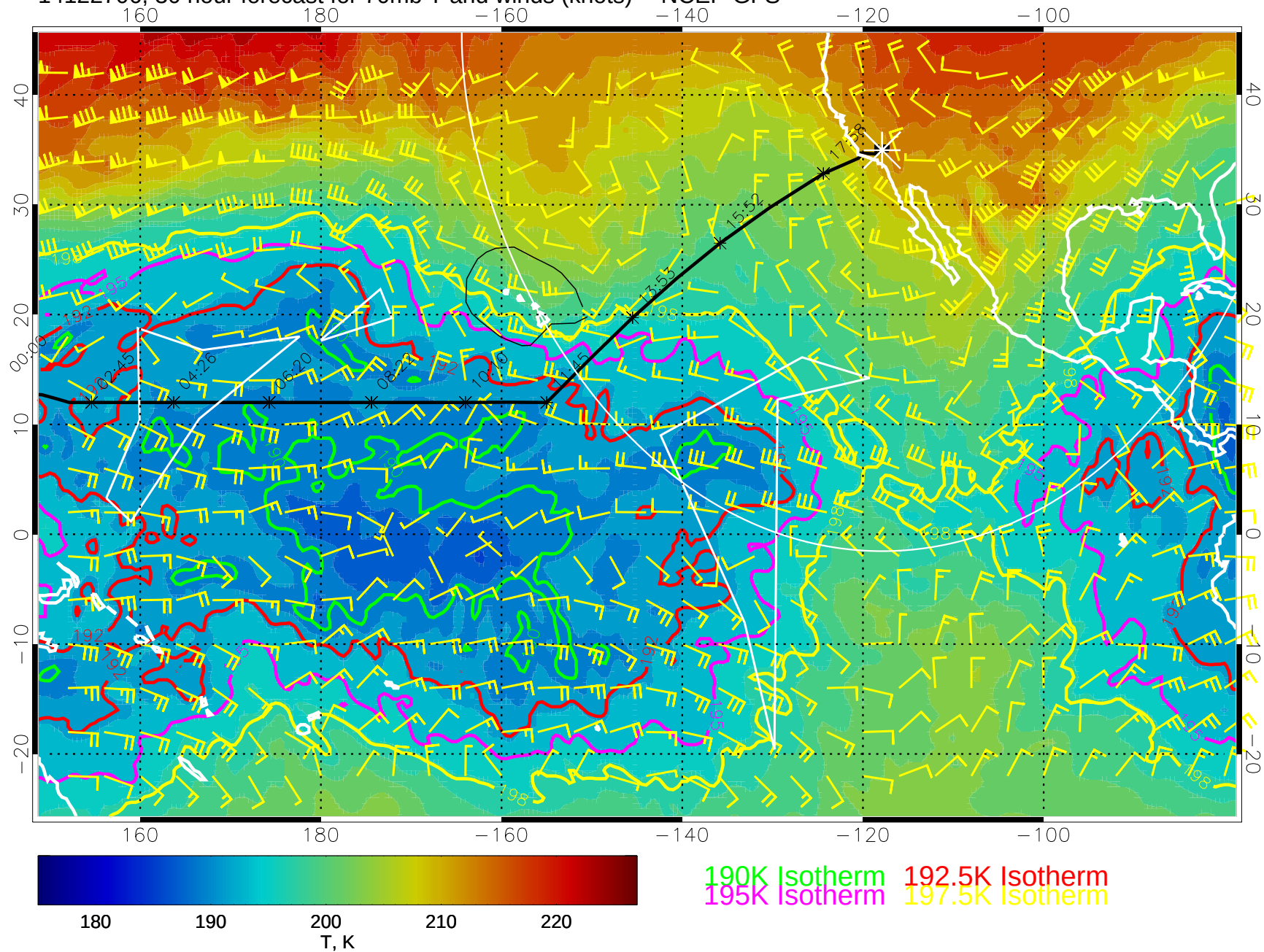
14122706, 30 hour forecast for 70mb T and winds (knots) -- NCEP GFS
