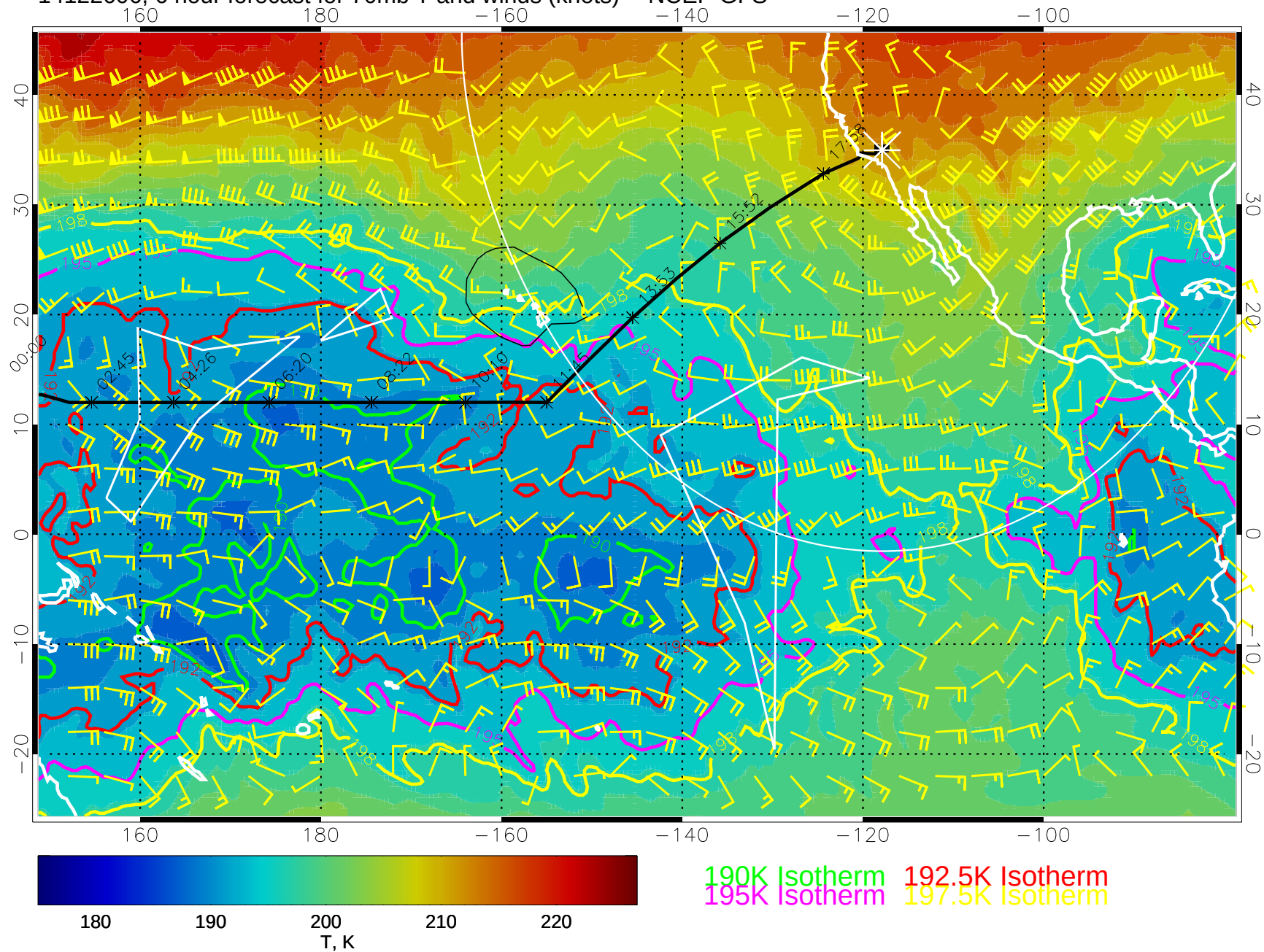
14122606, 6 hour forecast for 70mb T and winds (knots) -- NCEP GFS
