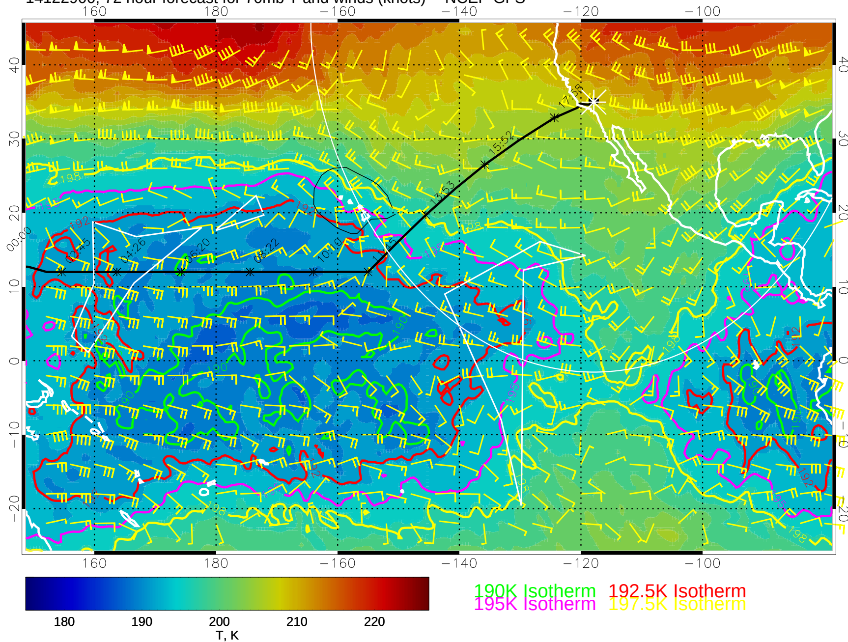
14122900, 72 hour forecast for 70mb T and winds (knots) -- NCEP GFS
