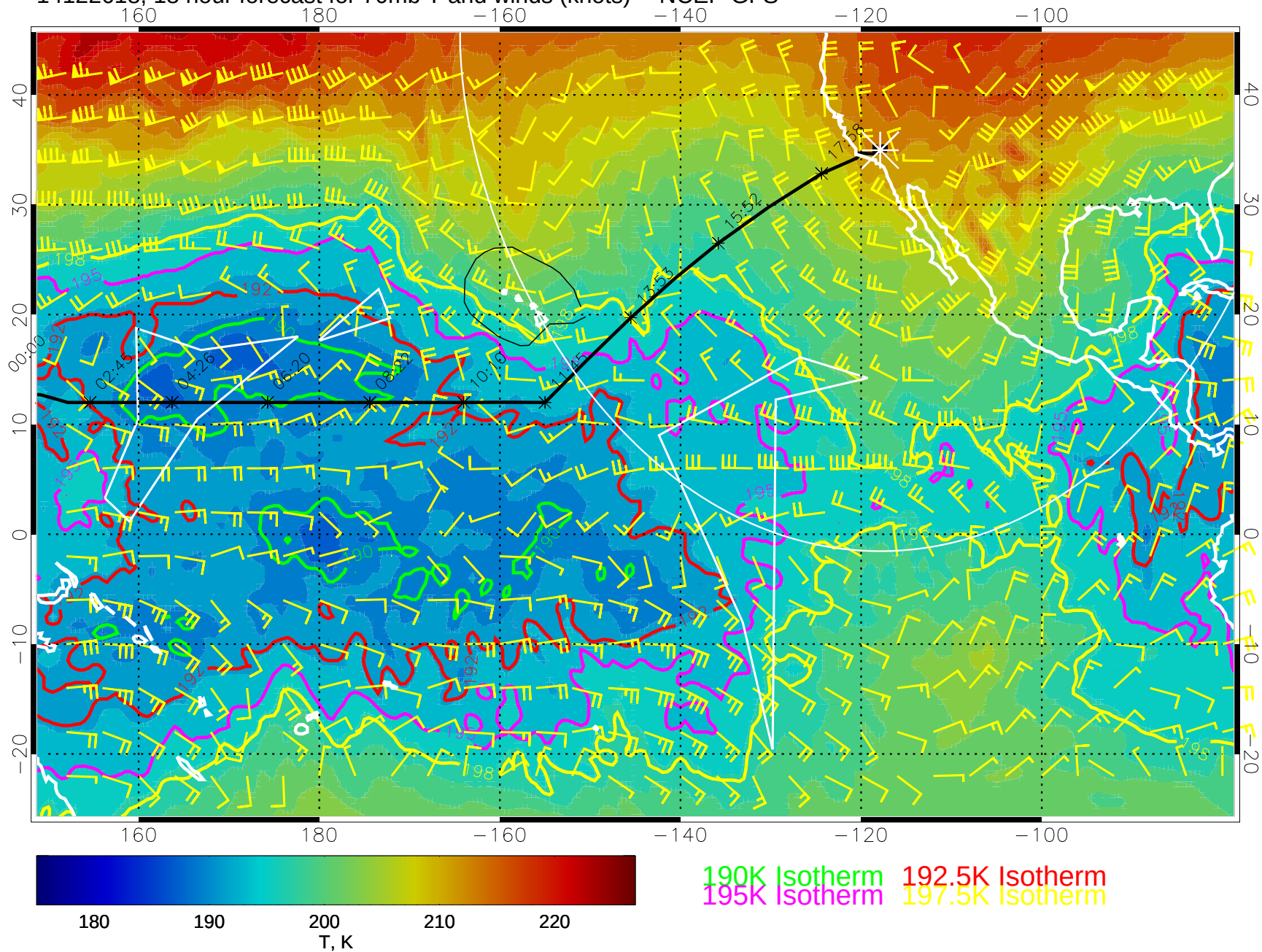
14122618, 18 hour forecast for 70mb T and winds (knots) -- NCEP GFS
