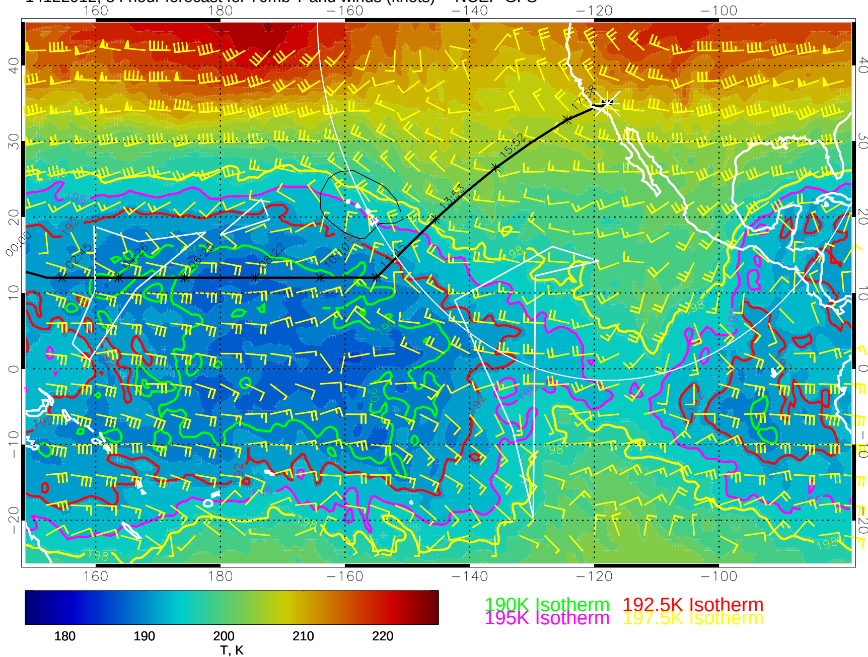
14122912, 84 hour forecast for 70mb T and winds (knots) -- NCEP GFS
