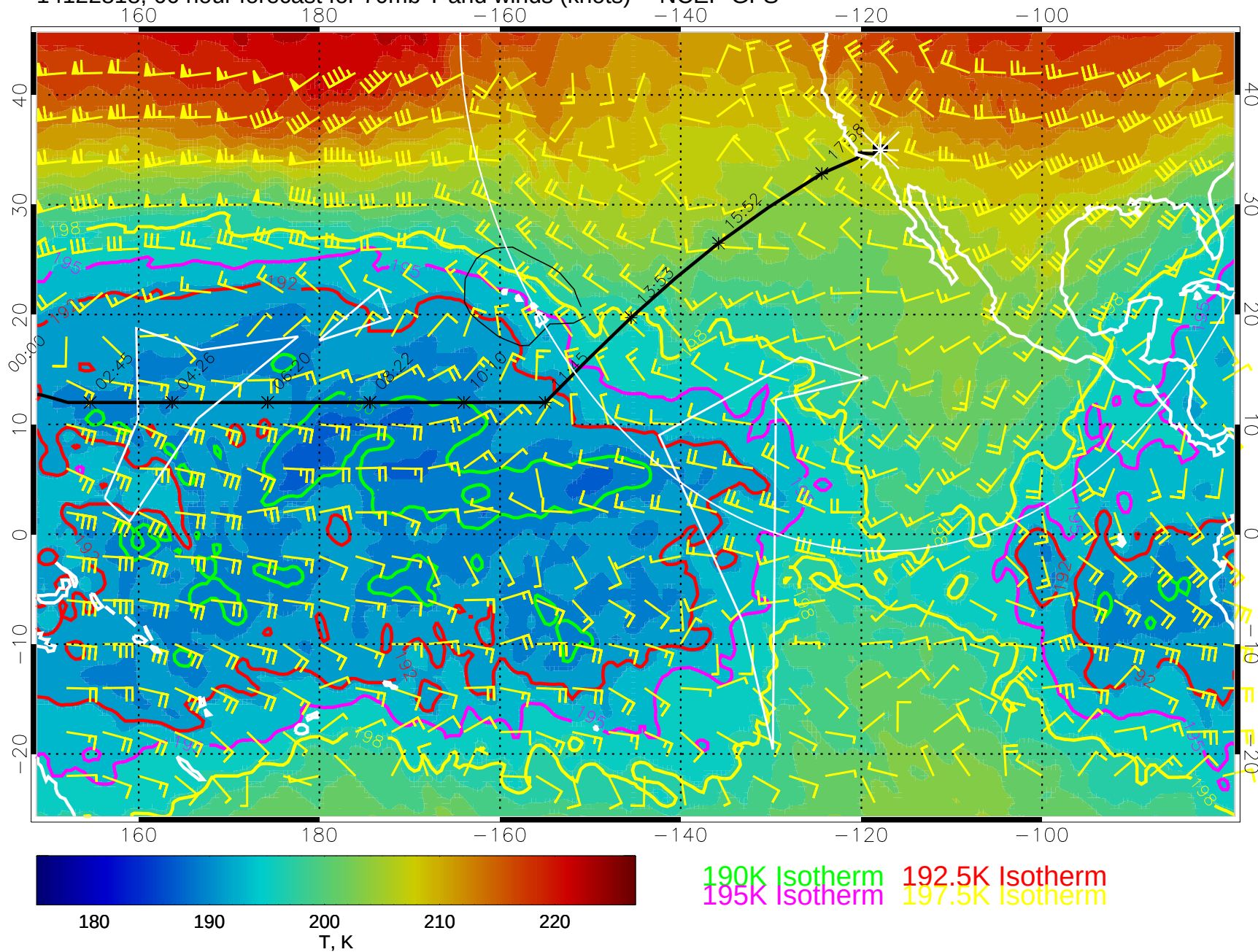
14122818, 66 hour forecast for 70mb T and winds (knots) -- NCEP GFS
