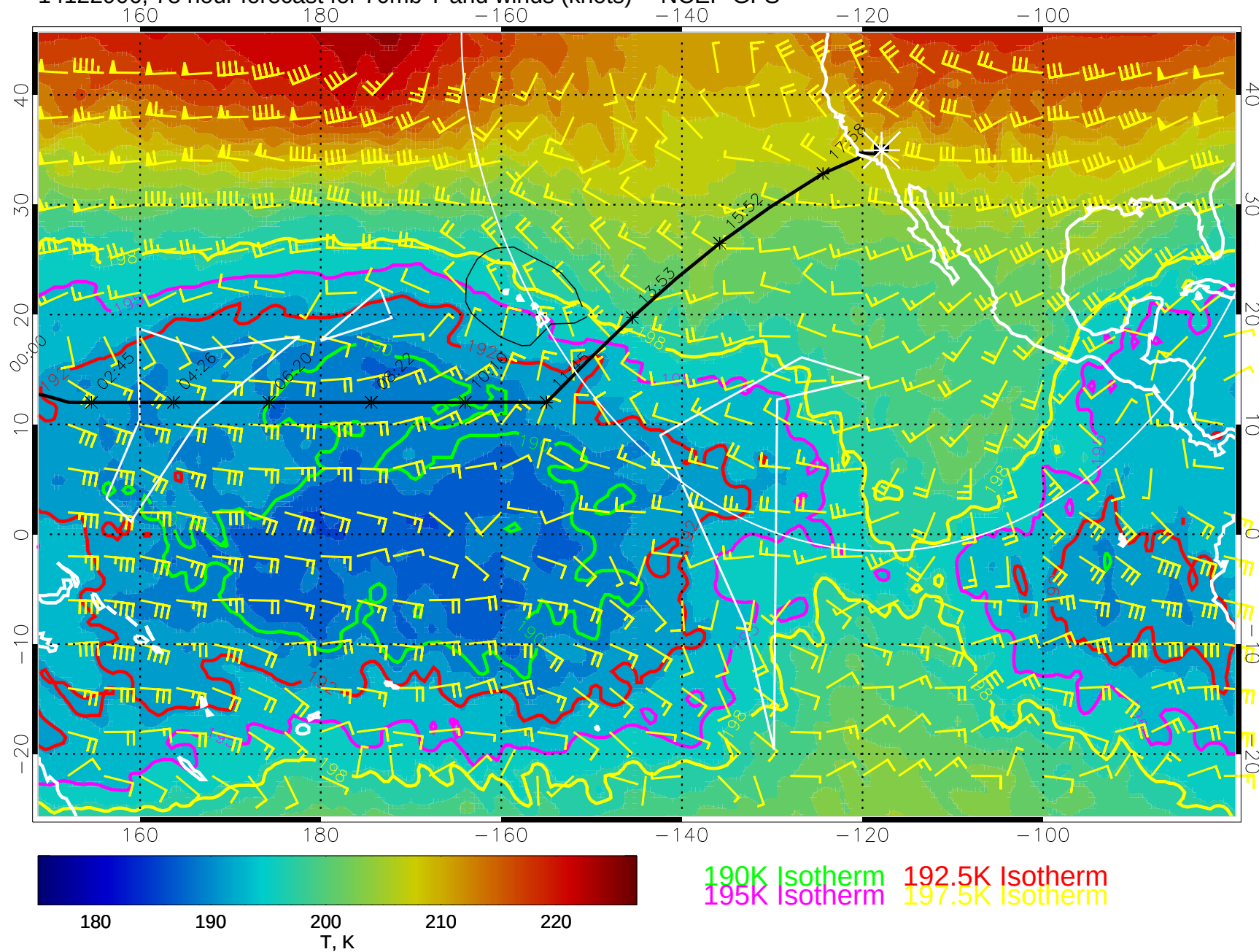
14122906, 78 hour forecast for 70mb T and winds (knots) -- NCEP GFS
