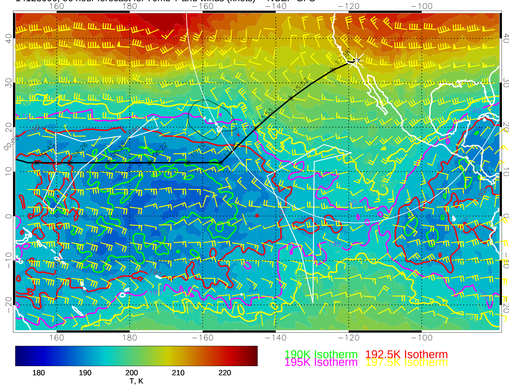
14123000, 96 hour forecast for 70mb T and winds (knots) -- NCEP GFS
