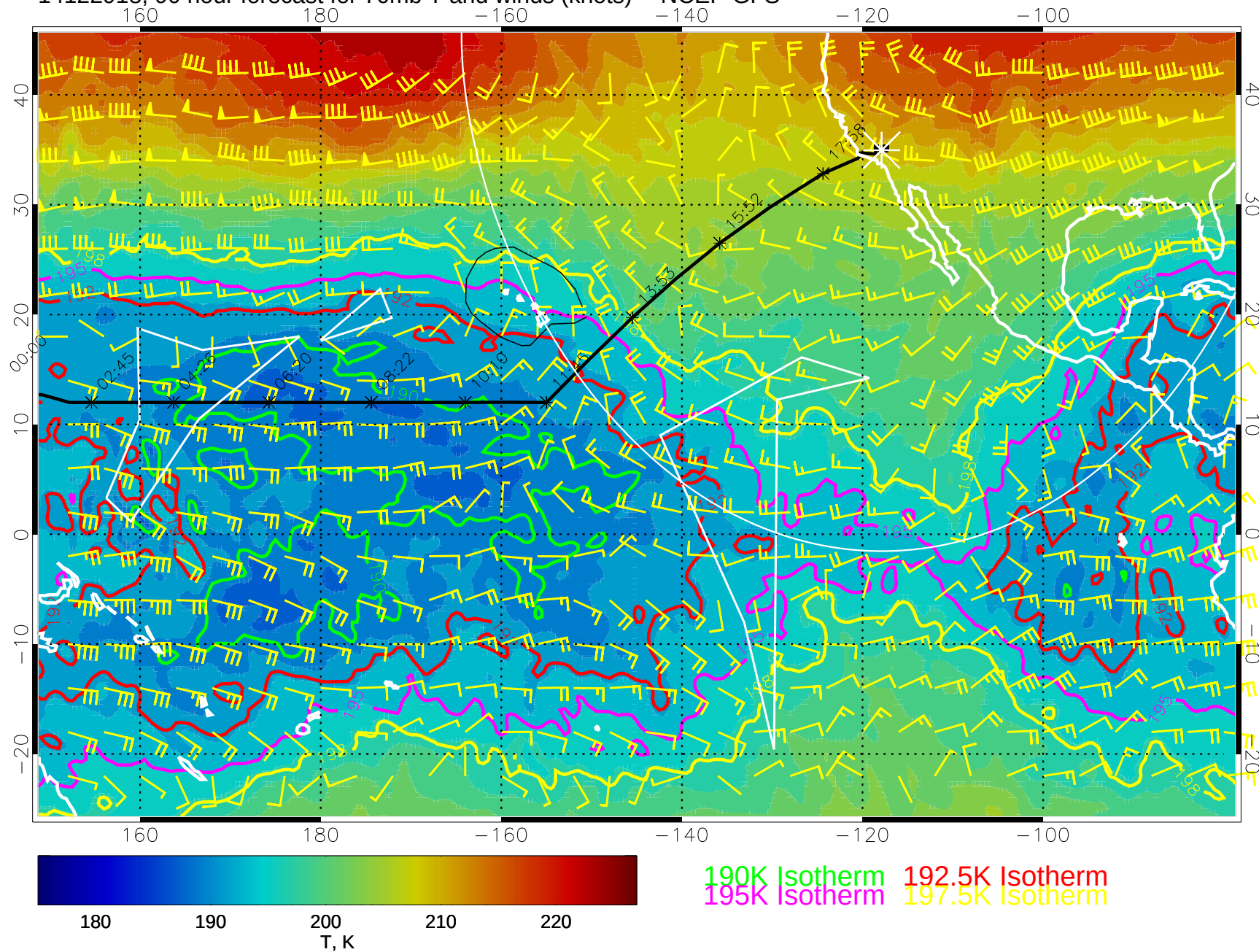
14122918, 90 hour forecast for 70mb T and winds (knots) -- NCEP GFS
