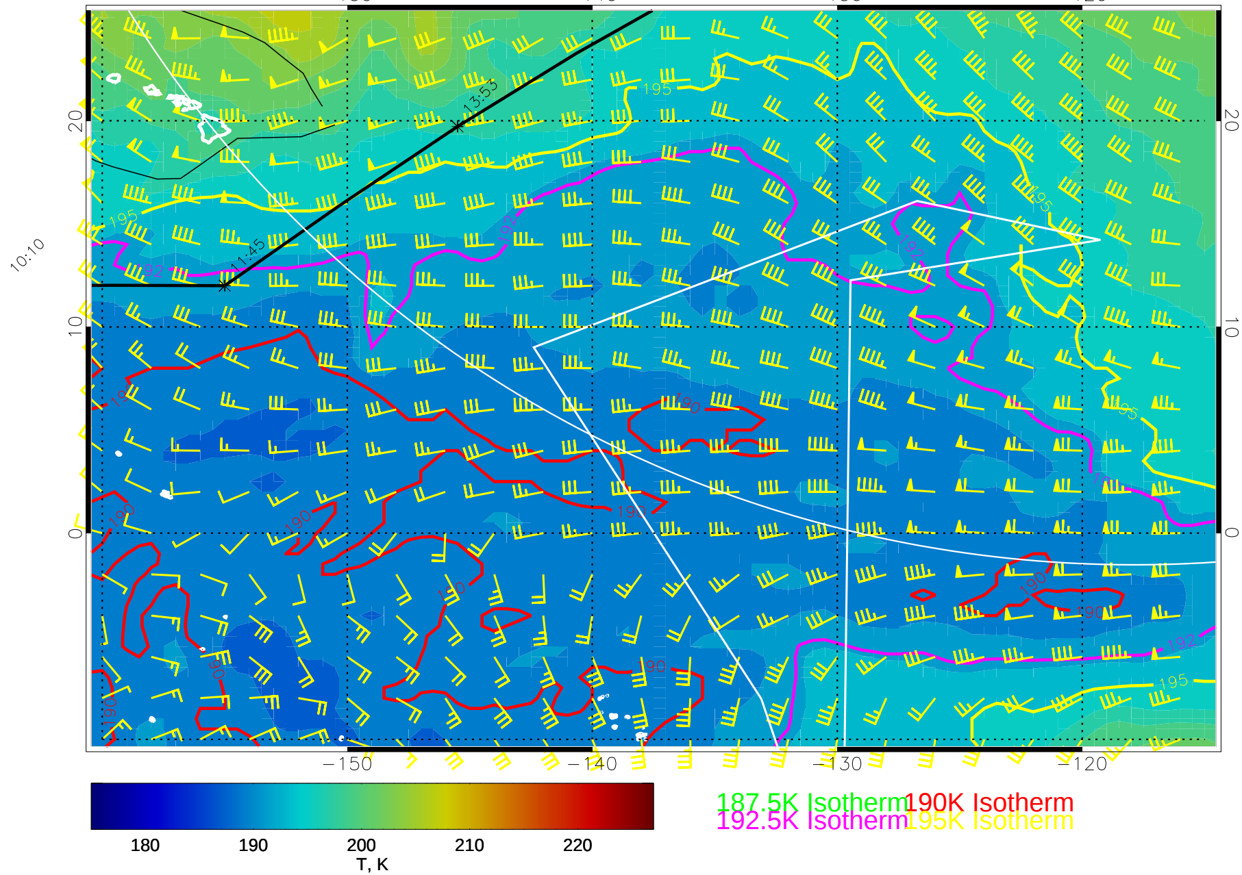
14122700, 24 hour forecast for 100mb T and winds (knots) -- NCEP GFS
