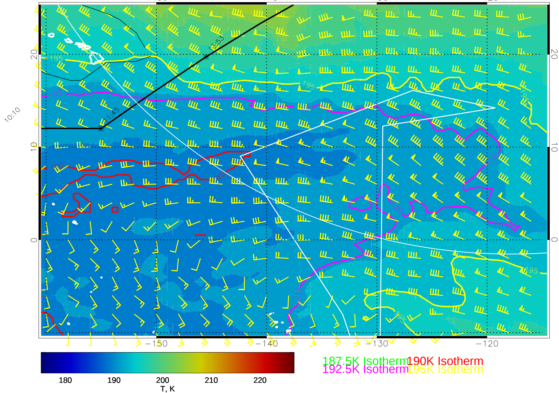
14122912, 84 hour forecast for 100mb T and winds (knots) -- NCEP GFS
