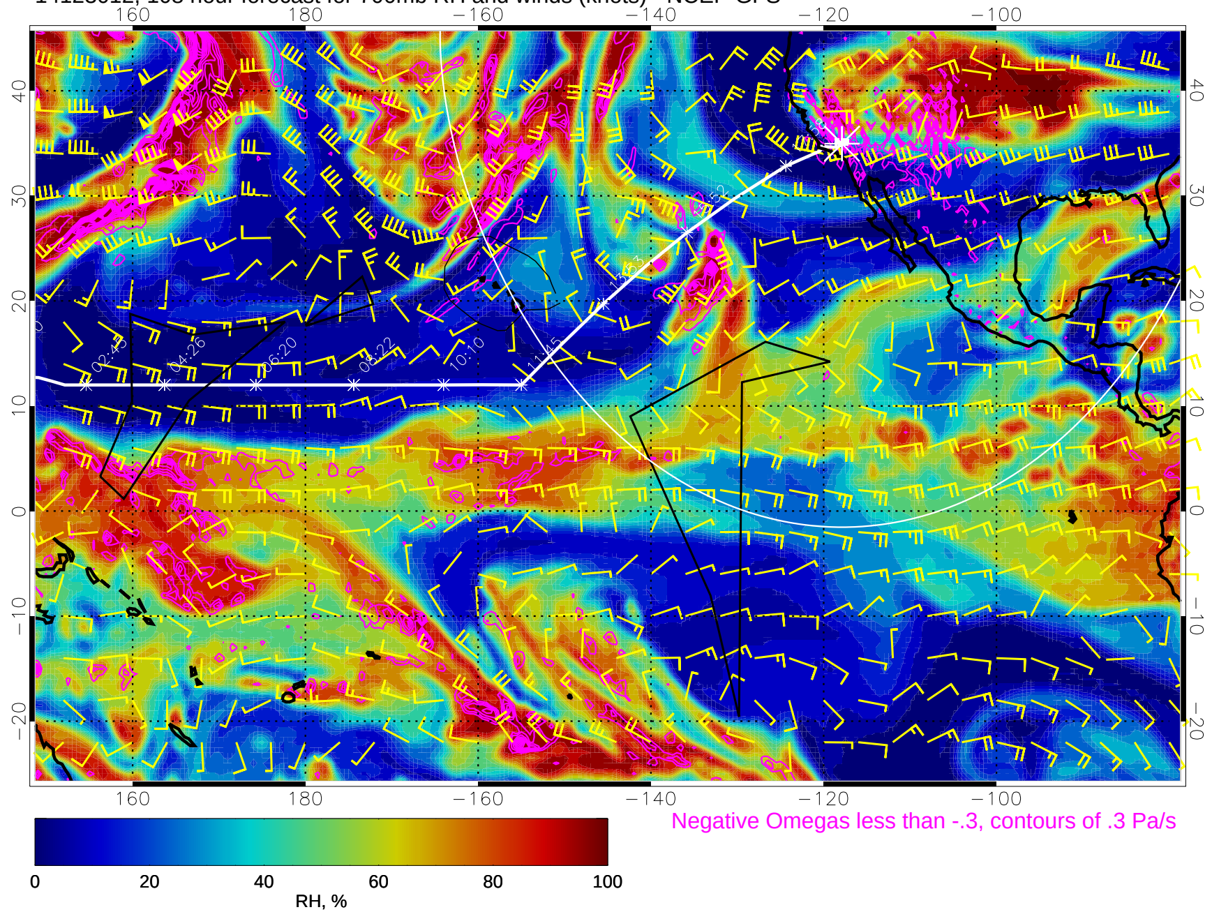
14123012, 108 hour forecast for 700mb RH and winds (knots) - NCEP GFS
