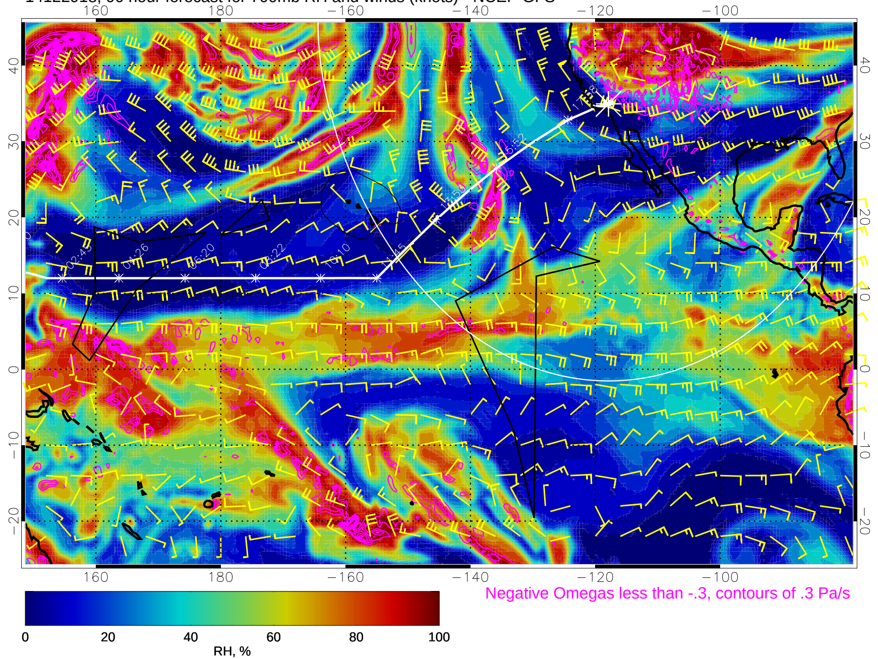
14122918, 90 hour forecast for 700mb RH and winds (knots) - NCEP GFS
