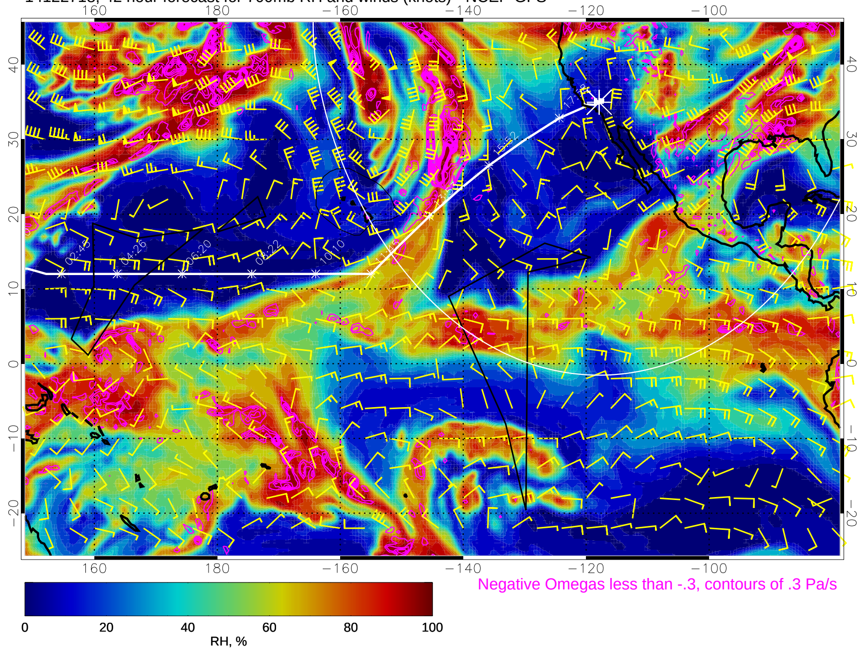
14122718, 42 hour forecast for 700mb RH and winds (knots) - NCEP GFS
