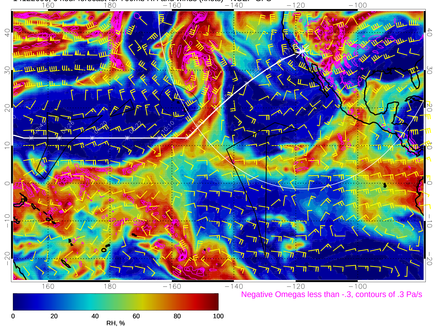
14122606, 6 hour forecast for 700mb RH and winds (knots) - NCEP GFS
