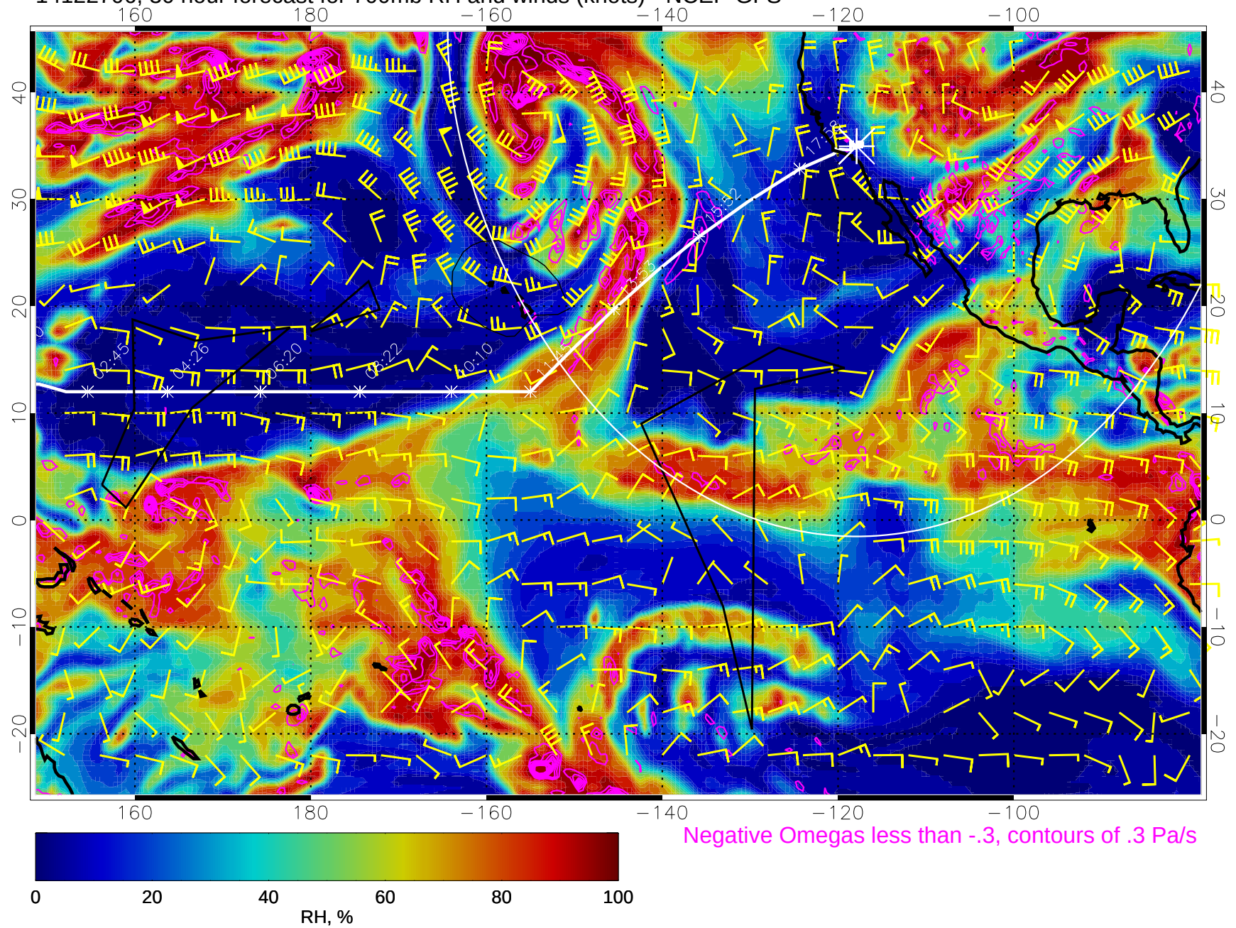
14122706, 30 hour forecast for 700mb RH and winds (knots) - NCEP GFS
