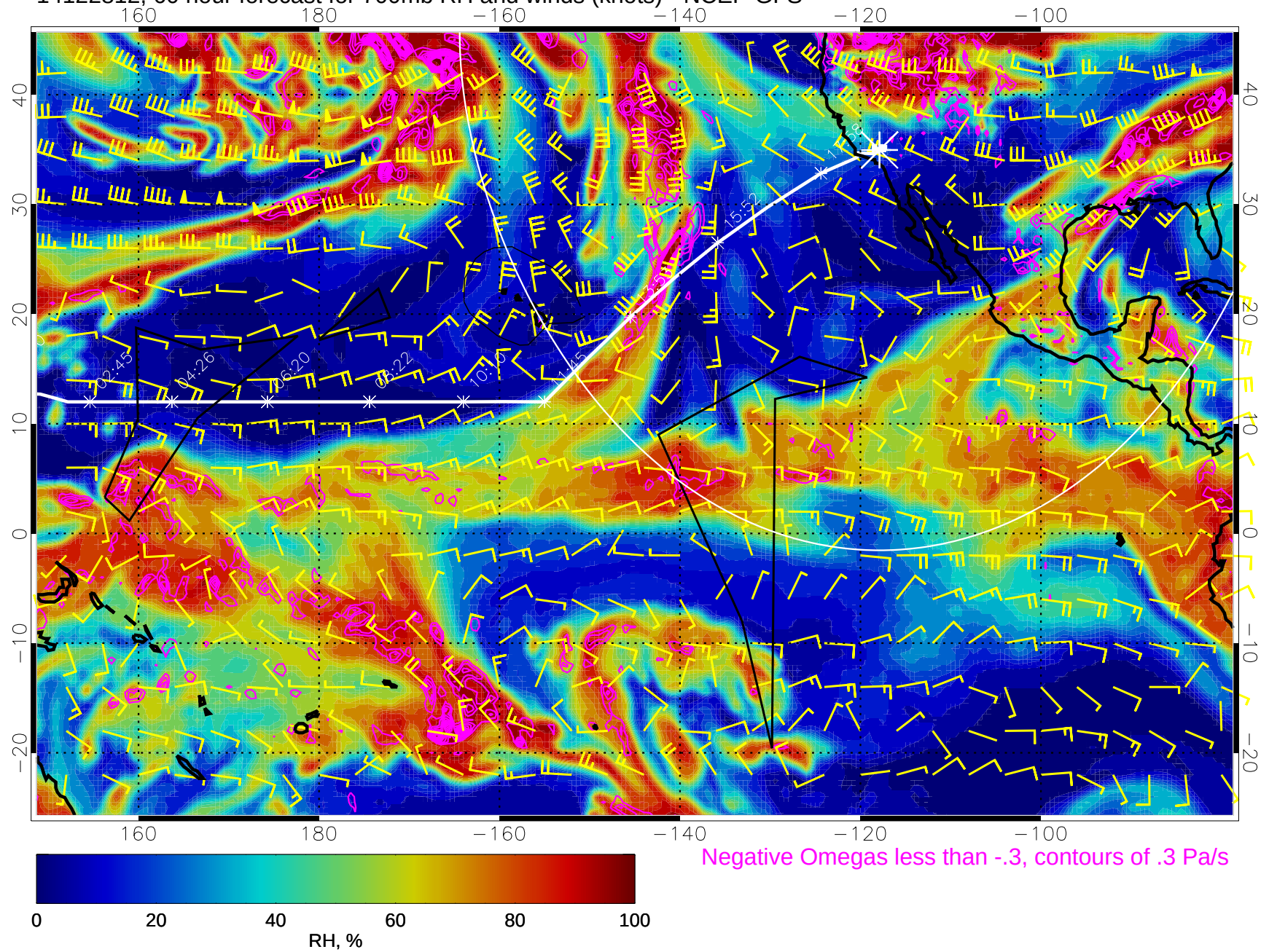
14122812, 60 hour forecast for 700mb RH and winds (knots) - NCEP GFS
