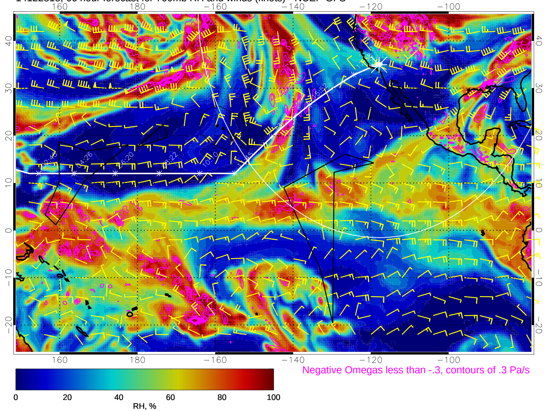
14122818, 66 hour forecast for 700mb RH and winds (knots) - NCEP GFS
