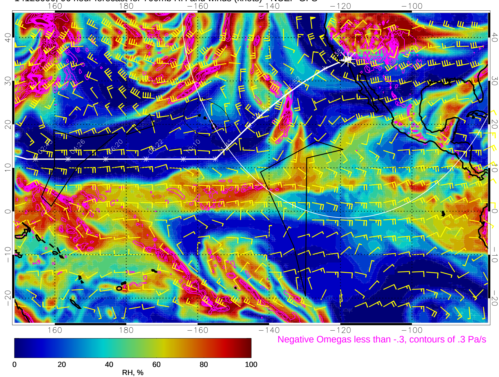
14123000, 96 hour forecast for 700mb RH and winds (knots) - NCEP GFS
