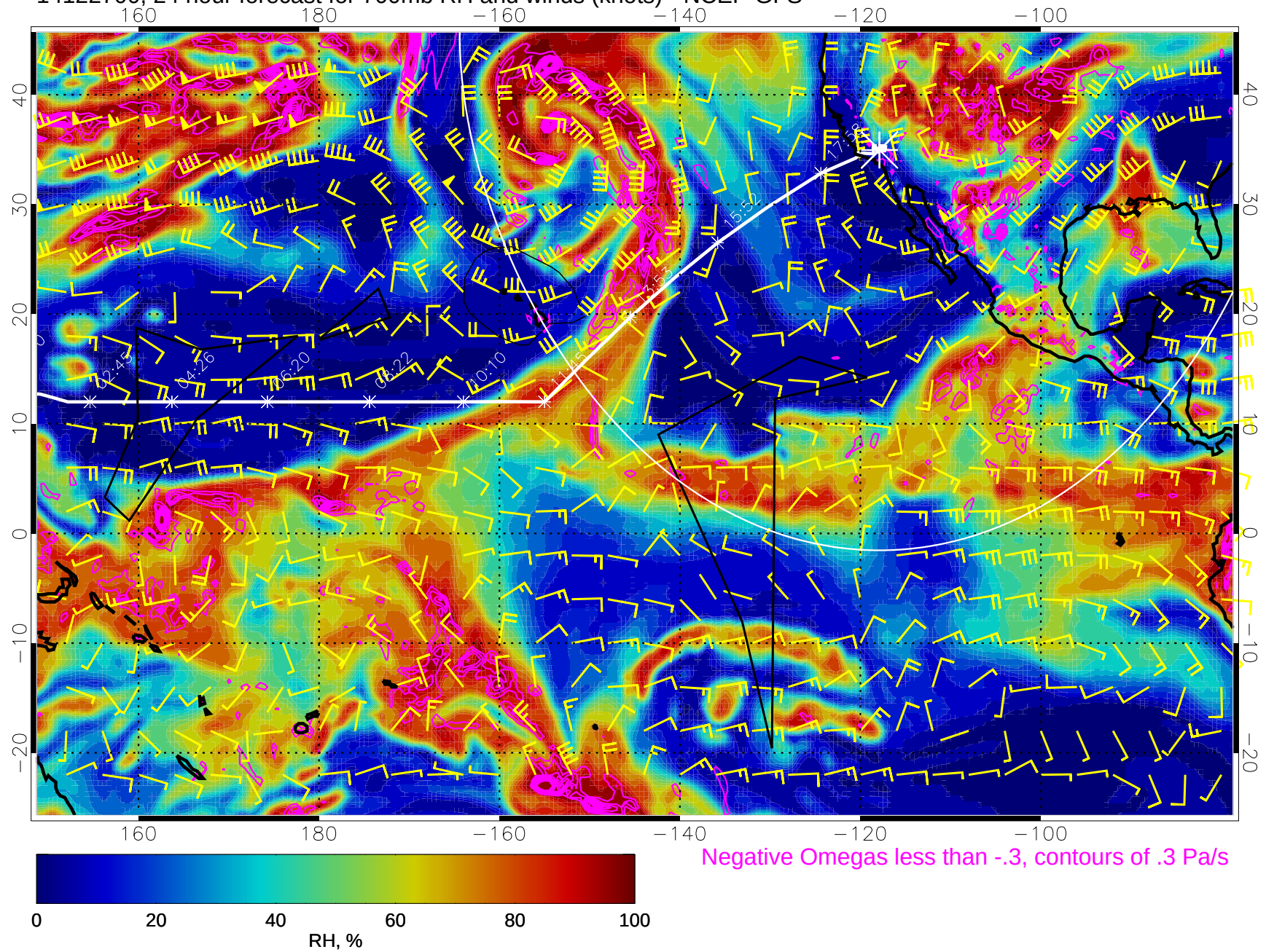
14122700, 24 hour forecast for 700mb RH and winds (knots) - NCEP GFS
