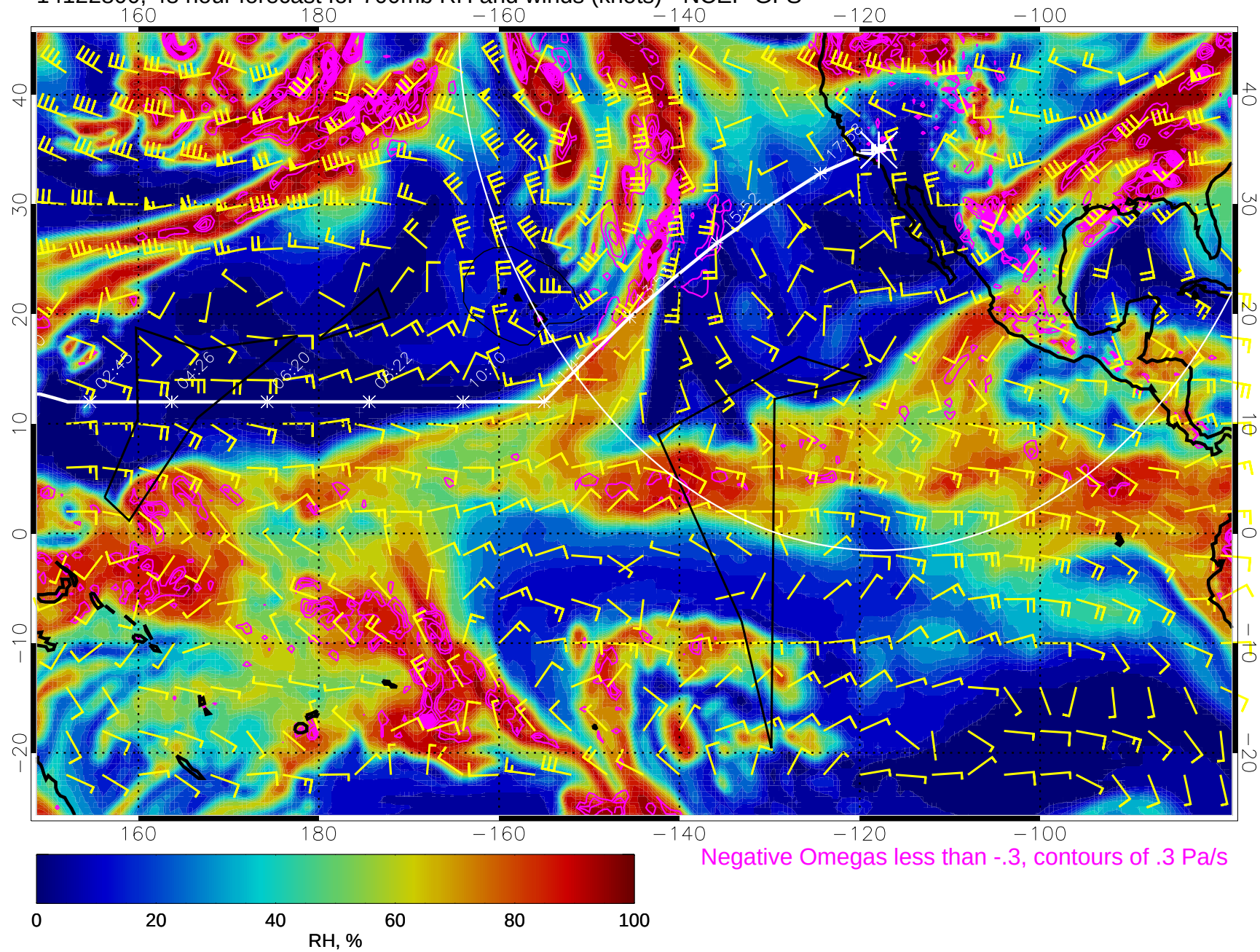
14122800, 48 hour forecast for 700mb RH and winds (knots) - NCEP GFS
