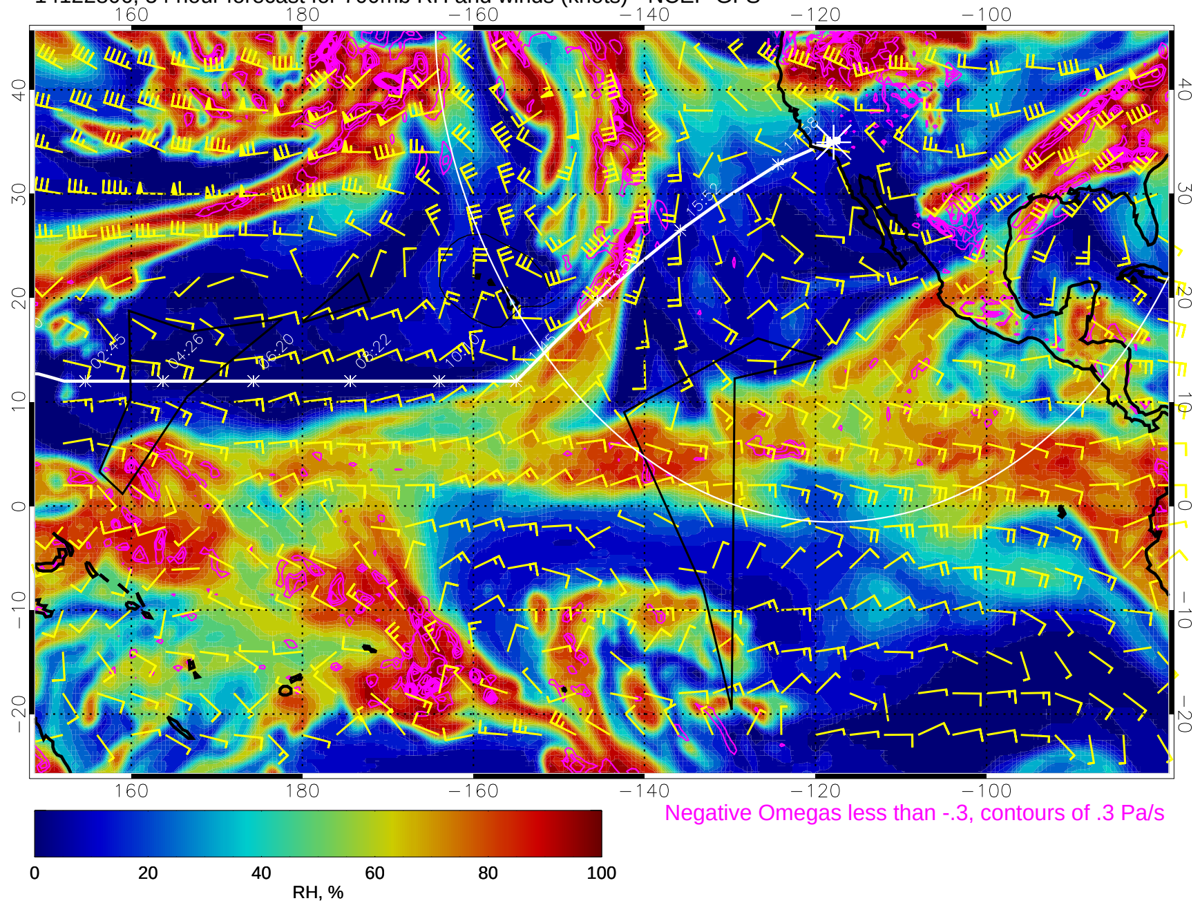
14122806, 54 hour forecast for 700mb RH and winds (knots) - NCEP GFS
