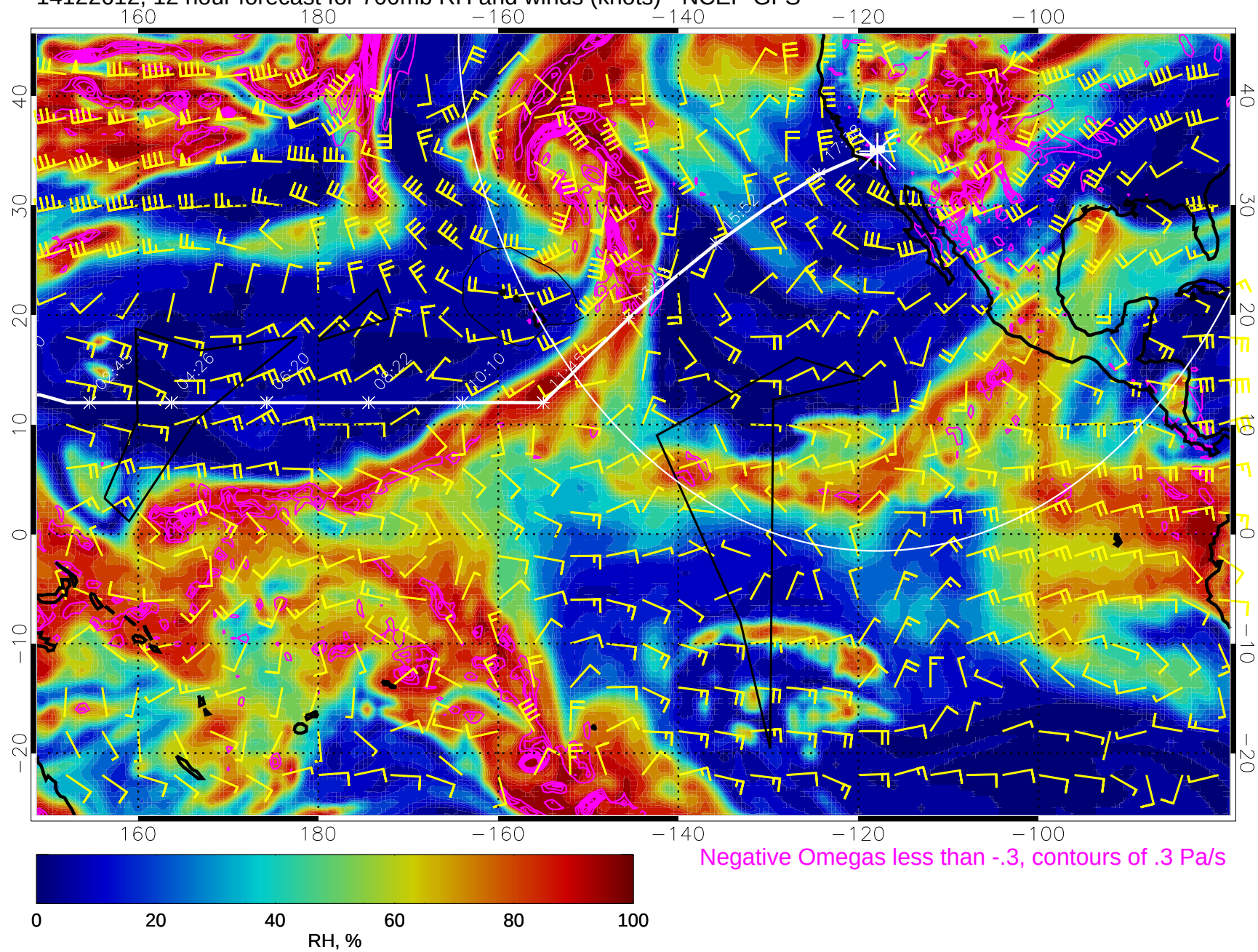
14122612, 12 hour forecast for 700mb RH and winds (knots) - NCEP GFS
