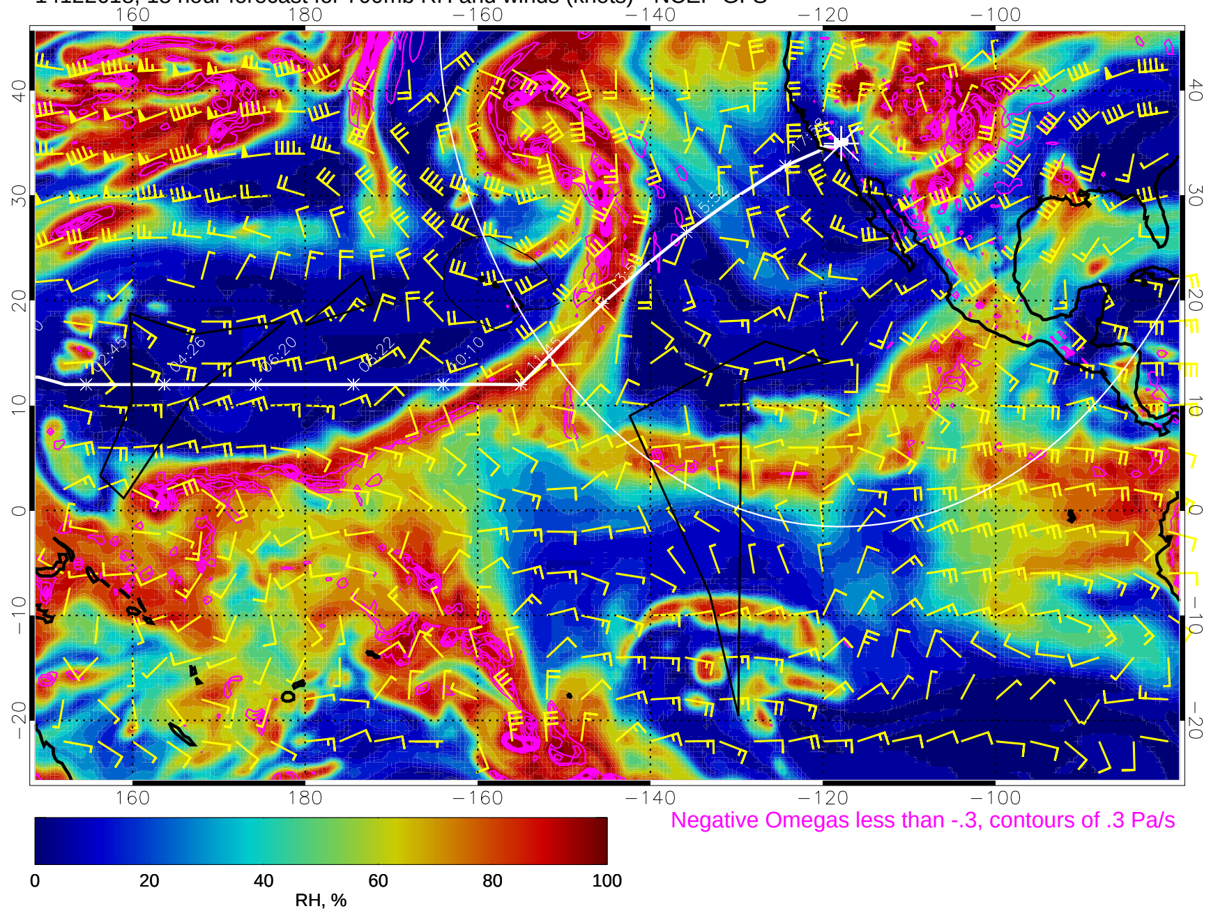
14122618, 18 hour forecast for 700mb RH and winds (knots) - NCEP GFS
