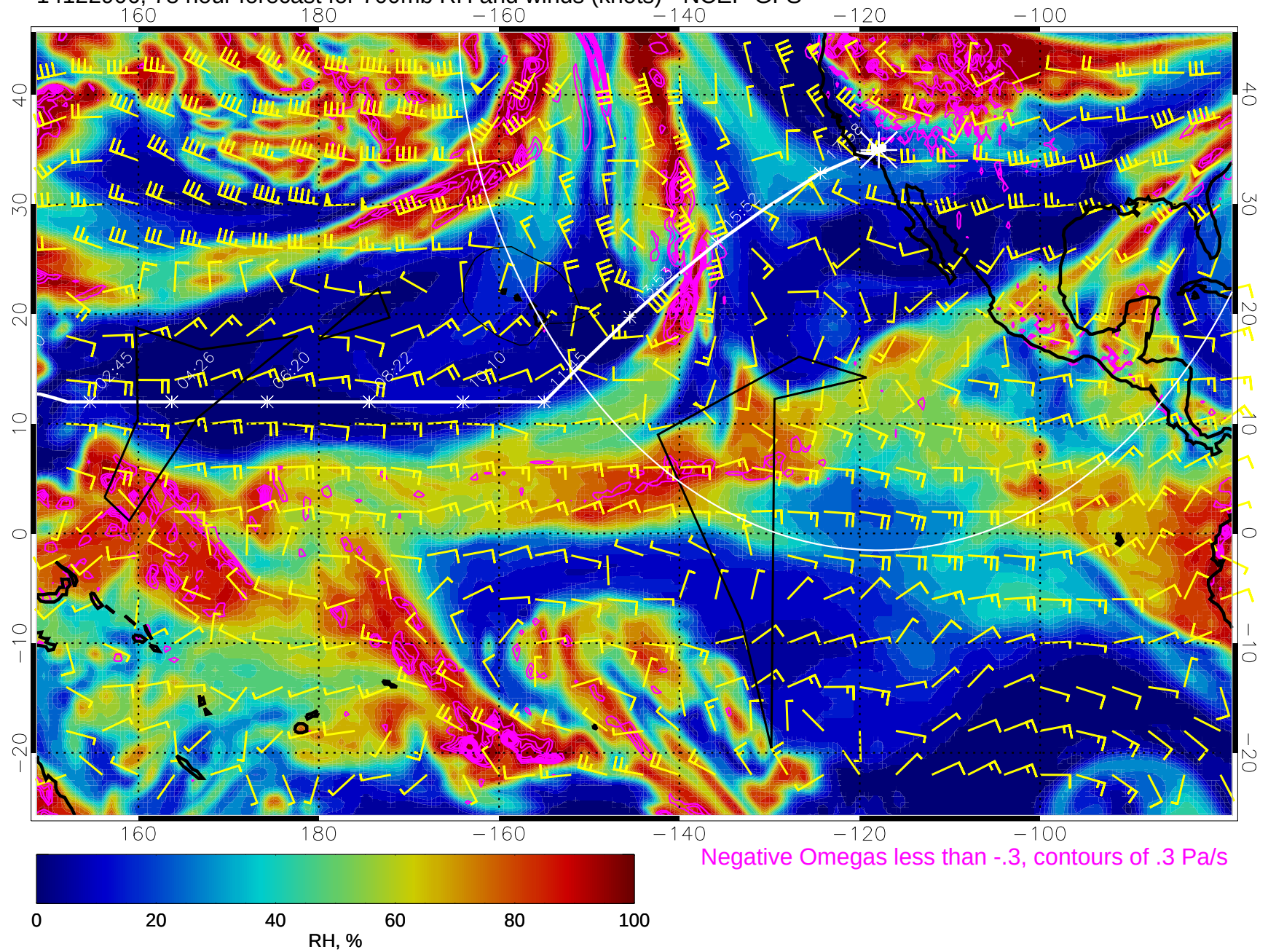
14122906, 78 hour forecast for 700mb RH and winds (knots) - NCEP GFS
