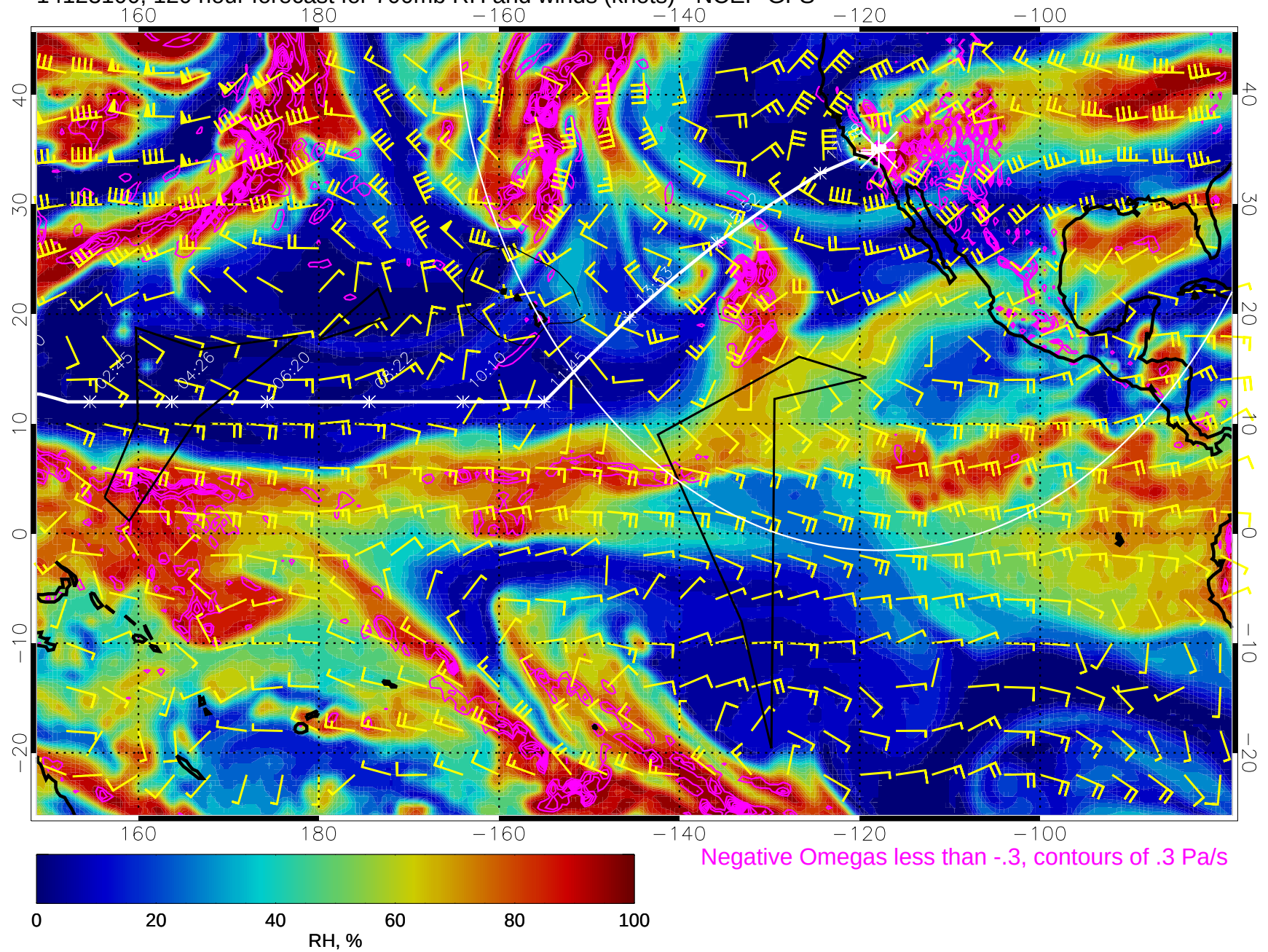
14123100, 120 hour forecast for 700mb RH and winds (knots) - NCEP GFS
