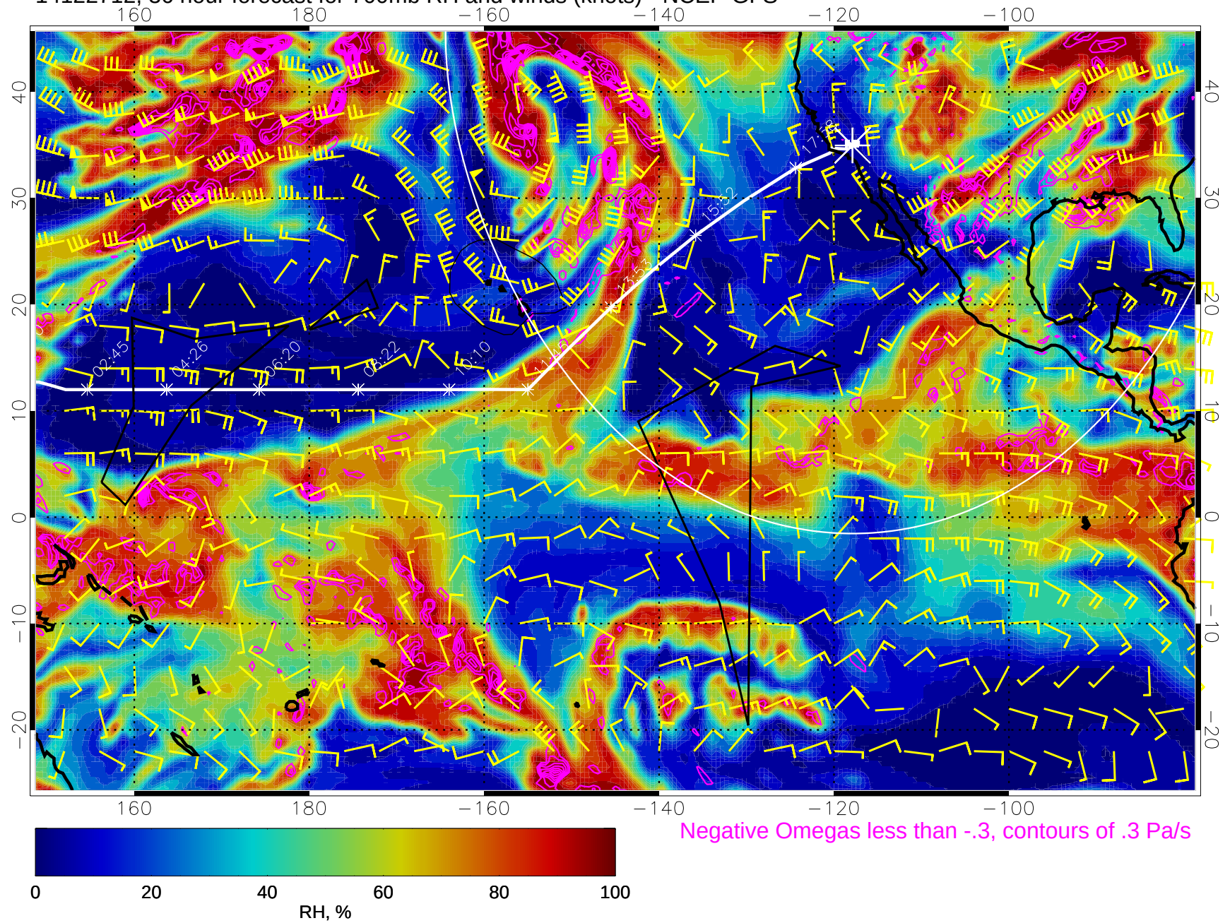
14122712, 36 hour forecast for 700mb RH and winds (knots) - NCEP GFS
