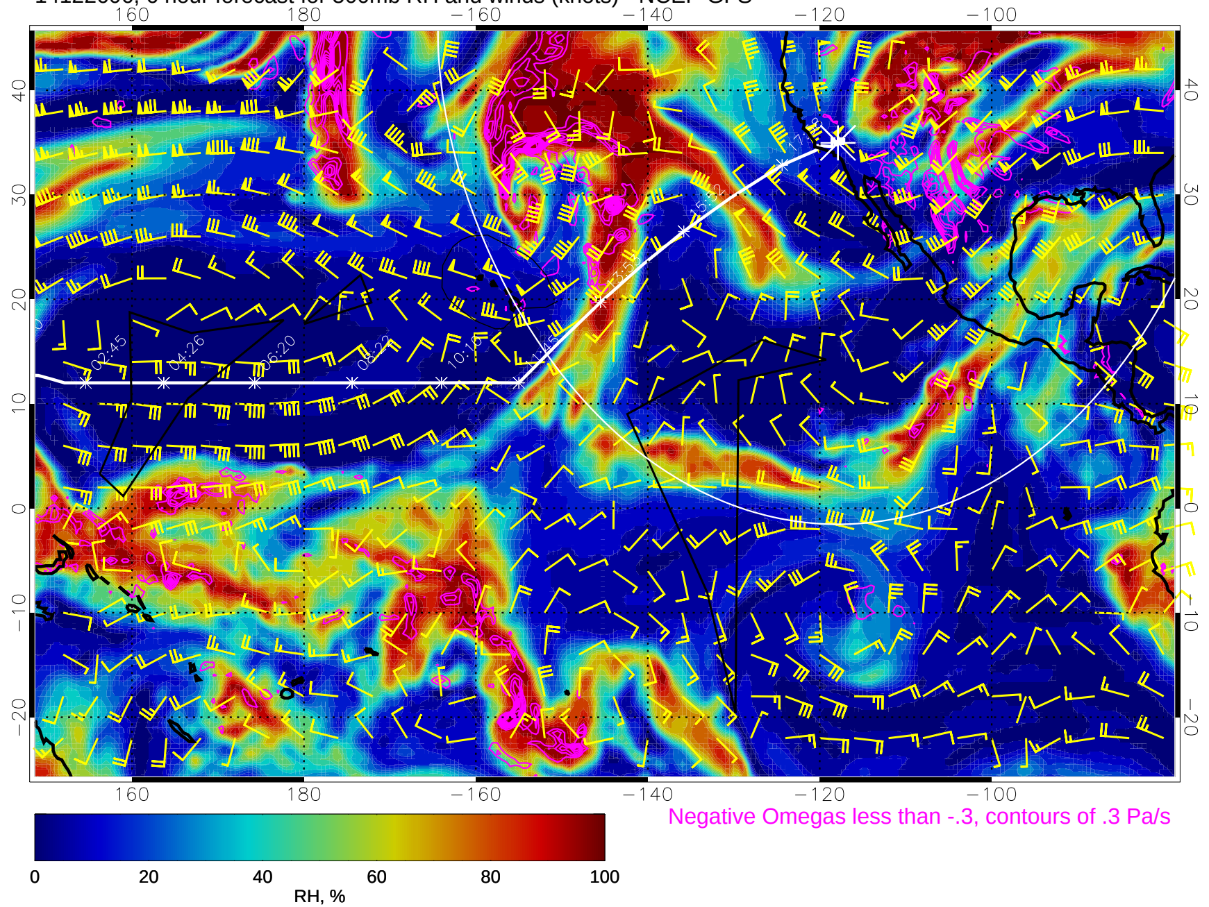
14122606, 6 hour forecast for 500mb RH and winds (knots) - NCEP GFS
