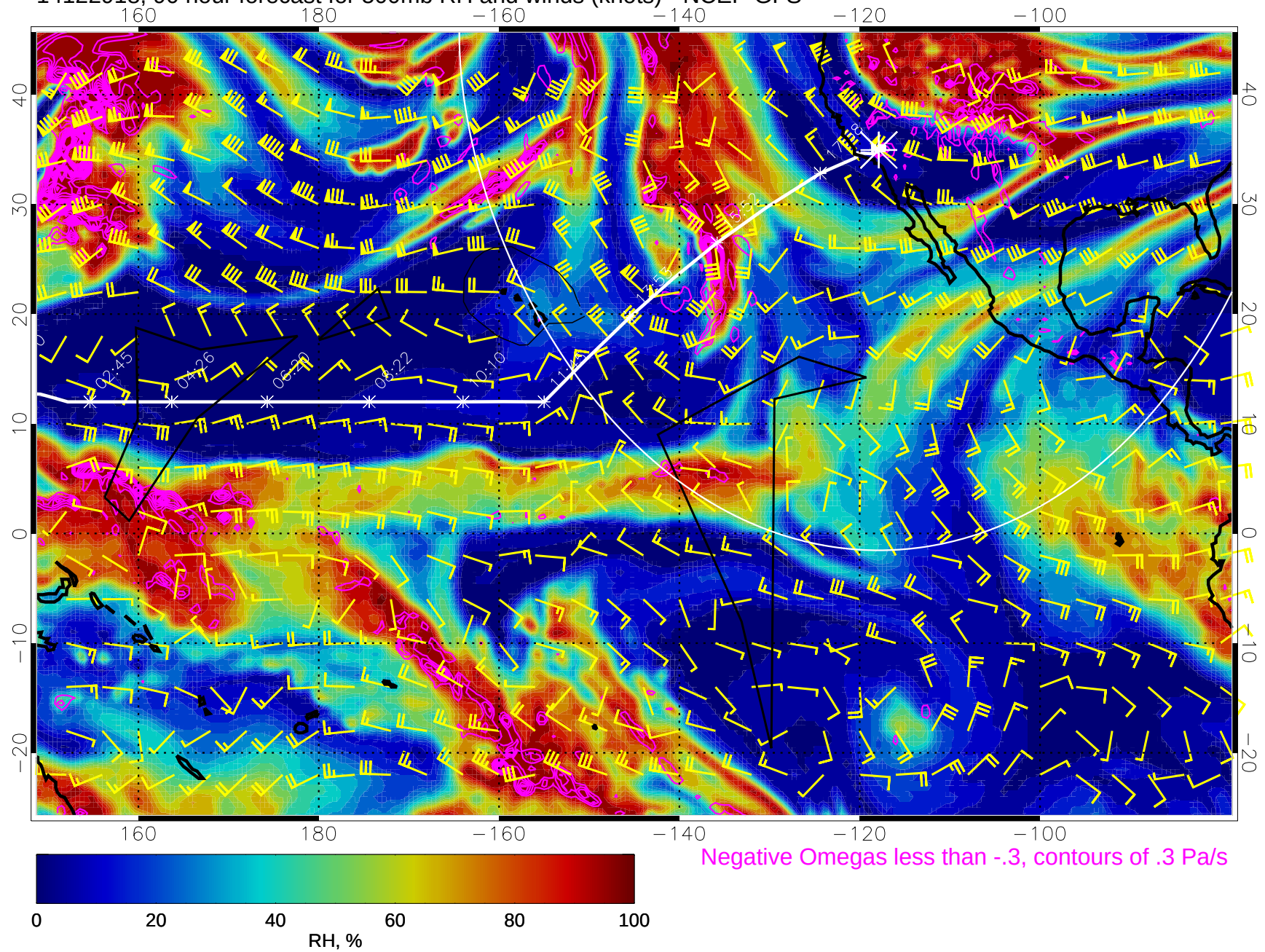
14122918, 90 hour forecast for 500mb RH and winds (knots) - NCEP GFS
