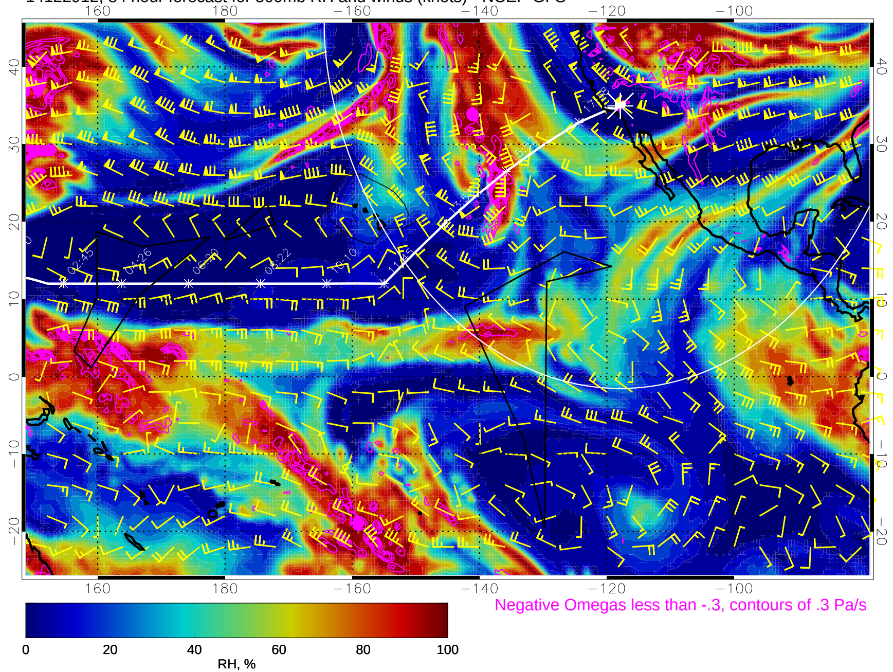
14122912, 84 hour forecast for 500mb RH and winds (knots) - NCEP GFS
