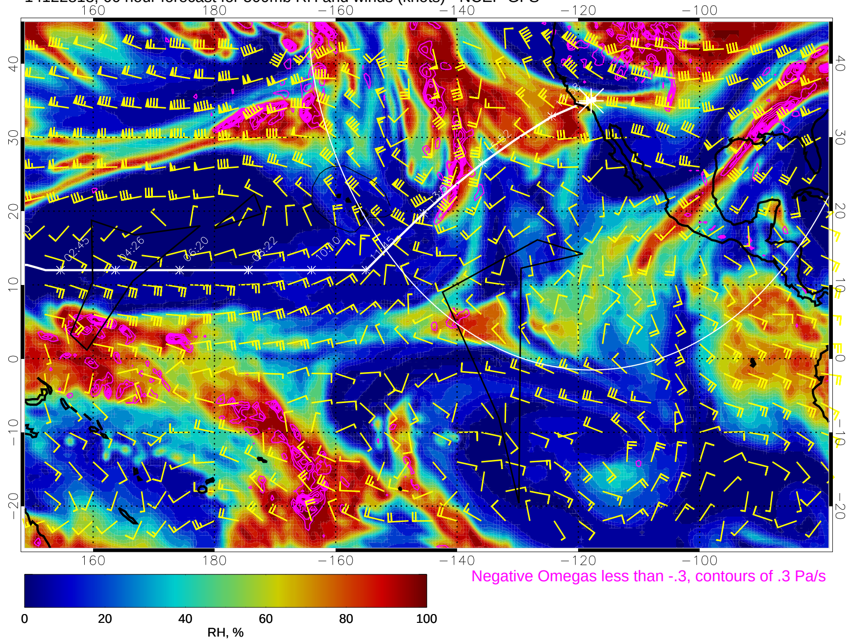
14122818, 66 hour forecast for 500mb RH and winds (knots) - NCEP GFS
