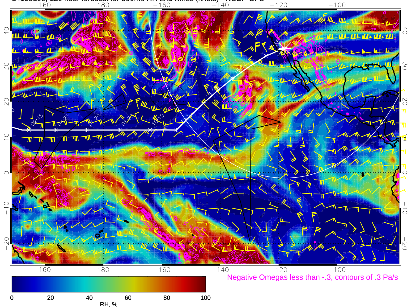
14123100, 120 hour forecast for 500mb RH and winds (knots) - NCEP GFS
