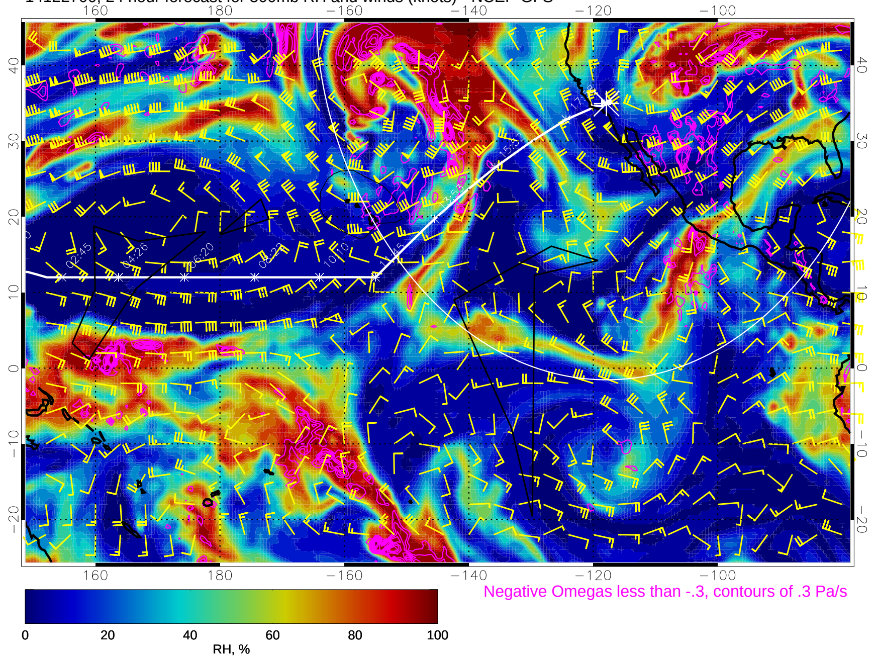
14122700, 24 hour forecast for 500mb RH and winds (knots) - NCEP GFS
