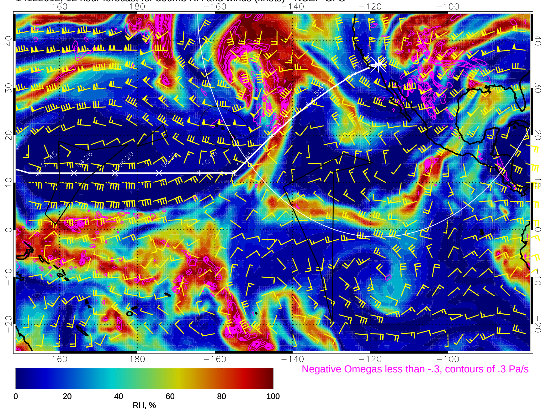
14122612, 12 hour forecast for 500mb RH and winds (knots) - NCEP GFS
