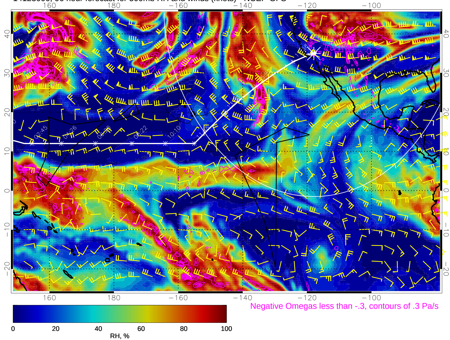
14123000, 96 hour forecast for 500mb RH and winds (knots) - NCEP GFS
