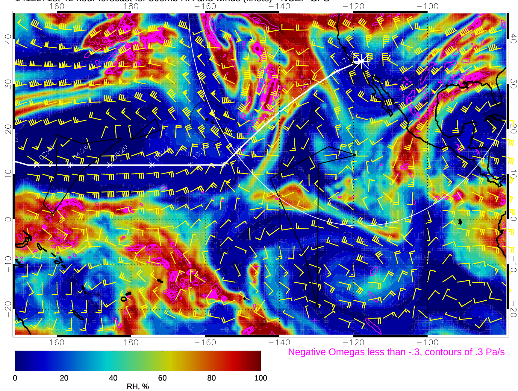
14122718, 42 hour forecast for 500mb RH and winds (knots) - NCEP GFS
