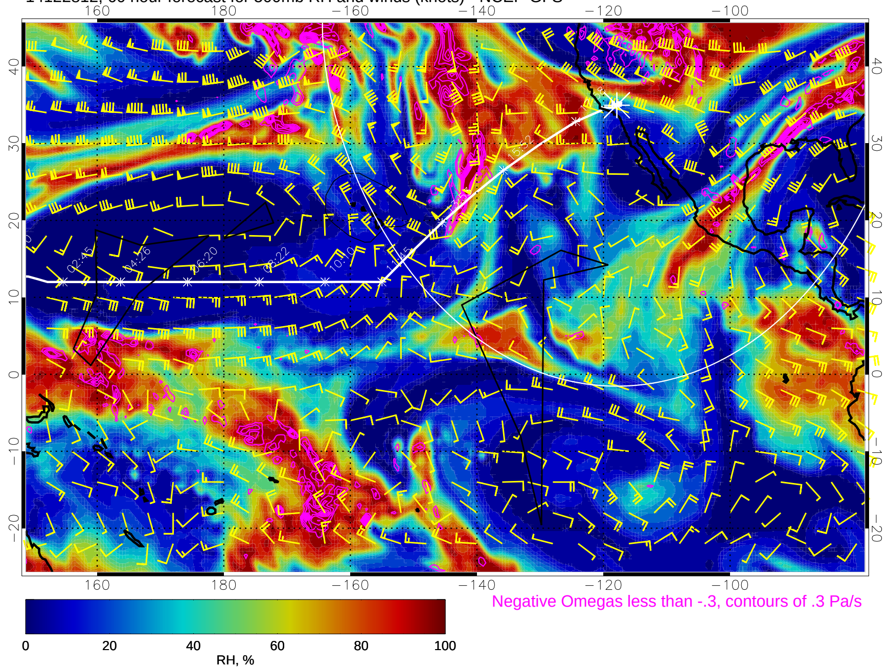
14122812, 60 hour forecast for 500mb RH and winds (knots) - NCEP GFS
