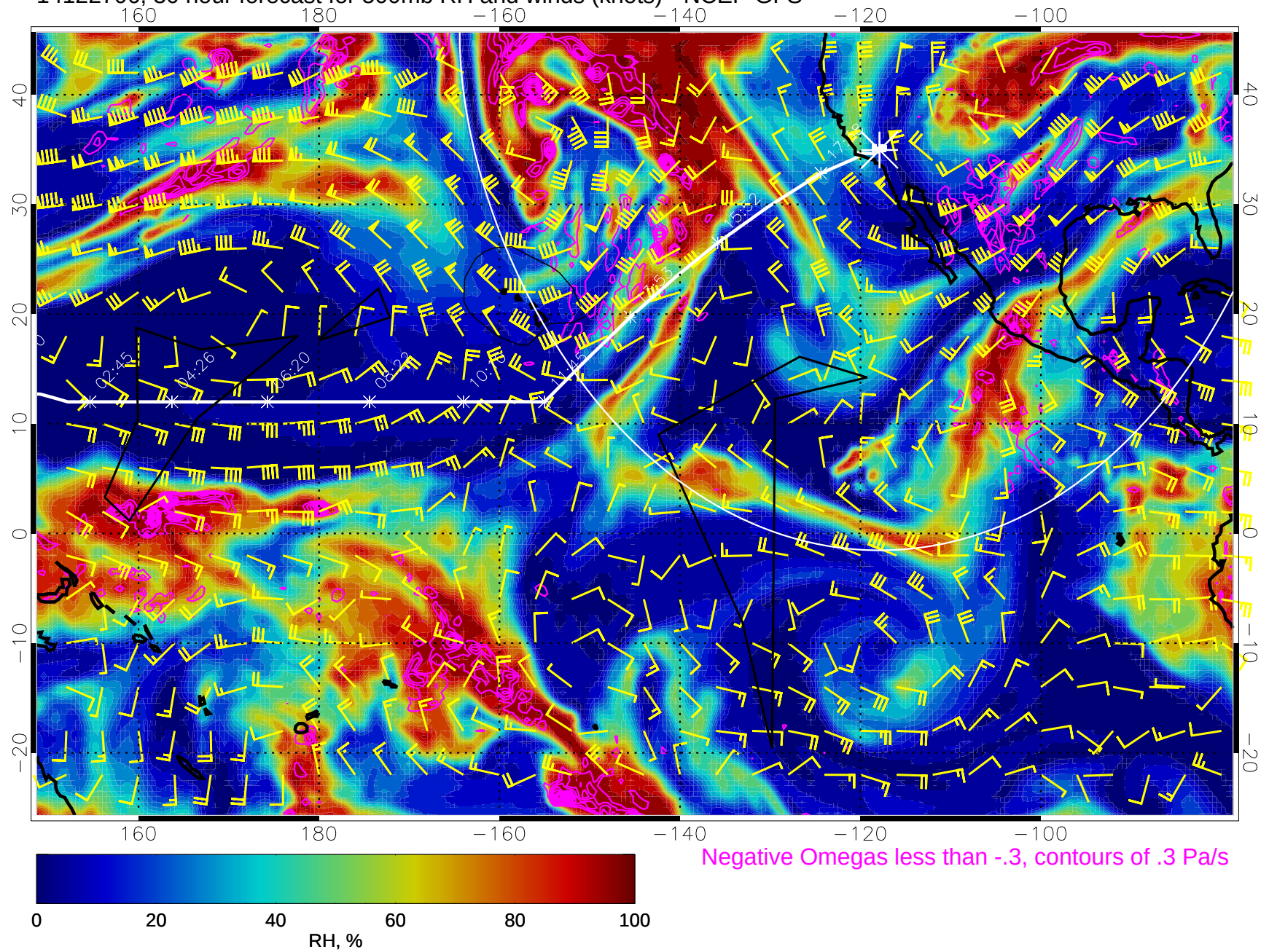
14122706, 30 hour forecast for 500mb RH and winds (knots) - NCEP GFS
