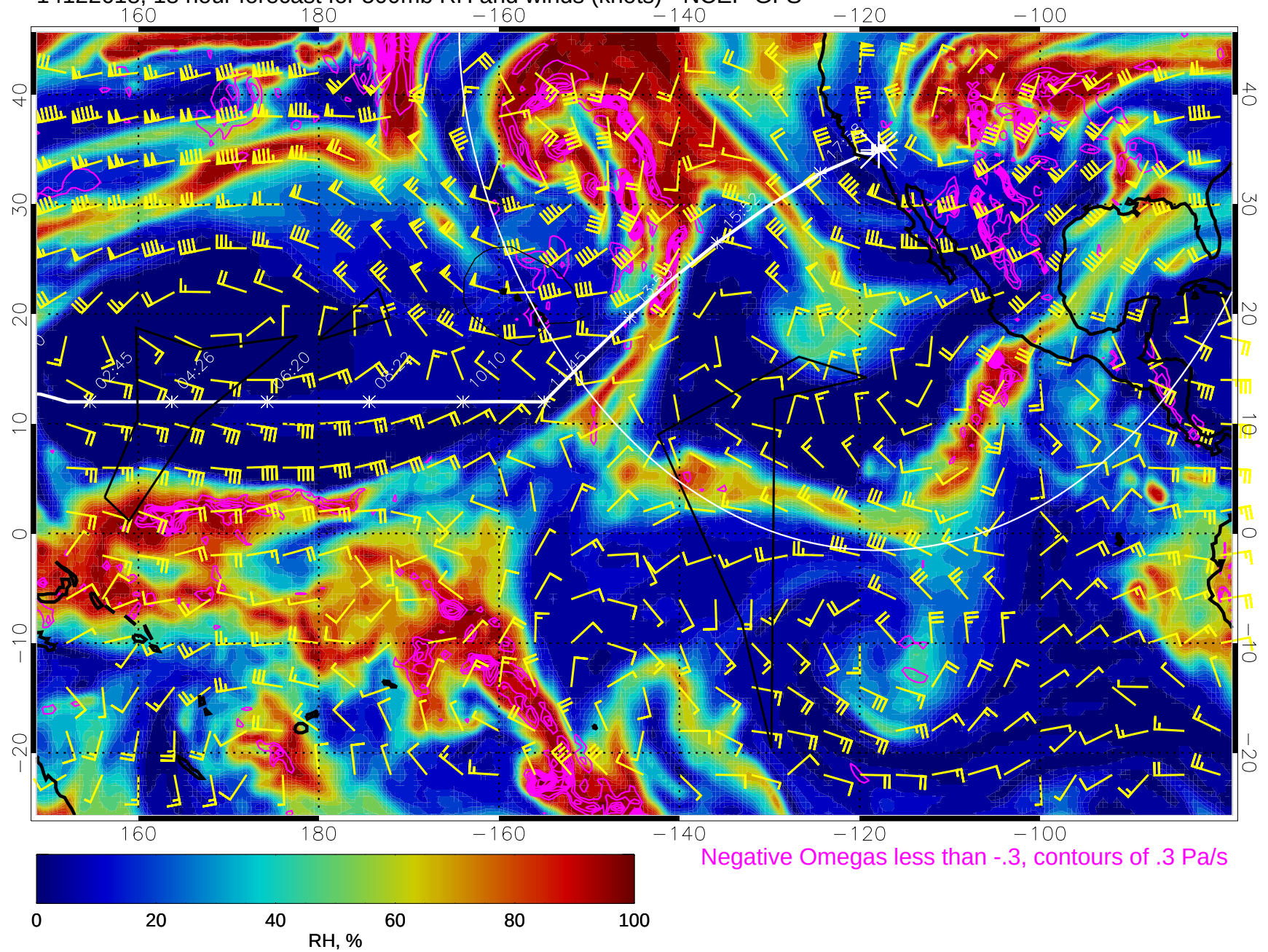
14122618, 18 hour forecast for 500mb RH and winds (knots) - NCEP GFS
