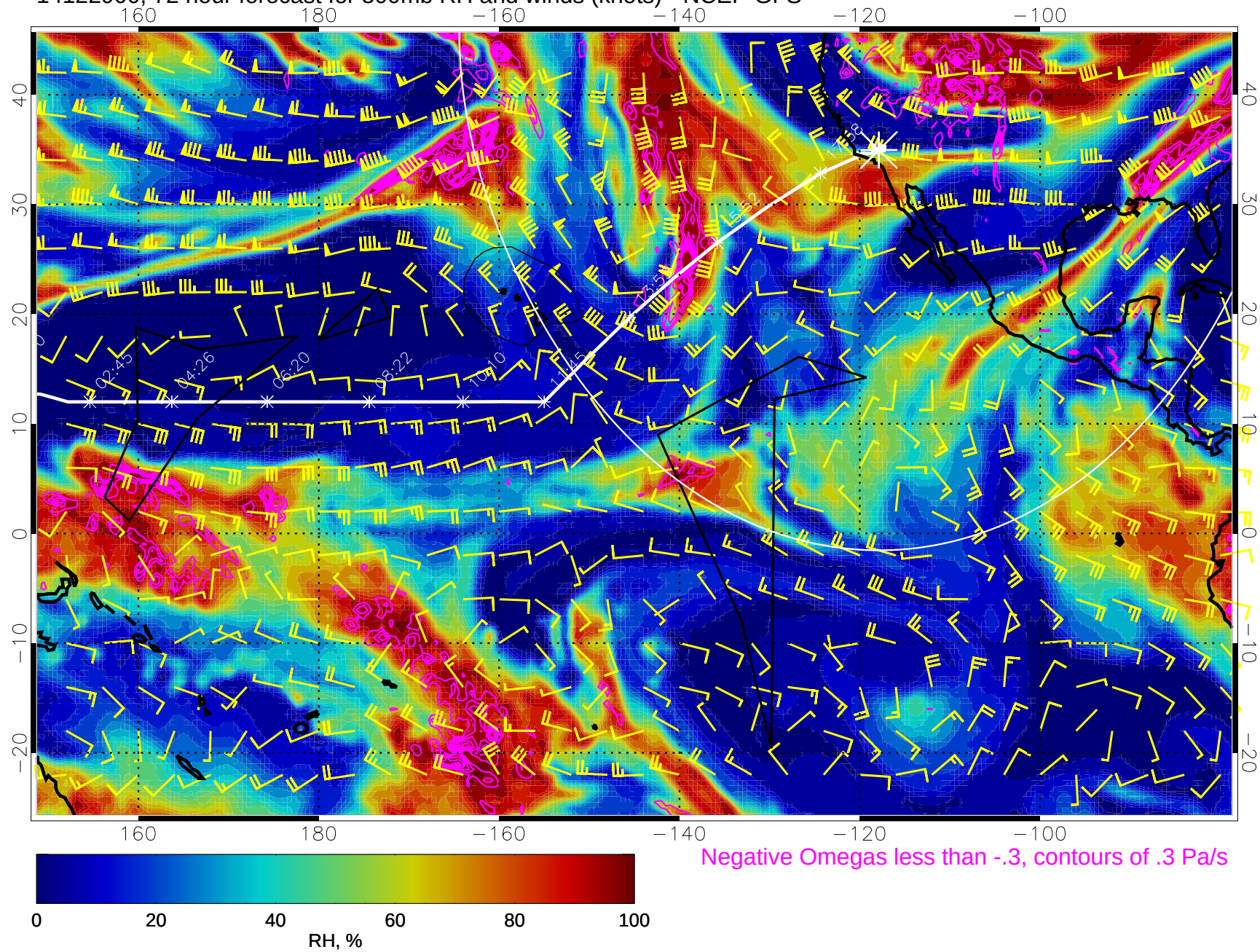
14122900, 72 hour forecast for 500mb RH and winds (knots) - NCEP GFS
