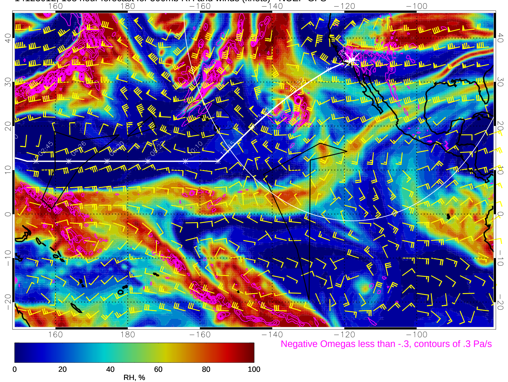
14123012, 108 hour forecast for 500mb RH and winds (knots) - NCEP GFS
