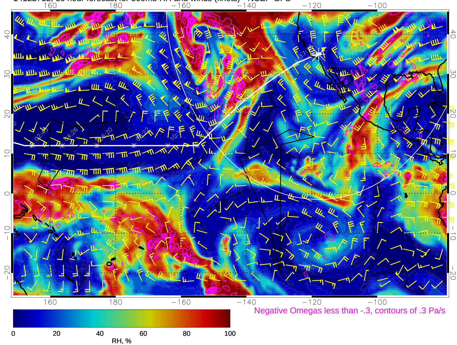
14122712, 36 hour forecast for 500mb RH and winds (knots) - NCEP GFS
