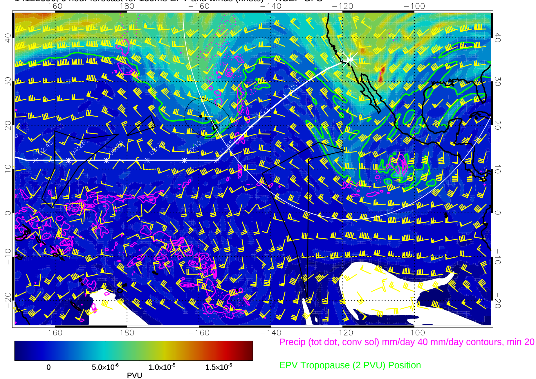
14122606, 6 hour forecast for 150mb EPV and winds (knots) -- NCEP GFS
